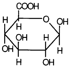
D-glucuronic acid
