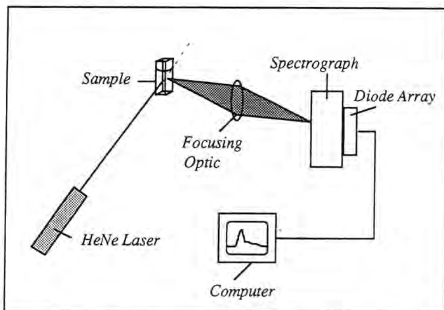
Figure 2.1. Experimental arrangement for recording emission spectra from phthalocyanine species emitting in the near-IR.
