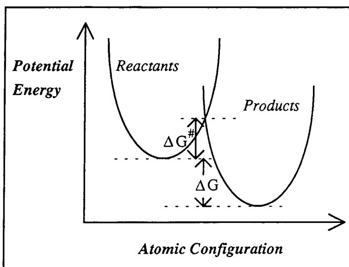
Figure 6.1. Potential energy profile of electron transfer [16] .
