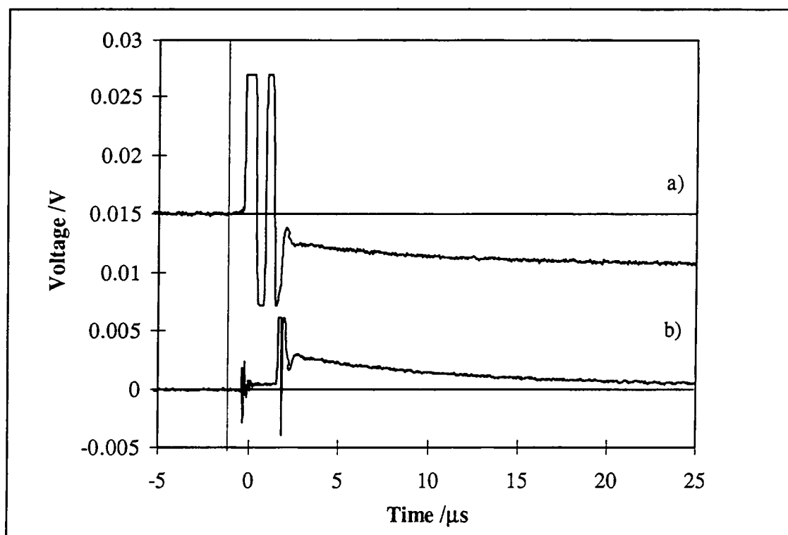
Figure A.7. ^1O_2 decay sensitised by phthalocyanine without (a) and with (b) the switch (offset for clarity).
