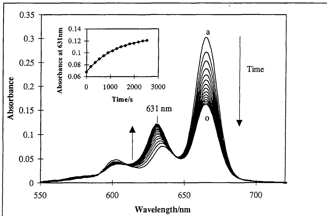
Figure 4.14. Rate of formation of (AlPc)_2F^- ( 2 \times 10^{-6} \text{ mol dm}^{-3} AlPcCl + 2.5 \times 10^{-5} \text{ mol dm}^{-3} F^- in MeOH). a) 'Zero' seconds, o) 2700 seconds (180 s intervals between traces). Dimer is characterised by growth of absorption at 631 nm.
