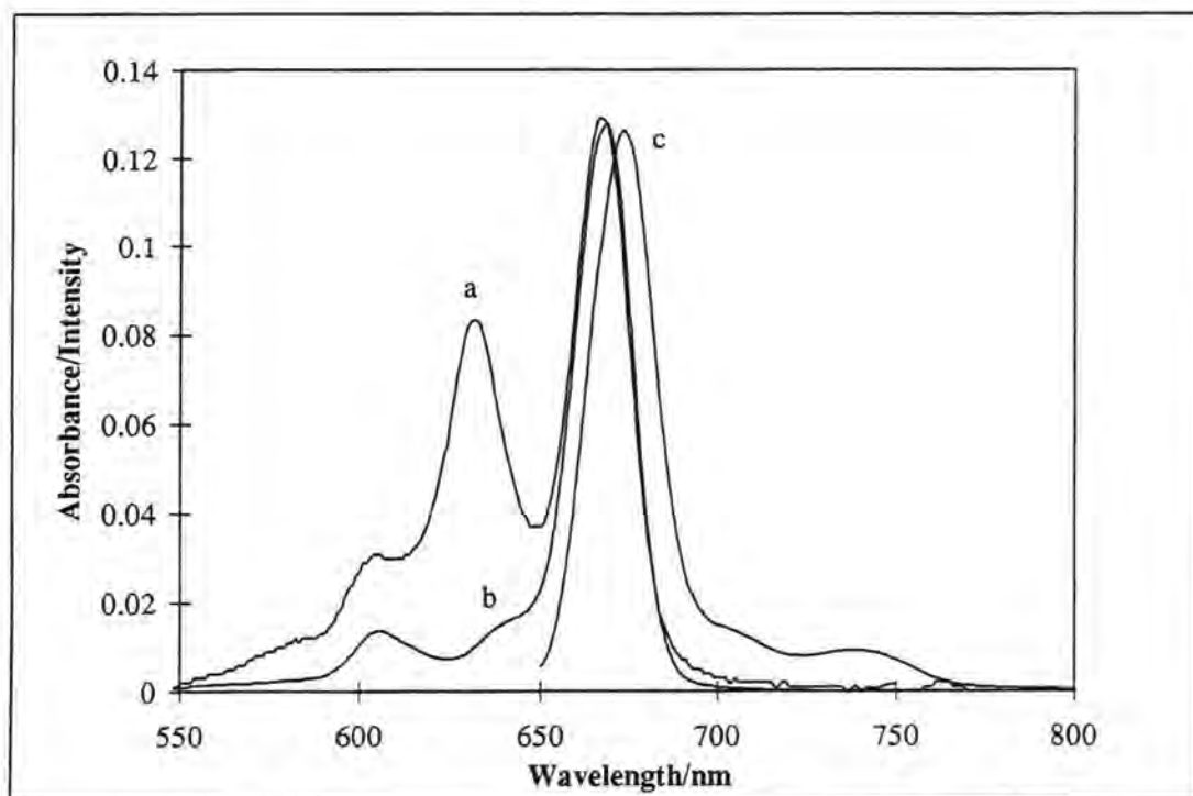
Figure 4.15. a) Absorption, b) Excitation ( \lambda_{em} = 760 nm) and c) Emission spectra ( \lambda_{ex} = 630 nm) of (AlPc)_2F^- ( 2 \times 10^{-6} mol dm -3 AlPcCl + 2.5 \times 10^{-5} mol dm -3 F - ) in MeOH.
