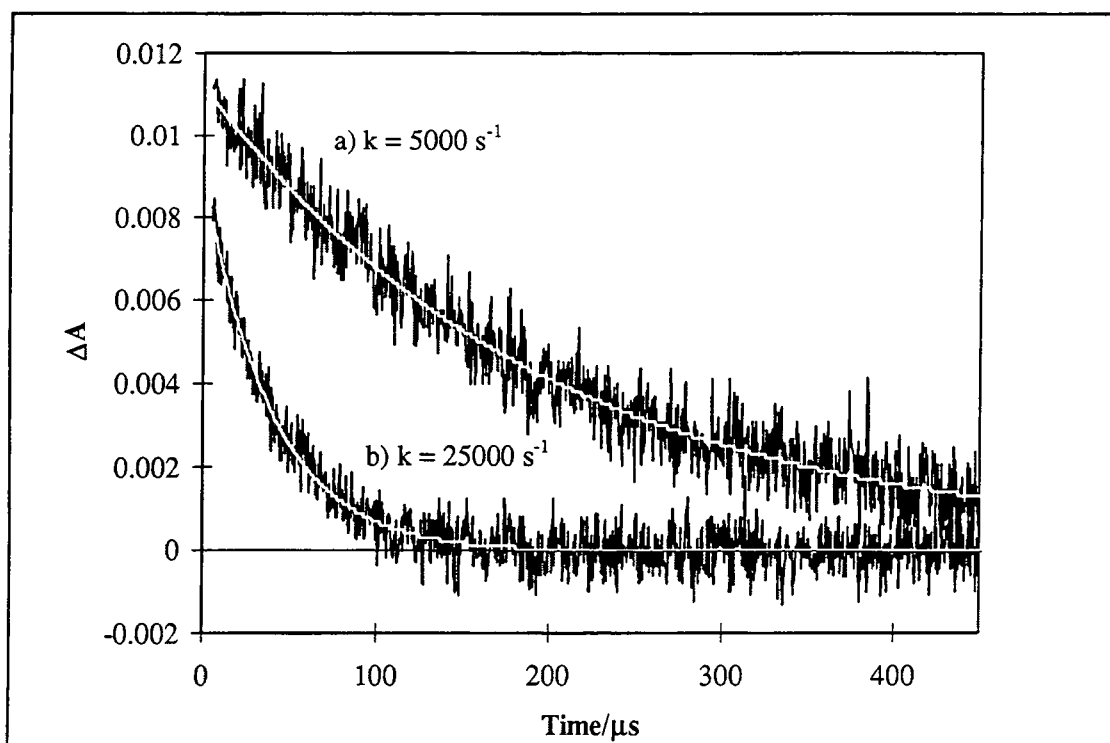
Figure 5.5. Triplet transient decays ( \lambda_{ex} = 355 \text{ nm} ). a) t\text{Bu}_4\text{ZnPc} (Probe = 490 nm) and b) t\text{Bu}_4\text{ZnPcH}^+ (Probe = 500 nm).
