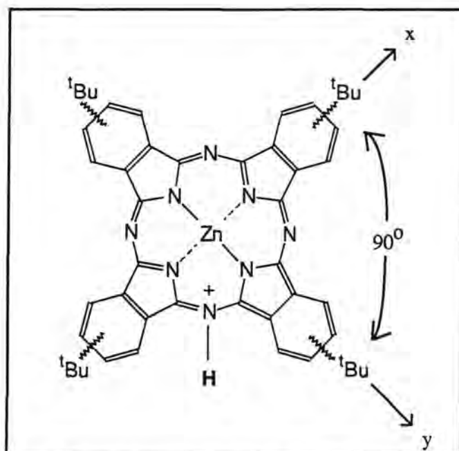
Figure 5.7. Structure of {}^t\text{Bu}_4\text{ZnPcH}^+ .
