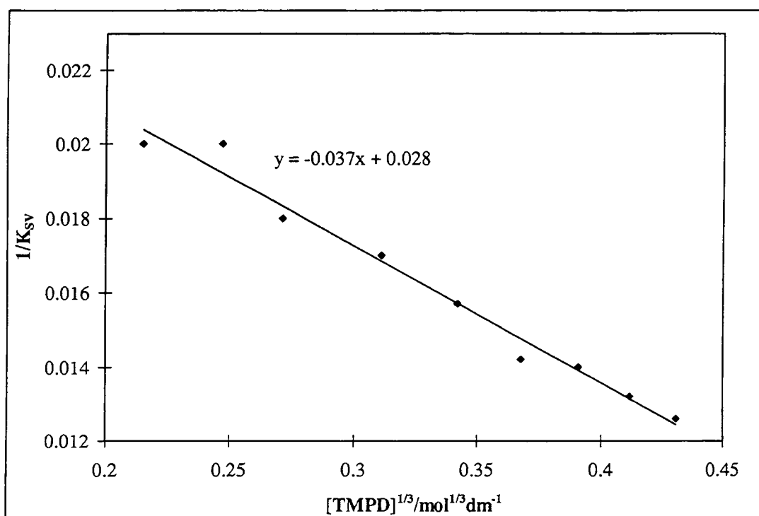
Figure 6.15. Application of finite sink approximation to TMPD quenching data.
