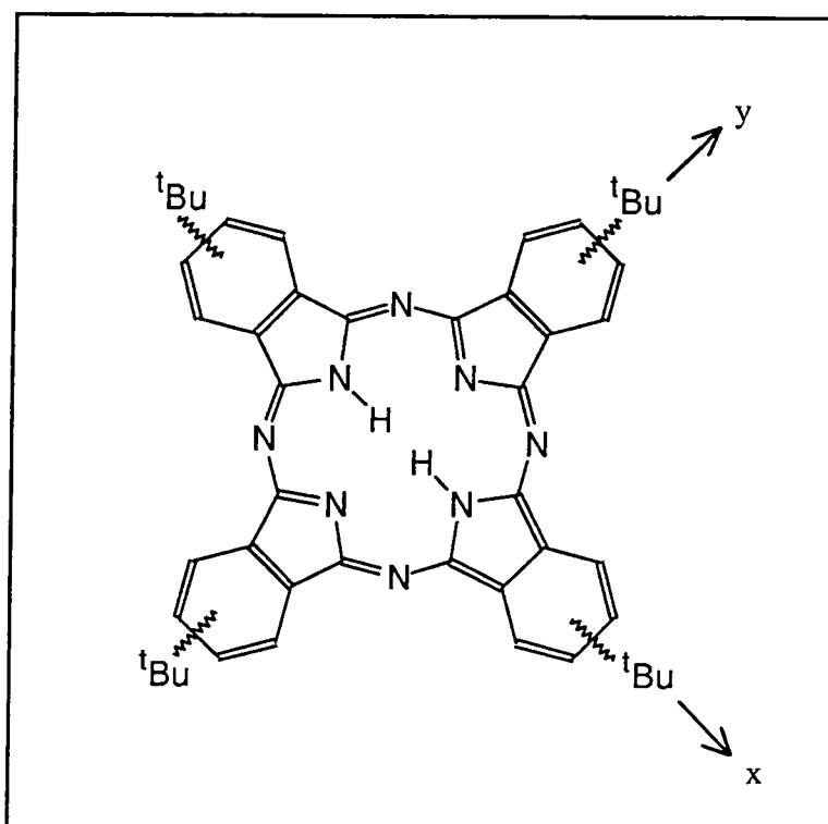
Figure 1.6. Structure of tetra t -butyl metal free phthalocyanine.
