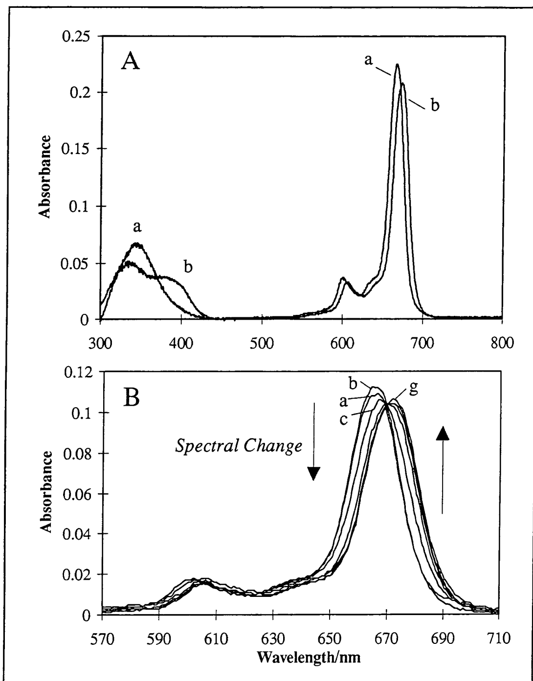
Figure 6.4. UV/Visible absorption spectra of \text{ZnPcS}_2 in \text{MeOH} + \text{CN}^- ions
