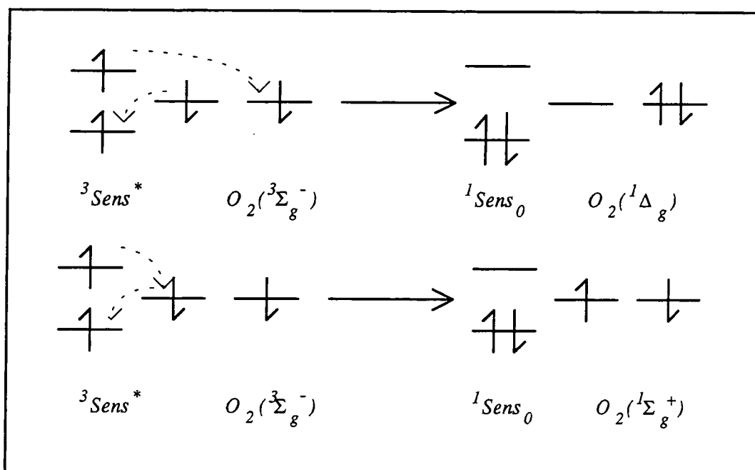
Figure 1.4. Formation of singlet oxygen.
