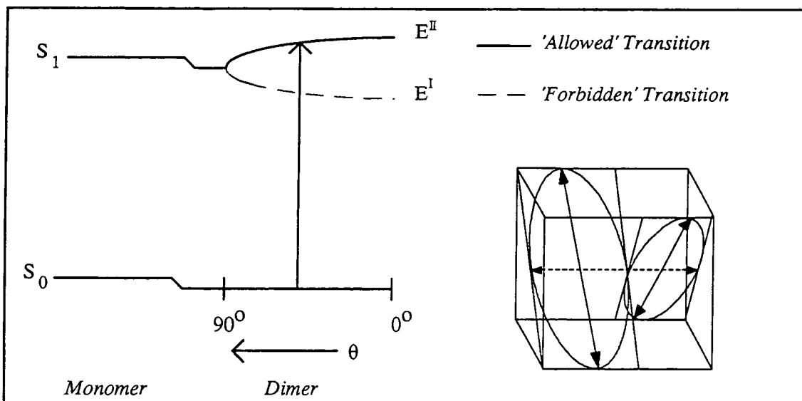
Figure 4.3. Exciton coupling of an 'out-of-plane' dimer [13] .
