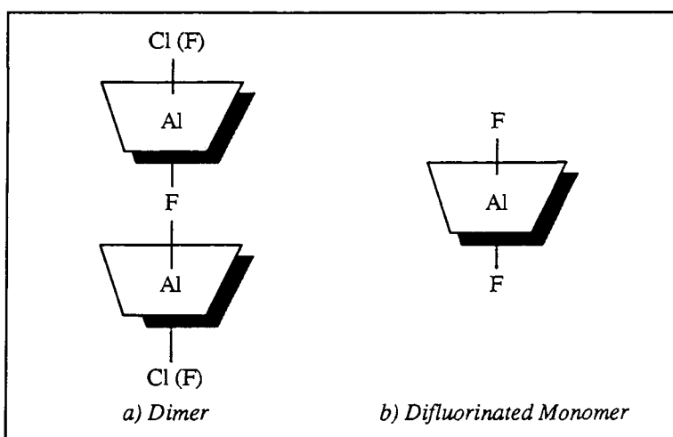
Figure 4.18. Geometry of (\text{AlPc})_2\text{F}^- dimer (a) and \text{AlPcF}_2^- monomer (b).
