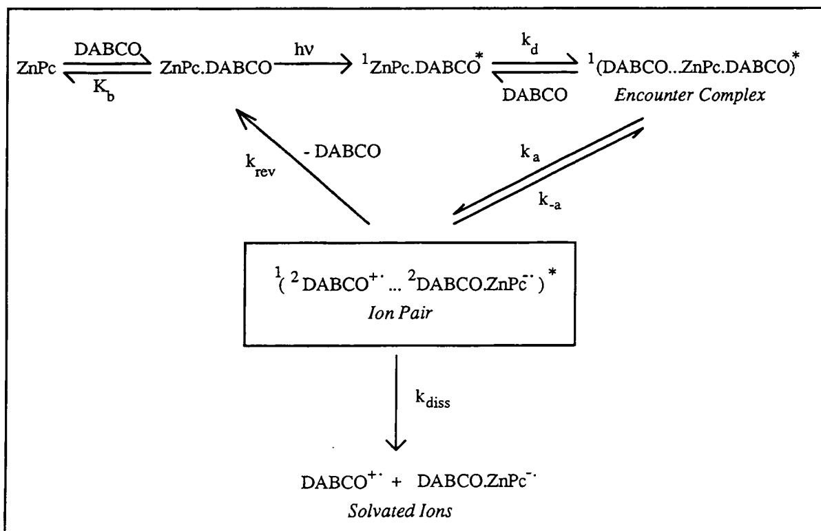
Figure 6.12. Formation of DABCO...ZnPc.DABCO ion pair upon irradiation of ZnPc in 1% pyr/tol in the presence of > 0.01 \text{ mol dm}^{-3} DABCO.
