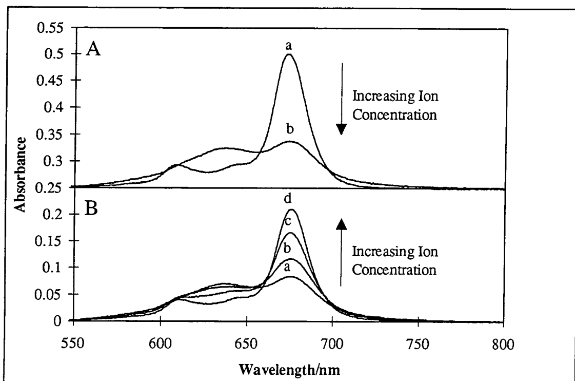
Figure 3.2. A. Aggregation of ZnPc(CHMeCO 2 H) 4 in EtOH induced by potassium acetate. a. \sim 0 \text{ mol dm}^{-3} b. 10^{-4} \text{ mol dm}^{-3} .
