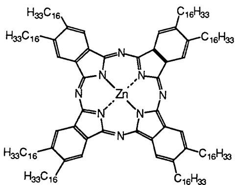
ZnC16
