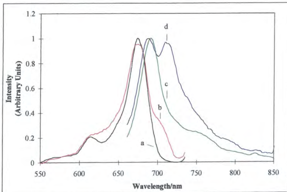
Figure 5.16. Fluorescence excitation spectra of a) t\text{Bu}_4\text{ZnPc} and b) \text{ZnPcS}_2 on cellulose ( \lambda_{em} = 740 \text{ nm} ).
