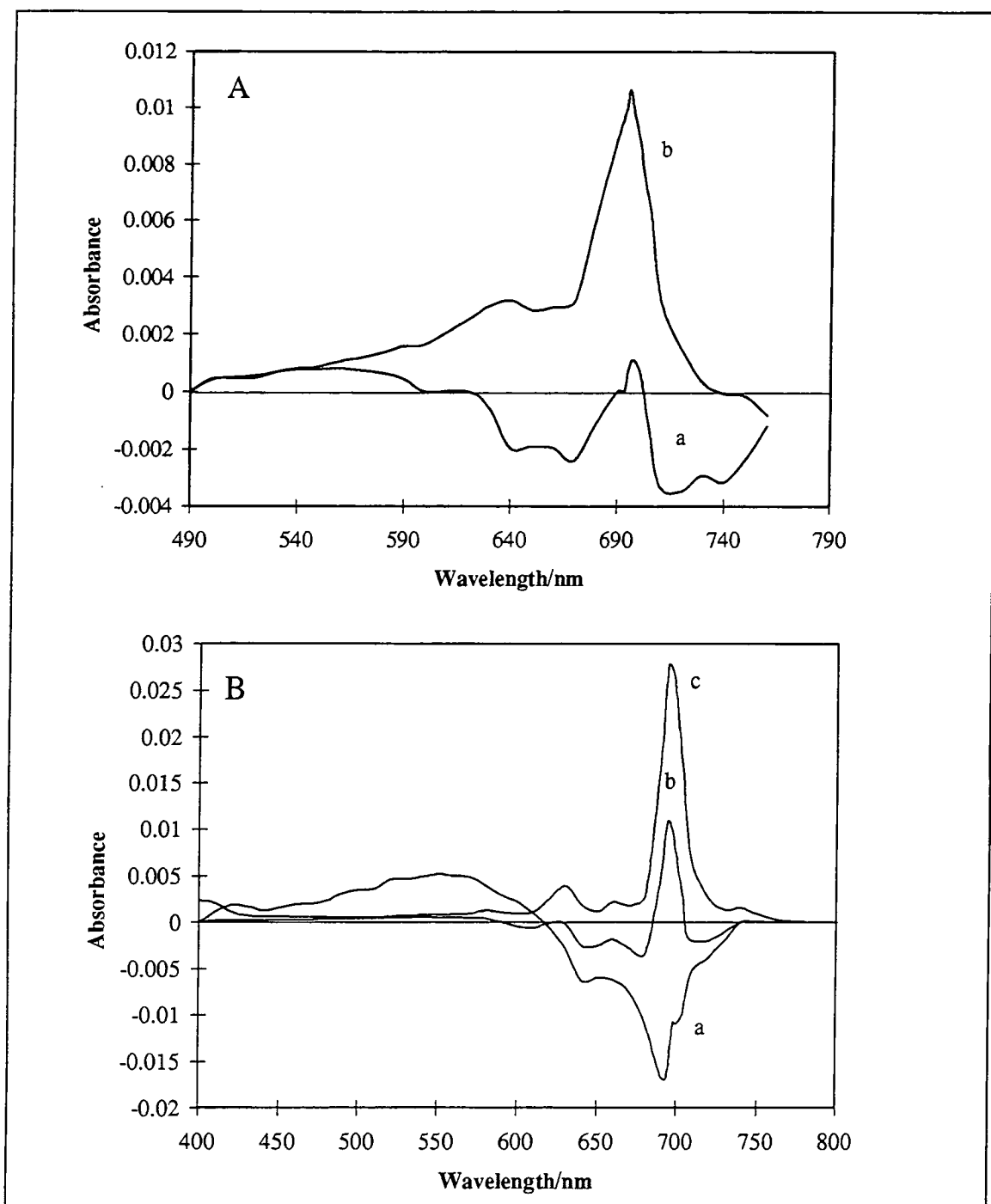
Figure 4.25. Transient absorption spectra of C10 in EPA ( \lambda_{ex} = 638 nm). A. 77 K, a) 10 \mu s after excitation, b) Trace a corrected for ground state absorption. B. 200 K, a) 10 \mu s after excitation, b) 300 \mu s after excitation, c) Trace b corrected for ground state absorption.
