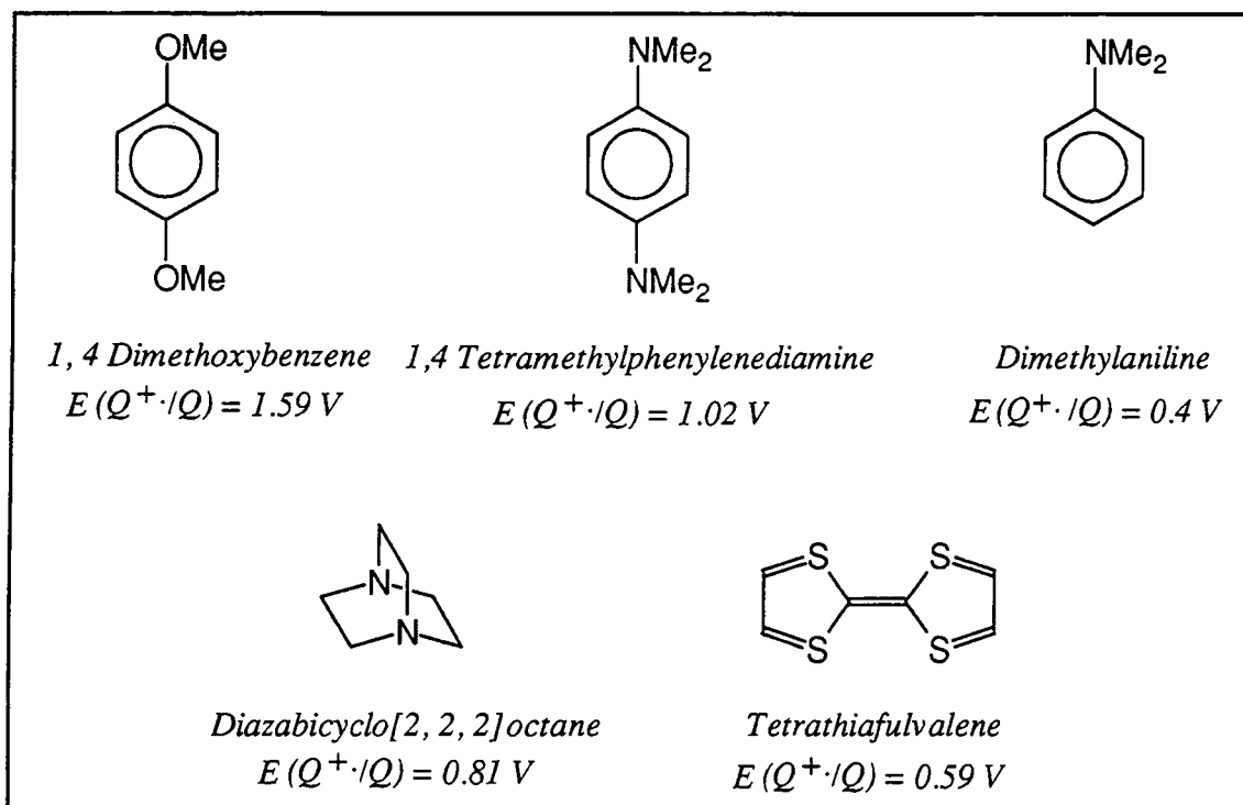
Figure 6.10. Structure of simple organic quenchers.
