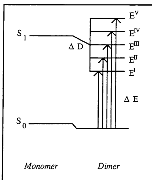
Figure 4.27. Energy level splitting of C10 in EPA at 77 K.
