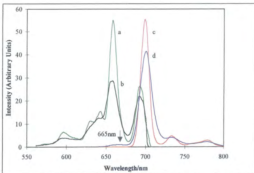
Figure 4.6. Temperature dependence of fluorescence excitation ( \lambda_{em} = 760 \text{ nm} ) a) 77 K, b) 293 K and emission spectra ( \lambda_{ex} = 630 \text{ nm} ), c) 77 K, d) 293 K, of t\text{Bu}_4\text{H}_2\text{Pc} in EPA.
