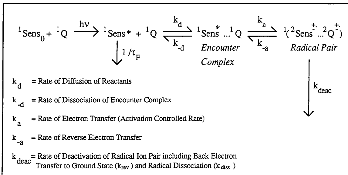
Figure 6.2. Processes involved in fluorescence quenching by electron transfer [16] .
