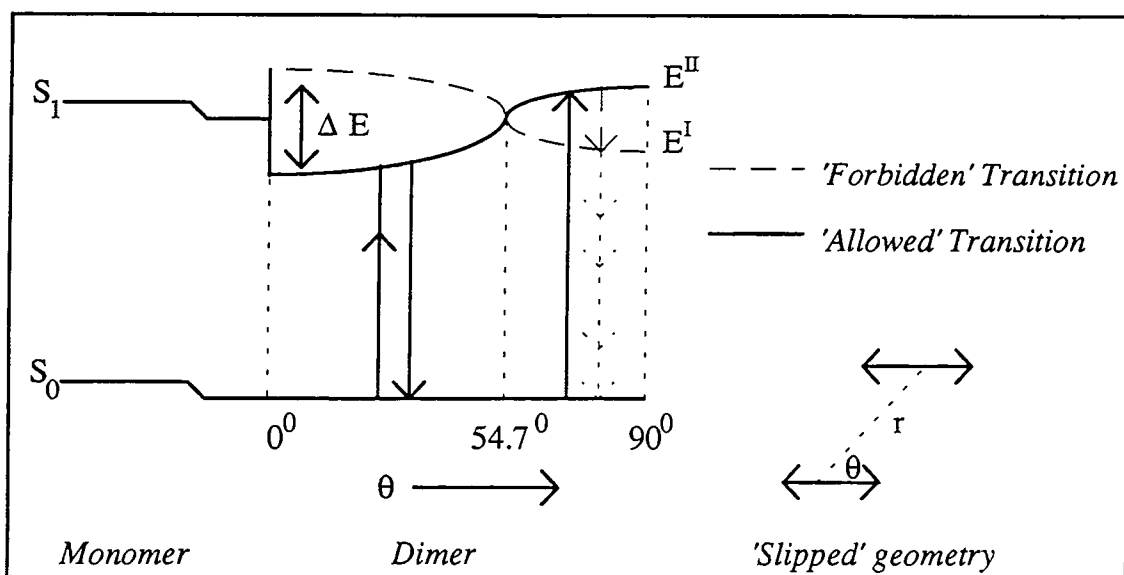
Figure 4.1. Energy level splitting on exciton coupling of a 'slipped' dimer [13] .
