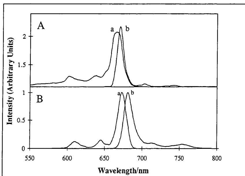
Figure 3.8. a) Excitation ( \lambda_{em} = 750 nm) and b) Emission ( \lambda_{ex} = 630 nm) spectra at 77 K. A. \text{ZnPcS}_2 in EtOH, B. \text{ZnPc}(\text{CMe}(\text{CO}_2\text{Me})_2)_4 in EPA. Spectra are offset for clarity and have been normalised at \lambda_{max} .
