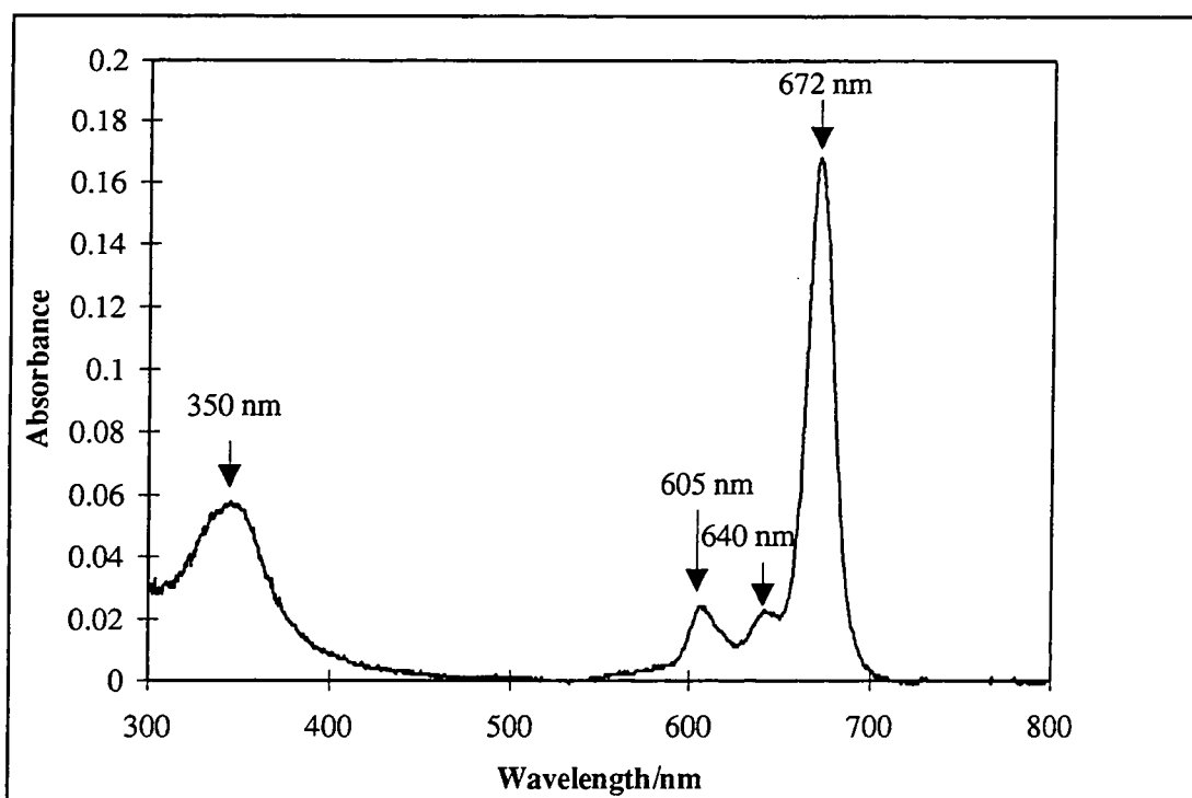
Figure 1.5. UV/Visible absorption spectrum of ZnPc in 1% pyridine/toluene solution.
