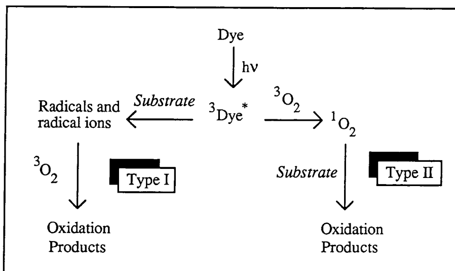
Figure 1.3. Destructive pathways of PDT.
