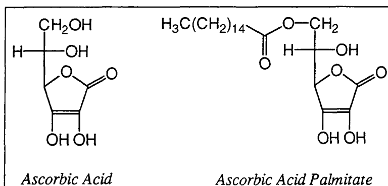
Figure 6.22. Structures of ascorbic acid (AA) and ascorbic acid palmitate (AAP).
