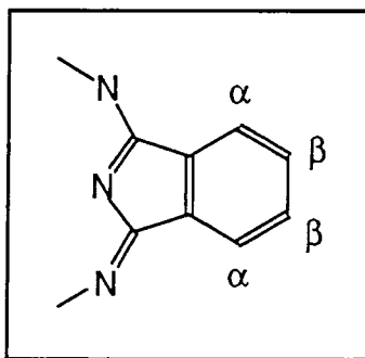
Figure 3.9. \alpha and \beta positions of zinc phthalocyanine.
