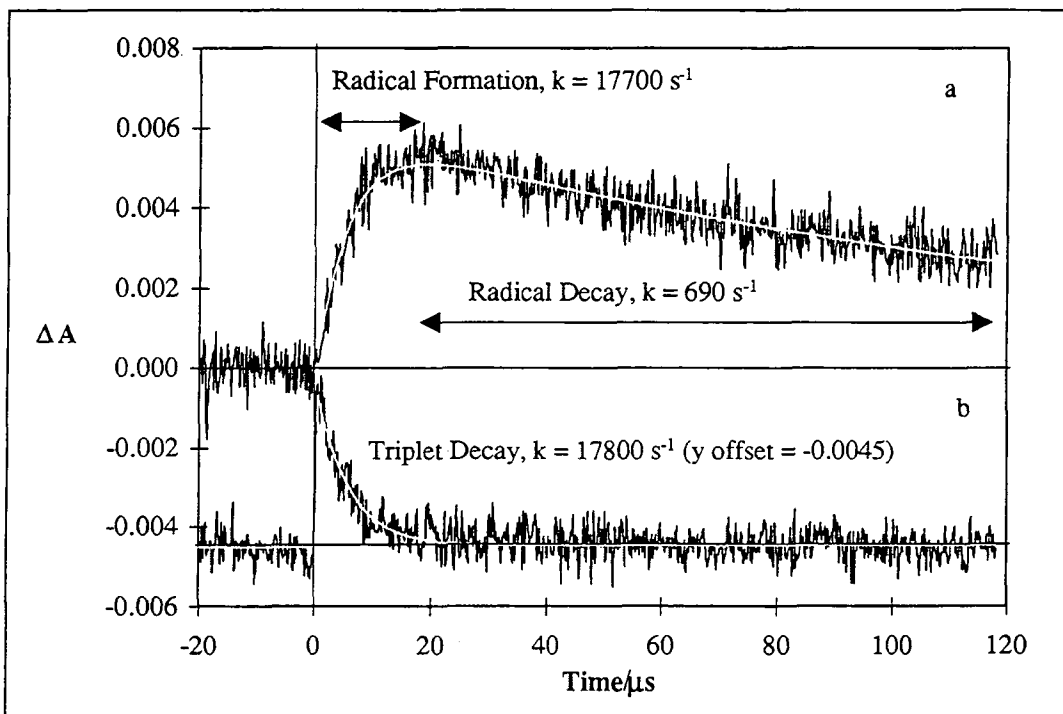
Figure 6.24. Transient study of {}^t\text{Bu}_4\text{ZnPc} in MeOH + 0.01 \text{ mol dm}^{-3} ascorbic acid palmitate, \lambda_{ex} = 638 \text{ nm} . Deactivation of triplet species (b) (probe wavelength = 490 \text{ nm} ) and formation and decay of \text{Pc}^{\cdot-} radical (a) (probe wavelength = 600 \text{ nm} ). Decays have been offset for clarity.
