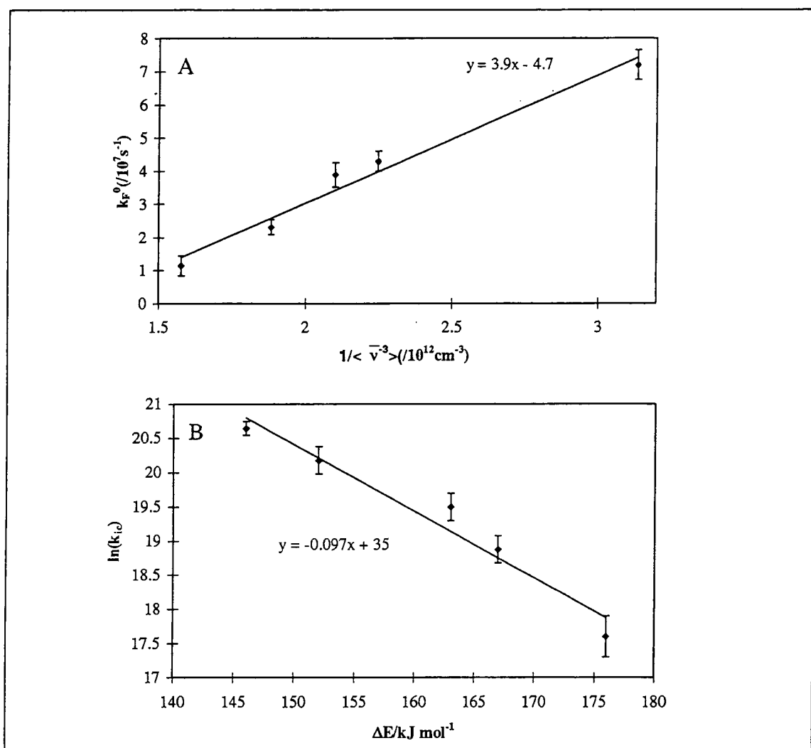
Figure 5.8. Dependence of k_F^0 and k_{ic} on \Delta E ( S_1 \leftarrow S_0 ) of \text{PcH}_n^{n+} .
