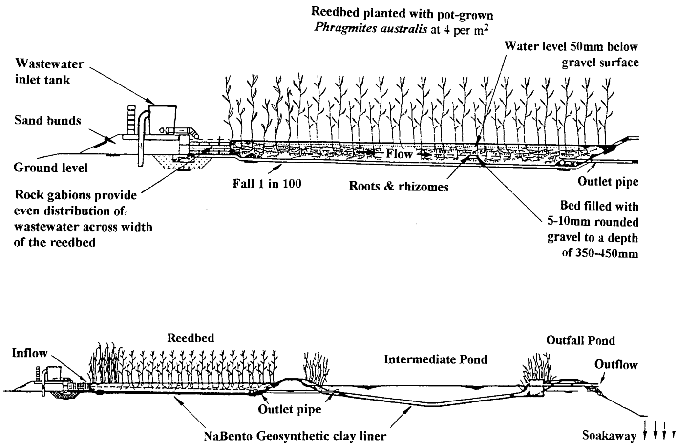
Figure 3. Cross-sections through the CATS Terminal horizontal subsurface-flow reedbed system
