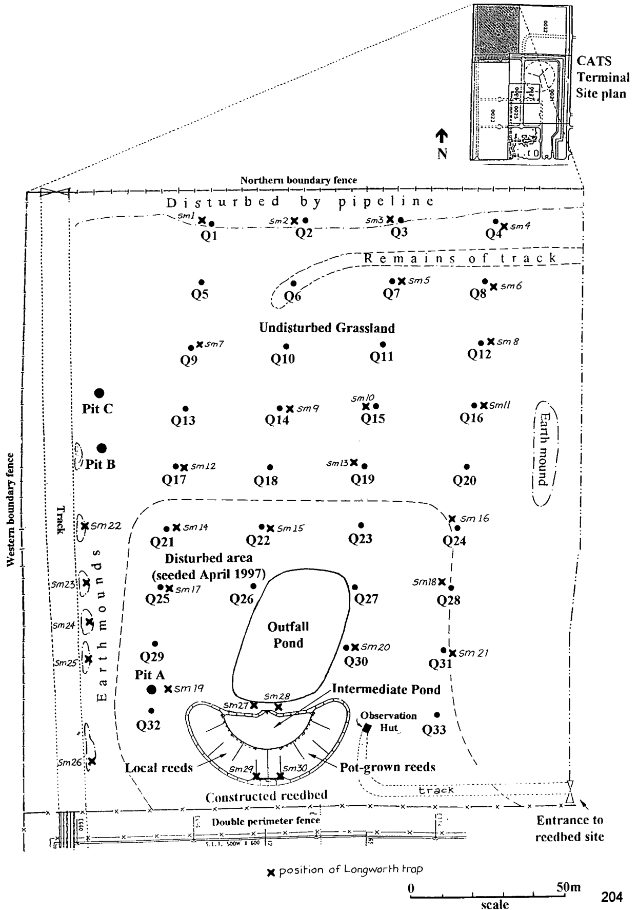
Figure 50. CATS Terminal constructed reedbed and grassland site showing location of Longworth traps.
