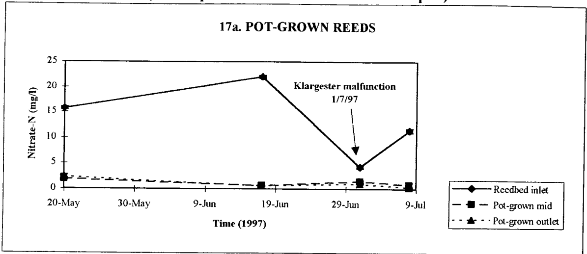
Figure 17. Graphs to show the nitrate-N (mg/l) content of water samples from the CATS Terminal reedbed between 20/5/97-9/7/97 (data represent the mean +/- SE of 3 samples)
