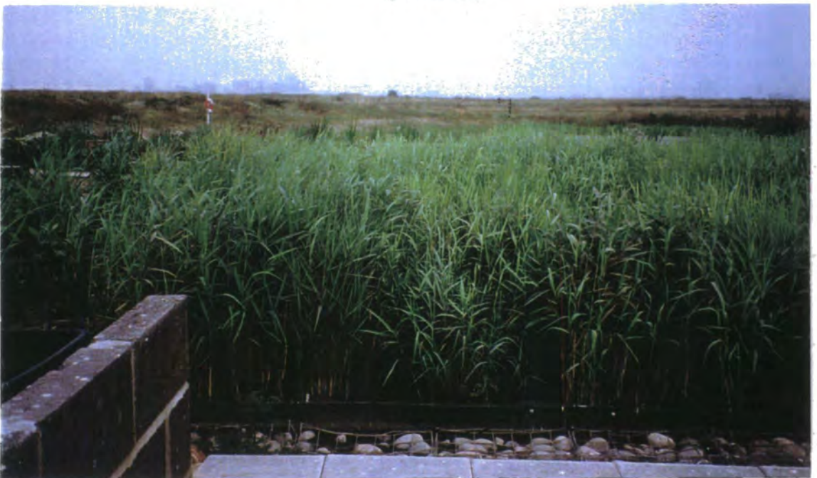
Plate 16. Pot-grown Phragmites australis inlet section of the CATS Terminal reedbed, August 1997, showing shoot-density of individually planted specimens.
