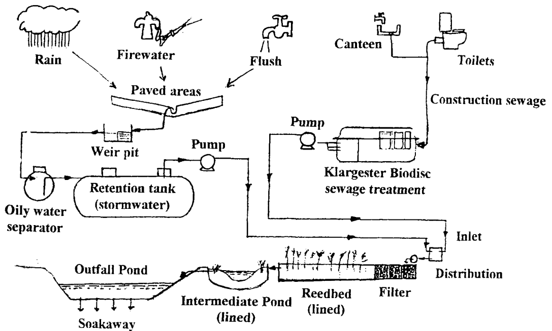
Figure 2. Sources of influent wastewater to the CATS Terminal reedbed.
