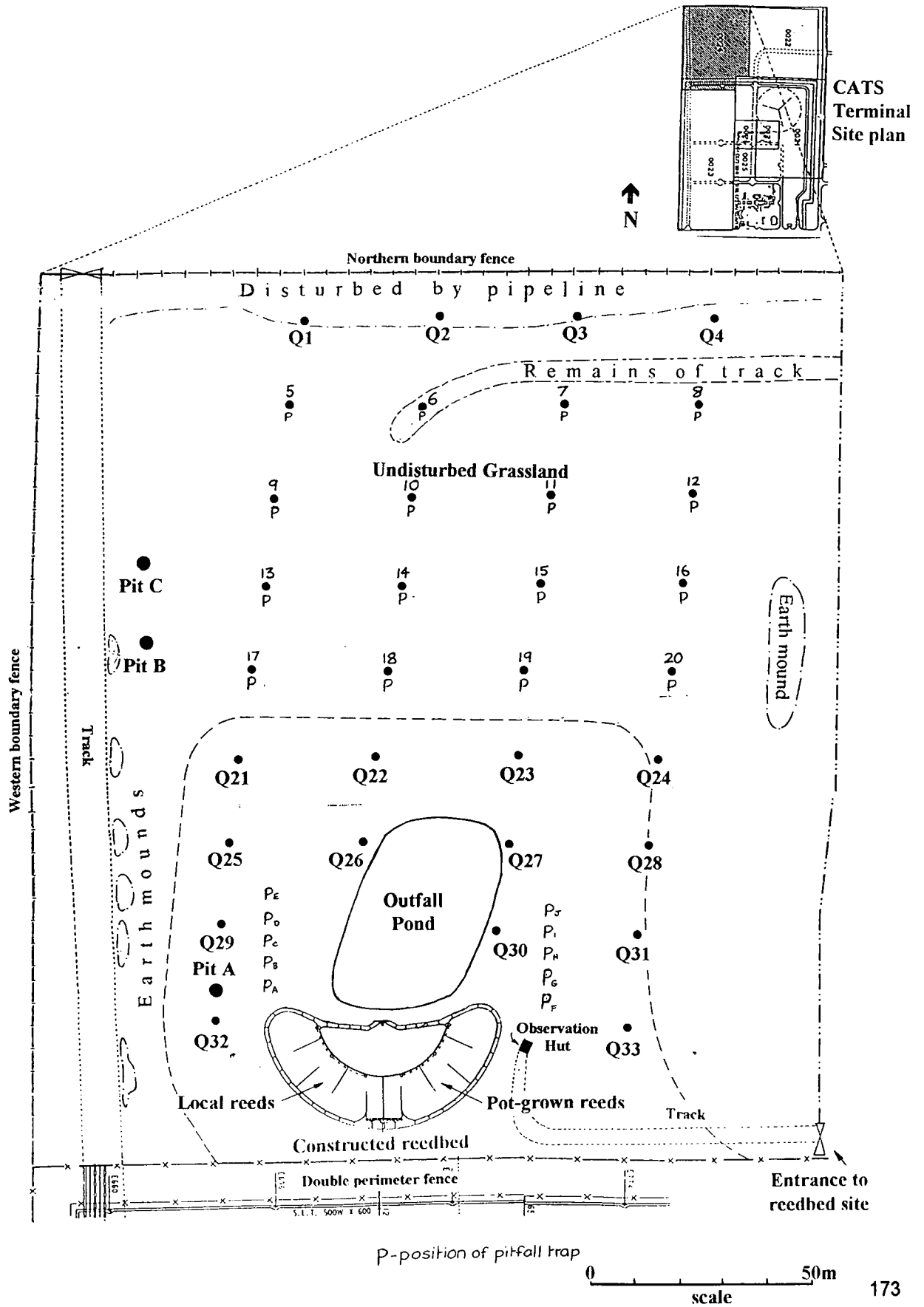
Figure 44. CATS Terminal constructed reedbed and grassland site showing location of pitfall traps.
