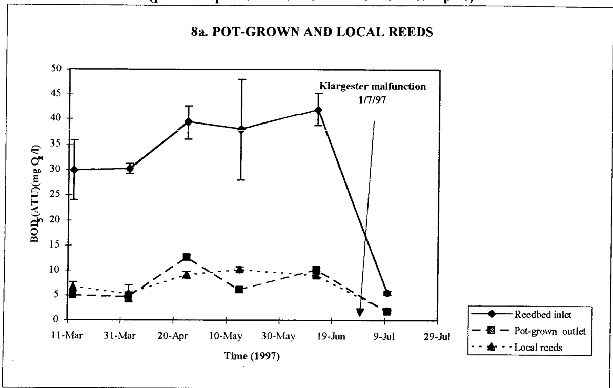
Figure 8. Graphs to show the BOD 5 (ATU)(mg O 2 /l) of water samples from the CATS Terminal reedbed between 13/3/97- 10/7/97 (points represent the mean +/- SE of 3 samples)
