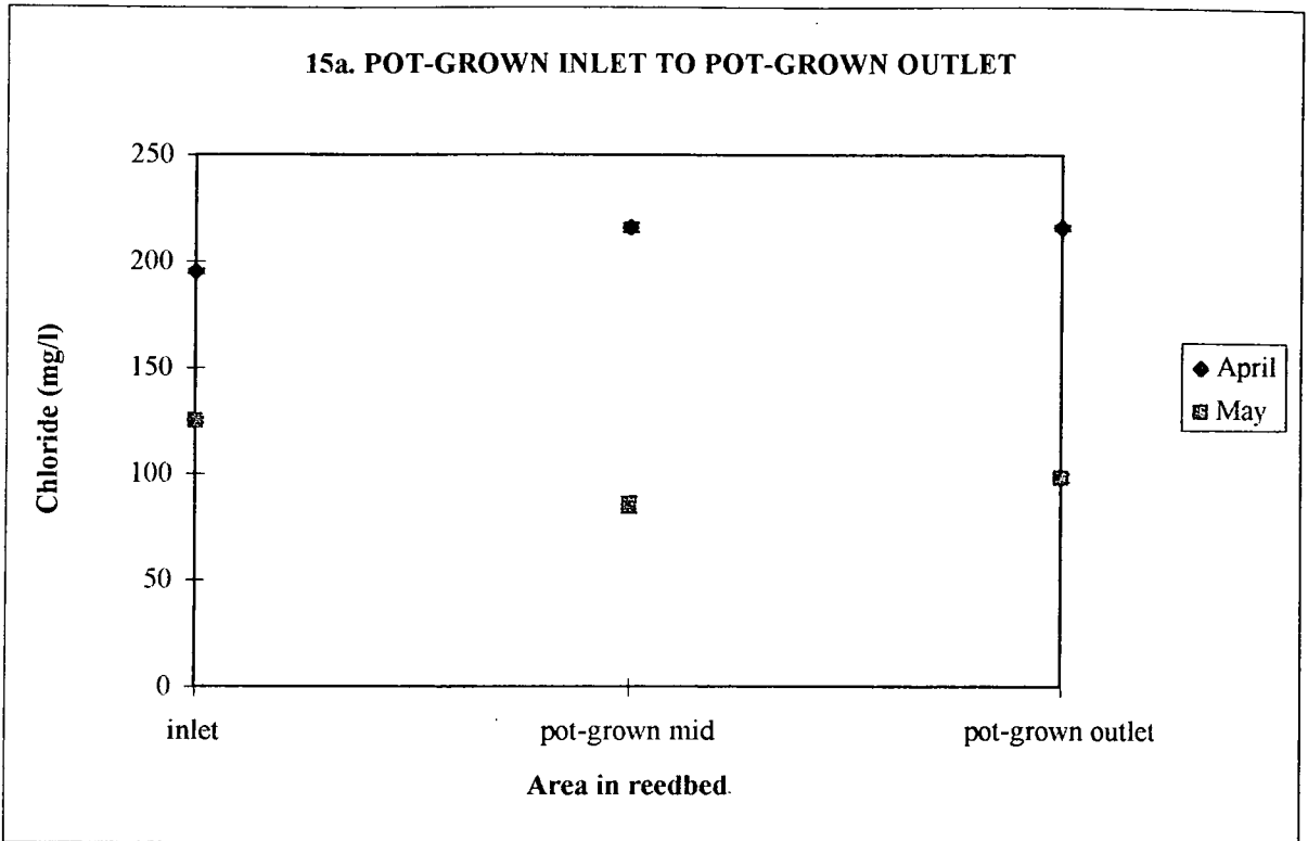
Figure 15. Graphs to show the chloride (mg/l) content of water samples from the CATS Terminal reedbed on 21/4/97 & 21/5/97 (data represent the mean +/- SE of 3 samples)
