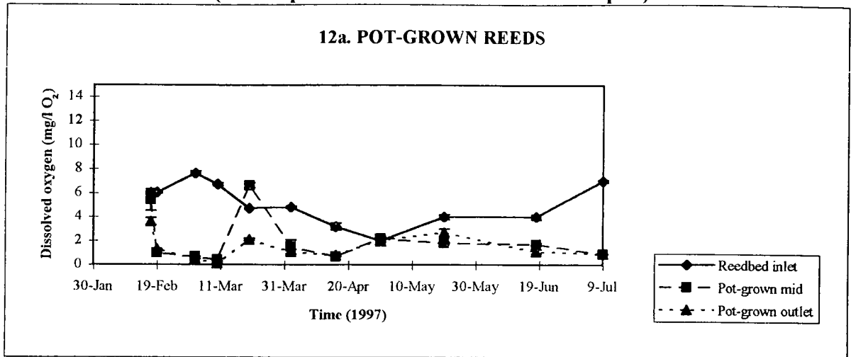
Figure 12. Graphs to show the Dissolved oxygen content (mg/l O 2 ) of water samples from the CATS Terminal reedbed and the ICI No.6 brinefield between 17/2/97-9/7/97 (data represent the mean +/- SE of 3 samples)
