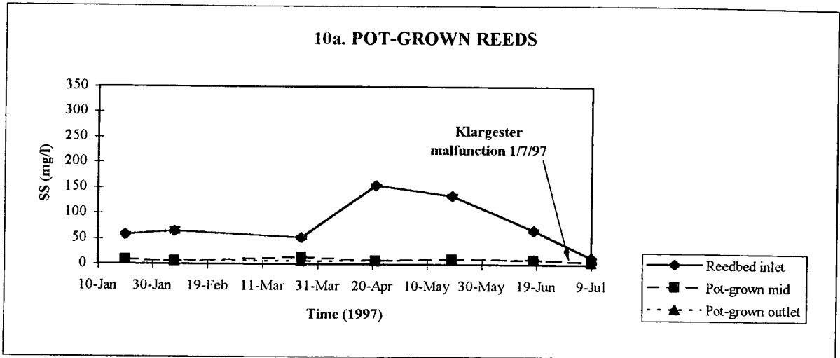
FIGURE 10. Graphs to show the Suspended Solids (mg/l) from the CATS Terminal reedbed between 20/1/97 - 9/7/97 (data represent the mean +/- SE of 3 samples)
