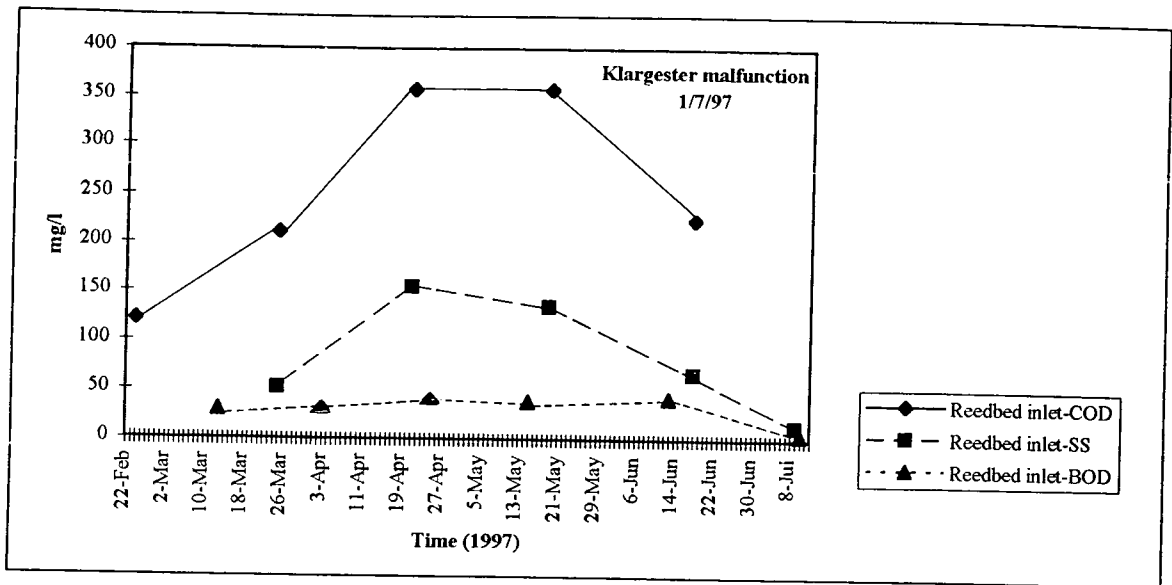
Figure 11. Graph to show the relationship between SS, BOD 5 & COD (mg/l) of inlet water samples from the CATS Terminal reedbed between 25/2/97-10/7/97
