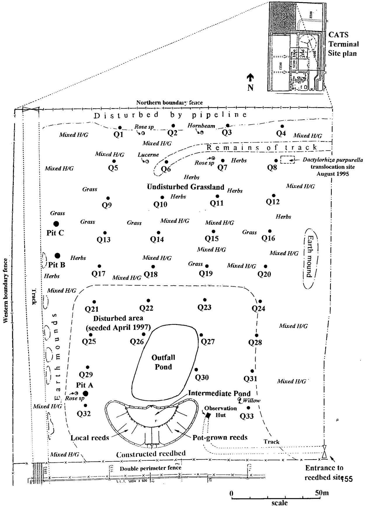
Figure 40. CATS Terminal constructed reedbed and grassland site showing distribution of vegetation communities.
