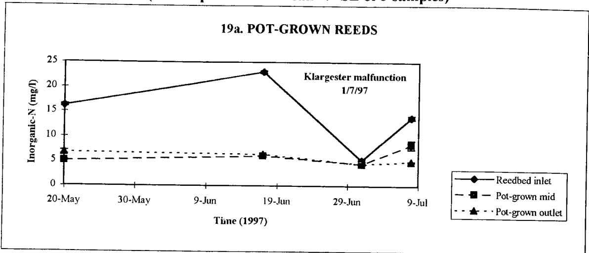
Figure 19. Graphs to show the inorganic-N (mg/l) content of water samples from the CATS Terminal reedbed between 20/5/97-9/7/97 (data represent the mean +/- SE of 3 samples)
