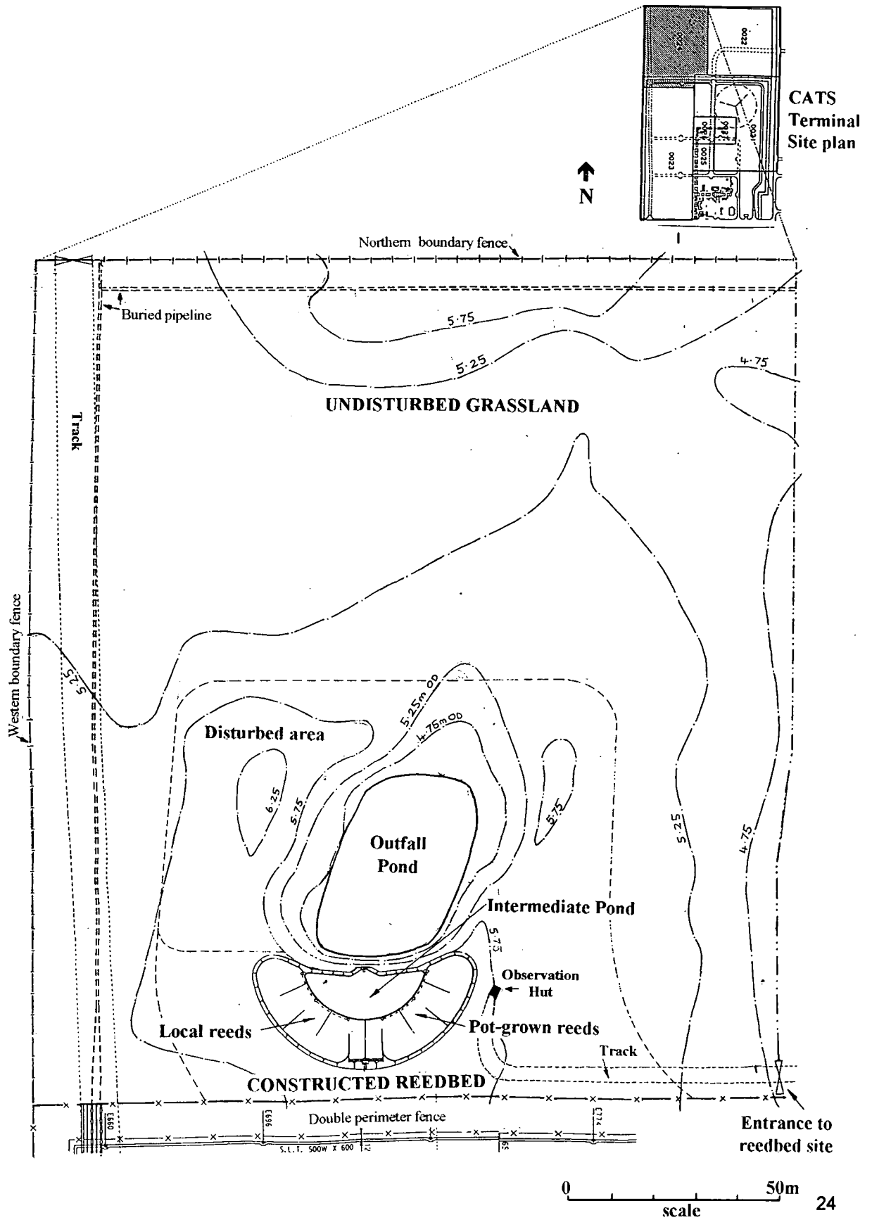
Figure 4. CATS Terminal constructed reedbed and grassland site. (Adapted from CATS Terminal Project drawing no.7983-15/00/00/40/252/0024)
