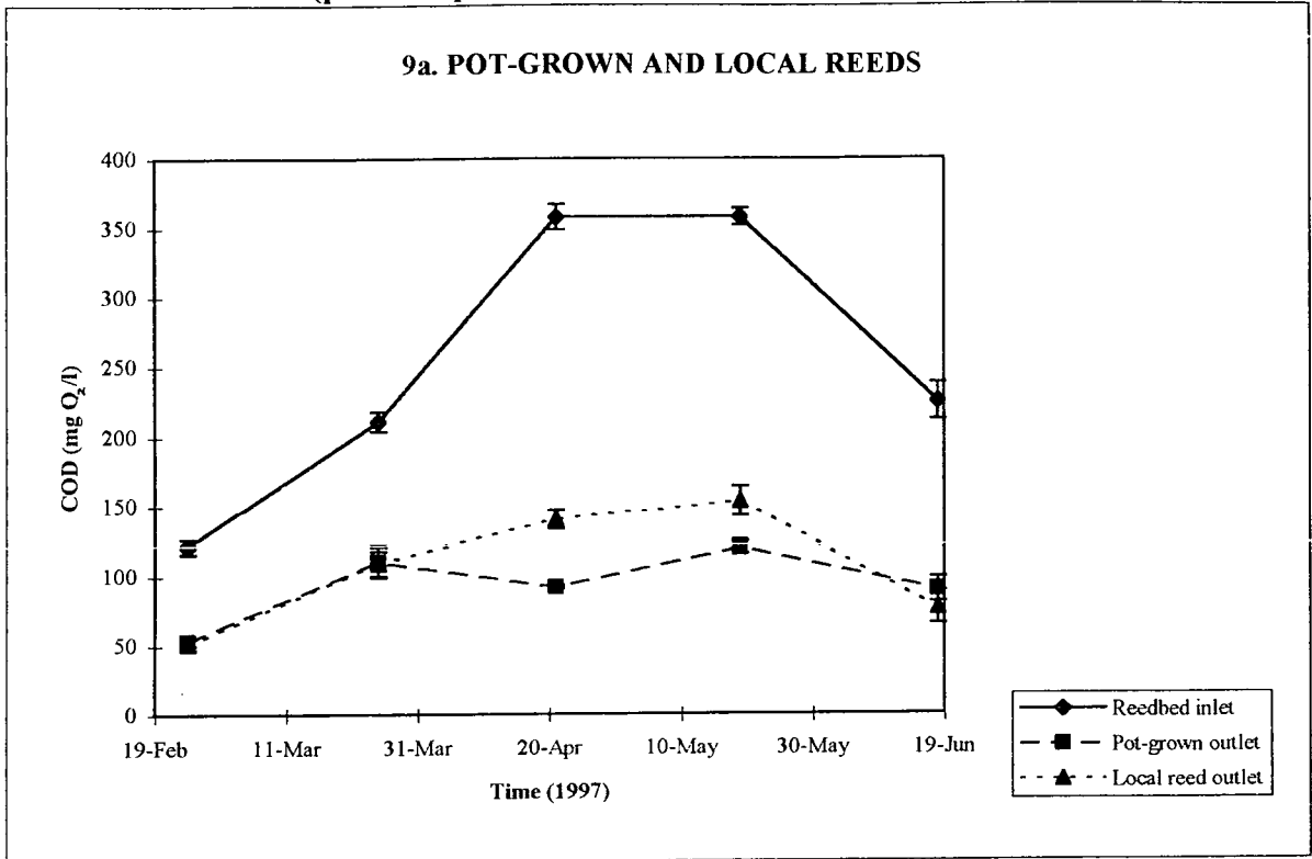
Figure 9. Graphs to show the COD (mg O 2 /l) of water samples from the CATS Terminal reedbed between 25/2/97 - 18/6/97 (points represent the mean +/- SE of 3 samples)
