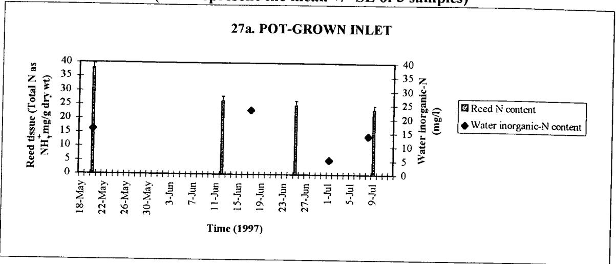
Figure 27. Nitrogen content in water and reed leaf tissue in the pot-grown section of the CATS Terminal reedbed between 20/5/97-9/7/97 (data represent the mean +/- SE of 3 samples)
