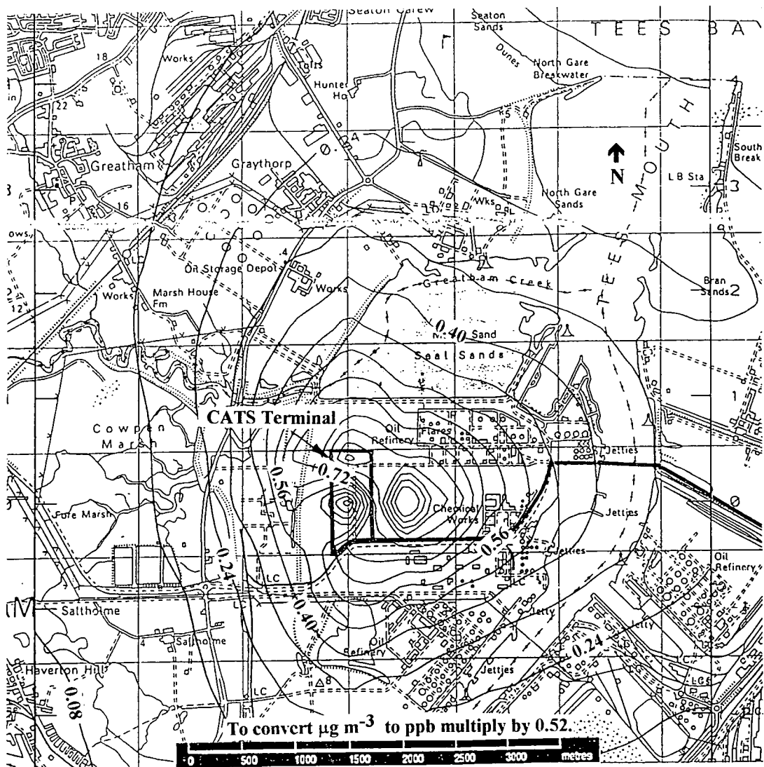
Figure 33. Predicted isopleths showing the contribution of the gas processing plant to the NO x annual average ground level concentration ( \mu\text{g m}^{-3} ). (Amoco CATS Environmental Statement, Anon, 1990)
