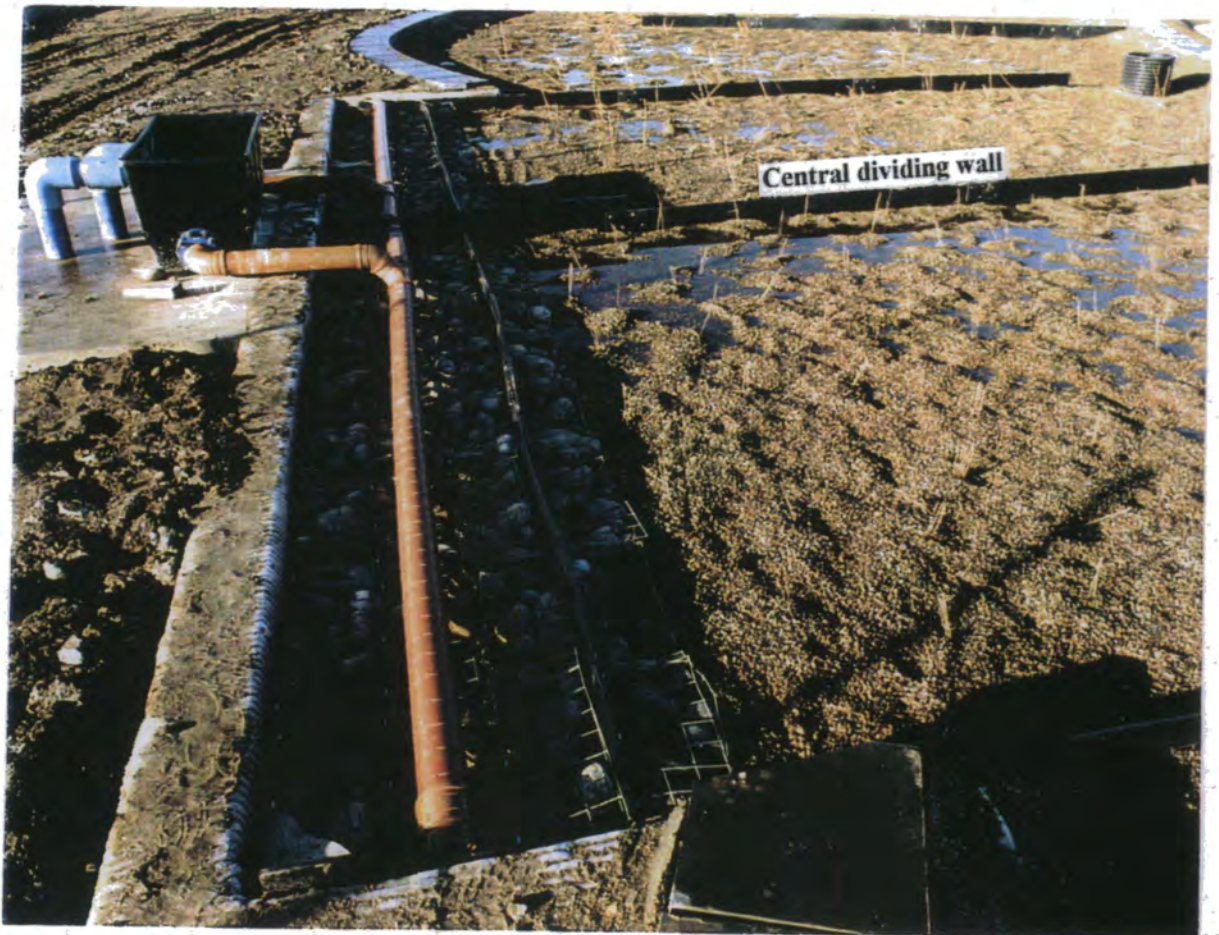
Plate 4. Wastewater inlet sections of the CATS Terminal reedbed, January 1997. (One month after planting, pot-grown Phragmites australis can be seen in the foreground, local transplanted Phragmites australis in the background).
