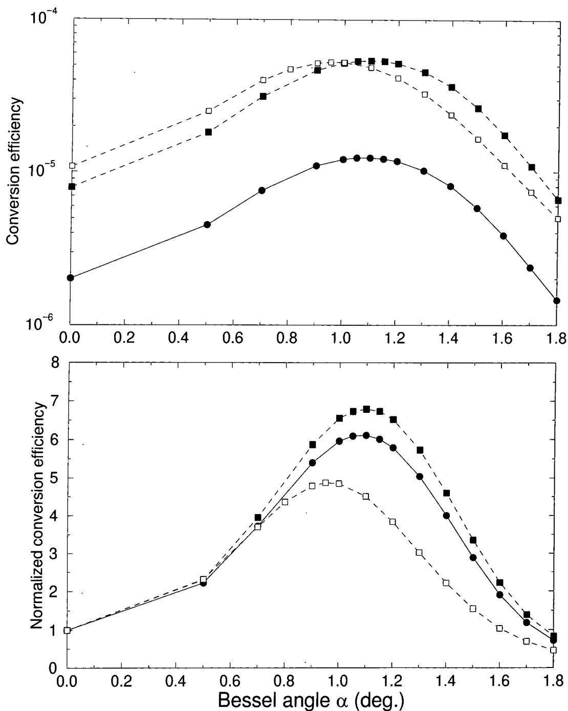
Figure 6.4: Same as Fig. 6.2 but for b = 2 mm. Top: Absolute conversion efficiencies for atomic hydrogen (circles and solid lines) and xenon (squares and dashed lines) versus the Bessel angle \alpha for the following focusing parameters: (L, b) = (0.5, 2) mm. Filled symbols are for a rectangular gas profile, open symbols for a truncated Lorentzian gas profile. Bottom: Normalized conversion efficiencies R(\alpha) with respect to the value in the Gaussian limit ( \alpha = 0^\circ ). The total energies on target are obtained from those given in Fig. 6.2 after multiplying by 2/5=0.4 .
