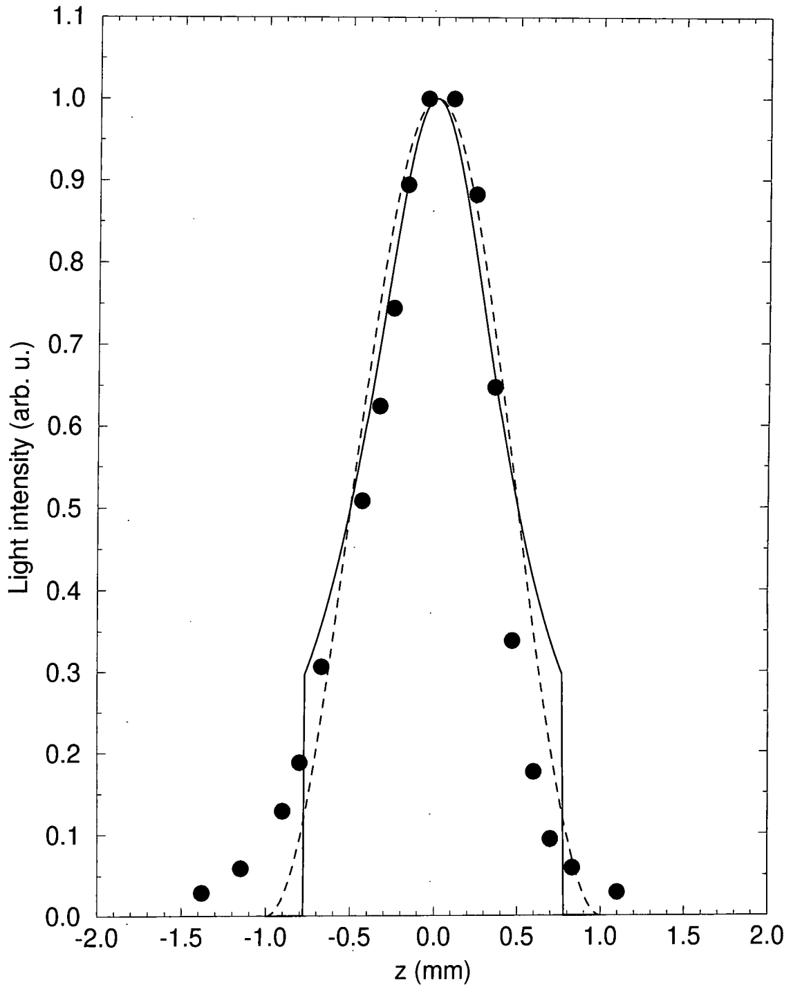
Figure B.1: Comparison between the truncated Lorentz profile (solid line) and the cosine-square profile (dashed line) for fitting experimental data points of a typical gas jet profile (filled circles). The experimental data points have been taken from Li [125] and show the intensity of laser induced fluorescence light (in arb.u.) versus the position (in mm) of the detector. The gas density is taken proportional to the detector signal. The FWHM of this gas jet profile is approximately 1 mm and this value of L has been taken for the fitting profiles.
