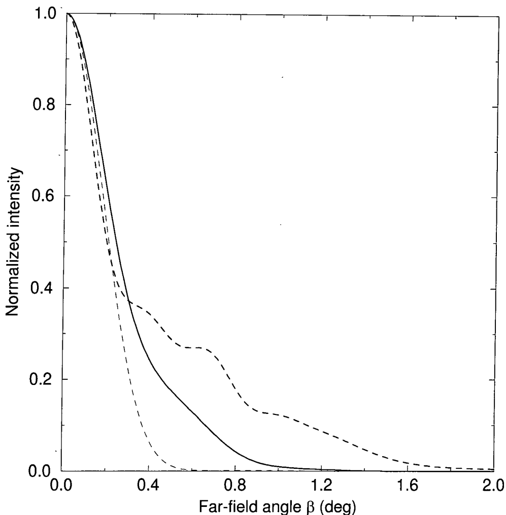
Figure 5.7: Far-field profile for a Gaussian beam ( \alpha = 0^\circ , b_G = 2 \text{ mm} ) as a function of the far-field angle \beta for various peak focal intensities I_f , obtained within the time-dependent approach. Thick dashed line: full calculation for I_f = 3 \times 10^{13} \text{ W/cm}^2 , thick solid line: same but for I_f = 1 \times 10^{13} \text{ W/cm}^2 , thin dashed line: same as thick dashed line but with photoionization neglected.
