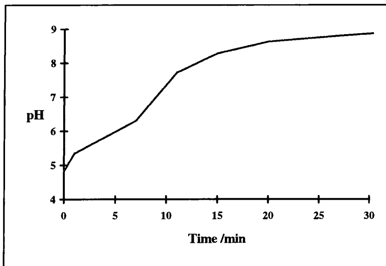
Figure 6.5 pH of \text{Cu}^{2+} Reaction with Neutramag and Ultrasonic Bath
