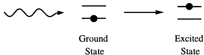
Figure 2.2 Atomic Excitation
