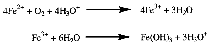
Scheme 3.1 Oxidation of \text{Fe}^{2+}
