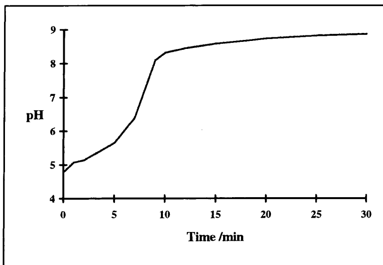
Figure 6.4 pH of \text{Cu}^{2+} Reaction with Neutramag and Pulsed Ultrasonic Probe
