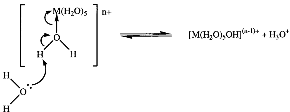
Figure 2.1 Deprotonation of Hexa-Aqua M(II) Species
