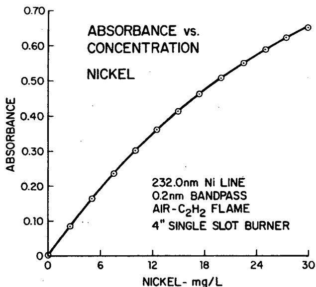
Figure 2.6 Example of Deterioration of Absorbance with Increasing Concentration
