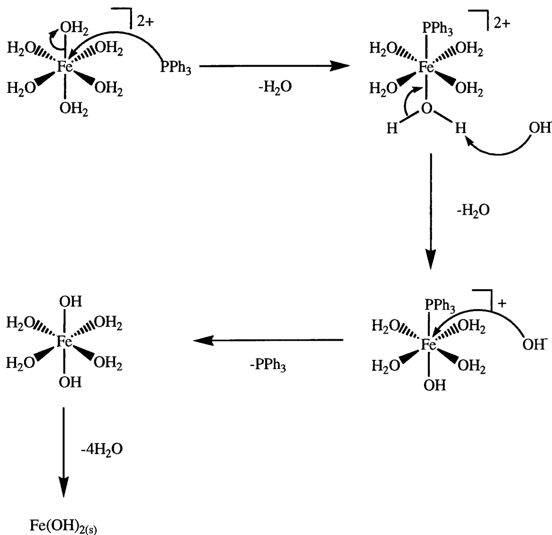
Scheme 1.2 Catalytic Reaction of \text{Fe}^{2+} with \text{PPh}_3
