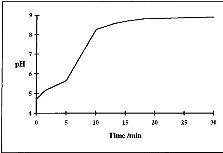
Figure 6.3 pH of \text{Cu}^{2+} Reaction with Neutramag and Ultrasonic Probe
