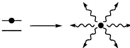
Figure 2.3 Energy Emission from Excited Atoms
