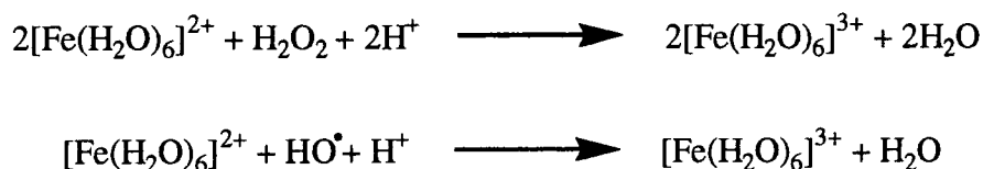
Scheme 6.1
