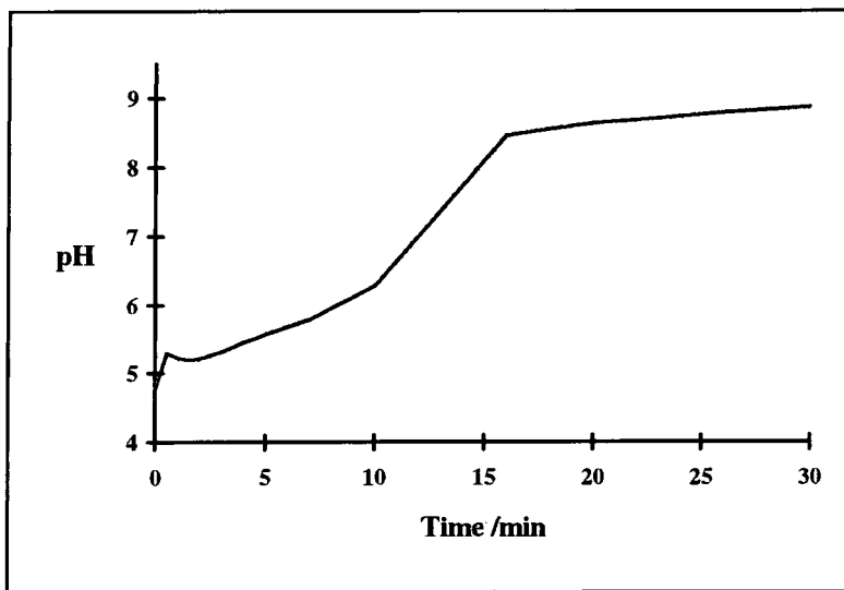
Figure 6.2 pH of \text{Cu}^{2+} Reaction with Neutramag and No Ultrasound
