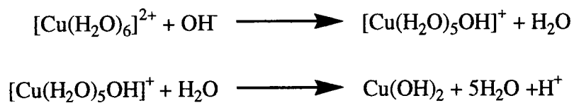
Figure 3.6 Proton Abstraction and Precipitation of Cu 2+ with Low Concentration of OH -
