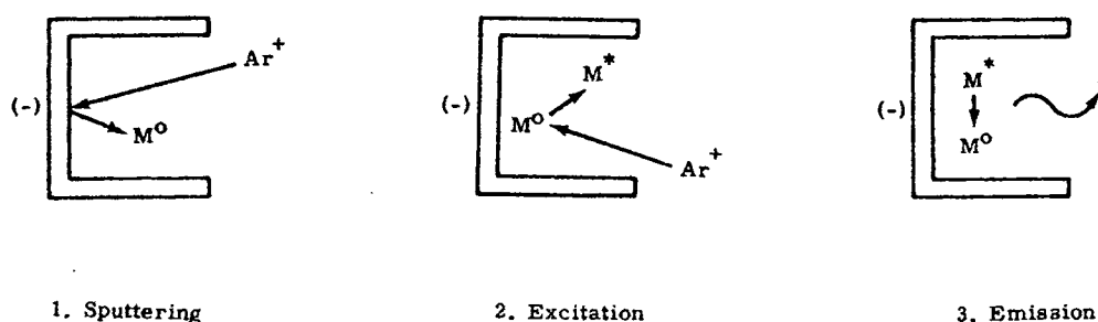
Figure 2.4 Lamp Emission of Desired Wavelength
