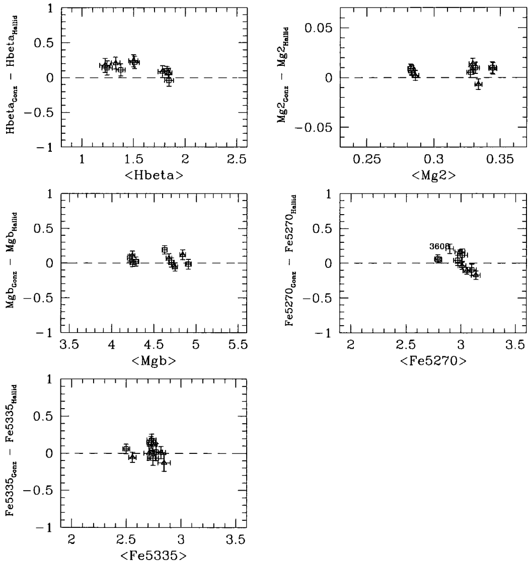
Figure 5.8: Differences between the central measurements of H \beta , Mg 2 , Mgb, Fe5270 and Fe5335 obtained here for major and minor axis axes of each galaxy, and 2'' \times 5'' measurements of González (1993), are plotted against the mean of both central measurements. Errors are given for all quantities based on final errors for all measurements. Open square symbols correspond to major axis measurements and open triangle symbols to minor axis measurements. For outlier points, labels are given indicating the galaxy NGC number, for major axis measurements to the upper left of the point position marked by the centre of error-bars, and for minor axis measurements to the lower right of the point position.
