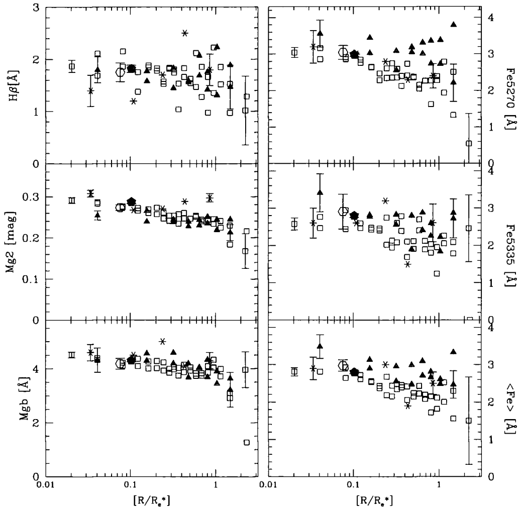
Figure 5.4: Comparison of NGC 4478 major axis measurements of H\beta , Mg_b , Mg_2 , Fe5270 , Fe5335 and \langle Fe \rangle given by open square symbols with those of Gorgas et al. (1990), given by filled triangle symbols and Peletier (1989) given by asterisk symbols. Central measurements of González (1993) and Trager et al. (1998) are given at representative radii, by closed pentagon and open hexagon respectively. Radii are given as \log(R/R_e^*) where R_e^* = R_e / \sqrt{1-\epsilon} and values of R_e and \epsilon are those given in table 5.2. For line-strength gradient measurements, error bars are given for the central and outermost measurements.
