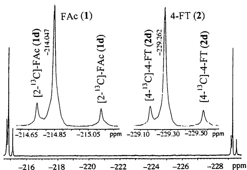
Fig. 2.8: ^{19}\text{F}\{^1\text{H}\} NMR of FAc ( 1 & 1d ) and 4-FT ( 2 & 2d ) labelled via [3\text{-}^{13}\text{C}] -pyruvate ( 100 ) metabolism.
