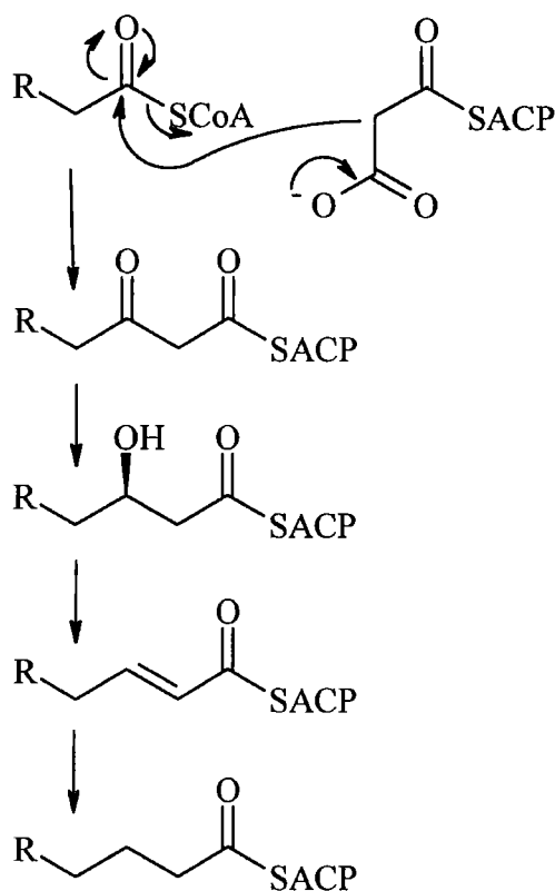
Fig. 1.3: Fatty acid biosynthesis and \beta -oxidation.
