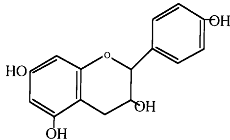
Figure 1.3. Structure of Flavon-3-ol (Catechins).
