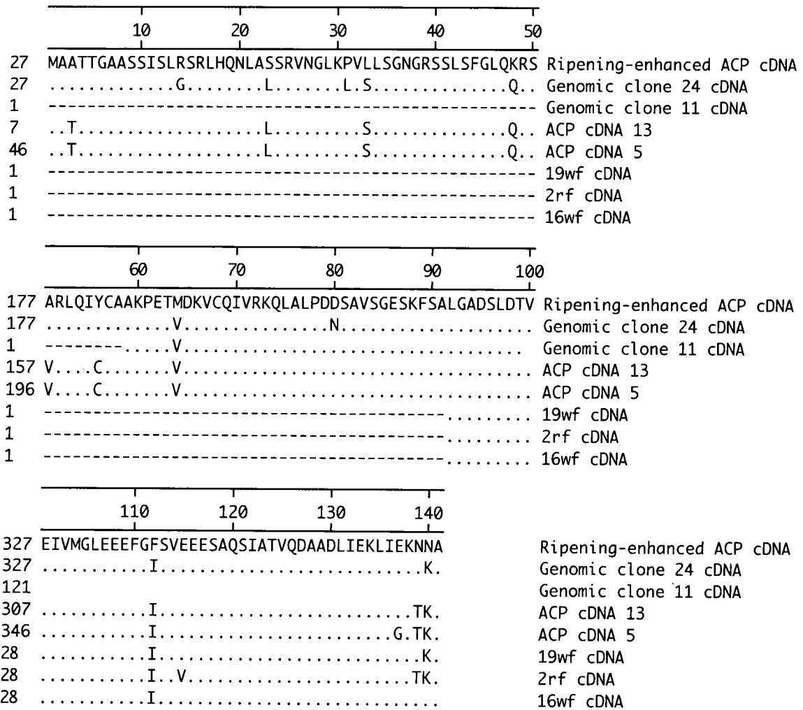
Figure 6.7. Comparison of the predicted amino acid sequences from the ORFs of the ACP clones isolated from strawberry fruit. Dots (.) and hyphens (-) represent homologous or missing bases. Only substituted bases are shown
