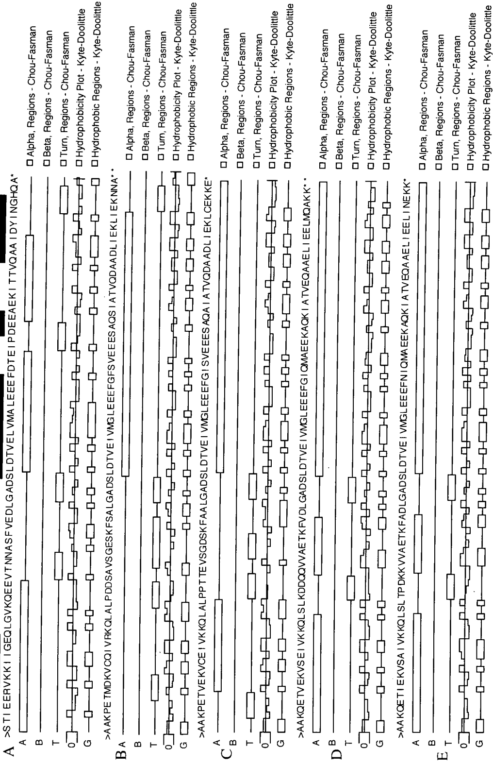
Figure 3.13. Predicted secondary structure of ACPs from E. coli (A), strawberry (RE-ACP; B), coriander (ACP-I; C), B. napus ACP (28f10; D) and Arabidopsis (ACP-I; E). Three structures, alpha, beta and turn ( \beta bends) regions were determined by the Chou-fasman method (DNASTAR). Black bars indicate \alpha -helices of E. coli ACP determined by NMR. Hydrophobicity was measured using the Kyte and Doolittle method.
