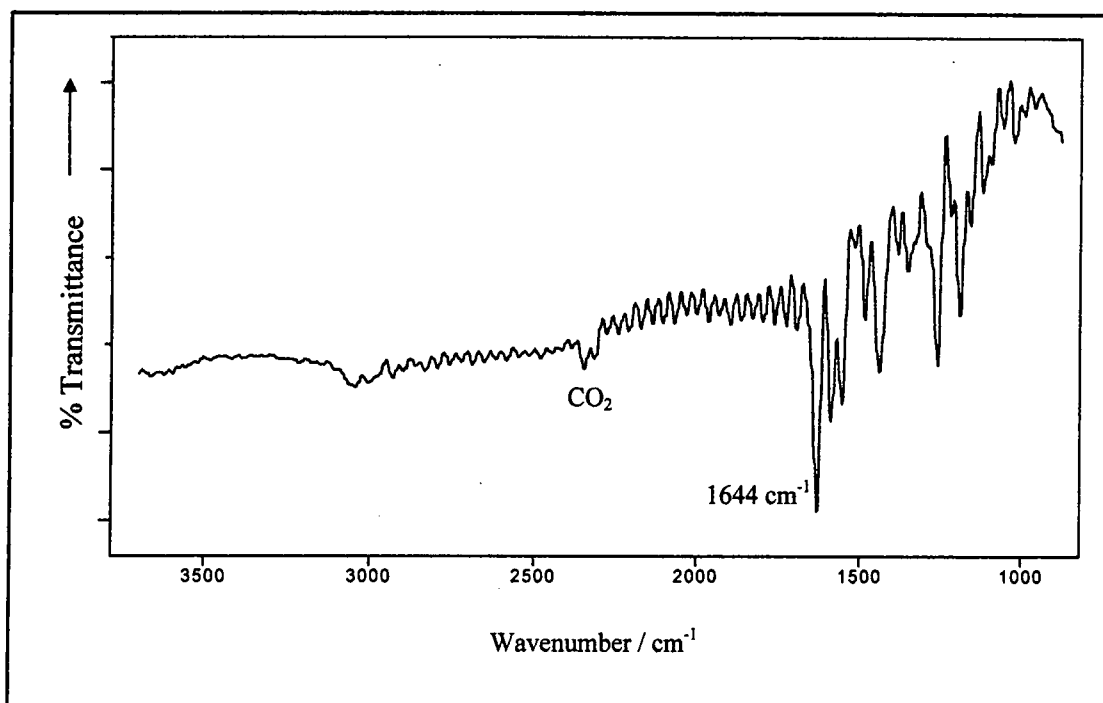
Figure 4.64 Infra-red spectrum of O-methyl DBM in CCl 4 at 77 K, with solvent spectrum subtracted
