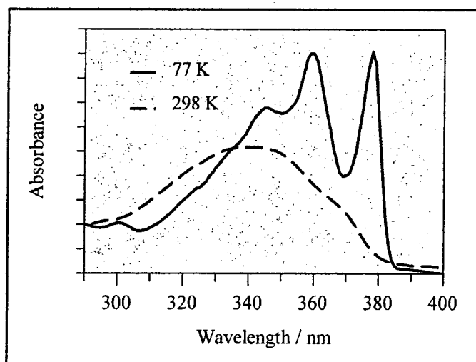
Figure 3.11 Absorption spectrum of dibenzoylmethane in EPA at room temperature and 77 K (data taken from this work - see section 3.2.2)
