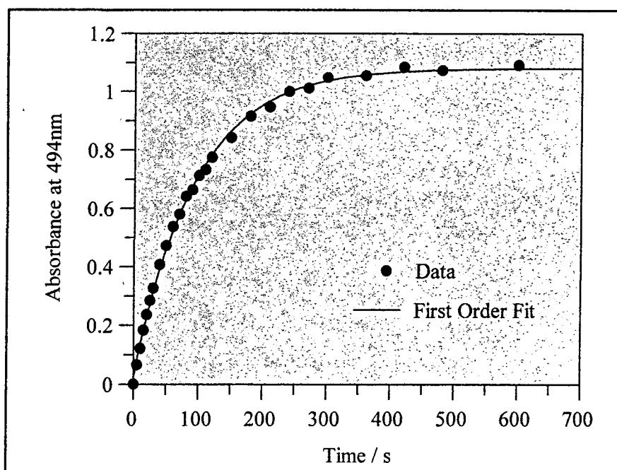
Figure 4.36 Formation of the ring closed form of Aberchrome 540 in toluene with time during irradiation at 342 nm
