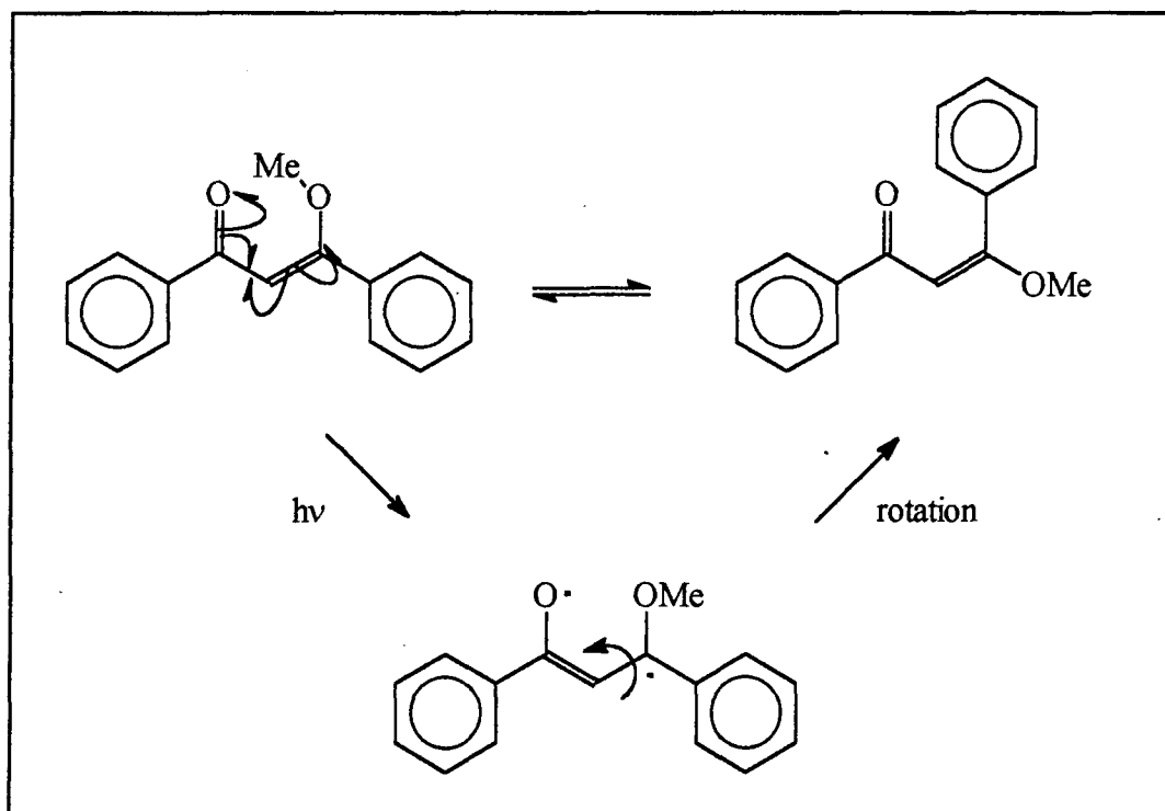
Figure 4.29 Photochemical, radical Z \rightarrow E isomerisation of O-methyl DBM 36
