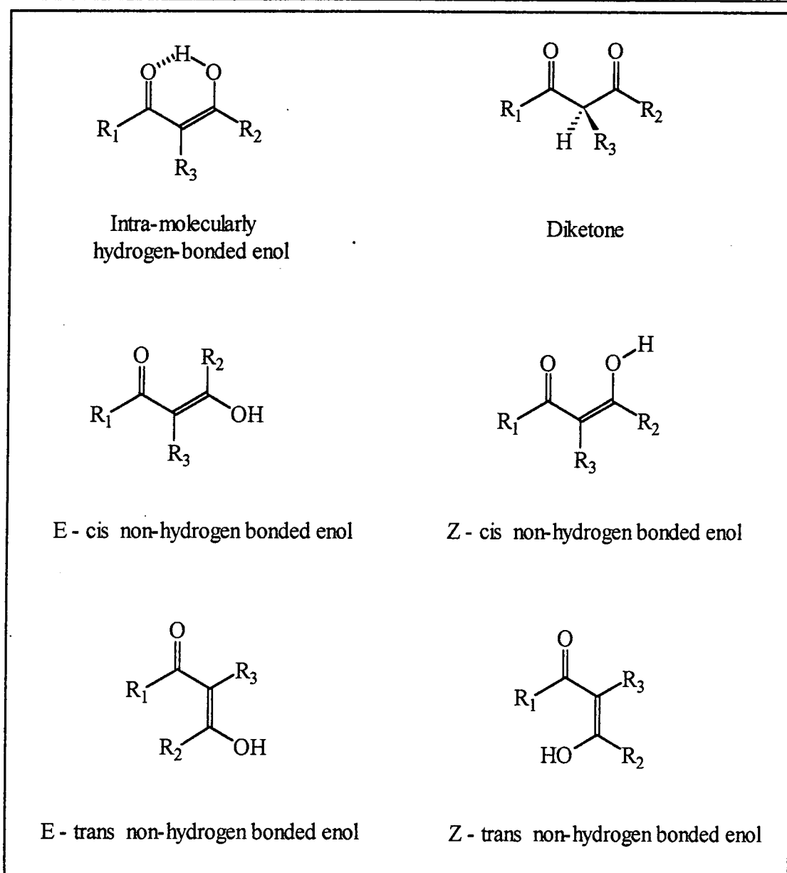
Figure 3.8 Possible isomers of 1,3-dicarbonyl compounds
