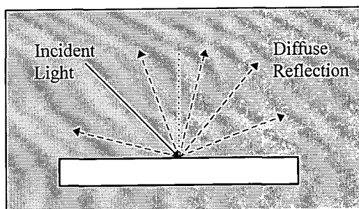
Figure 2.24 Diffuse reflection
