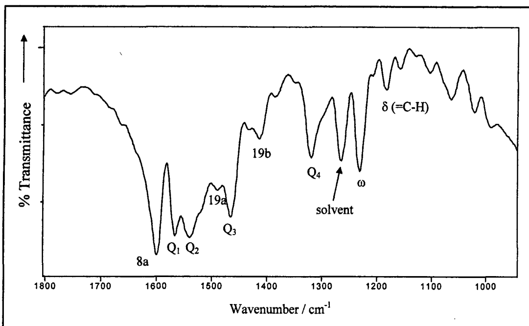
Figure 4.63 Infra-red spectrum of DBM in \text{CH}_2\text{Cl}_2 at 77 K, with solvent spectrum subtracted (assignment of peaks based on table 4.8, from reference 40; some peaks may be distorted due to solvent)
