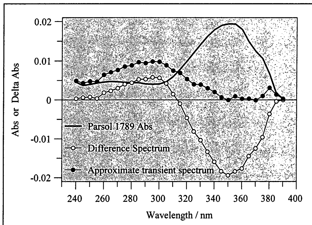
Figure 4.43 Approximate transient absorption spectrum for Parsol 1789 in cyclohexane, pumping at 340 nm (initial delta absorbance values plotted)
