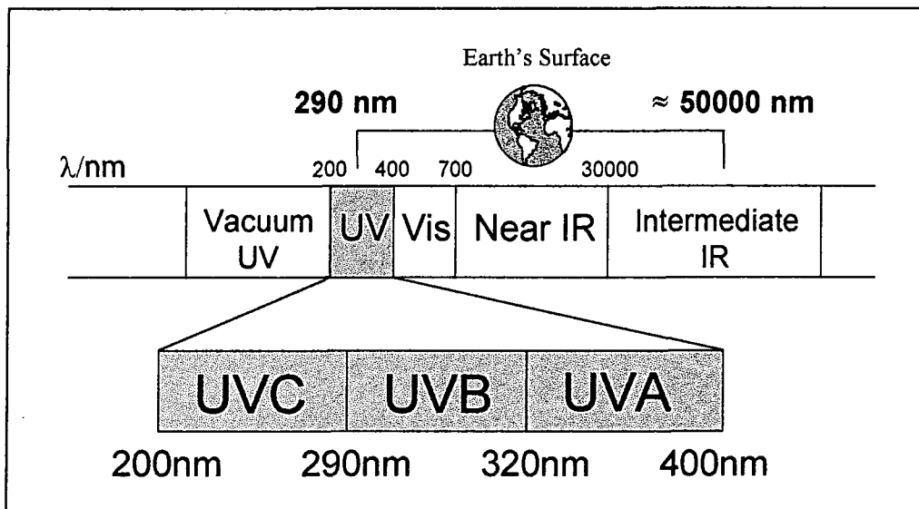
Figure 1.1 A portion of the electromagnetic spectrum
