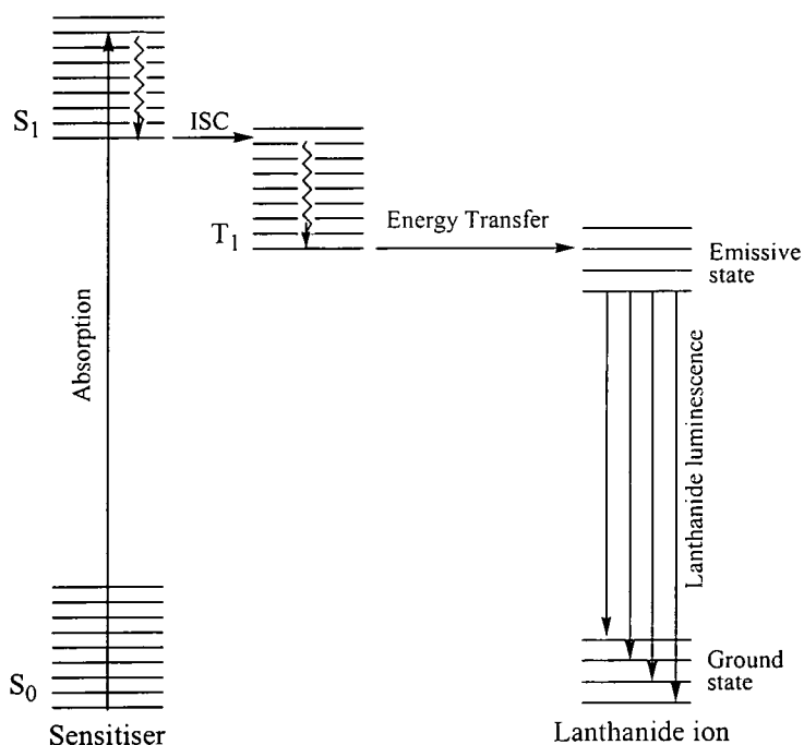
Figure 1.4 Sensitised emission
