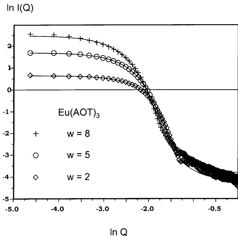
Figure 2.3 SANS data and model fits for \text{Eu}(\text{AOT})_3 reversed micelles using \text{H}_2\text{O}-h\text{-AOT}-\text{C}_6\text{D}_{12}
