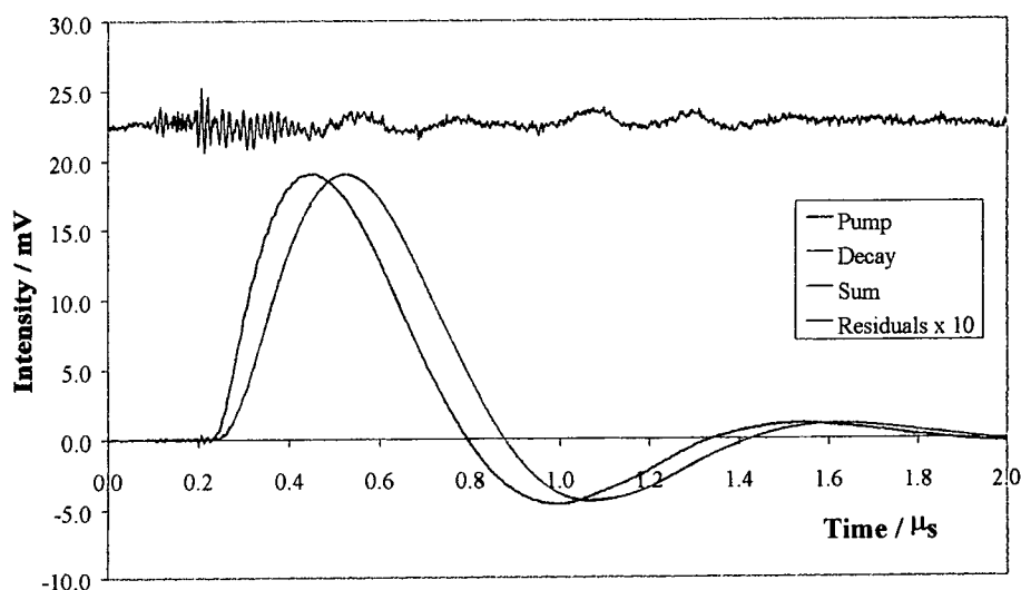
Figure 1.6 The IRF, decay, fit and residuals \times 10 for [\text{Nd}(\text{dota})]^{3-} in H 2 O. The data gives a lifetime of 75.7 ns.
