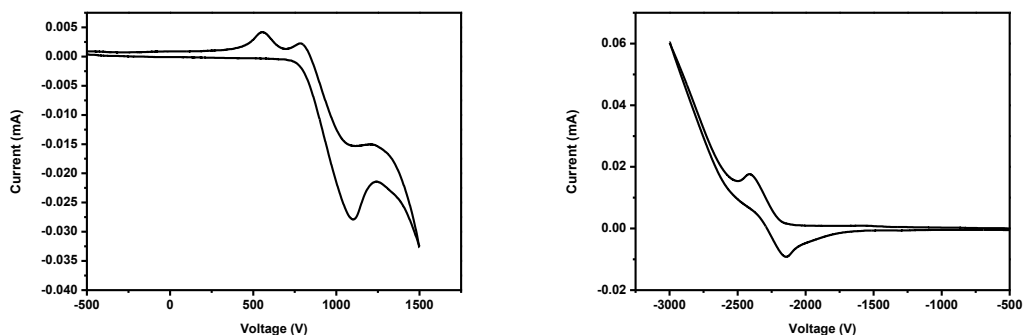
Figure 2.8 – Cyclic voltammograms showing oxidation (left: in DCM) and reduction (right: in THF) waves for 157 vs ferrocenium/ferrocene couple ( \text{FcH}^+/\text{FcH} = 0.0 \text{ V} ).
