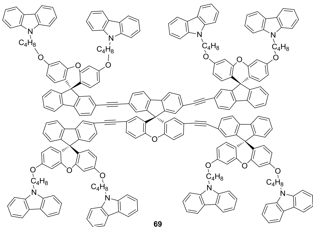
Figure 1.19 - Structure of a branched spiro(fluorene-9,9'-xanthene) derivative
