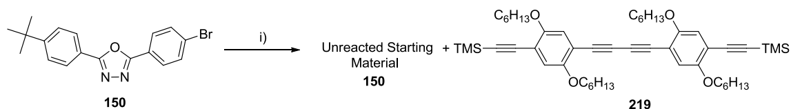
Scheme 4.5 – Attempted Sonogashira coupling of 150 and 212
