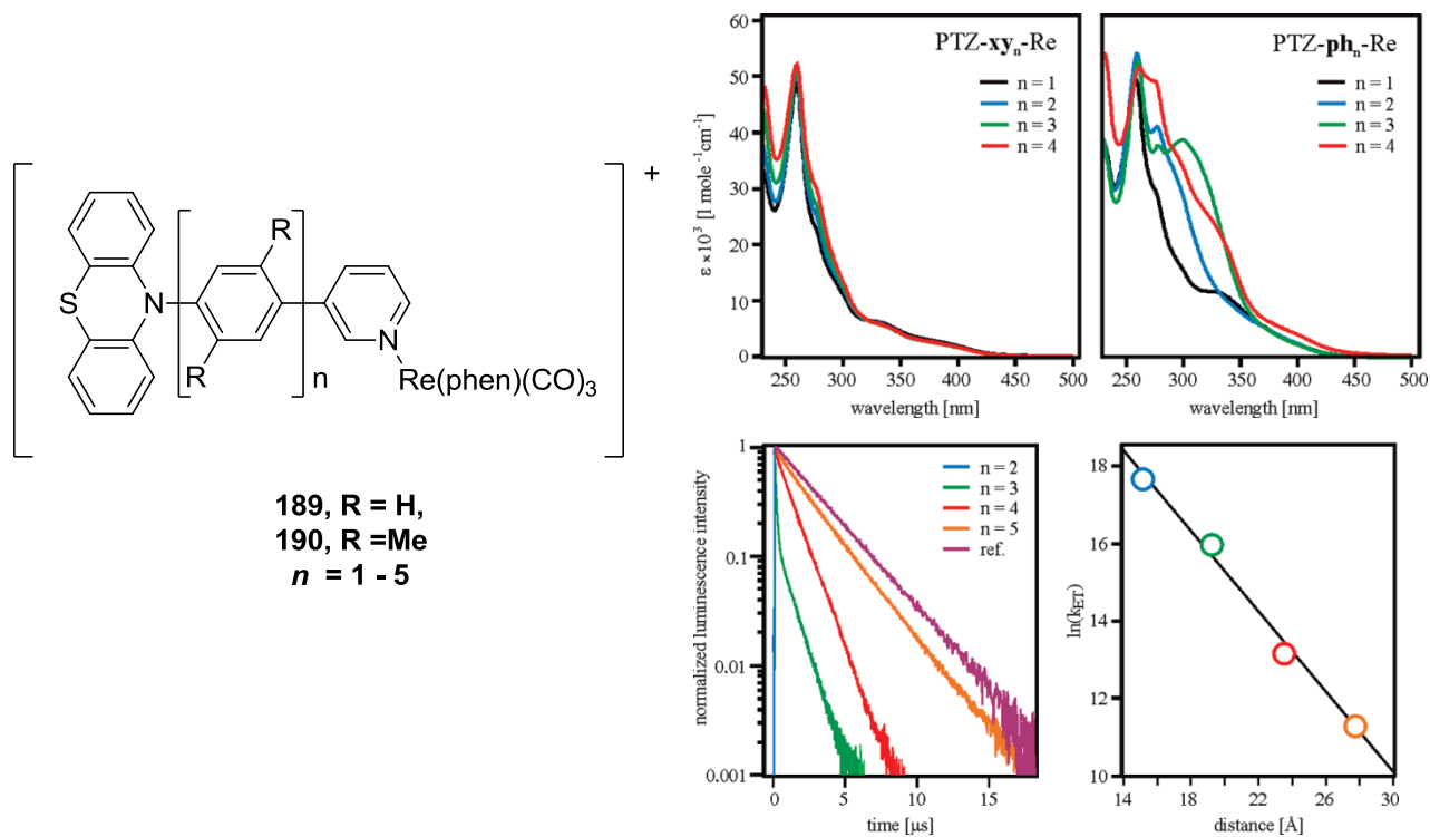
Figure 4.3 - (a) Structures of wire candidates 189 and 190 (PTZ = phenothiazine) (b) absorption spectra of wire candidates in dichloromethane solution (c) plot of fluorescence decay and distance dependence on rate of ET for p-xylylene molecular wires with plot for reference complex [\text{Re}(\text{phen})(\text{CO})_3(\text{pyridine})]^+
