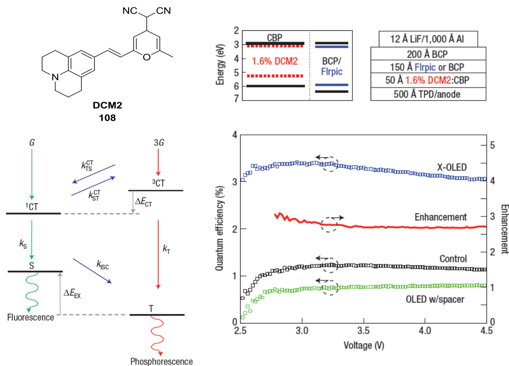
Figure 2.1- Proposed energy pathways for emission in displayed device structure and voltage vs. efficiency plot for the various OLEDs in the study 70
