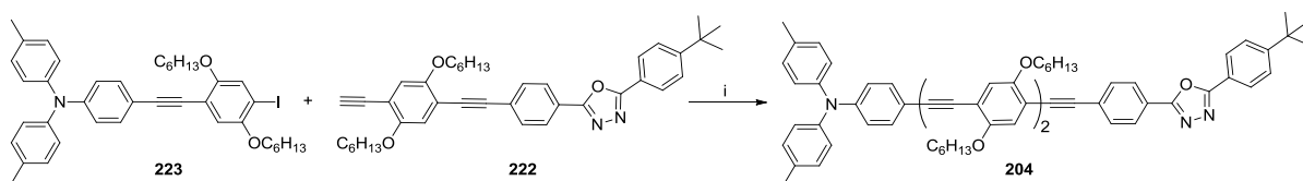
Scheme 4.9 – Synthesis of 204
