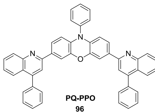
Figure 1.33 - A representative structure of a phenoxazine – acceptor system 96
