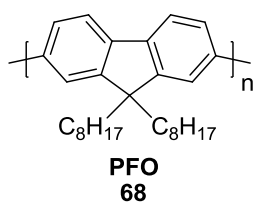
Figure 1.18 - Structure of PFO
