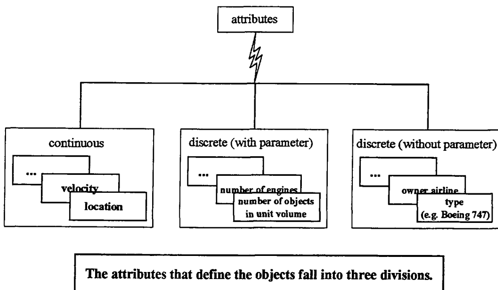
Figure 5.1: Attributes
