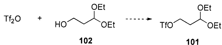
Figure 21 Proposed preparation of 101
