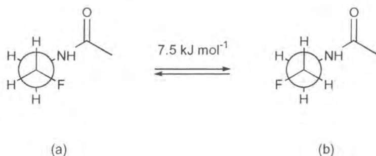
Figure 51 Calculated energy difference between gauche (a) and anti conformations (b) for N -(2-fluoroethyl)acetamide 156 .
