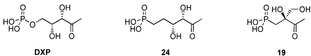
Figure 9 Structural analogies between DXP, 24 and 19 .
