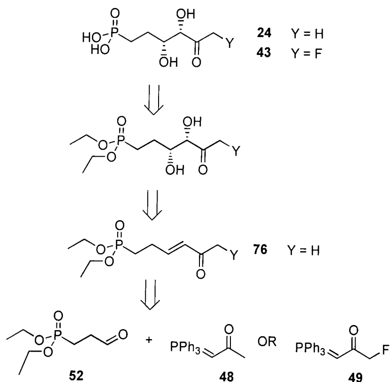
Figure 19 Retrosynthetic analysis to 24 and 43 .
