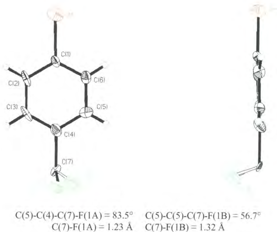
Figure 39 50 % Probability ellipsoid plot of 4-bromobenzyl fluoride 149 .
