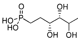
Threo -5( R,S )-3,4,5-trihydroxyhexylphosphonic acid 46
