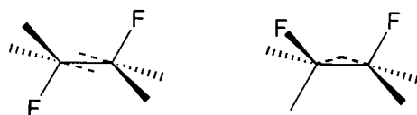
Figure 44 Comparison of the sp^3 orbital overlap (dashed lines) for the anti and gauche conformers of 1,2-difluoroethane 153 .
