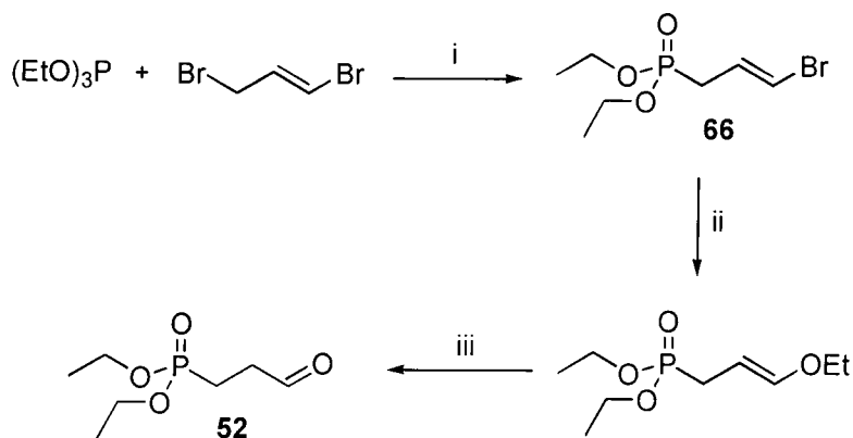
Scheme 18 i. 120-140 °C, 90 %; ii. NaOEt / EtOH, 1 h, reflux, 66 %; iii. HCl (aq) (no yield given). 88
