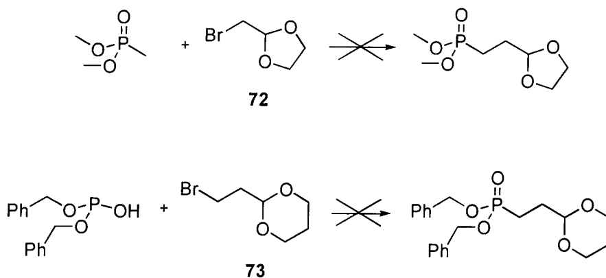
Scheme 21 Proposed routes to protected phosphono acetals.
