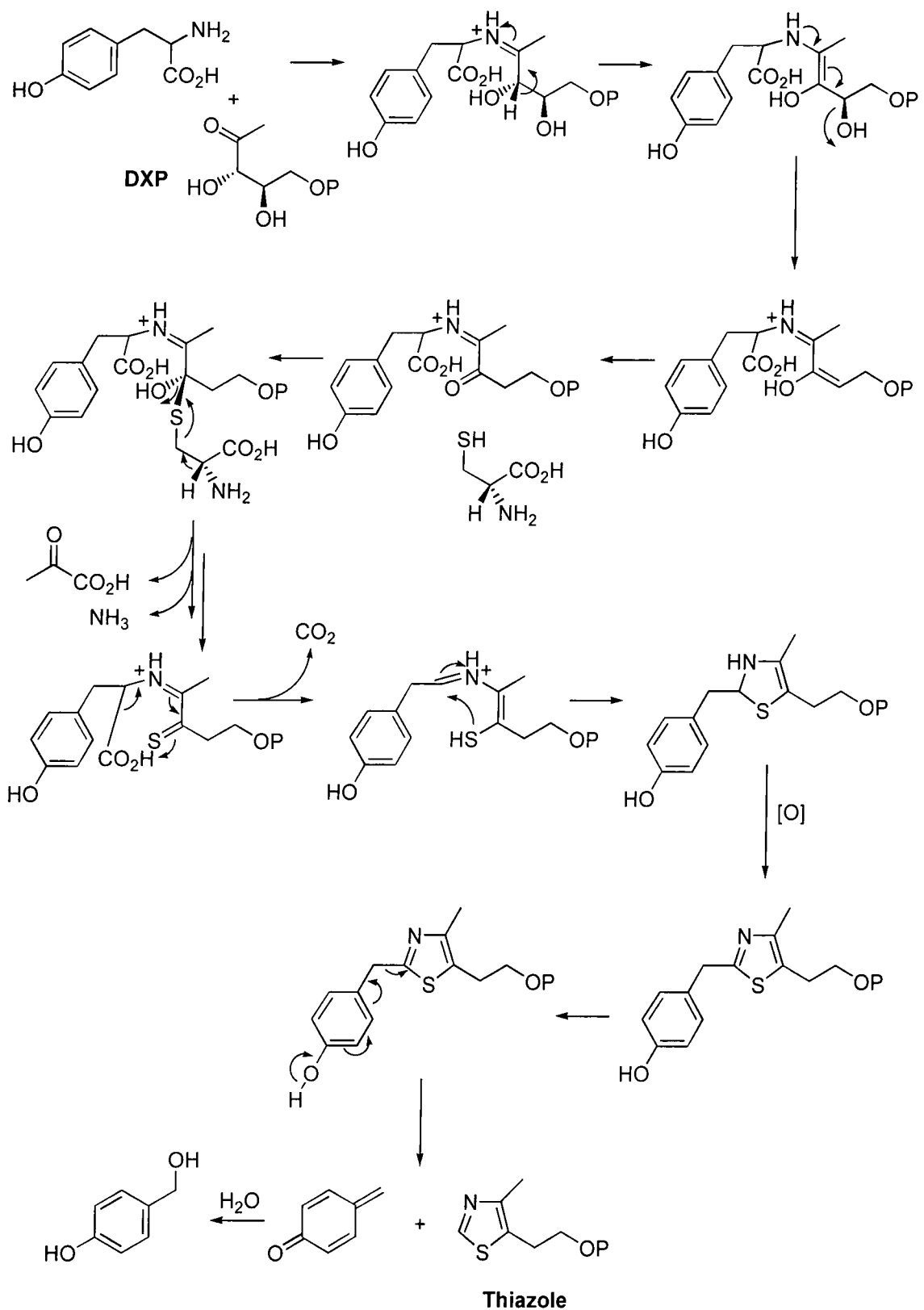
Scheme 5 Putative mechanism for the biosynthesis of the thiazole unit in enteric bacteria from tyrosine and DXP. 24
