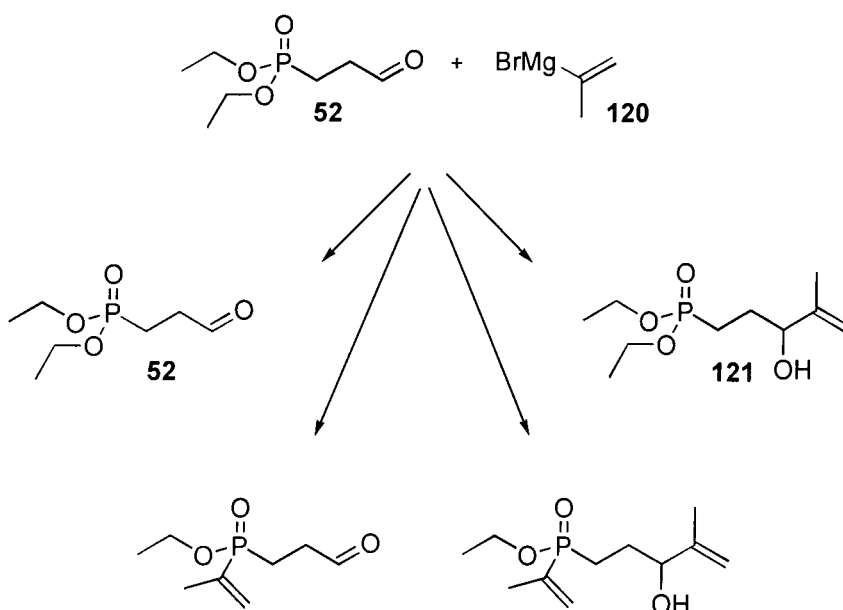
Scheme 54 Reaction products of diethyl 3-oxopropylphosphonate 52 with isopropenylmagnesium bromide 120 at 0 °C.
