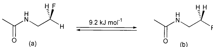
Figure 52 Calculated energy difference for the gauche (a) and anti conformations (b) of N -(2-fluoroethyl)acetamide 156 with the CCNH, CNCO and CCNC dihedral angles constrained at 0, 0 and 180^\circ respectively.
