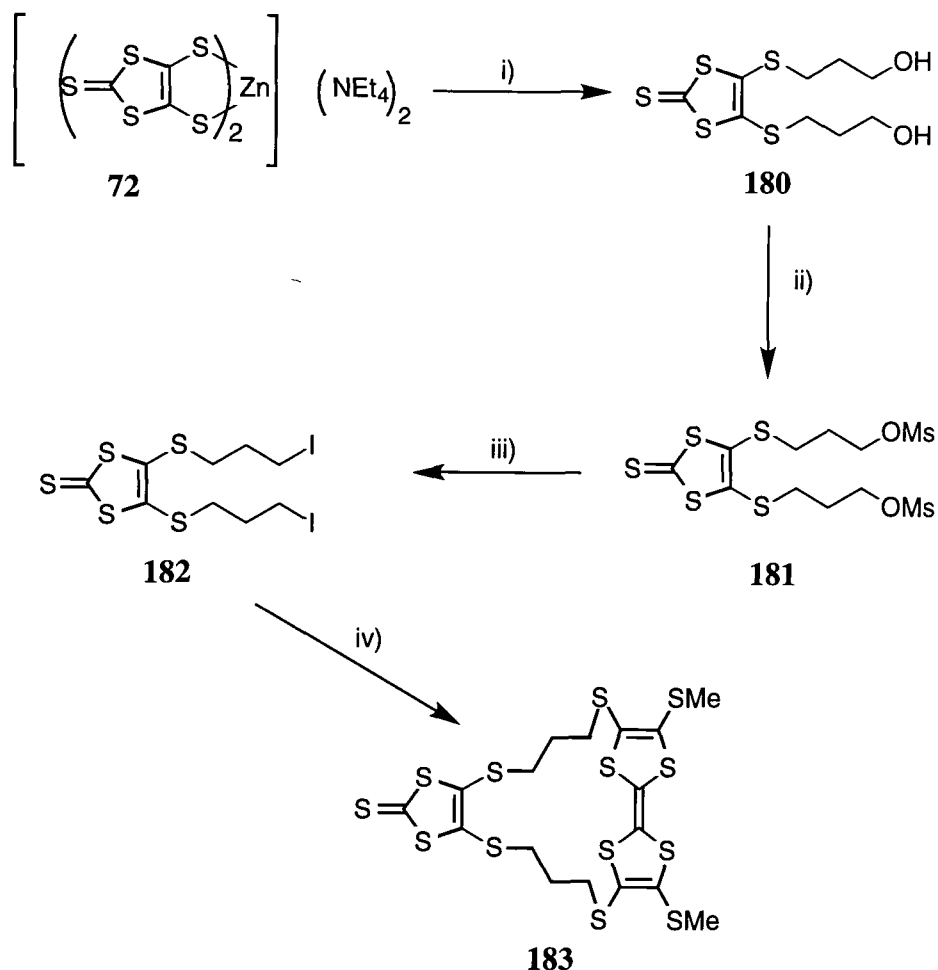
Scheme 3.12 Reagents and Conditions: i) MeCN, 3-bromopropanol; ii) MsCl, pyridine, DCM; iii) NaI, acetone, reflux; iv) 153 , CsOH, DMF, high dilution.
