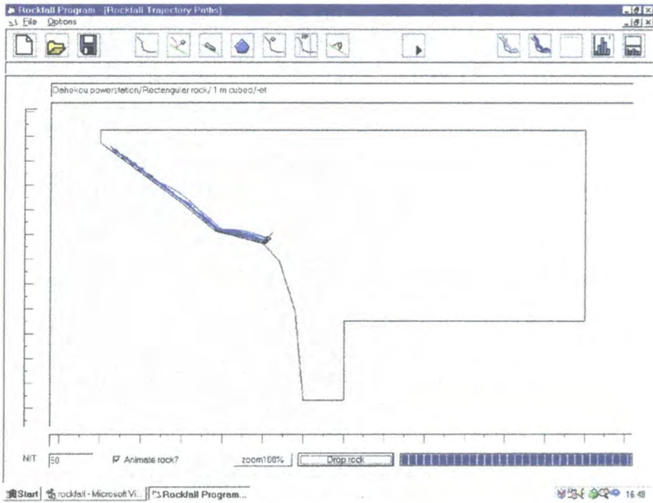
Figure 6.25: Trajectories of the 1m 3 rectangular rocks with a 1000 kJ capacity rock fall net.
