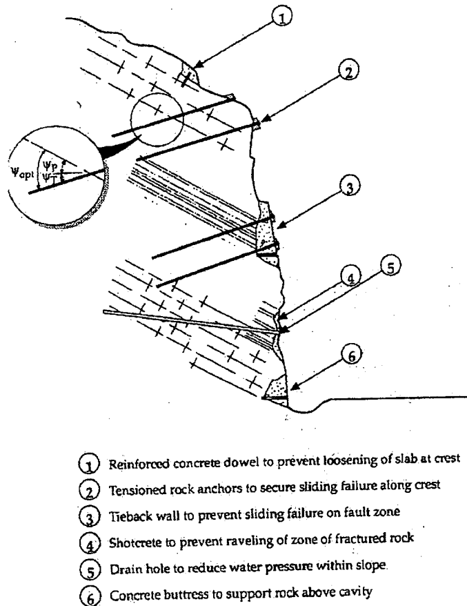
Figure 2.3: Rock reinforcement (Wyllie and Norrish, 1996).
