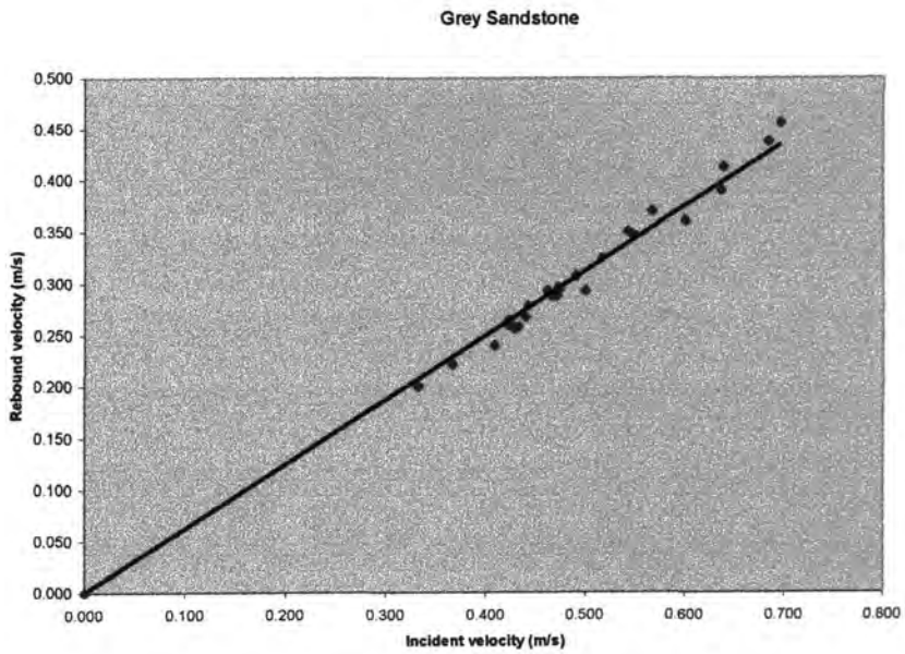
Figure A4.4: Incident v rebound velocity for a grey sandstone disc.
