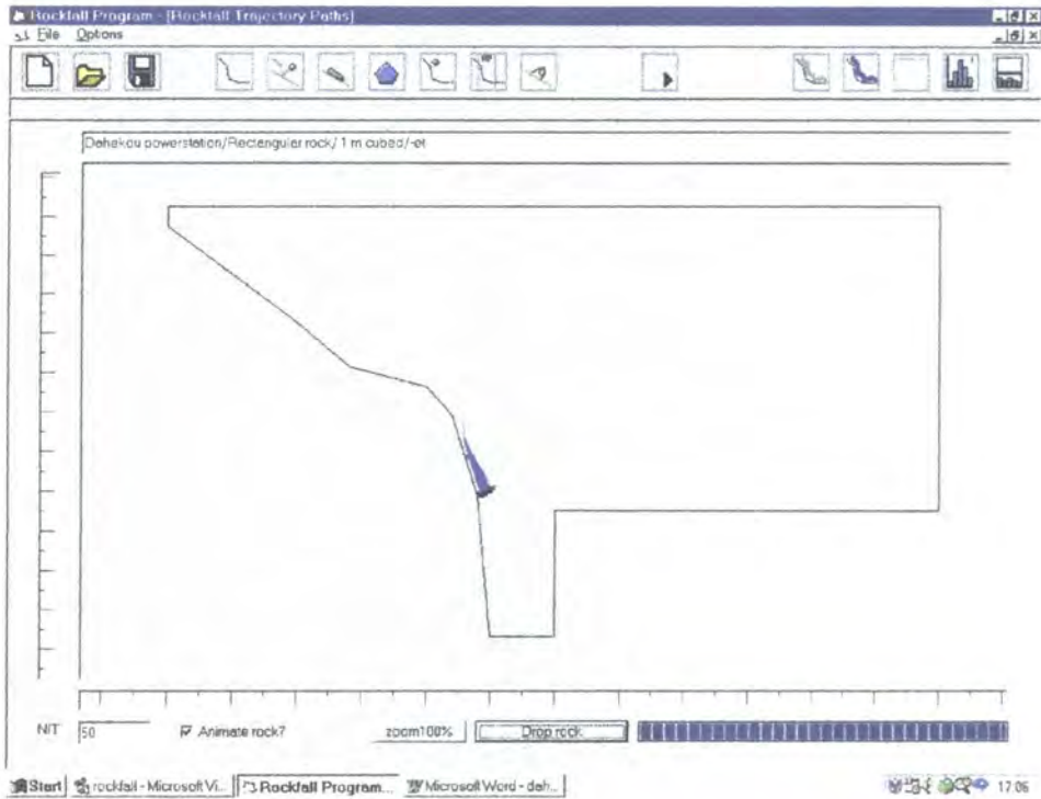
Figure 6.27: Trajectories for a 1m 3 rectangular rock originating from the middle slope region with a 500kJ capacity rock fall net.
