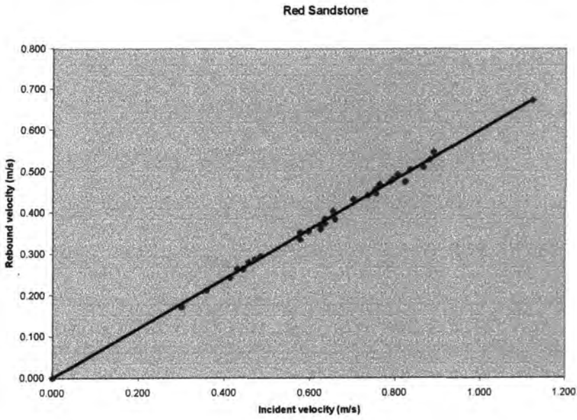
Figure A4.3: Incident v rebound velocity for a red sandstone disc.
