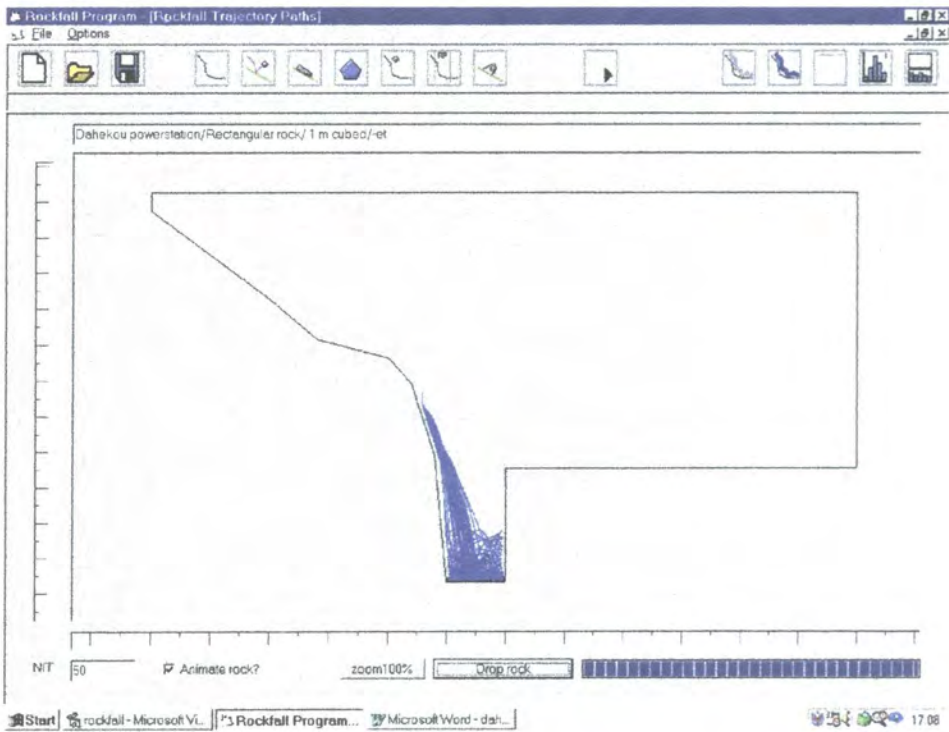
Figure 6.26: Trajectories for a 1m 3 rectangular rock originating from the middle slope region with no rock fall net.
