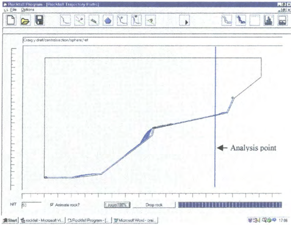
Figure 6.35: Rock trajectories for the central section.
