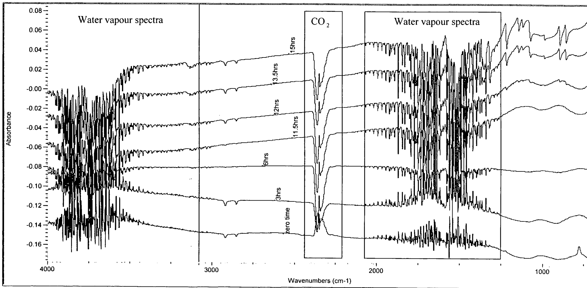
Fig.4.15. External reflection FTIR spectra from 4000-650 \text{cm}^{-1} for stearic acid spread on a 120% supersaturated solution of dl-aspartic acid at a compression surface pressure of 12 mN/m.
