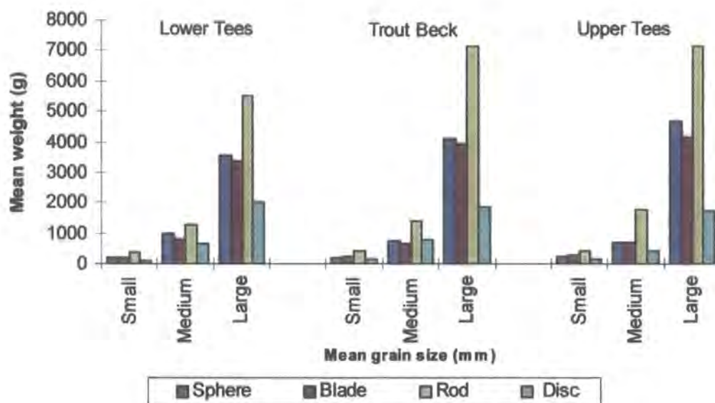
Figure A1.3. Mean weight distribution of clasts in three size groups for four shape classes at the Lower Tees, Trout Beck and the Upper Tees sites.
