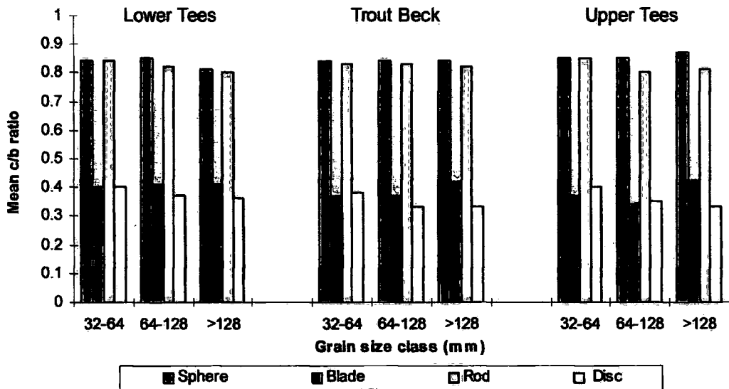
Figure A1.7 Mean distribution of c/b ratio of clasts in three size groups for four shape classes at the Lower Tees, Trout Beck and the Upper Tees sites.
