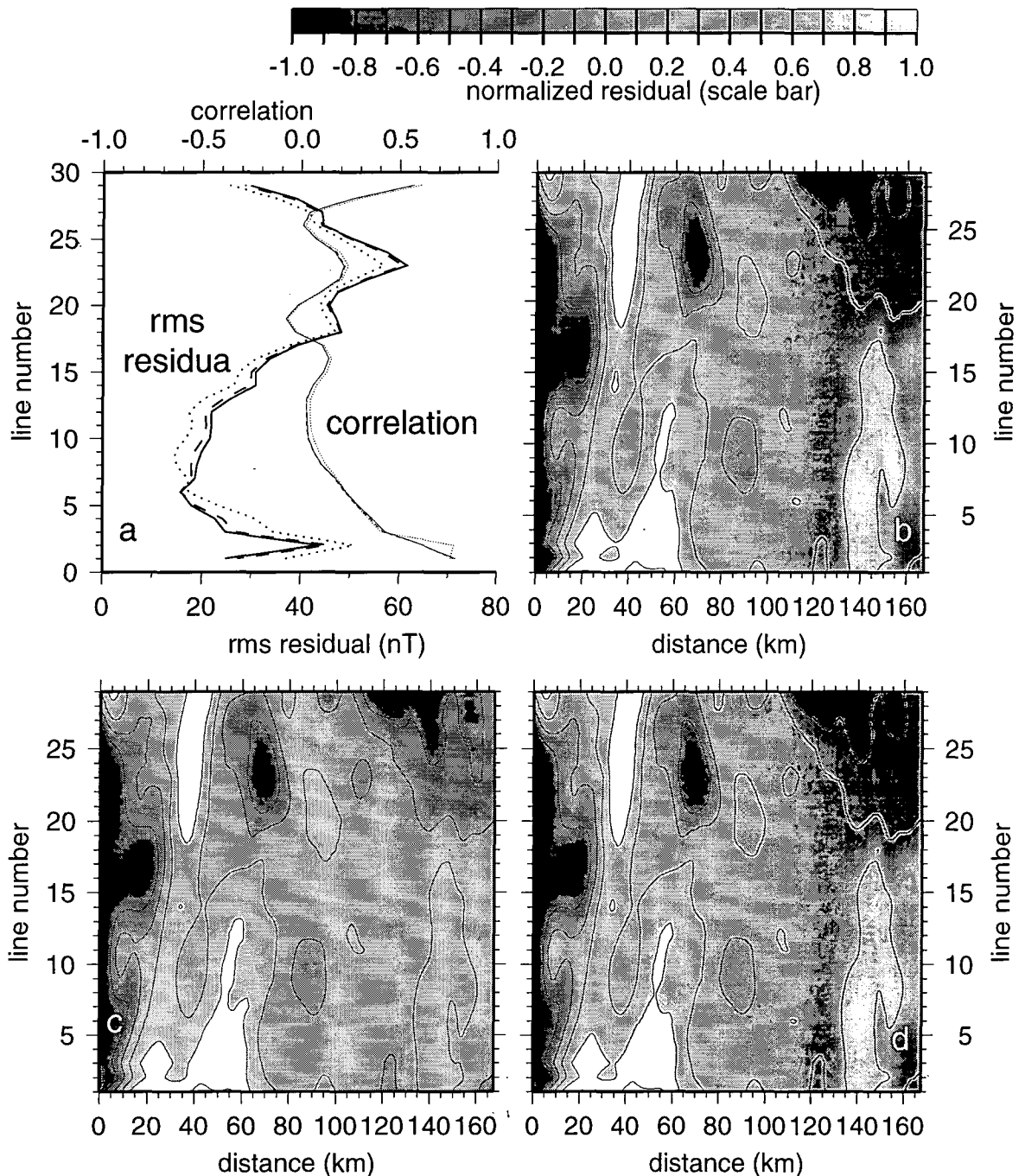
Figure 5.7 (a) Correlation coefficients (thin lines) and rms residua (thick lines) between the observed magnetic field and a forward calculated magnetic field along each of the lines 1-29 of figure 5.6. Each forward calculated field was computed from a model whose upper surface was extracted from the depth to basement chart (Fig. 5.2) along the coincident line. Each model was described by a lower surface at 14 km depth and a magnetization vector defined by Van der Voo (1990; I=46 , D=0 ; solid line), Galdeano et al. (1989; I=58 , D=-43 ; dashed line) and an induced magnetization vector ( I=57 , D=-9 ).
