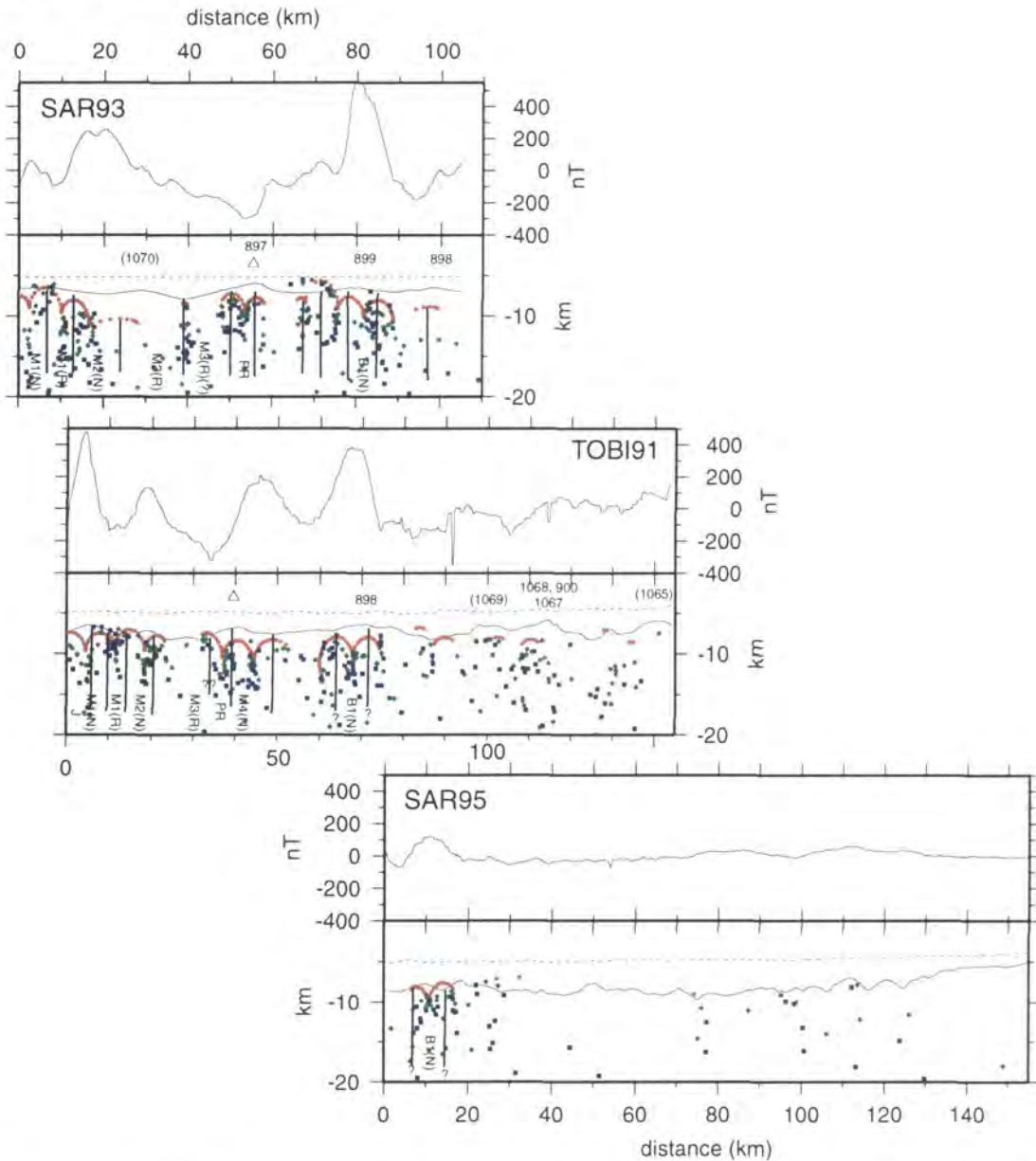
Figure 6.6 Euler deconvolution of magnetic anomalies (upper panels) along profiles SAR93, TOBI91 and SAR95 (aligned along common longitude). Window length = 2 km (see section 4.2). Solutions shown (lower panels) for structural indices of 0.0 (semi-infinite contact; red circles), 0.5 (step contact; green diamonds) and 1.0 (dyke-like contact; blue squares). ODP Sites, peridotite ridge, fish tracks and acoustic basement shown in lower panels (see Fig. 6.3 caption). Boundaries of magnetic blocks determined by positions of apices of solution clusters (SI=0.0); contacts of seafloor spreading blocks and other magnetic contacts (including B1(N)) labelled. See text for discussion.
