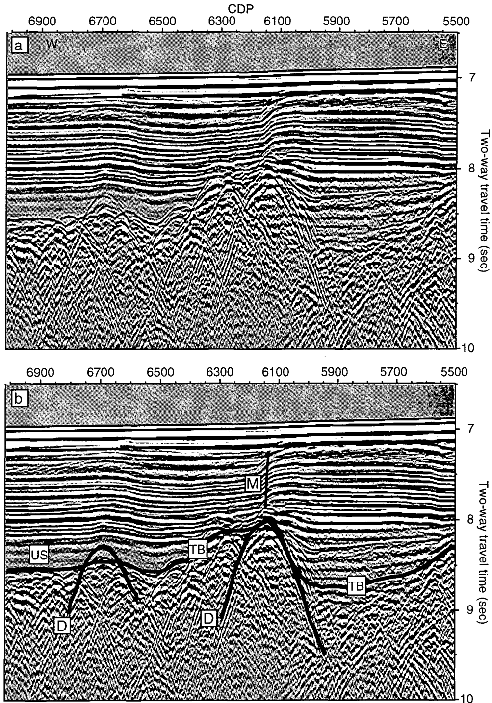
Figure 5.3 Multichannel seismic reflection profile CAM-142 between CDP 5500 and 7000. (a) uninterpreted section, (b) interpreted section. Top basemet event picked and interpreted and shown as heavy line (TB), which is commonly obscured by diffractions (D) making precise interpretation of travel time picks difficult. M indicates axis of monocline in post-rift sediments directly above the basemet high over which ODP Leg 149 drill site 898 lies 8 km along strike to the north. The basemet high is possibly the northern continuation of peridotite ridge segment R4. US denotes the lowermost package of sediments (directly above top basemet) which have little internal character and approximately the same velocity as the uppermost basemet (Dean et al., submitted; see Chapter 6) introducing further difficulty in defining TB, especially in basemet lows.
