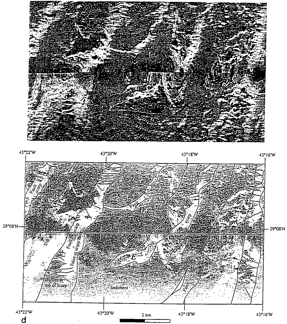
Fig 4. (d) Example of "hooked" fault terminations from western ridge flank (see text for discussion). Single swathe with vehicle track running E–W through centre. Five inward (east) facing normal faults are at top of image, with centre one ( D ) hooking west to join second from left. Insonification in northern half of image is to north, so face of this hooked fault is insonified along its whole length. Second fault from right hooks west in lower part of image, where insonification is to south, so face of hooked part is in shadow but dip slope is insonified ( E ).
