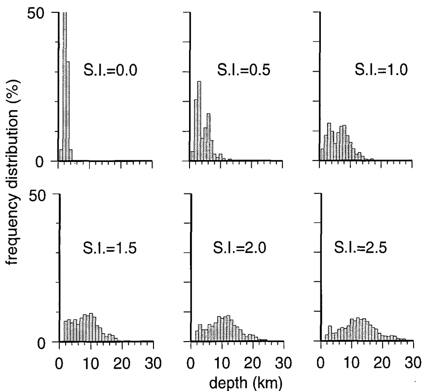
Figure 5.14 Distributions of Euler solutions for structural indices (S.I.) of 0.0-2.5 resulting from the deconvolution of the field over the ocean-continent transition in region S2 ( 40^{\circ} - 41^{\circ} N, 13^{\circ} - 11^{\circ} W).
