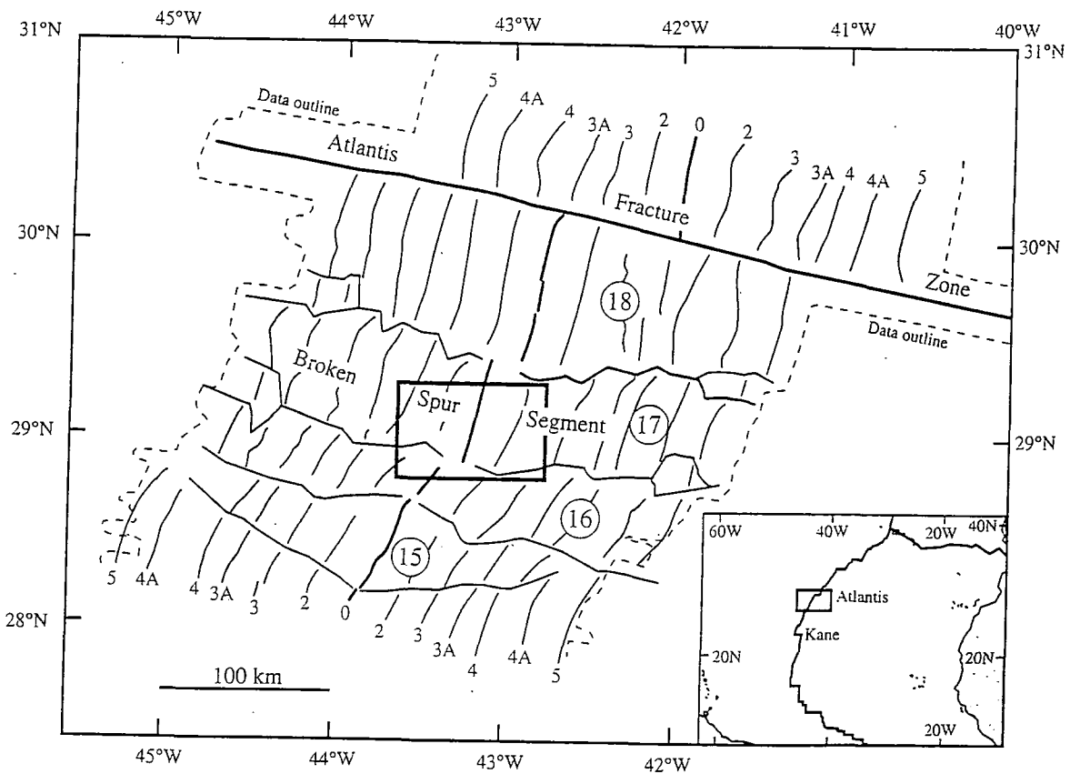
Fig. 1. Inset: location of study area between Atlantis and Kane transform faults on the Mid-Atlantic Ridge. Main figure: heavy box outlines area of present study. Heavy lines show current plate boundary and Atlantis fracture zone. Lighter lines give crustal isochrons (labelled by magnetic anomaly number) and bathymetric segment boundaries [10,11], with segment numbers [31] circled. Dashed line marks extent of regional gravity, magnetic and multibeam bathymetry coverage [10,11].
