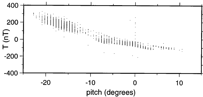
Fig. AI.3 Total field magnetic anomaly associated with pitching motion of SAR. For angles of \pm 5^\circ anomaly produced is as large as \sim 100 nT.
