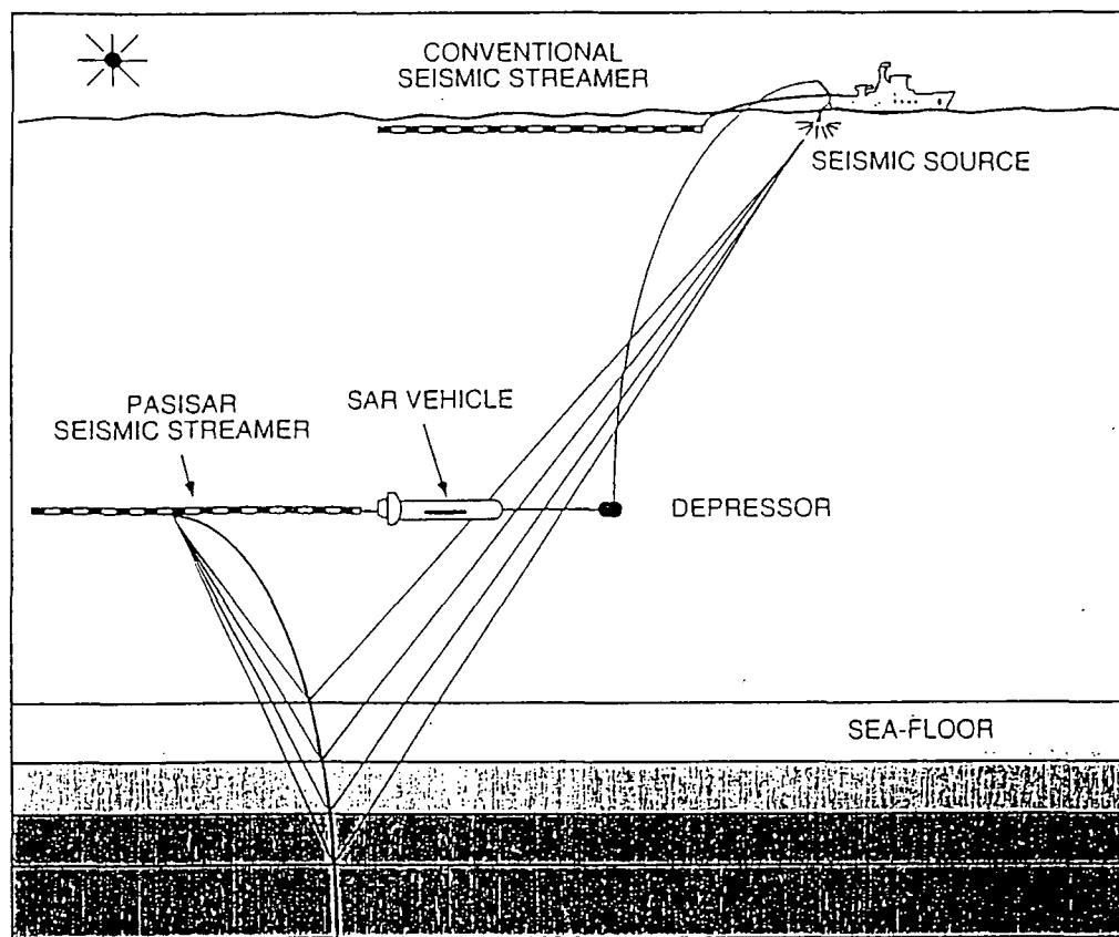
Figure 1.4 Geometry of a near-bottom geophysical experiment as exemplified by IFREMER's System Acoustique Remorque (SAR). Three orthogonal fluxgate magnetometers are mounted externally on the vehicle to minimize the effects of electrical noise generated by the SAR's circuitry. The vehicle is towed at near constant altitude above the seabed either by altering the length of tow cable out or by changing the ship speed. Noise derived from the motion of the ship is damped by the use of an umbilical between the depressor weight and the ship. The SAR is also capable of towing a seismic streamer (from Minshull, 1995).
