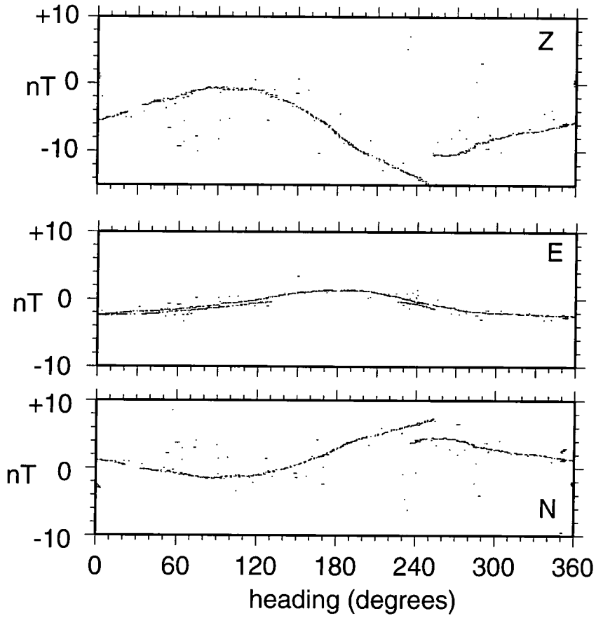
Fig. AI.2 Magnetic fields in down, east and north directions associated with the SAR vehicle as a function of heading. Offsets of up to 4 nT at \sim 270^\circ are likely to be a result of instrument drift.
