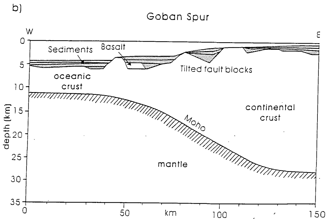
Figure 1.2 Cross sections showing the typical structure through (a) the Håttan Bank continental margin (from White et al., 1987b; Morgan et al., 1989), an example of a volcanic margin and (b) the Goban Spur continental margin (from Horsefield et al., 1994, after White, 1992), an example of a non-volcanic margin.
