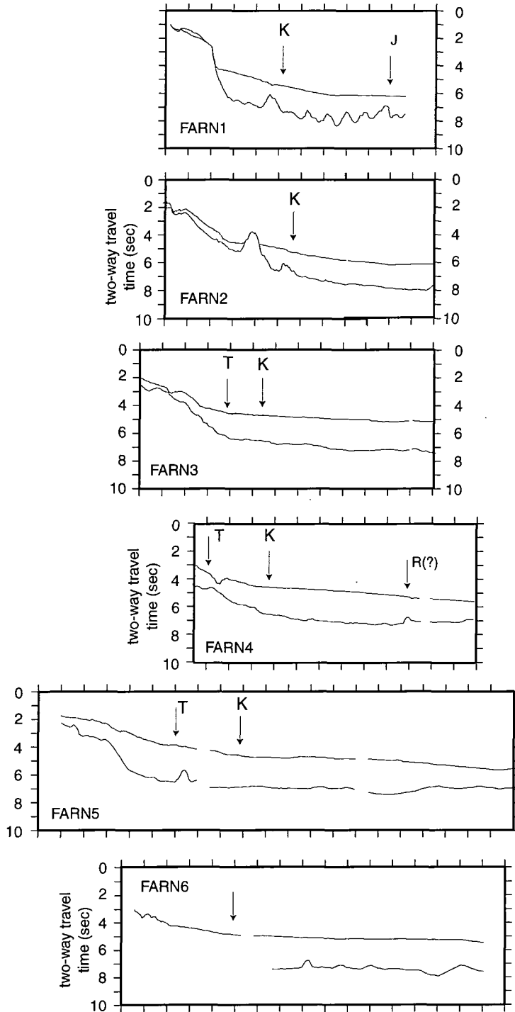
Figure 7.4 Line drawings of acoustic basement and seabed on single-channel seismic reflection profiles FARN1-FARN6 aligned parallel to the margin. Abscissa is tickmarked at 1 hour intervals, which is equivalent to ~10 km. Arrows labelled K mark the seaward extent of continental crust (from Keen and de Voogt, 1988); those labelled T mark alternative positions based on the character of the basement and the slope of the seabed. The arrow labelled R marks the position of a basement ridge downstrike of a basement ridge on MCS profile 85-4 (Fig. 7.5) which may be associated with the seaward extent of the OCT.
