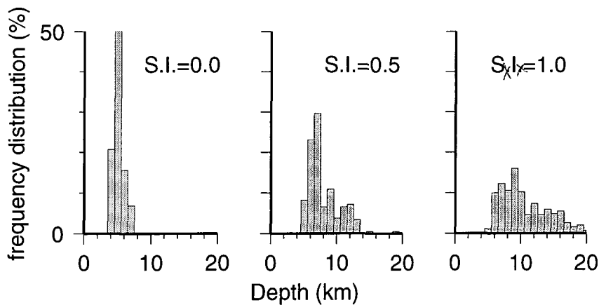
Figure 5.11 Euler deconvolution solution distributions for structural indices (S.I.) of 0.0, 0.5 and 1.0 over the region of continental crust (see Fig. 5.10).
