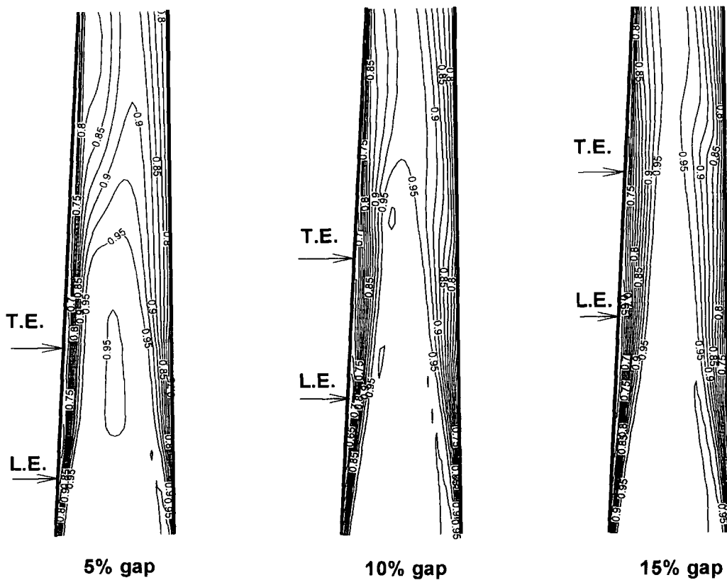
Figure 5-5 Comparison of calculated time-averaged loss contours in the diffusers in a meridional section at mid pitch
