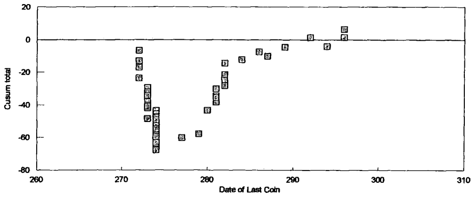
Figure 7.104: Mint 2 antoniniani of Tetricus I & II UK hoards csum
