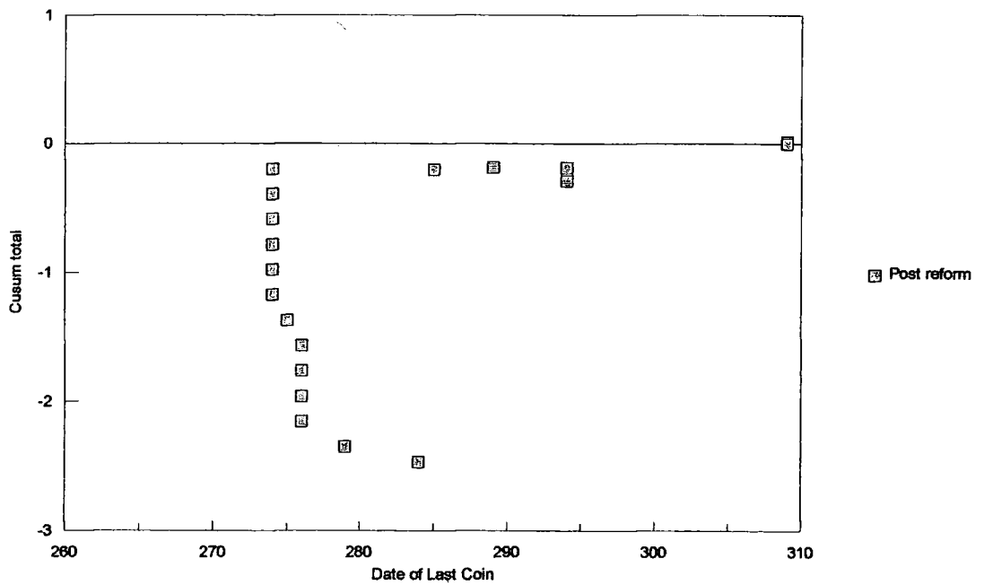
Figure 7.31: Aurelian Rome Mint post reform "aurellani" French hoards cusum
