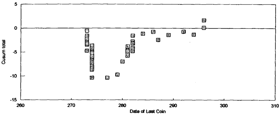
Figure 7.105: Mint 2 antoniniani of Tetricus II UK hoards csum
