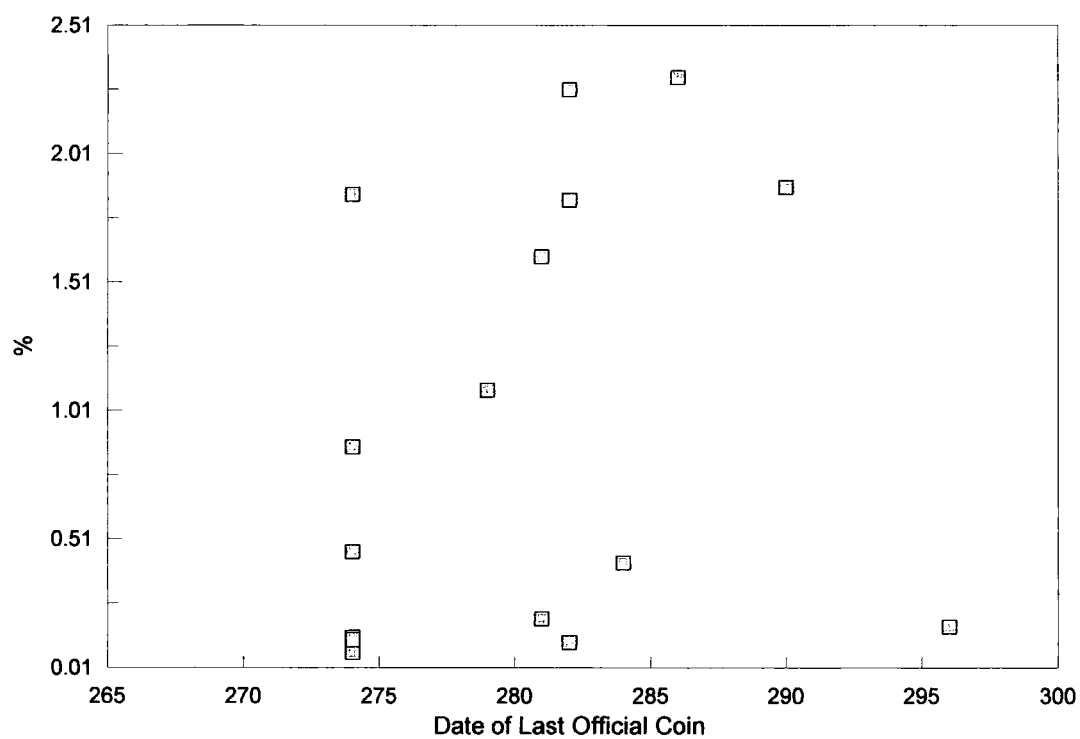
Figure 10.1: DIVO CLAVDIO imitations UK hoards
