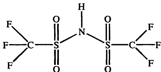
Figure 6.8a Bis(trifluoromethanesulphonyl)amide 7
