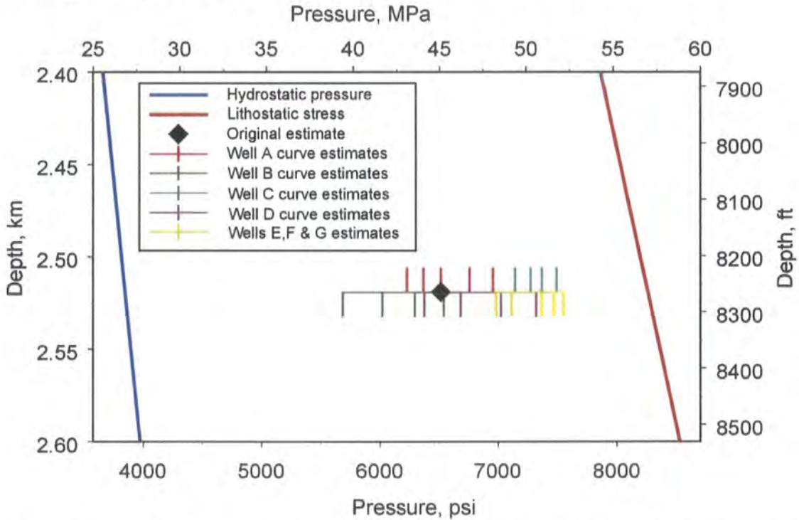
Figure 6.3 Range of pore pressures calculated by comparing the data point in Figure 6.2 against the lithology specific compaction curves shown in Figure 6.2.
