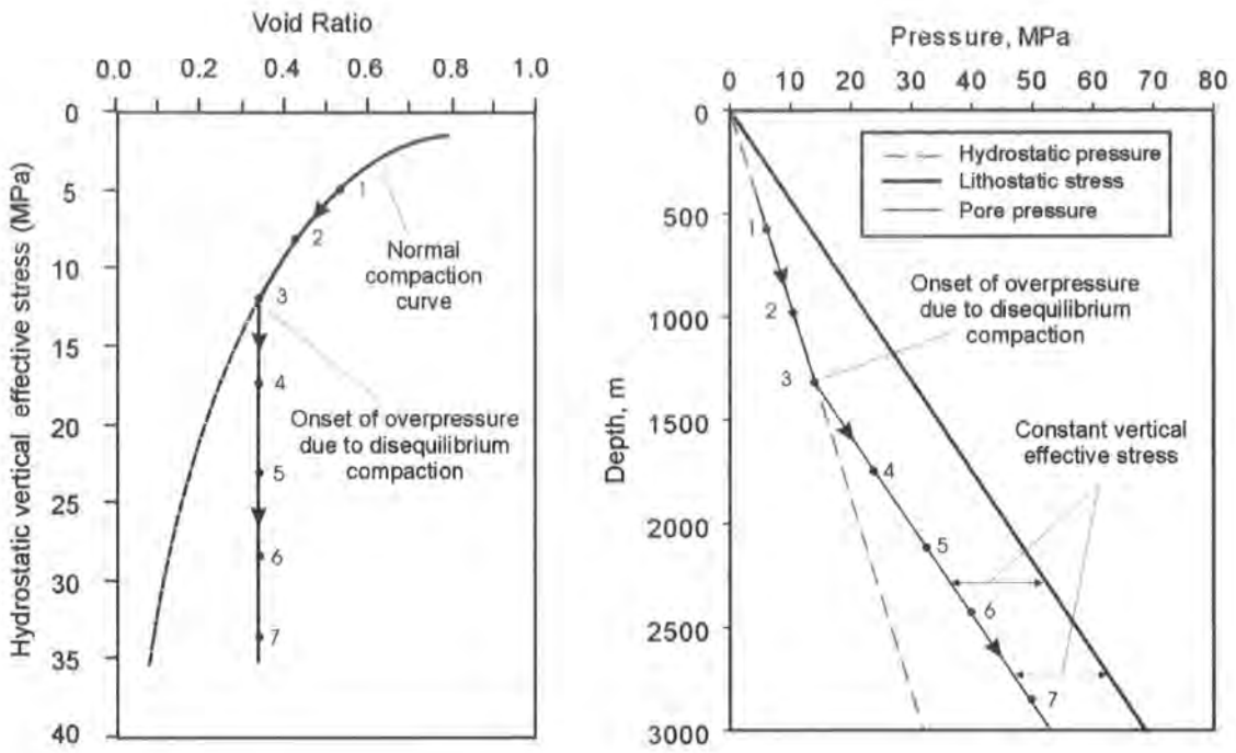
Figure 1.7 Relationship between porosity and vertical effective stress
