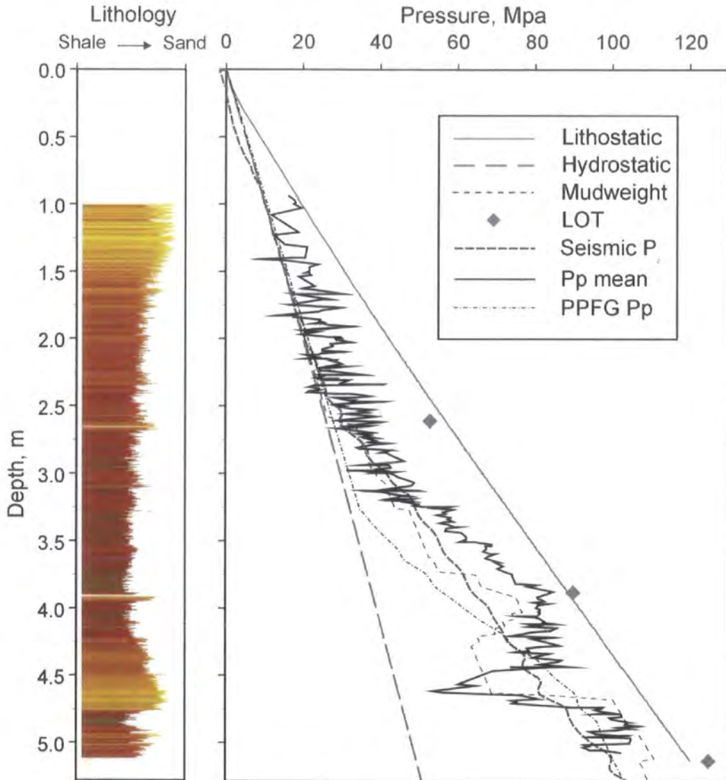
Figure 4.14 comparison of the pore pressure estimates derived from seismic PPFG and mean effective stress approaches with mudweights used to drill Well D.
