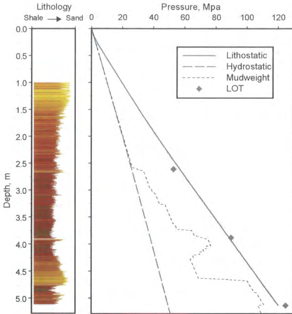
Figure 4.1 Simplified lithological column and pressure data for Well D. Shading in the lithology column represents clay fraction derived from the gamma ray log.
