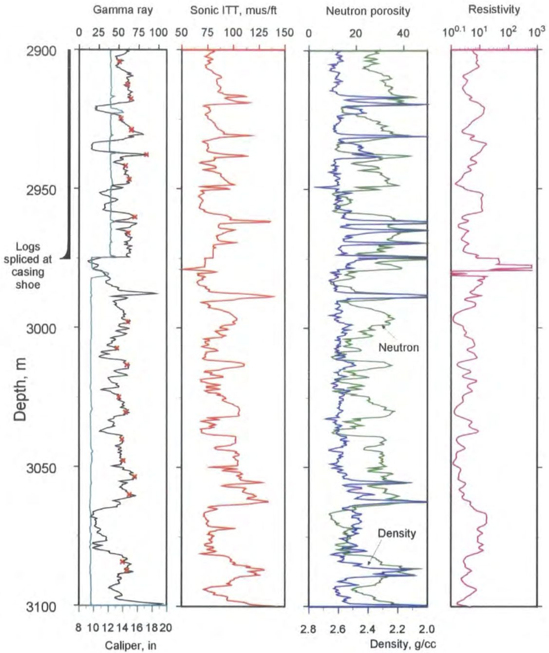
Figure 2.9: Log plot showing gamma ray, caliper, sonic, neutron, density and resistivity curves used in the pressure analysis. Points for inclusion in the analysis are marked with an X.
