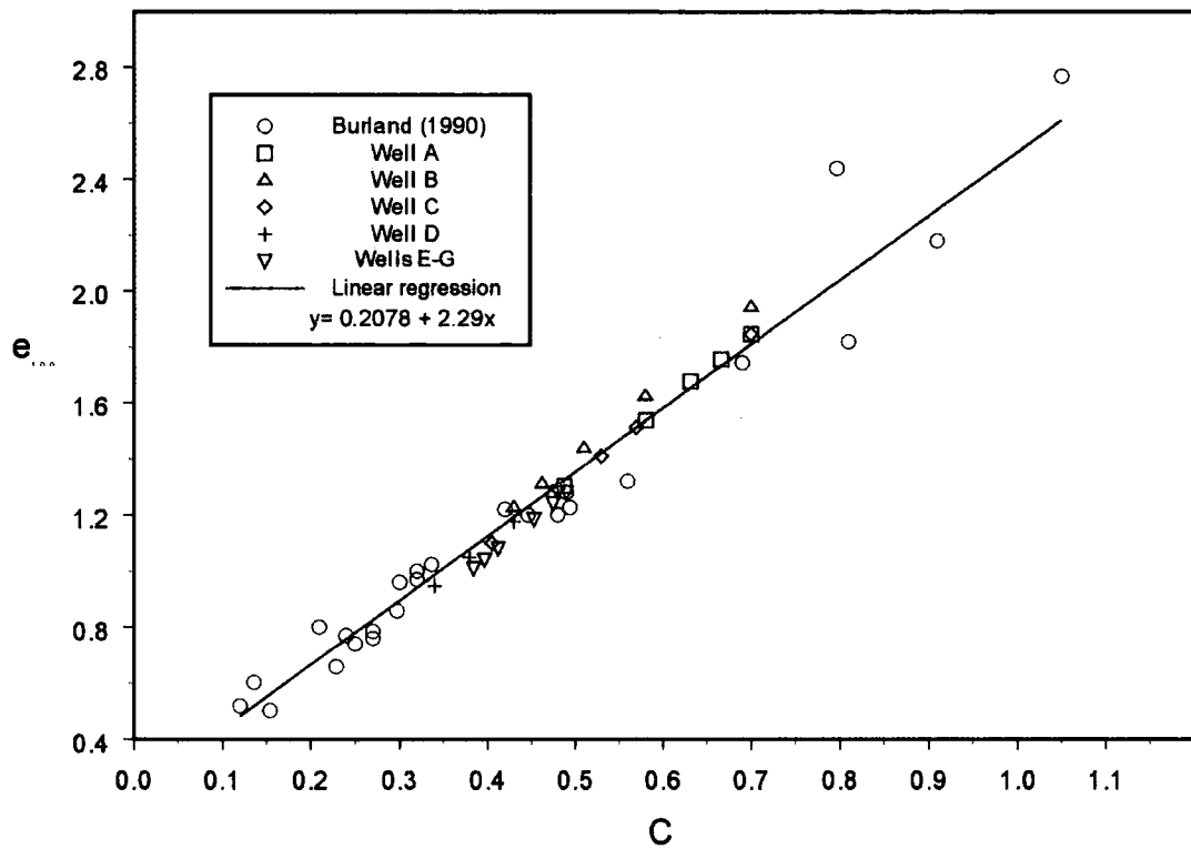
Figure 6.1: Comparison of sediment mechanical parameters e_{100} and C_c derived from direct measurements on samples (Burland, 1990) and fitting of compaction curves to porosity data in this study.
