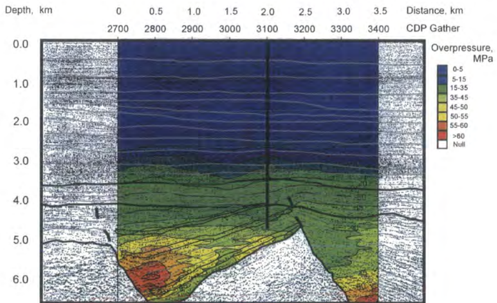
Figure 4.10. Overpressure distribution calculated using a mean effective stress approach and overlain onto the 2D seismic stack as for Figure 4.5.
