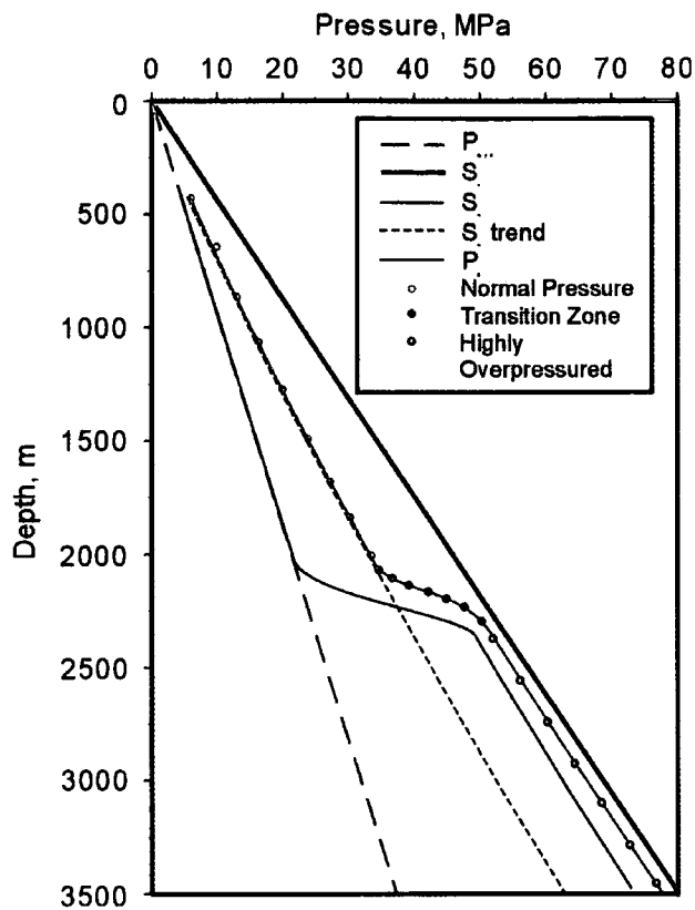
Figure 6.4a Schematic pressure plot illustrating the correlation between pore pressure and horizontal stress increase.
