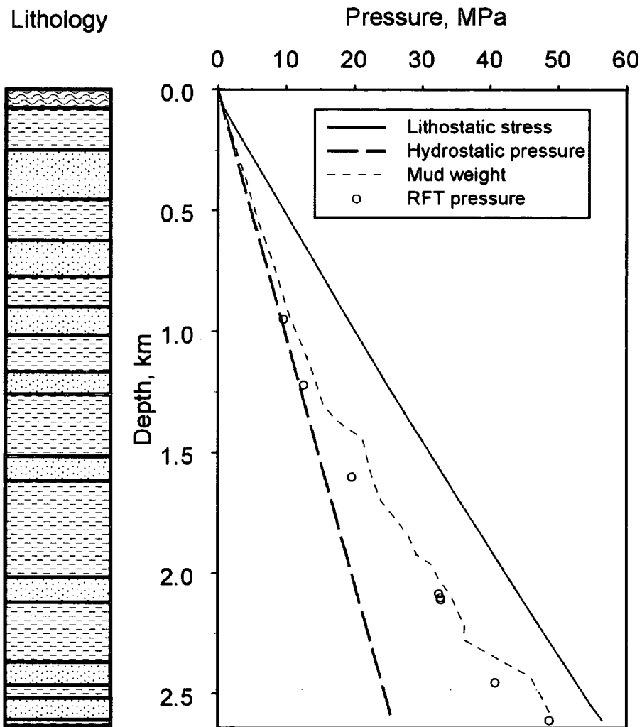
Figure 3.14 Simplified lithological column and pressure data for Well C.
