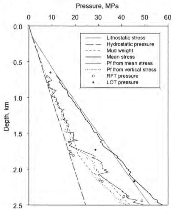
Figure 3.9 Computed pore pressures from mean and vertical effective stress for Well B plotted along with hydrostatic pressure and lithostatic stress profiles as well as direct pore pressure measurements made in the borehole.
