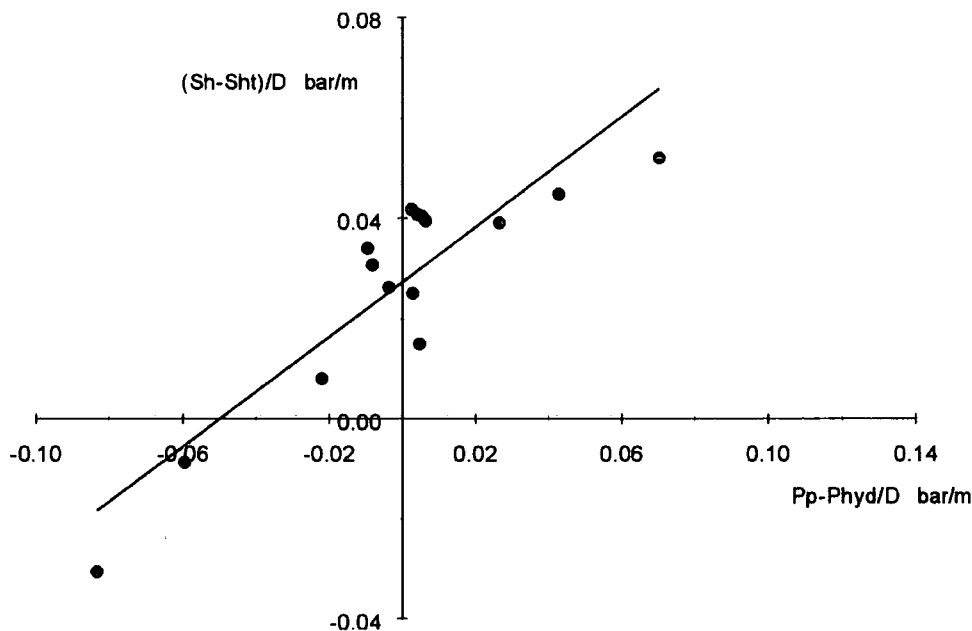
Figure 6.3 influence of overpressure ( p_p - p_{hyd} ) on the deviation of the minimum horizontal stress ( s_h ) from a normal trend ( s_{h_p} ) normalised for depth. Redrawn after Breckels and van Eekelen (1982) for Brunei data.
