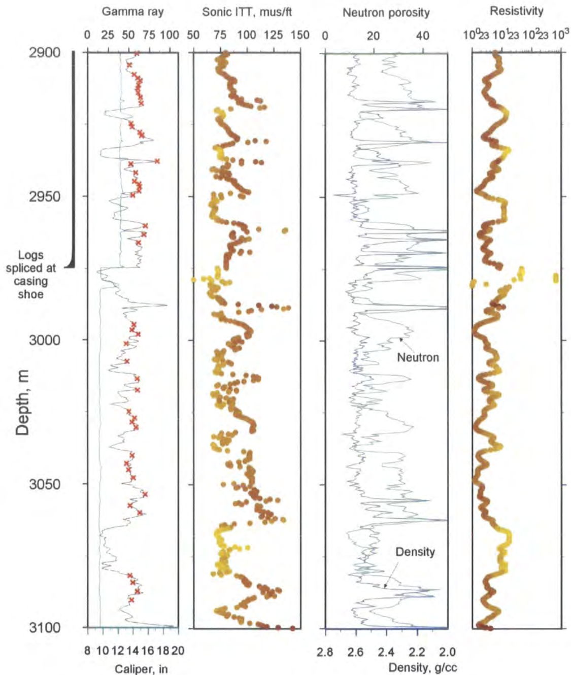
Figure 2.10: Log plot showing gamma ray, caliper, sonic, neutron, density and resistivity curves used in the pressure analysis of wells in digital format. The sonic and resistivity curves are shaded for clay fraction. Points for inclusion in the analysis are marked with an X.
