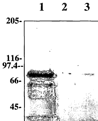
Figure 5.14 A) Gel slice protease assay of the partially purified Ara12 sample generated by differential Q Sepharose batch elution followed by fractionation on phenyl Superose. Proteins were separated on an 8% native polyacrylamide gel and the gel was cut into 2mm strips. Protein was extracted from the gel slices with 10mM Tris.HCl, pH7.5; 6.25mM CaCl 2 and protease activities of the extracts were determined with FTC-casein. B) Extracts displaying relatively high protease activities were analysed by SDS-PAGE on an 8% polyacrylamide gel. Lane 1, 10µl of partially purified Ara12 sample as applied to gel; lane 2, 10µl extract from gel slice number 4; lane 3, 10µl extract from gel slice number 5.
