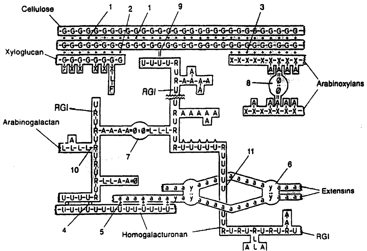
Figure 1.5 Representative primary structures and possible cross-links of wall polymers. The numbers below on the left refer to the interactions between different types of cell wall polymers illustrated above. The symbols on the right refer to the nature of those interactions. The diagram does not constitute a model of a plant cell wall and no significance is placed on the size and relative spacing of the molecules portrayed. (Figure adapted from Fry, 1986).
