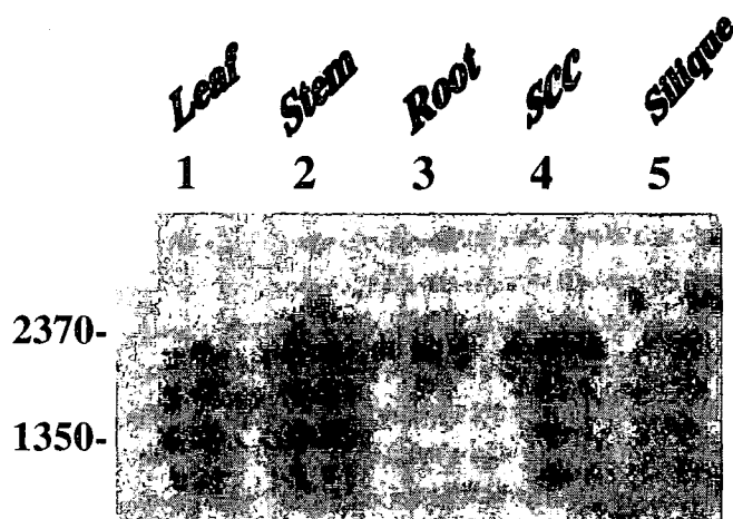
Figure 3.16 Expression of slpk mRNA as determined by Northern blot hybridisation analysis. Total RNA was prepared from Arabidopsis leaf, stem, root and silique tissues and from suspension-cultured cells (SCC). A Northern blot (10µg for each sample) was probed using the slpk cDNA probe.
