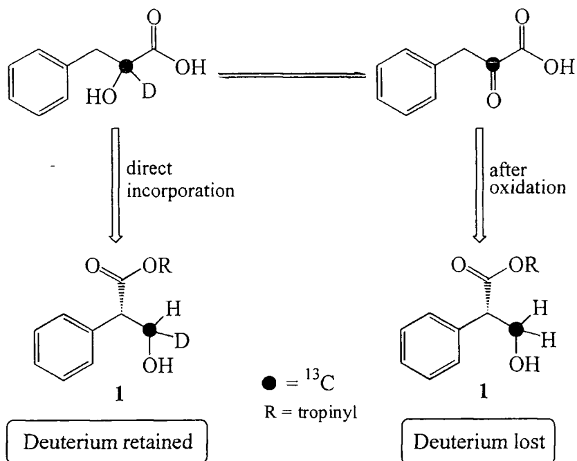
Scheme 32 Deuterium was incorporated intact into the tropate moiety of hyoscyamine ( 1 ) following a feeding experiment with [2\text{-}^{13}\text{C}, {}^2\text{H}] -phenyllactate to D. stramonium , demonstrating that phenyllactate ( 51 ) was the closer precursor than phenylpyruvate ( 38 ) to tropic acid ( 35 ).
