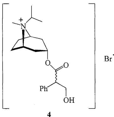
Figure 3 Ipratropium bromide (4), a synthetic analogue of atropine (2) is used in modern medicine as an effective inhaled anti-asthmatic drug, and is marketed by the pharmaceutical company, Boehringer Ingelheim, under the proprietary name, Atrovent ® .
