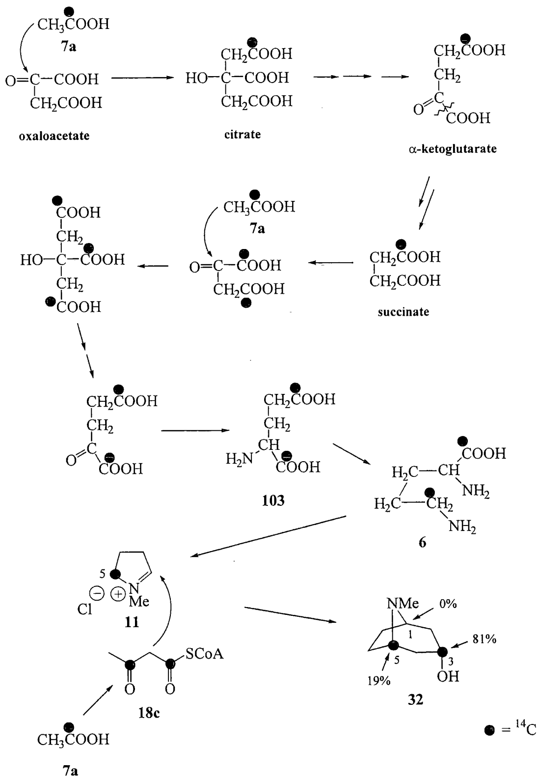
Scheme 84 The incorporation of [1-^{14}\text{C}] -acetate (7a) into the tropane (32) via the Krebs cycle.
