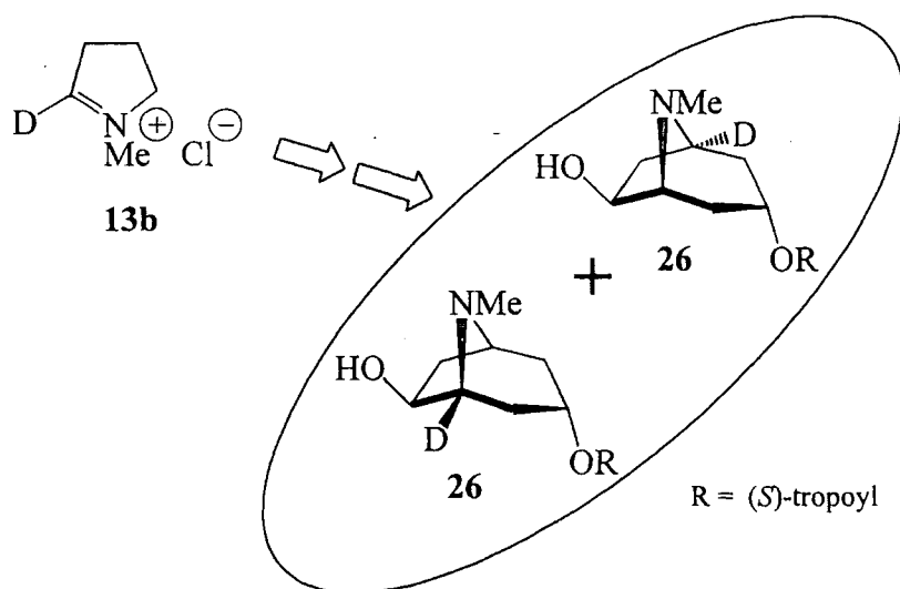
Figure 8 Deuterium was found to be incorporated into both bridgehead carbons of 6 \beta -hydroxyhyoscyamine (26) after feeding N-methyl-[2- ^2\text{H} ]-pyrrolinium chloride (13b) to D. stramonium .
