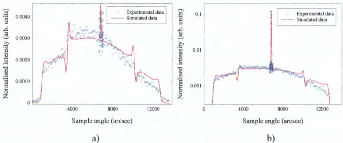
Figure 7.8. Fe/Au (111) grown on sapphire, thick buffer, a) diffuse scan through Kiessig minimum, b) log scale, \lambda = 0.8 \text{ \AA} .
