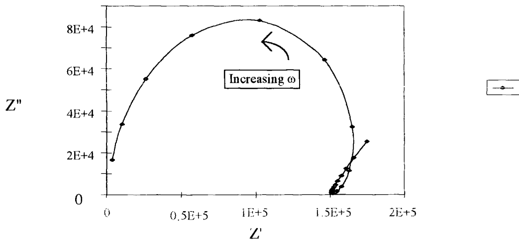
Figure 5.7 (b) - Locus of impedance with frequency in complex plane for sample of Zn_2GeO_4 at 89% r.h.
