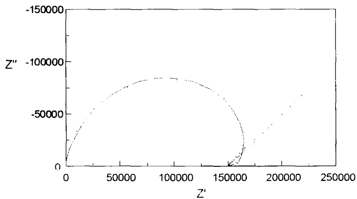
Figure 5.9 (b) - Experimental data and simulation for sample of Zn_2GeO_4 at 89% r.h.
