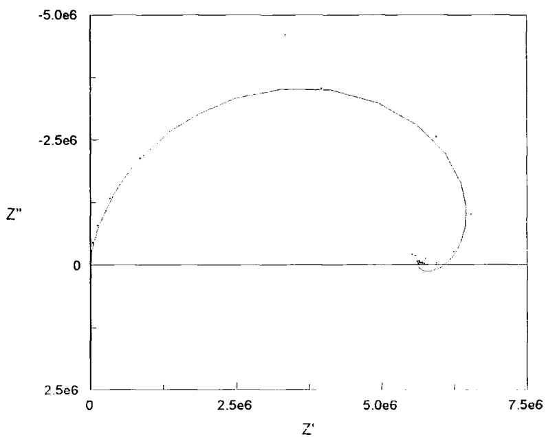
Figure 5.9 (d) - Experimental data and simulation for sample of Zn 2 GeO 4 at 68% r.h.
