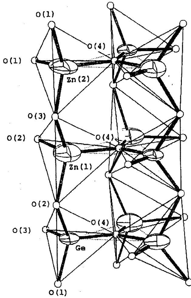
Figure 2.4 - \text{MO}_4 in the zinc germanate structure 42
