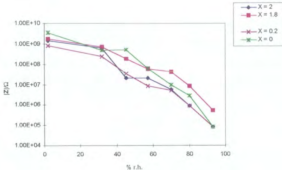
Figure 5.4 - Impedance versus humidity for sample of compositions Zn_xCo_{2-x}GeO_4 , for various x , at 173 Hz.
