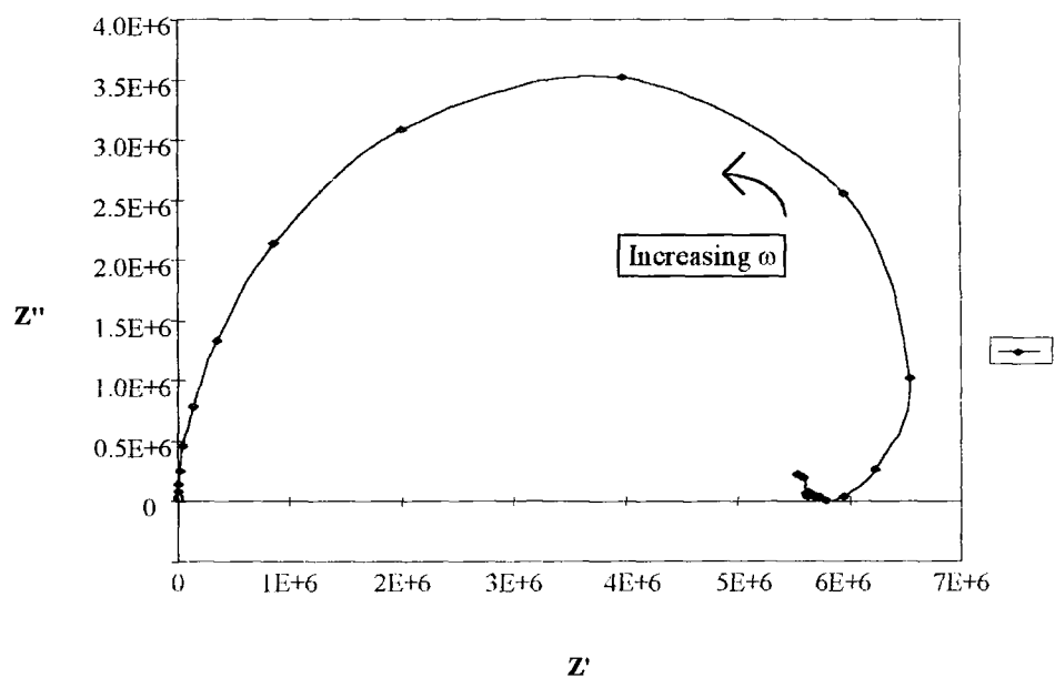
Figure 5.7 (d) - Locus of impedance with frequency in complex plane for sample of Zn_2GeO_4 at 68% r.h.
