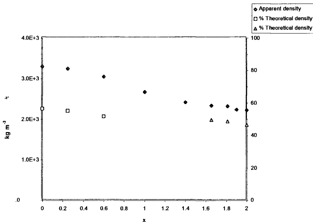
Figure 3.7 - Apparent density versus composition for Zn_xCo_{2-x}GeO_4 in kg\ m^{-3} and as a percentage of theoretical density.
