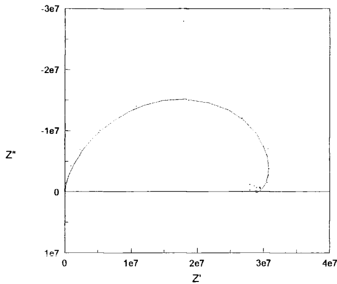
Figure 5.9 (g) - Experimental data and simulation for sample of Zn_2GeO_4 at 40% r.h.
