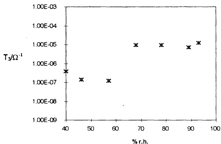
Figure 5.10 (g) - T_3 versus relative humidity
