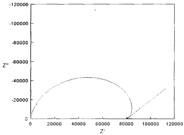
Figure 5.9 (a) - Locus of impedance with frequency in the complex plane with points showing experimental data and line showing simulated impedance of equivalent circuit for sample of Zn_2GeO_4 at 93% r.h.
