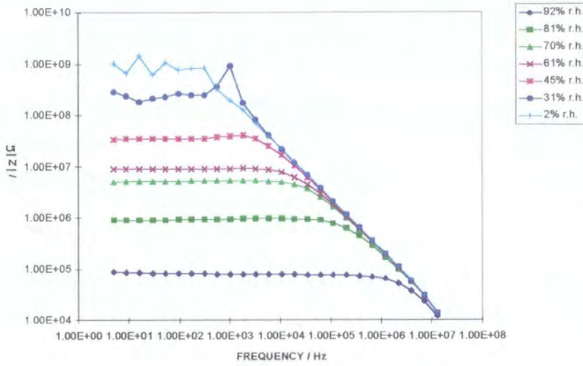
Figure 5.3 (c) - Impedance versus frequency for sample of composition Zn_xCo_{2-x}GeO_4 , x = 0.2 , at various humidities.
