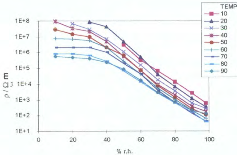
Figure 4.4 - Resistivity versus relative humidity for sample of composition Zn_xCo_{2-x}GeO_4 , x = 1.6 , at temperatures of 10 to 90°C.
