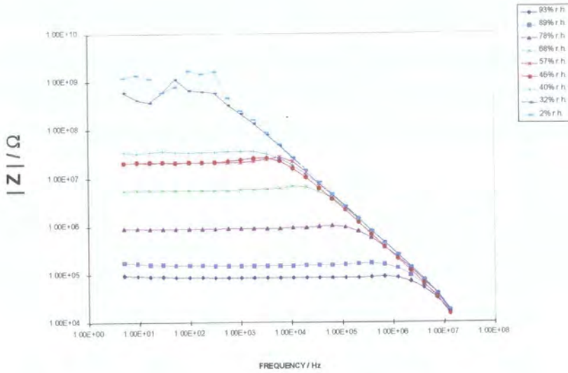
Figure 5.3 (a) - Impedance versus frequency for sample of composition Zn_xCo_{2-x}GeO_4 , x = 2 , at various humidities.
