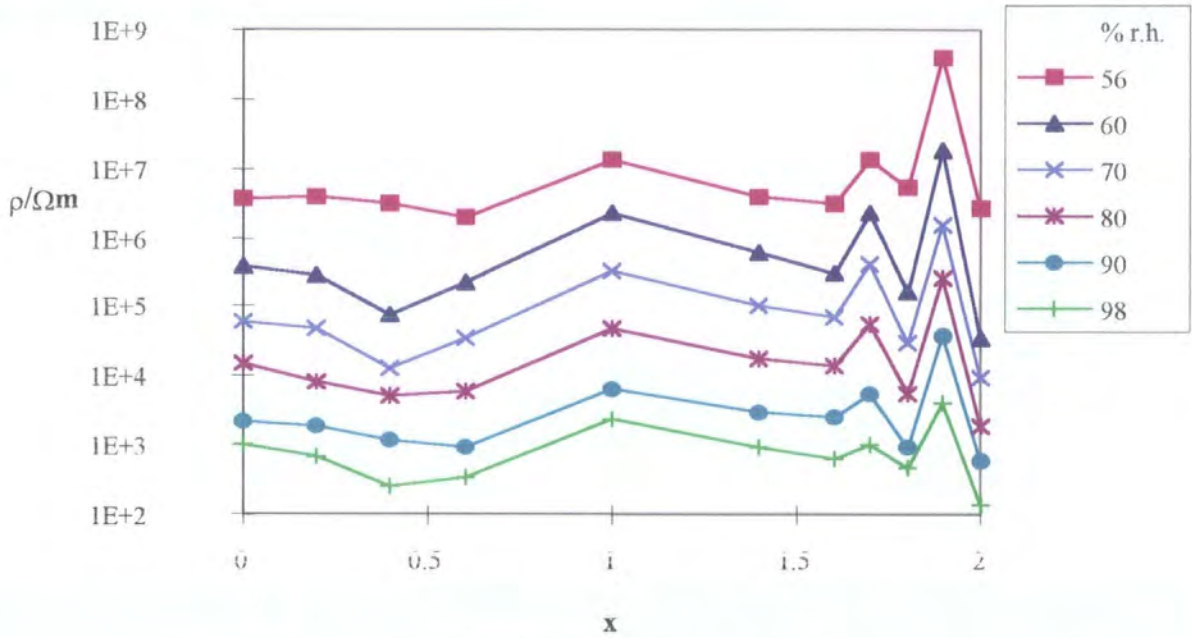
Figure A3.1 - Temperature 10 °C
