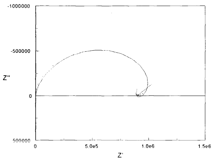
Figure 5.9 (c) - Experimental data and simulation for sample of Zn 2 GeO 4 at 78% r.h.
