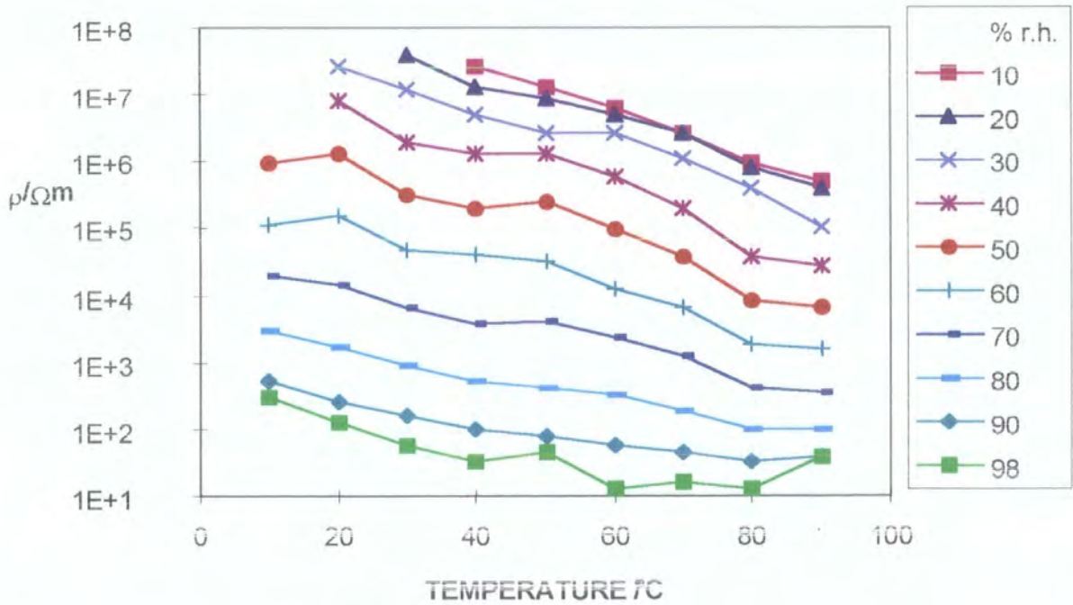
Figure A2.2 - x = 0.4
