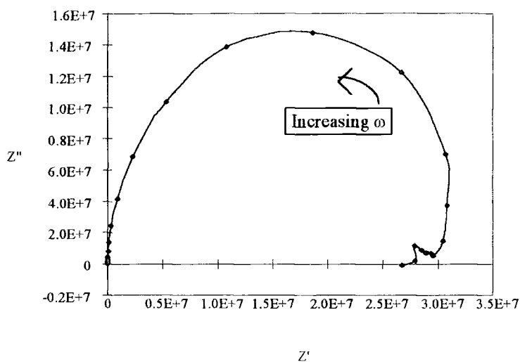
Figure 5.7 (g) - Locus of impedance with frequency in complex plane for sample of Zn_2GeO_4 at 40% r.h.
