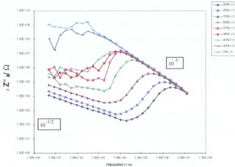
Figure 5.5 (b) - Z'' versus frequency for a sample of composition Zn_2GeO_4 at various humidities.
