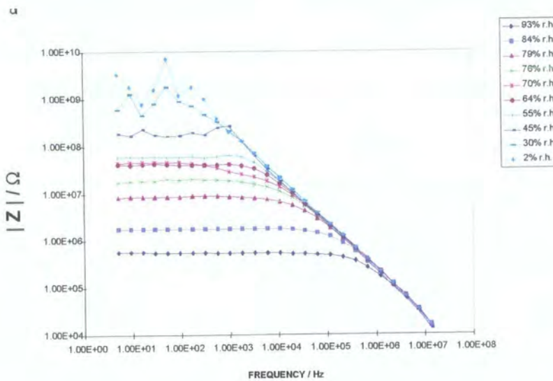
Figure 5.3 (b) - Impedance versus frequency for sample of composition Zn_xCo_{2-x}GeO_4 , x = 1.8 , at various humidities.
