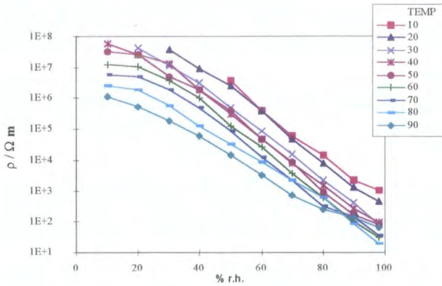
Figure 4.3 - Resistivity versus relative humidity for sample of composition Zn_xCo_{2-x}GeO_4 , x = 0 , at temperatures of 10 to 90°C.
