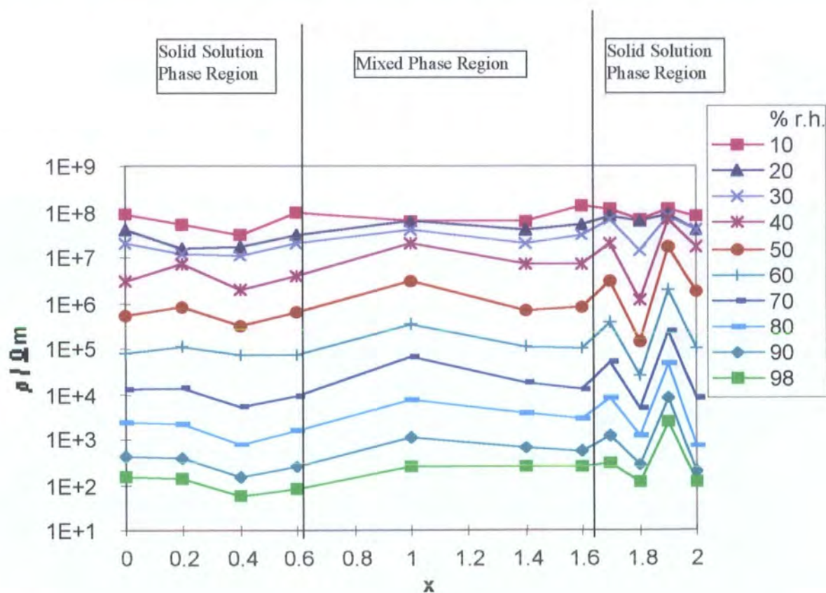
Figure 4.9 - Resistivity versus composition for samples of Zn_xCo_{2-x}GeO_4 , at 40^\circ\text{C} and various humidities.
