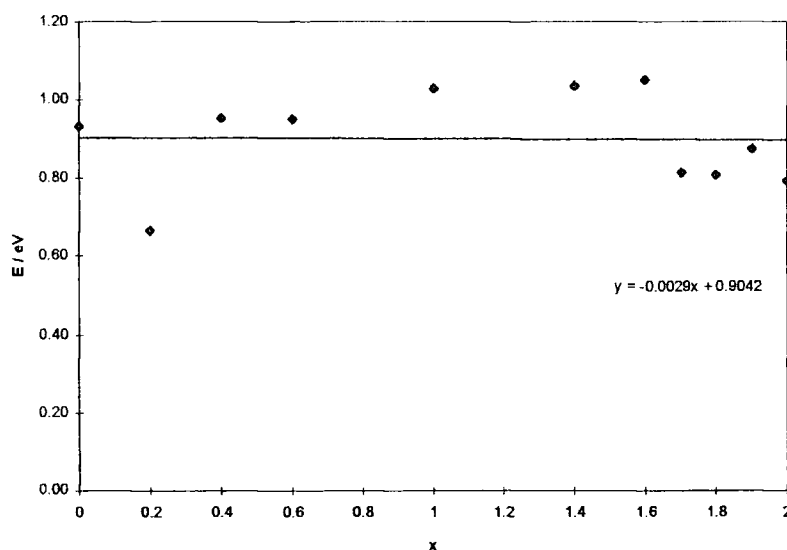
Figure 4.12 - Activation energy versus composition, x , for samples of Zn_xCo_{2-x}GeO_4 .
