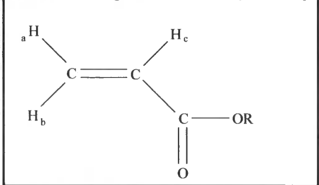
Scheme 3.8 Assignment of H's in Acrylate Groups
