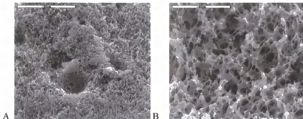
Figure 6.4 SEM Photographs (a) 2 g salt (2gs) (50 µm scale bar); (b) 2 g salt (2gs) (50 µm scale bar)
