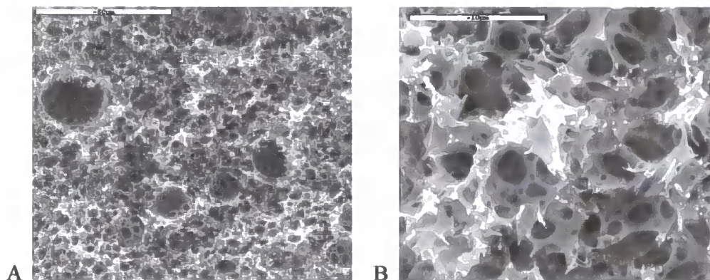
Figure 6.9 SEM Photographs (a) 0.75 g surfactant, 1.5 g salt (LSHS) (50 \mu\text{m} scale bar); (b) 0.75 g surfactant, 1.5 g salt (LSHS) (10 \mu\text{m} scale bar)
