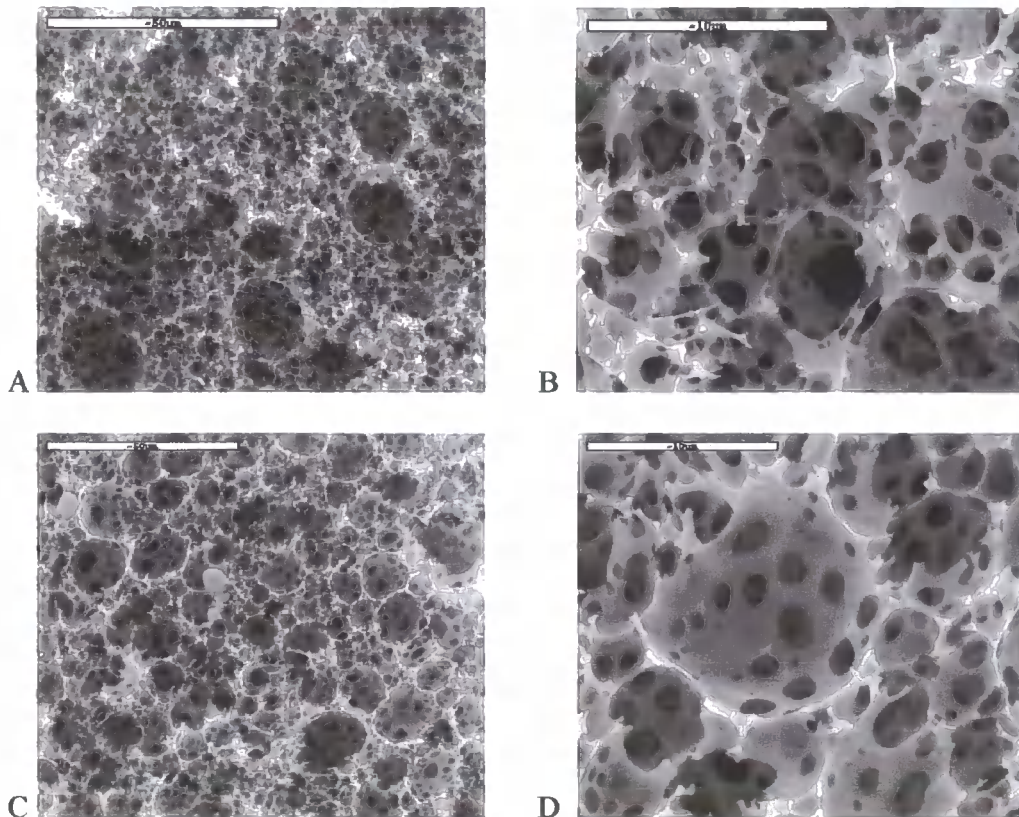
Figure 3.6 SEM Photographs (a) 0.2-H-S ( 50\mu\text{m} scale bar); (b) 0.2-H-S ( 10\mu\text{m} scale bar), (c) 0.2-L-S ( 50\mu\text{m} scale bar); (d) 0.2-L-S ( 10\mu\text{m} scale bar) *
