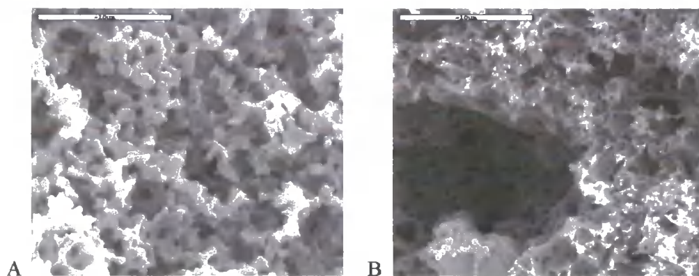
Figure 3.11 SEM Photographs(a) 0.2-L-T; (b) 0.2-H-T* (both 10 µm scale bars)
