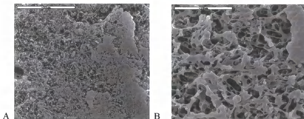
Figure 6.5 SEM Photographs (a) 3 g salt (3gs) (50 µm scale bar); (b) 3 g salt (3gs) (10 µm scale bar)
