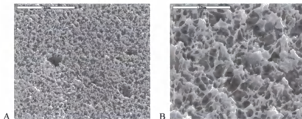
Figure 6.3 SEM Photographs (a) 1.5 g salt (HS) (50 \mu\text{m} scale bar); (b) 1.5 g salt (HS) (10 \mu\text{m} scale bar)
