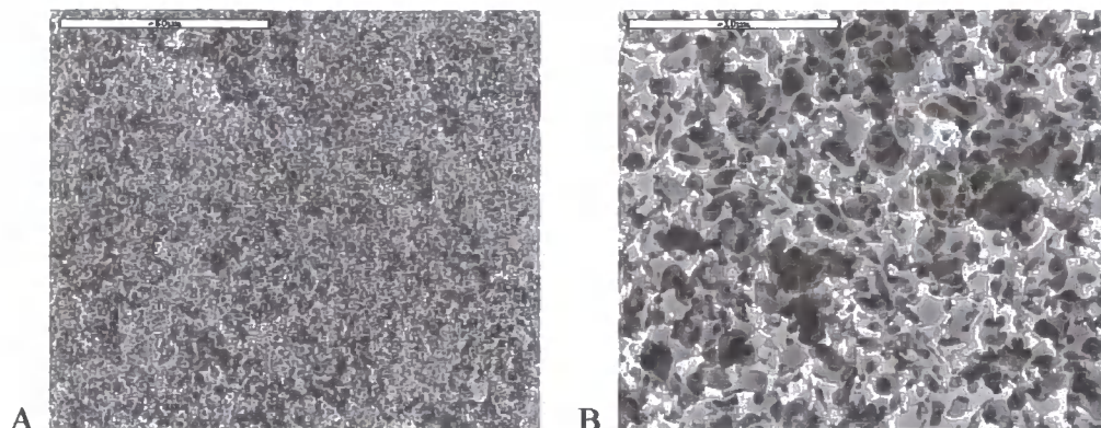
Figure 4.13 SEM Photographs (a) 0.4-M (50 µm scale bar); (b) 0.4-M (10 µm scale bar)*
