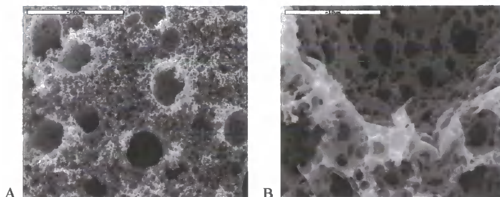
Figure 6.2 SEM Photographs (a) 1 g salt (DS) (100 \mu\text{m} scale bar); (b) 1 g salt (DS) (10 \mu\text{m} scale bar)
