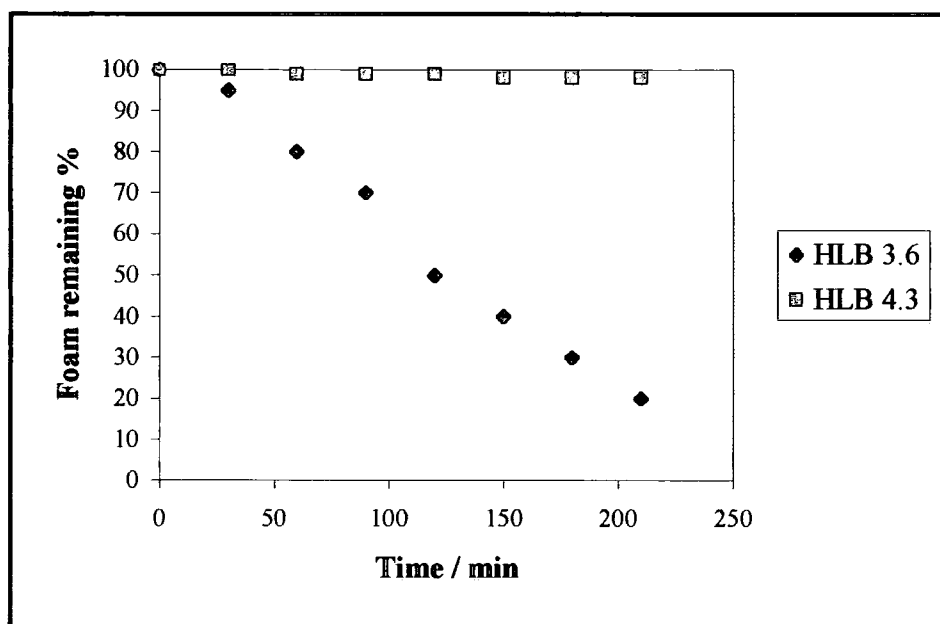
Figure 3.7 Phase Separation of 0.2-L-S HIPES Heated at 60°C
