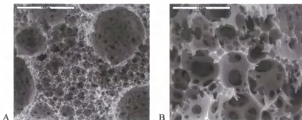
Figure 6.8 SEM Photographs (a) 0.5 g surfactant, 1 g salt (LSDS) (50 \mu\text{m} scale bar); (b) 0.5 g surfactant, 1 g salt (LSDS) (10 \mu\text{m} scale bar)
