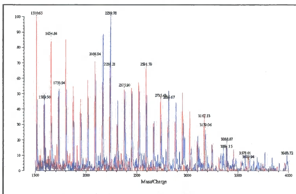
Figure 4.9 MALDI spectrum for PL diacrylate
