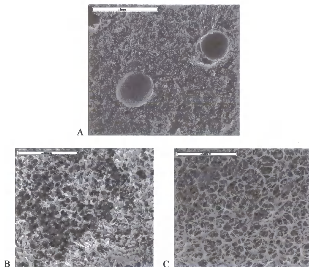
Figure 6.11 SEM Photographs (a) AIBN, 0 g salt (AIBNs)(1 mm scale bar) (b) AIBN, 0 g salt (AIBNs) (50 \mu m scale bar), non pore morphology; (c) AIBN, 0 g salt (AIBNs) (50 \mu m scale bar), morphology in cell;
