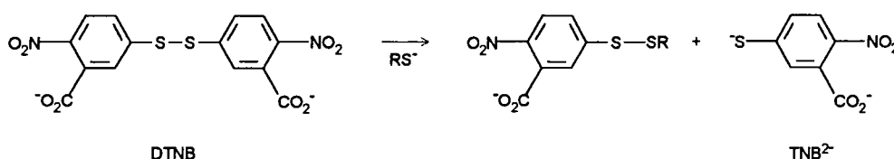
Scheme 3.4 The reaction involved in the Ellman procedure for thiol analysis
