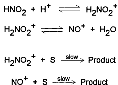
Scheme 1.3 Nitrosation of substrate S by acidified nitrous acid / NO +
