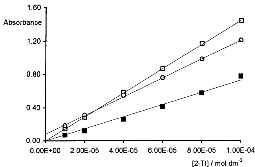
Figure 7.7 Plots of abs versus [2-TI]. ■ = water, 209 nm; □ = water, 252 nm; ○ = NaOH, 242nm
