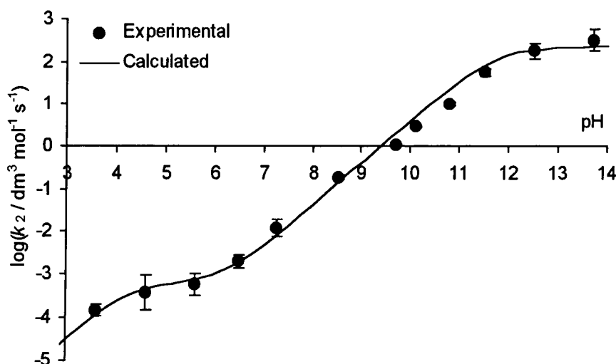
Figure 4.7 \log(k_2 / \text{dm}^3 \text{mol}^{-1} \text{s}^{-1}) versus pH for GSNO decomposition
