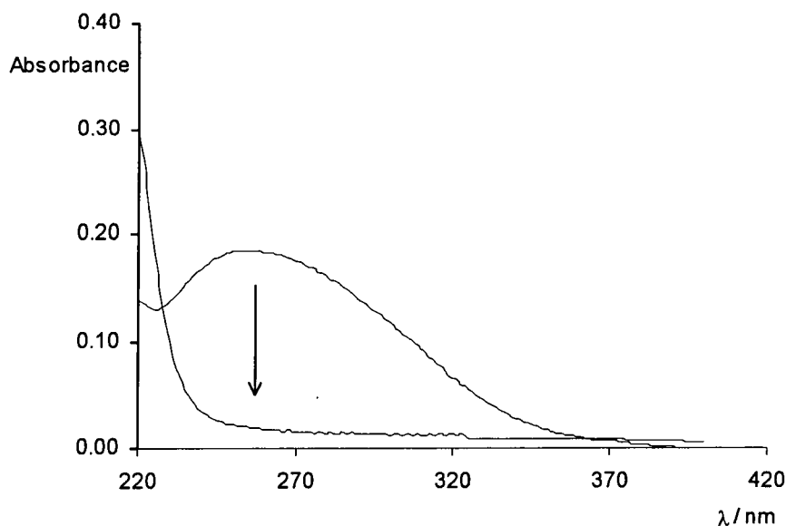
Figure 8.3 Oxidation of the S -nitrosated thioimidazole decomposition product ( [2\text{-TI}]_t = 4 \times 10^{-5} \text{ M} )
