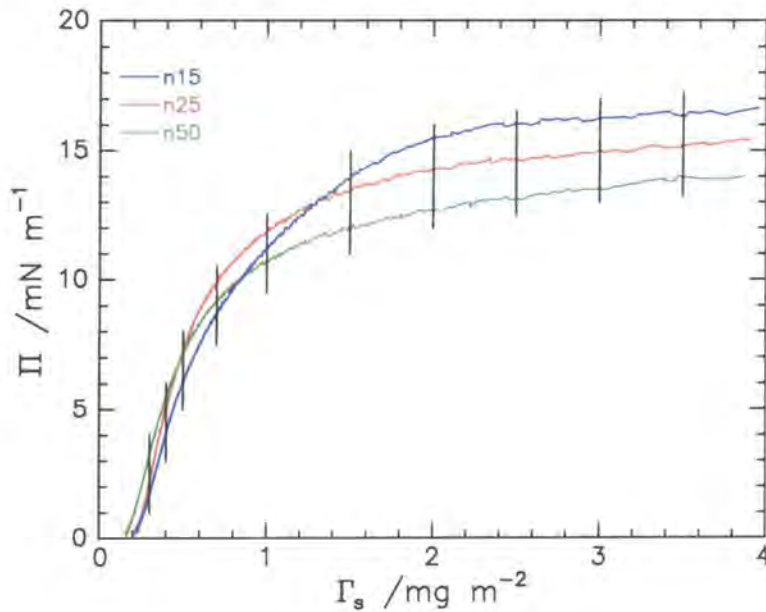
Figure 6.2.1. Surface pressure isotherms for all copolymers at the air-water interface. The lines on each plot represent the surface concentrations where neutron data was collected.
