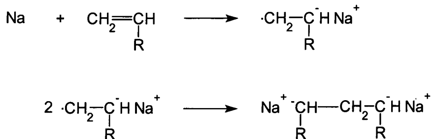
Figure 2.1.3. Preparation of propagating dianion using metallic sodium as an electron transferring agent.
