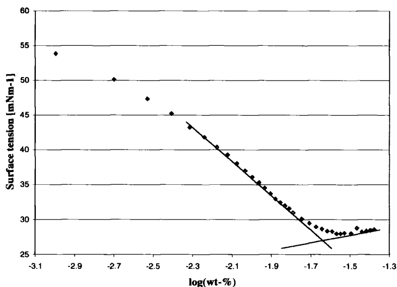
Figure 5-1: Graph of surface tension vs \log(\text{wt-\%}) concentration of Neodol 91-8 in water.
