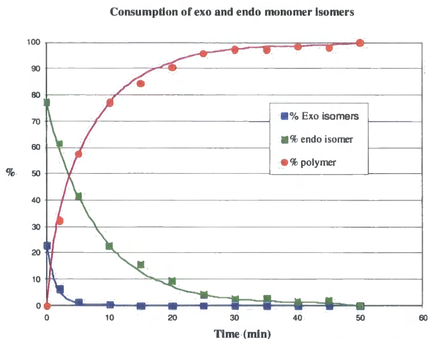
Figure 3-3: Consumption of exo and endo monomer isomers in a mixture of 5bX/N: Grubbs' Initiator (45:1 molar ratio) in H 2 O/CHCl 3 5/1 (V/V)
