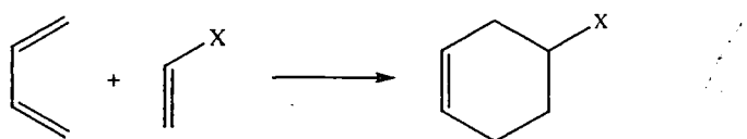
Figure 2-1: The Diels Alder reaction between a conjugated diene and an olefin.
