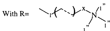
Repeat unit derived from exo monomers
