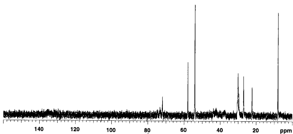
13 C-NMR spectrum (D 2 O, 100MHz) at 90 °C
