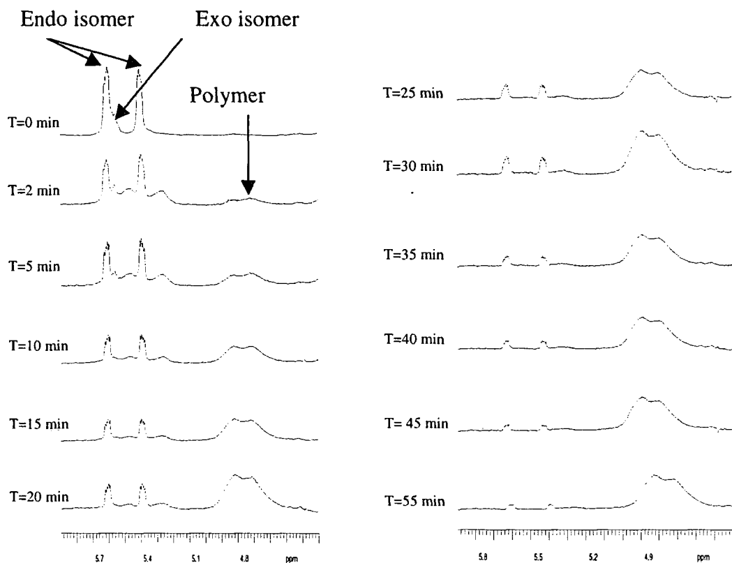
Figure 3-1: 1 H-NMR (300MHz) spectra recorded during the polymerisation of a mixture endo/exo (87/13) with Grubbs initiator.
