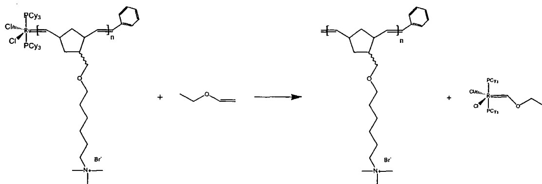
Figure 4-1: Termination reaction of the polymerisation using ethyl vinyl ether.
