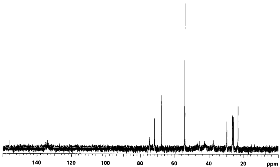
13 C-NMR spectrum (D 2 O, 100MHz) at 90 °C
