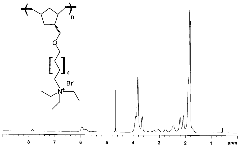
1 H-NMR spectrum (D 2 O, 400MHz) at 90 °C
