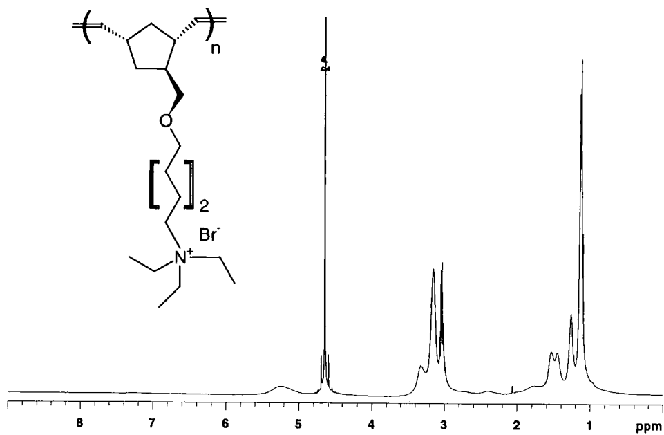
1 H-NMR spectrum (D 2 O, 400MHz) at room temperature
