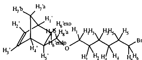
Assignment of hydrogen atoms
