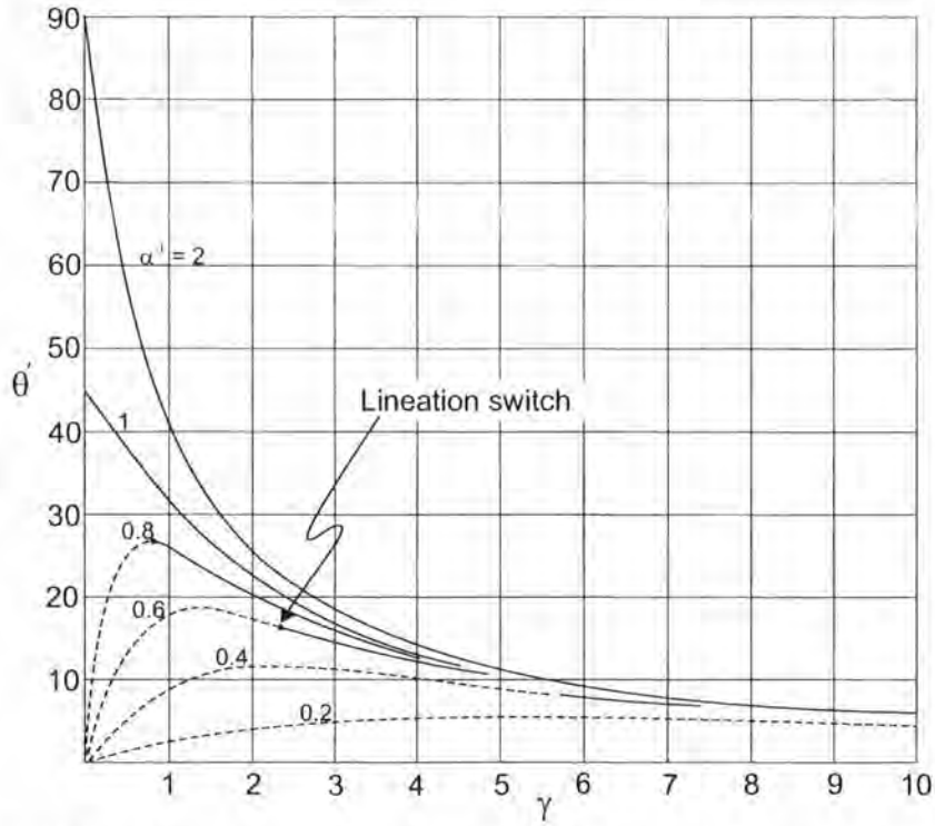
Figure 1.3. Plot of orientation of long axis of strain ellipse in horizontal plane ( \theta' ) for transpression. Continuous lines indicate X-axis horizontal, dashed lines indicate X-axis vertical (Sanderson and Marchini 1984).
