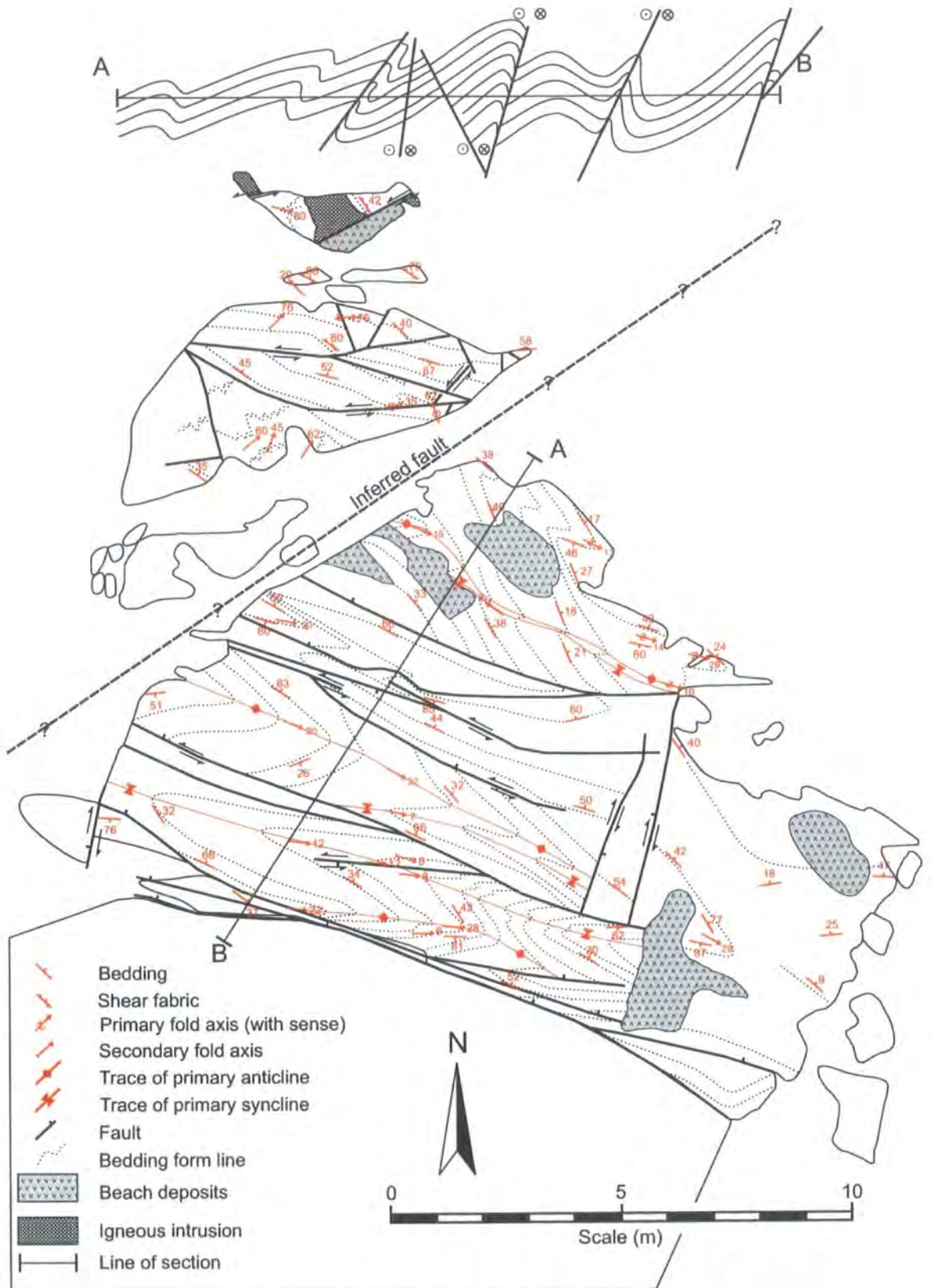
Figure 5.30. Large-scale map and cross-section to illustrate the general structure of Tract 6
