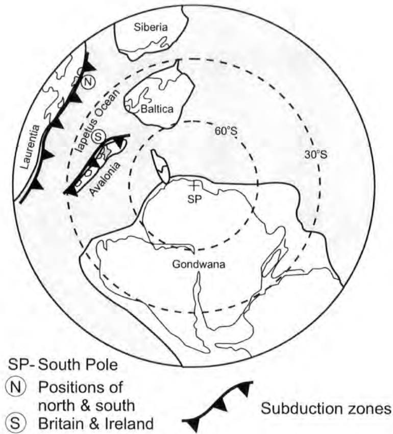
Figure 2.3. Global palaeontinental reconstruction for the Mid-Ordovician c. 470Ma. Note that not all continents are shown due to lack of data. Only selected subduction zones are shown (after Holdsworth et al. 2000).
