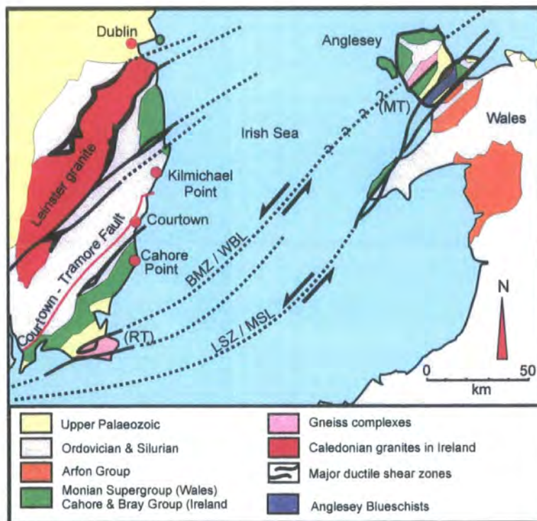
Figure 4.4. Simplified geological map of SE Ireland, Anglesey and NW Wales showing the main stratigraphic units, the relationship between the Rosslare Terrane (RT) and the Monian Terrane (MT) and major ductile shear zones (BMZ / WBL = Ballycogly Mylonite Zone / Wexford Boundary Lineament, LSZ / MSL = Llyn Shear Zone / Menai Strait Line). (Redrawn from Gibbons et al. 1994).
