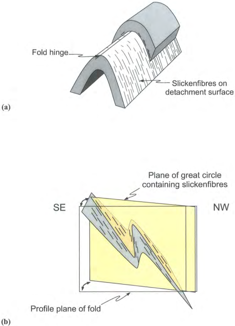
Figure 3.13. Relationship between bedding parallel detachments and slickenfibres in flexural slip folds. (a) Pattern of slicken fibres observed on bedding-parallel slip surfaces around simple flexural slip folds, where the contraction is normal to the fold hinge. Slickenfibres are perpendicular to the hinge (from Ramsay & Huber 1987). (b) Pattern of slickenfibres observed on asymmetric folds in domain 1. Note that the slickenfibres lie at an oblique angle to the fold hinge indicating oblique flexural slip.
