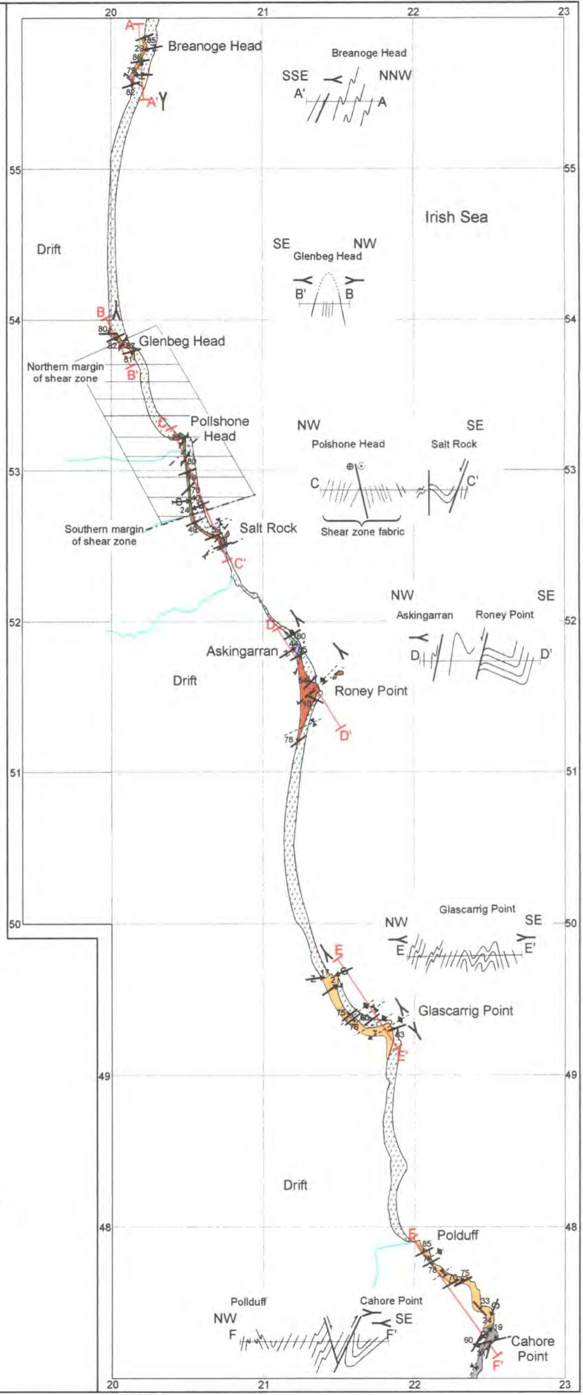
Figure 4.9. Simplified geological map and cross-sections of the coast between Cahore point and Breanoge Head
