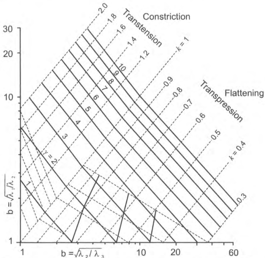
Figure 1.2. Logarithmic Flinn diagram contoured for various values of \gamma (simple shear, solid lines) and k (pure shear, dashed lines) values assuming constant volume (Fossen and Tikoff 1993).
