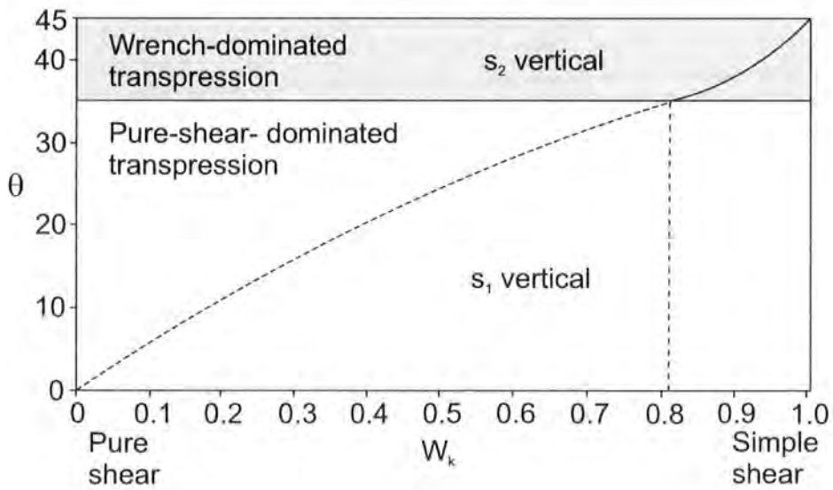
Figure 1.6. Relationship between W_k and the angle \theta , showing the transition from pure shear- to wrench-dominated transpression at w_{\text{ect}} = 0.81 and \theta = 35^\circ (Tikoff & Teysier 1994).
