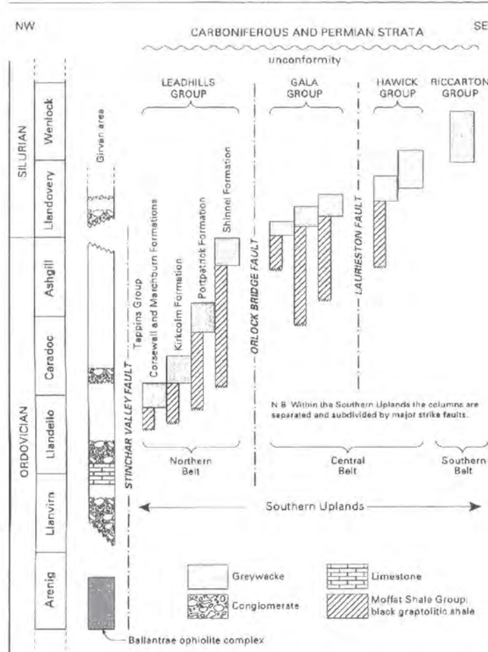
Figure 3.2. Schematic representation of stratigraphical relationships in SW Scotland (from Stone 1996).
