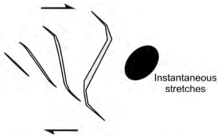
Figure 1.34. The sigmoidal form of en echelon tension gashes reflects the fact that the younger, narrower tips form as fractures initially orientated perpendicular to the maximum instantaneous stretching axis of the flow, while the older dilated central portion rotates with the same sense as the vorticity of the flow during progressive deformation (from Hanmer & Passchier 1991).
