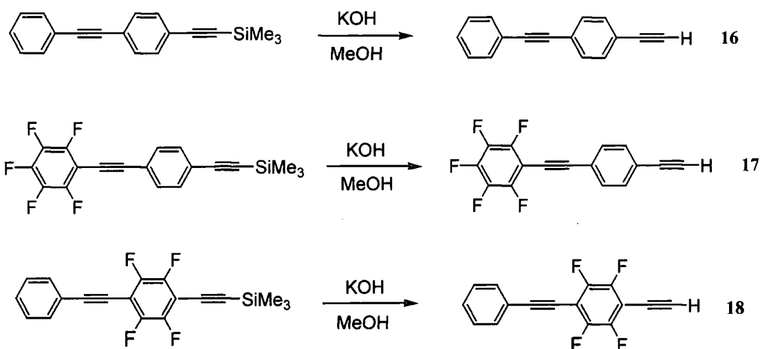
Scheme 7.4 Hydrodesilations of the 1-trimethylsilyl-4-(phenylethynyl)benzenes
