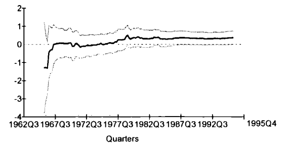
Coef. of DLRLDA(-5) and its 2 S.E. bands based on recursive OLS
