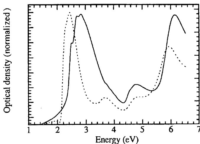
Figure 4-5 Absorption spectrum of PPV (solid line) and MEH-PPV (dashed line) reproduced from [11].
