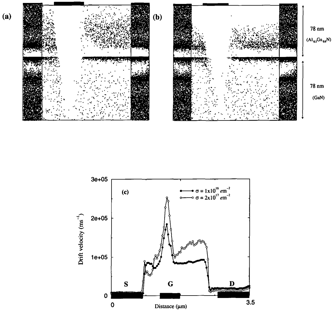
Figure 6.8: Effect of different polarization sheet charge densities on electron distribution and drift velocity through the wurtzite GaN HFET at room temperature when V_{gs} = -1 \text{ V} , V_{ds} = 30 \text{ V} . (a) \sigma = 10^{16} \text{ cm}^{-2} , (b) \sigma = 2 \times 10^{17} \text{ cm}^{-2} and (c) the associated electron drift velocity through the whole device.
