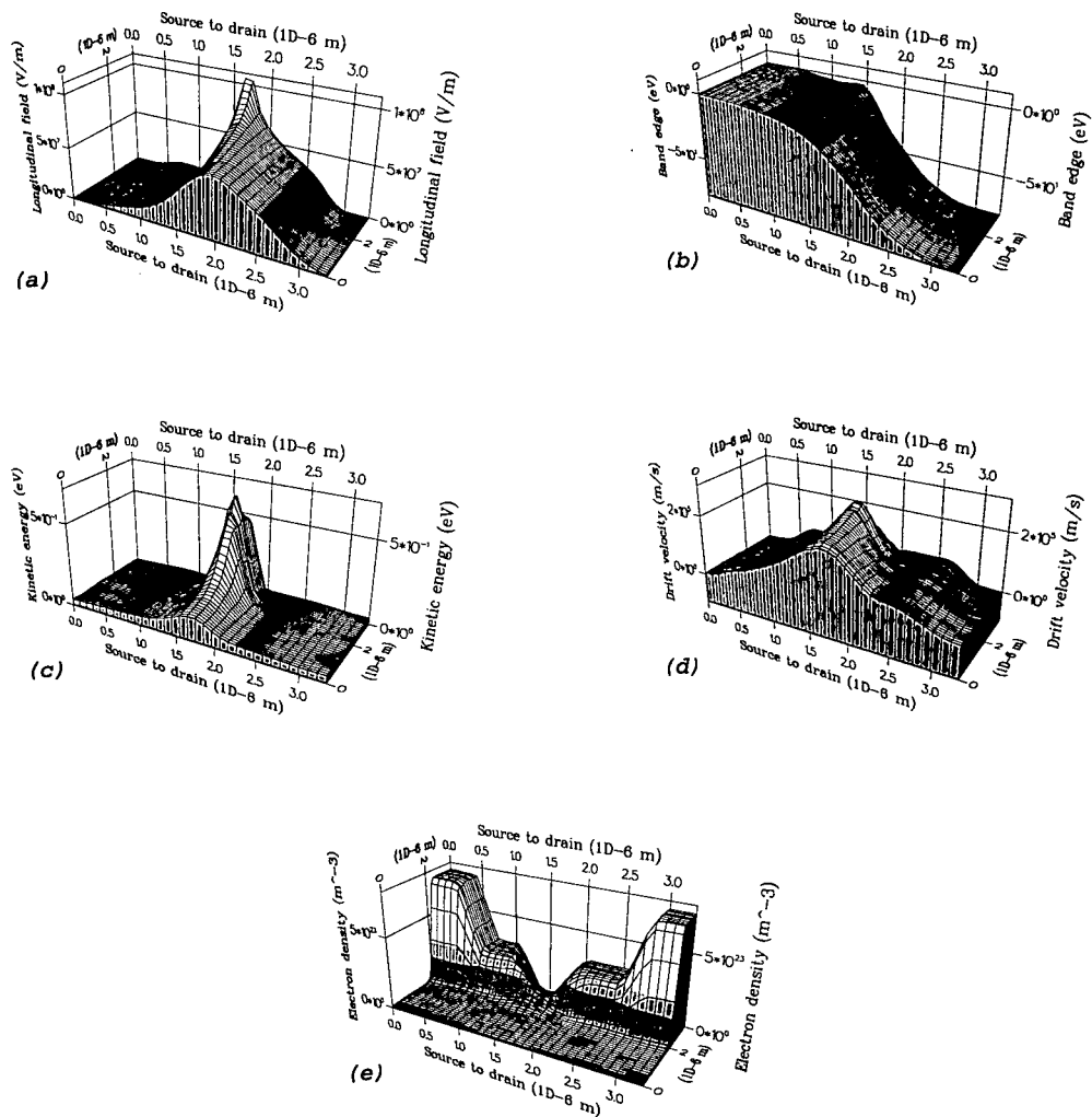
Figure 5.5: Three dimensional distribution of electron data recorded through the simulation of the GaN MESFET when the source-drain bias is 50 V and the gate voltage is -1 V at room temperature. This figure shows: (a) Longitudinal electric field, (b) \Gamma -valley conduction band profile, (c) Average kinetic energy, (d) Drift velocity and (e) Electron density.
