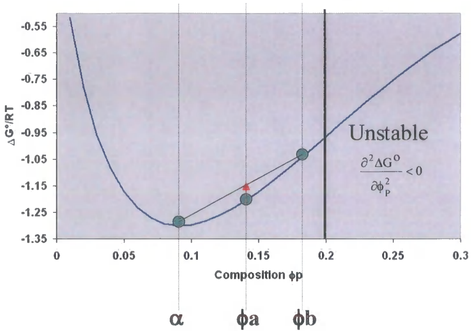
\Delta G^\circ vs Composition ( \chi=2.3 )
