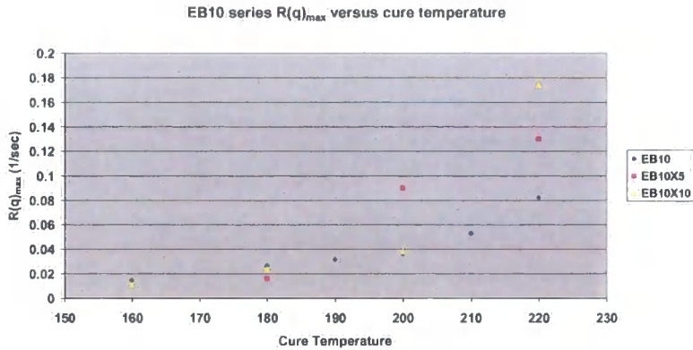
Graph 6.5.9 R(q)_{max} versus cure temperature for the primary spinodal decompositions in the series EB10
