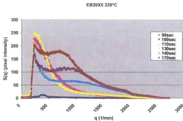
Graph 6.4.3.4 This graph shows the S(q) versus q plot for EB20X5 cured at 220°C. This shows the formation of a two spinodal peaks, one at low q early in the cure process and a secondary peak occurring after 130sec
