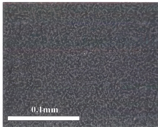
Figure 6.4.1.2 Optical micrograph of EB10X5 cured isothermally at 180^\circ\text{C} . This shows a small scale particulate morphology
