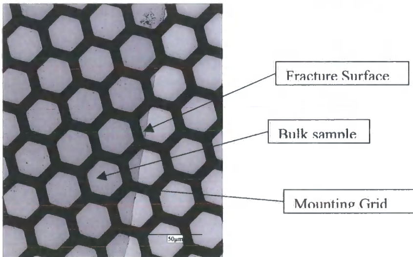
Figure 7.3.1 TEM micrograph of EBN15 showing the particulate morphology. The black honeycomb pattern is the TEM support grid.
