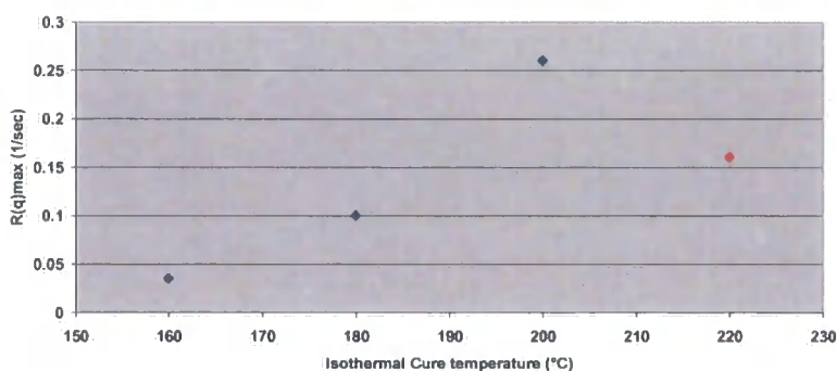
EB25X5 R(q)_{max} versus Cure Temperature
