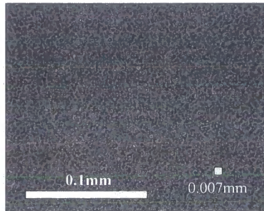
Figure 5.4.1.3 Optical micrograph of EB10 cured at 180°C. This shows a particulate morphology. The size of the dispersed particulates is very regular which suggest that the microstructure has formed by undergoing a PCT.
