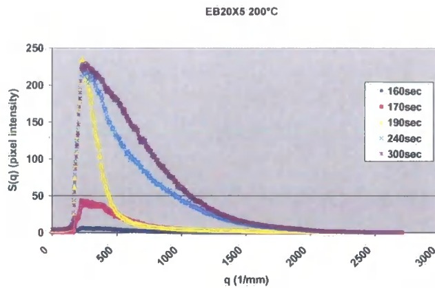
Graph 6.4.3.3 This graph shows the S(q) versus q plot for EB20X5 cured at 200°C. This shows the formation of a spinodal peak at low q
