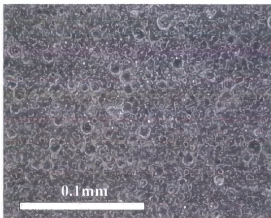
Figure 5.4.2.1 Optical micrograph of EB15 cured at 150 °C. This shows a particulate morphology with a range of different particle sizes. The scattering profile from this sample shows a well-defined spinodal peak that suggests the morphology has formed by a percolation to cluster transformation.
