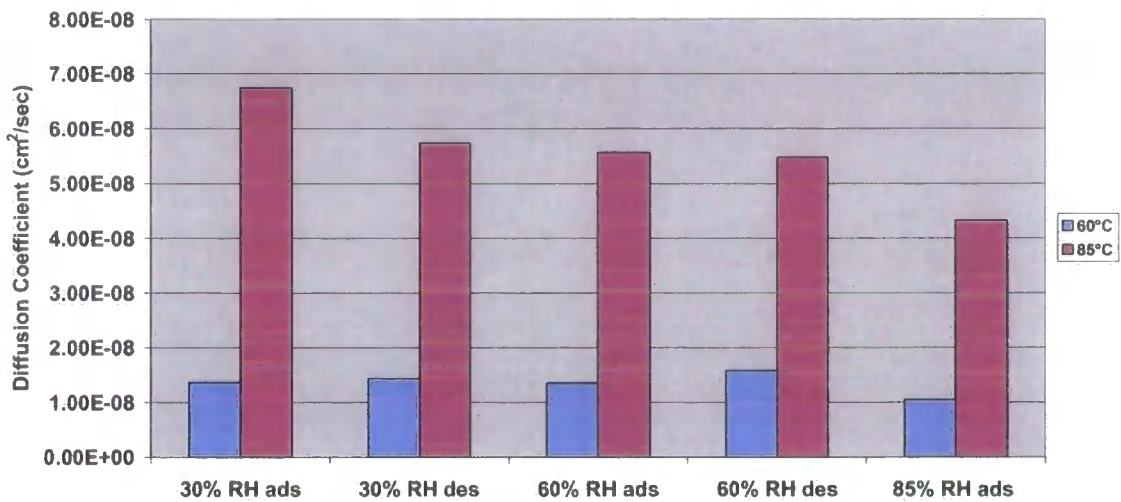
Graph 7.3.13 Diffusion Coefficients for EBN22.5 for adsorption and desorption isotherms at 60°C and 85°C. (ads= adsorption, des= desorption)
