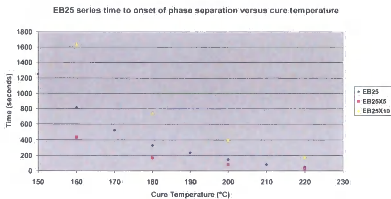
Graph 6.5.4 Time to onset of phase separation versus cure temperature for EB25 series.
