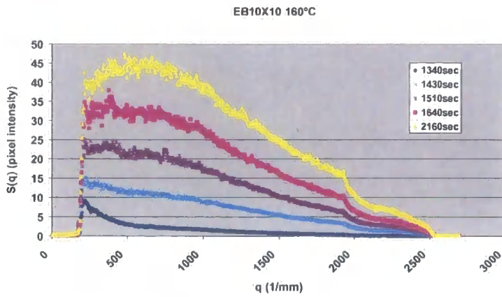
Graph 6.4.5.1 S(q) versus q plot for EB10X10 cured at 160 °C
