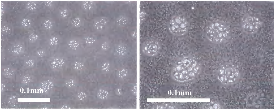
Figure 5.4.3.1 Optical micrographs of EB20 cured at 160°C. This morphology shows large discontinuous particles inside of which are particles from a secondary phase separation. The continuous phase also has small-scale dispersed particles resulting from a secondary phase separation.
