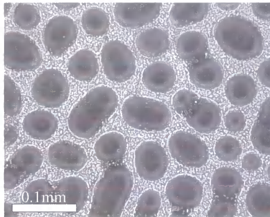
Figure 5.4.4.3 Optical micrograph of EB25 cured at 170°C. This shows a large two phase morphology that has formed from a percolation to cluster transformation. The continuous phase contains sub-included particles as a result of secondary phase separation.
