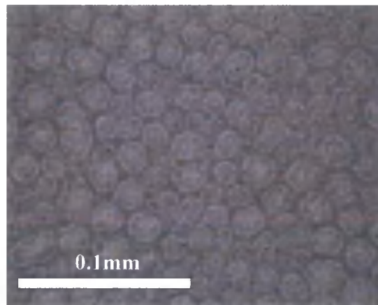
Figure 6.4.3.1 Optical micrograph of EB20X5 cured at 160°C showing a minor continuous phase and a major dispersed phase. It is likely that the continuous darker phase is the thermoplastic rich phase.
