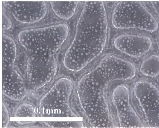
Figure 5.4.4.1 Optical micrograph of EB25 cured at 150°C. This morphology shows a continuous minor phase with a discontinuous majority phase containing sub- included particles from secondary phase separations.
