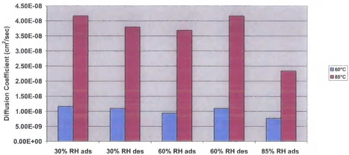
Graph 7.3.12 Diffusion Coefficients for EBN15 for adsorption and desorption isotherms at 60 °C and 85 °C. (ads= adsorption, des= desorption)
