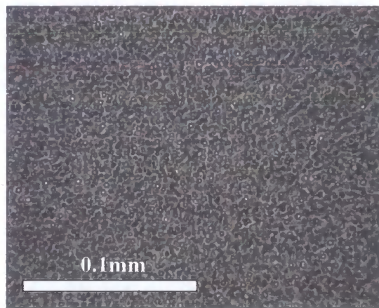
Figure 6.4.6.1 Optical micrograph of the cured morphology of EB15X10 cured at 160^{\circ}\text{C}
