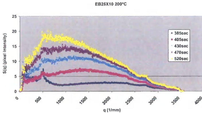
Graph 6.4.8.3 S(q) versus q plot for EB25X10 cured at 200 °C. This shows the formation of a broad spinodal peak.
