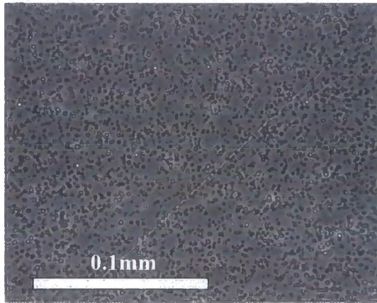
Figure 5.4.1.5 Optical micrograph of EB10 cured at 200 °C. This shows a particulate morphology that has formed from a percolation to cluster transformation.
