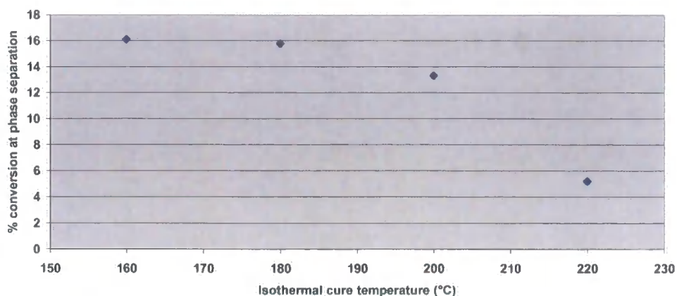
EB25X5 % conversion at onset of phase separation versus cure temperature
