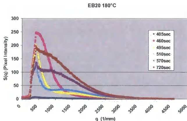
Graph 5.4.3.3 S(q) versus q for EB20 cured at 180°C. This scattering profile shows two spinodal peaks. A primary spinodal peak begins to form after 410 seconds at low q , this develops and shifts to lower q . At 510 seconds into the cure a second spinodal peak forms at a q value of 1500 \text{mm}^{-1}
