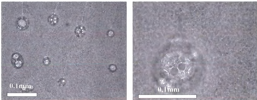
Figure 5.4.3.4 Optical micrographs of EB20 cured at 190 °C. This morphology shows large discontinuous particles inside of which are two different phases resulting from a secondary phase separation. The continuous phase also has small-scale dispersed particles resulting from a secondary phase separation.
