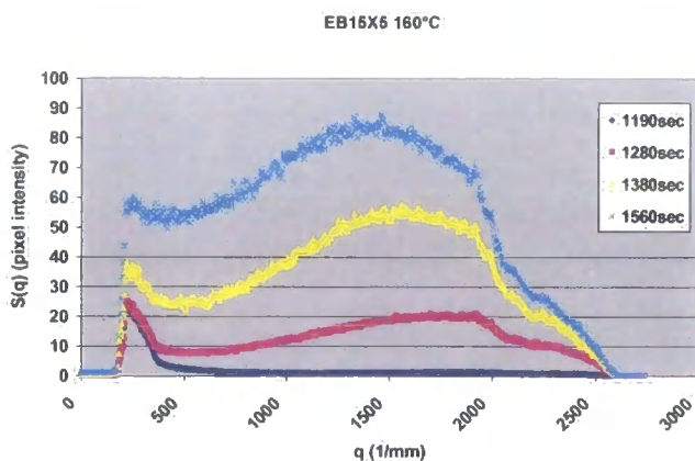
Graph 6.4.2.1 S(q) versus q plot for EB15X5 cured at 160°C
