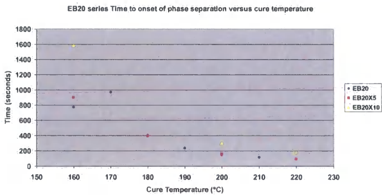
Graph 6.5.3 Time to onset of phase separation versus cure temperature for EB20 series.
