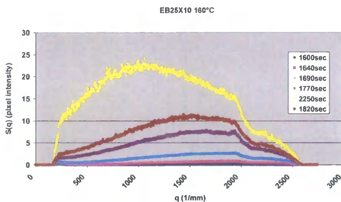
Graph 6.4.8.1 S(q) versus q plot for EB25X10 cured at 160°C. This shows the formation of a broad spinodal peak. At high q this has an unusual shape to the curve, which may indicate that some secondary small-scale phase separation event is occurring.
