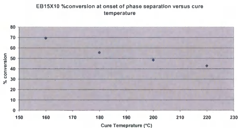
Graph 6.4.6.8 This graph shows the relationship between the isothermal cure temperature and the % conversion at the onset of phase separation for EB15X10. The decreasing conversion with increasing cure temperature suggests LCST behaviour.
