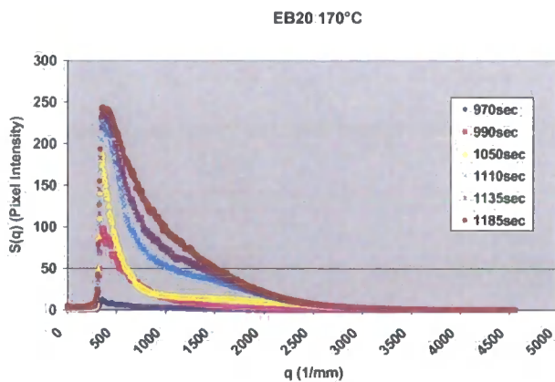
Graph 5.4.3.2 S(q) versus q for EB20 cured at 170^{\circ}\text{C} . This scattering profile shows two spinodal peaks. A primary spinodal peak begins to form after 990 seconds at low q , this develops and shifts to lower q . At 1110 seconds into the cure a second spinodal peak forms at a q value of 1500\text{ mm}^{-1} .
