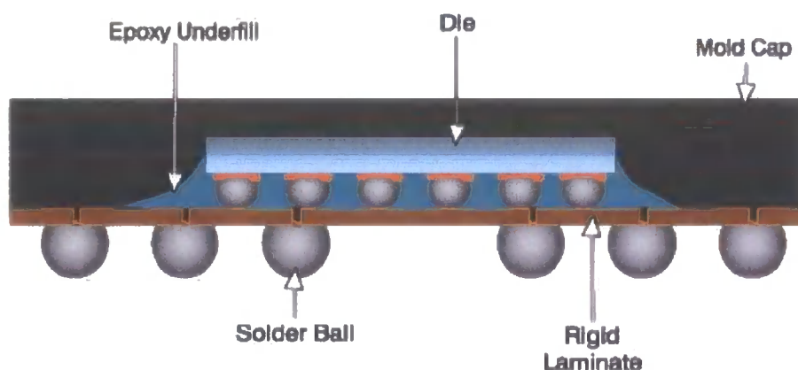
Figure 1.1.1.4 Cross section of a flipchip IC showing the epoxy underfill material.
