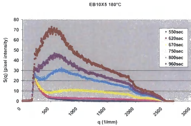
Graph 6.4.1.2 This shows the S(q) versus q plots for EB10X5 cured at 180^\circ\text{C} . This shows the formation of a single spinodal peak that shifts to lower q as the cure progresses.
