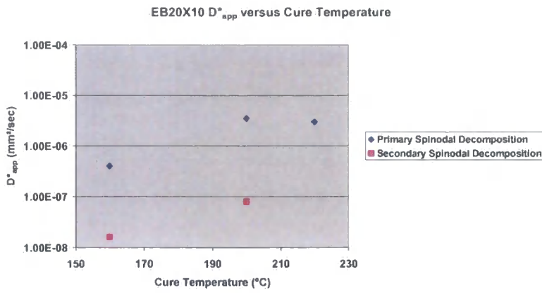
Graph 6.4.7.8 D^*_{app} versus isothermal cure temperature for both primary and secondary phase separations in EB20X10.
