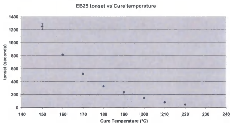
Graph 5.4.4.13 Time to onset of phase separation versus cure temperature for EB25.
