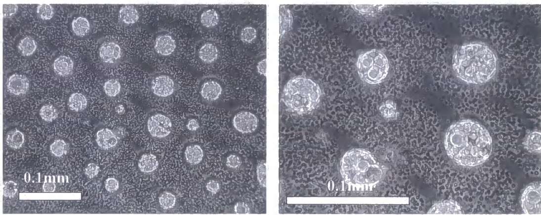
Figure 5.4.3.2 Optical micrographs of EB20 cured at 170°C. This morphology shows large discontinuous particles inside of which are smaller particles from a secondary phase separation. The continuous phase also has small-scale dispersed particles resulting from a secondary phase separation. This is likely to be the result of primary and secondary spinodal decompositions followed by percolation to cluster transformations.
