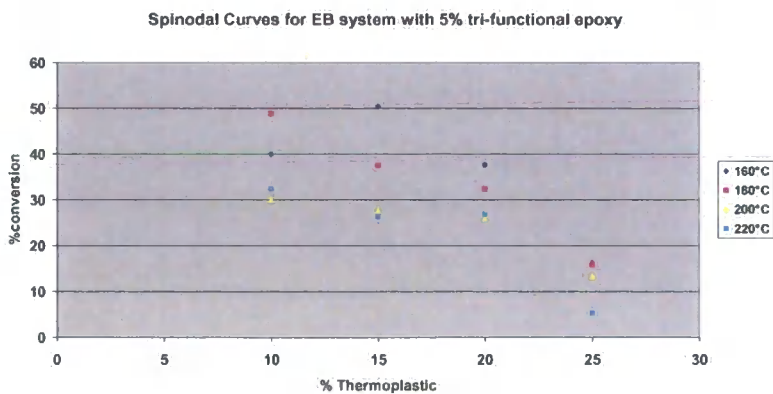
Graph 6.5.18 Phase diagram for EB system with 5% tri-functional epoxy resin. MYO510
