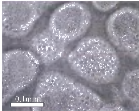
Figure 5.4.4.6 Optical micrograph of EB25 cured at 200°C. This shows a large scale two phase morphology that has formed from a percolation to cluster transformation. Both the phases contain sub-included particles as a result of secondary phase separation.
