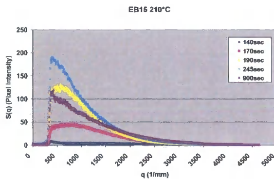
Graph 5.4.2.7 S(q) versus q for EB15 cured at 210°C. This scattering profile shows a broad spinodal peak that shifts to low q as the cure reaction progresses
