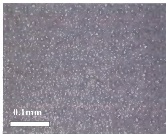
Figure 5.4.3.6 Optical micrograph of EB20 cured at 210°C. This shows a small scale particulate morphology that has formed from primary and secondary percolation to cluster transformation followed by complete dissolution of the primary structure.
