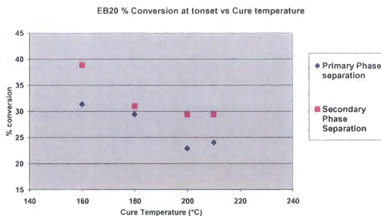
Graph 5.4.3.14 Graph showing the % conversion at the onset of phase separation for different isothermal cure temperatures for EB20. This shows falling % conversion at phase separation with increasing temperature for both primary and secondary spinodal peaks suggesting LCST behaviour.
