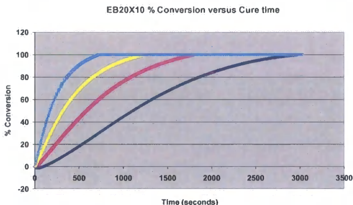
Graph 6.4.7.4 % Conversion versus cure time at different isothermal cure temperatures for EB20X10
