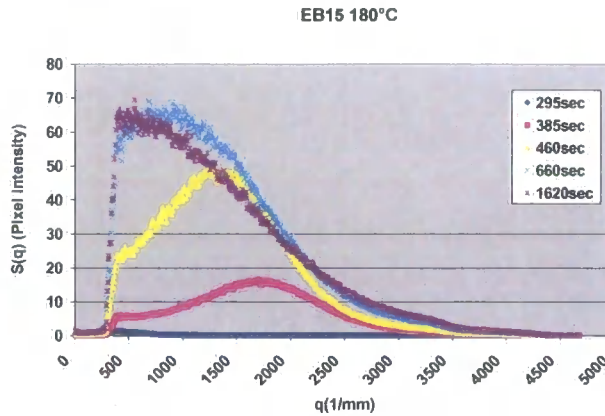
Graph 5.4.2.4 S(q) versus q for EB15 cured at 180^{\circ}\text{C} . This scattering profile shows a broad spinodal peak that shifts to low q as the cure reaction progresses.
