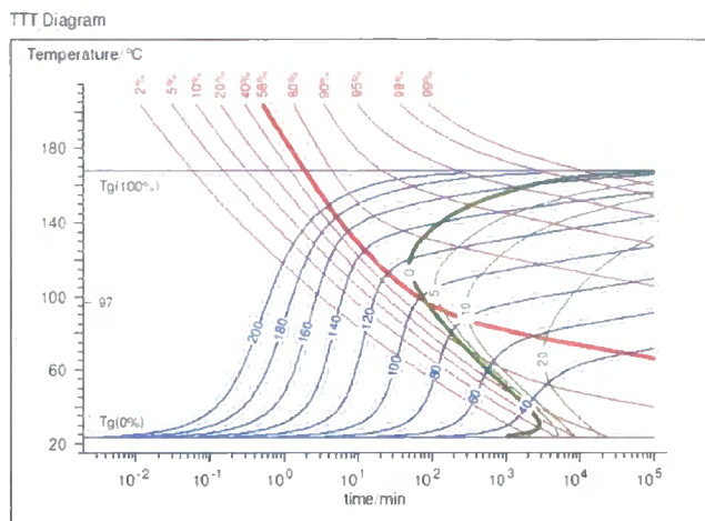
TTT diagram of an Epoxy Thermoset
