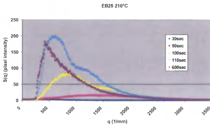
Graph 5.4.4.7 S(q) versus q for EB25 cured at 210°C. This scattering profile shows two spinodal peaks. A primary spinodal peak begins to form after 90 seconds at low q , this develops and shifts to lower q as the cure progresses. After 100 seconds into the cure a second spinodal peak forms at a q value of 1700 \text{mm}^{-1} , this peak also shifts to lower q as the cure progresses.
