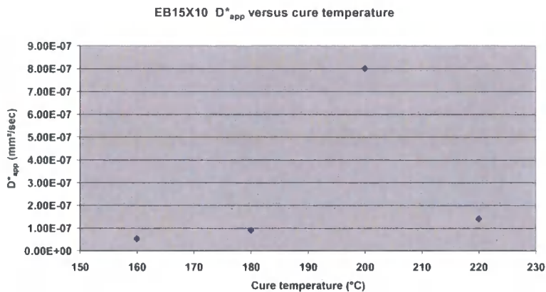
Graph 6.4.6.10 D^*_{app} versus isothermal cure temperature for EB15X10.
