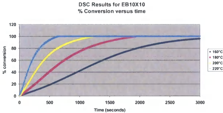
Graph 6.4.5.6 % Conversion versus cure time for different isothermal cure temperatures for EB10X10.
