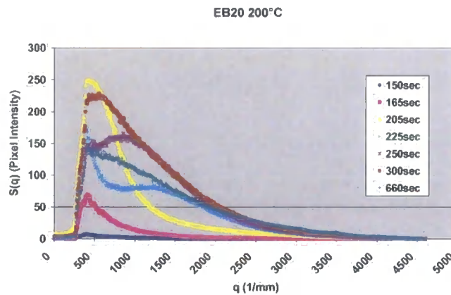
Graph 5.4.3.5 S(q) versus q for EB20 cured at 200°C. This scattering profile shows two spinodal peaks. A primary spinodal peak begins to form after 165 seconds at low q , this develops and shifts to lower q . After 255 seconds into the cure a second spinodal peak forms at a q value of 1400 \text{mm}^{-1} , this peak shifts to lower q as the cure progresses
