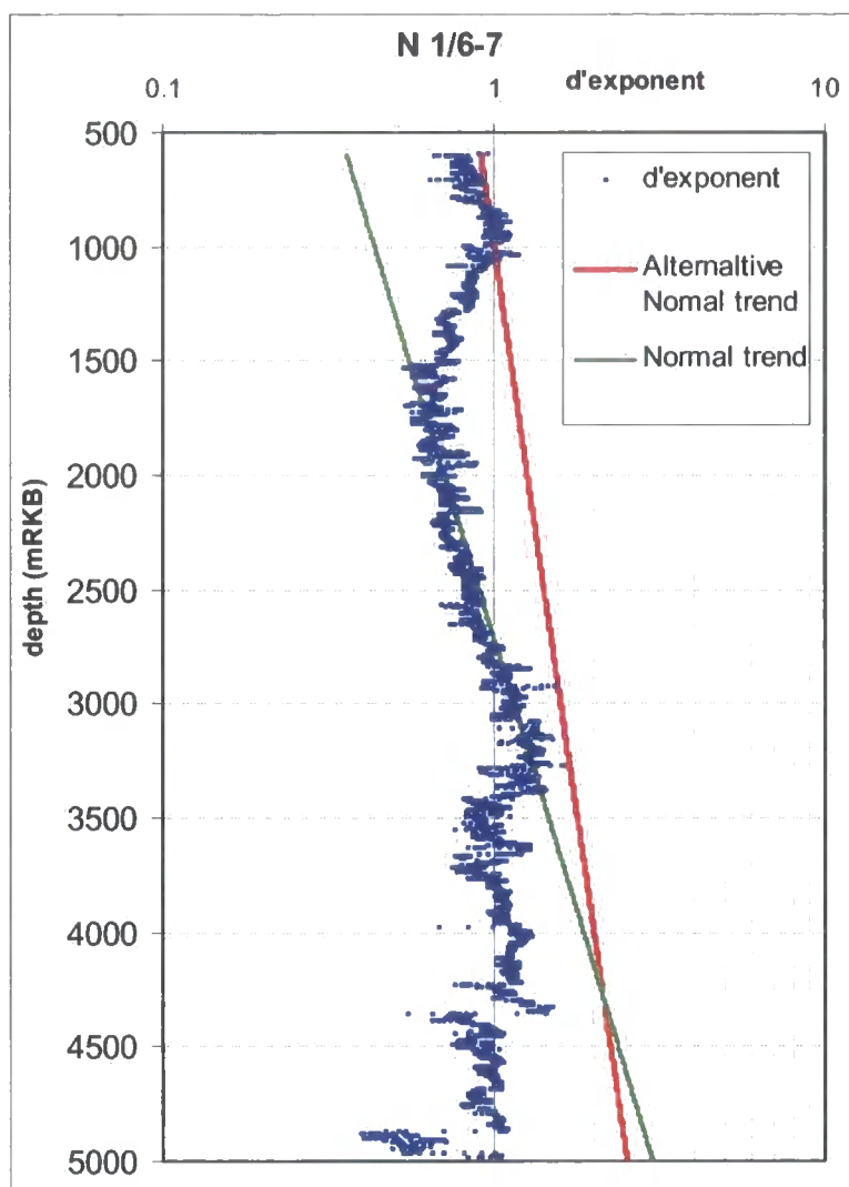
Figure 3.1 The corrected d'exponent plotted versus depth with a normal trend line overlaid in green. Normally new trend lines will be added paralleling the green line each time a new bit is put on the drill string. The new line will represent the actual MW. An alternative trend line is suggested in red. That trend line will also result in a reasonable calculated pore pressure at the target of interest (i.e. 4200 to 4800 m).
