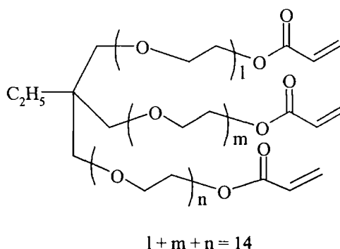
Figure 1.29 Trimethylolpropane ethoxylate triacrylate branched cross-linker
