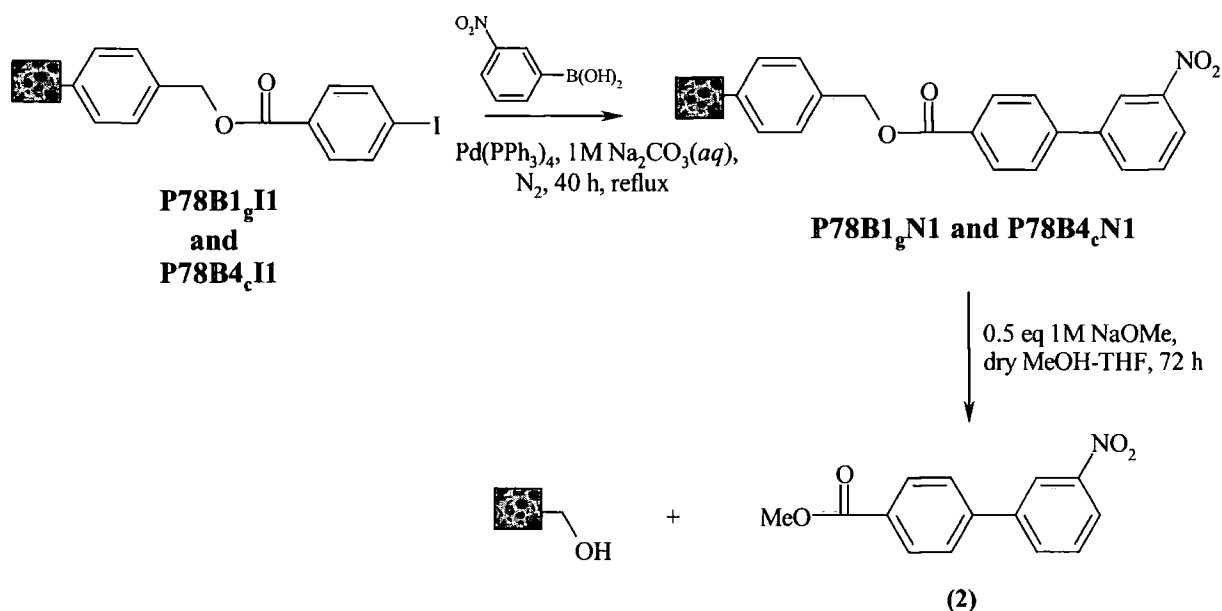
Figure 3.13 PolyHIPE-supported synthesis of 3-nitro-biphenyl-4'-carboxylic acid methyl ester
