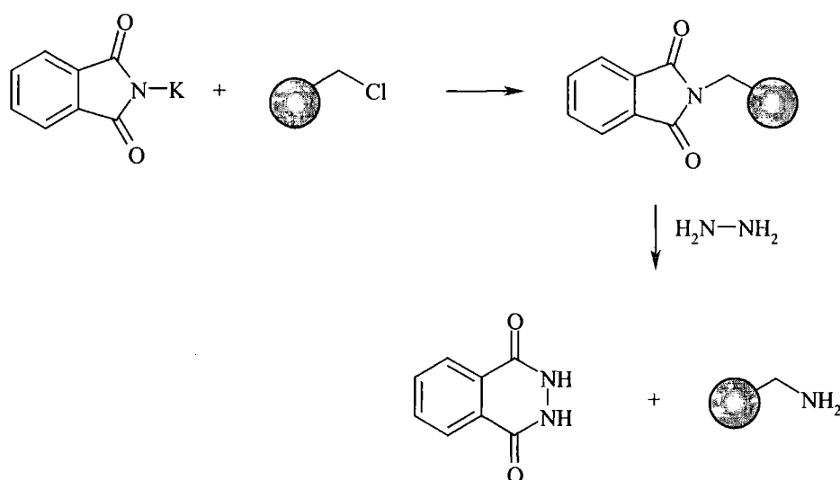
Figure 2.1 Preparation of aminomethyl resin via the Gabriel synthesis
