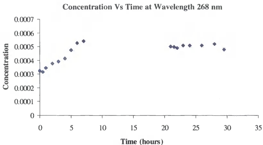
Figure 3.28 Graph of concentration of cesium carboxylate salt against flow-through time
