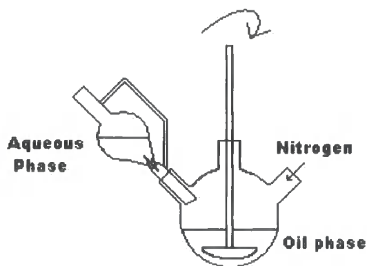
Figure 2.2 Schematic of the apparatus used in HIPE Synthesis
