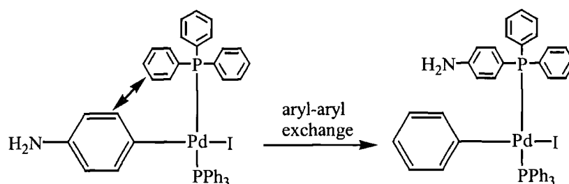
Figure 3.5 An example of aryl migration in Suzuki coupling reactions
