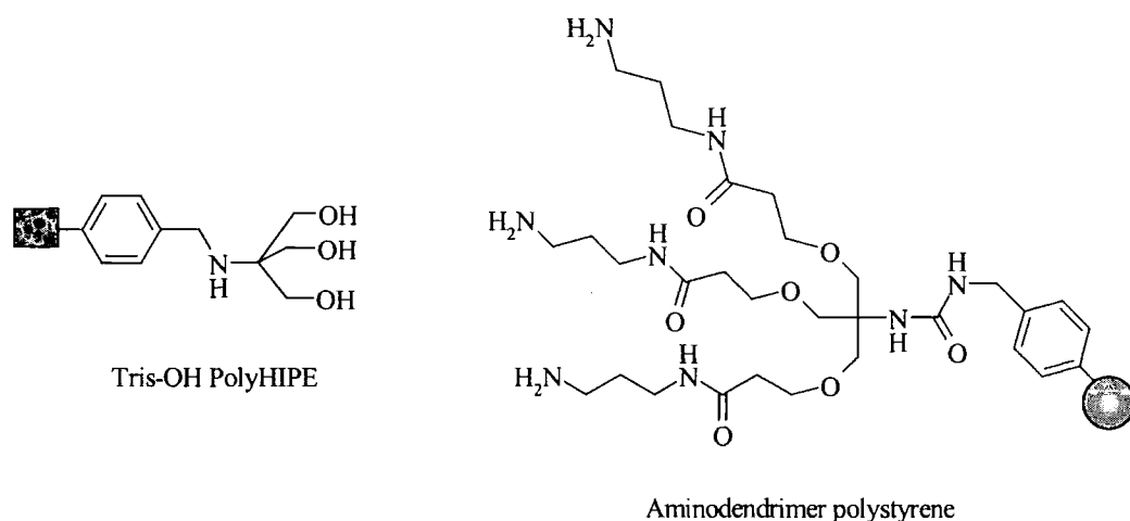
Figure 4.3 Highly loaded PolyHIPE and bead supports
