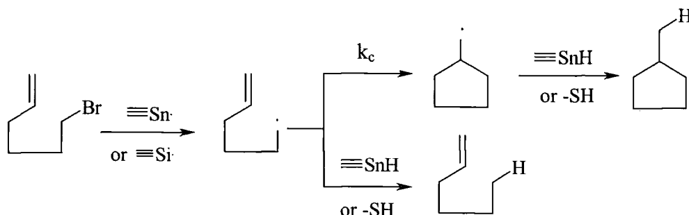
Figure 1.45 Radical-reduction mechanism of 6-bromohex-1-ene
