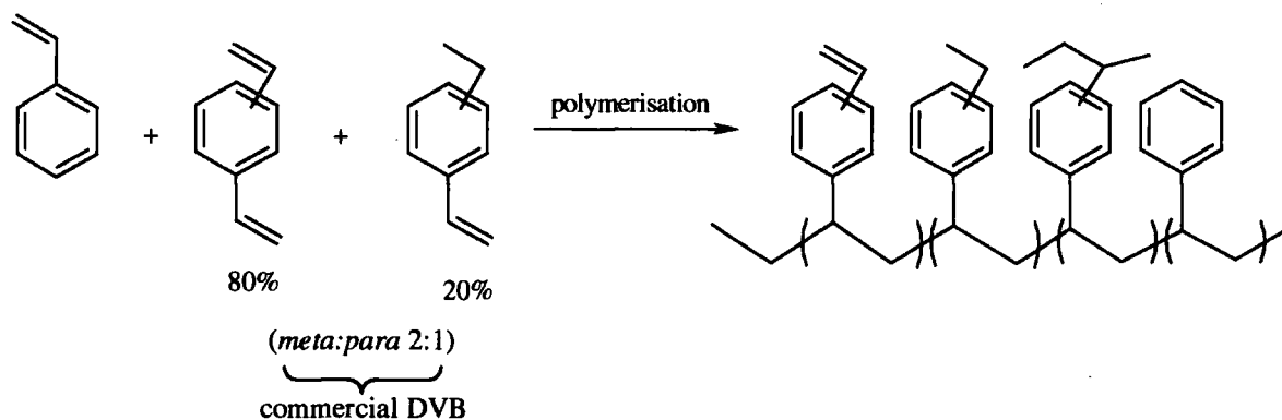
Figure 1.40 Unreacted vinyl groups in poly(styrene/DVB) PolyHIPEs
