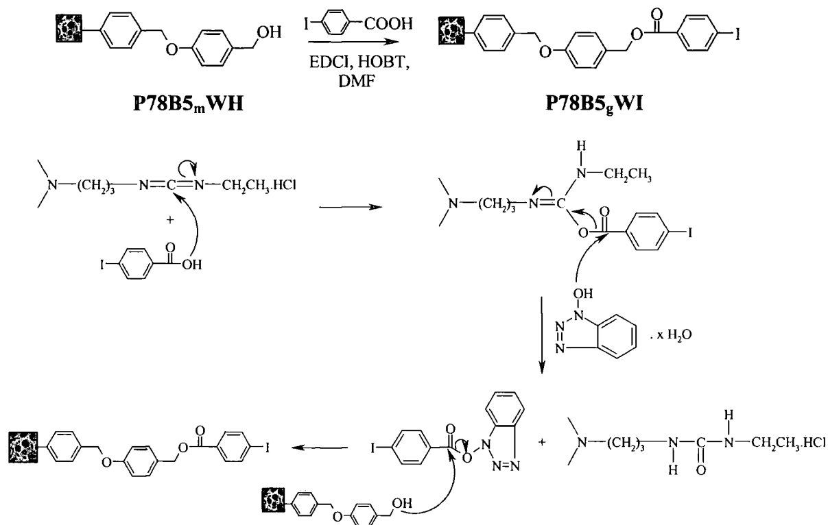
Figure 4.8 EDCI/HOBT-mediated coupling of Wang PolyHIPE and 4-iodobenzoic acid
