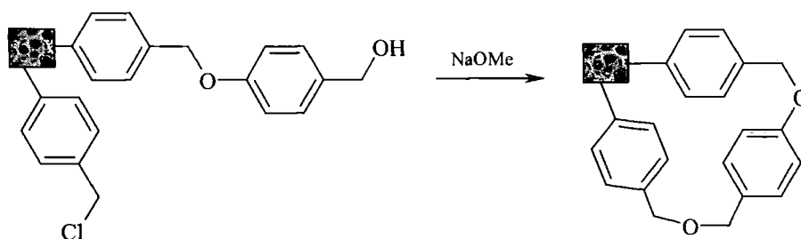
Figure 4.9 Cross-linking effect in highly loaded chloromethyl PolyHIPE
