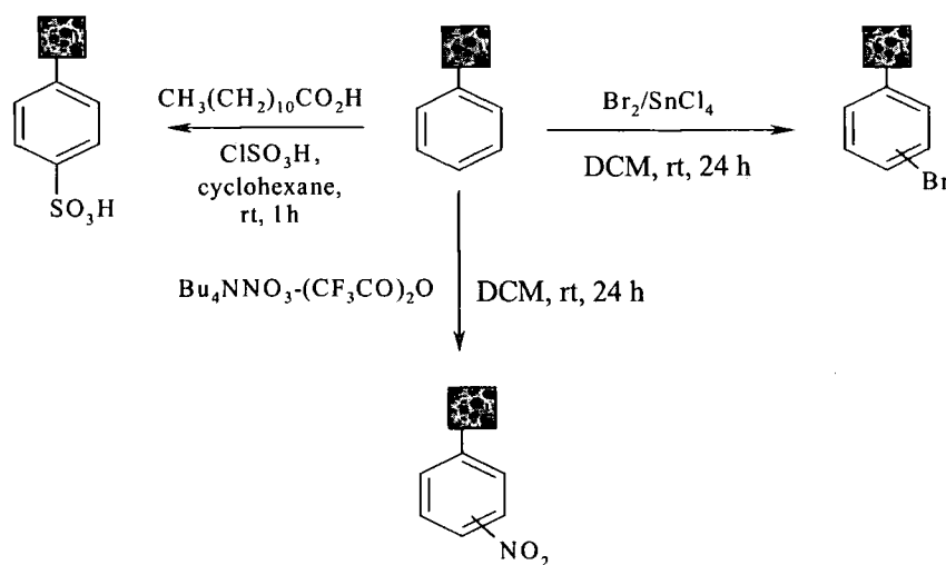
Figure 1.39 Sulfonation, bromination and nitration of poly(styrene/DVB) PolyHIPE
