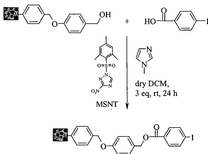
Figure 4.11 Reaction of 4-iodobenzoic acid with Wang linker using MSNT-mediated coupling
