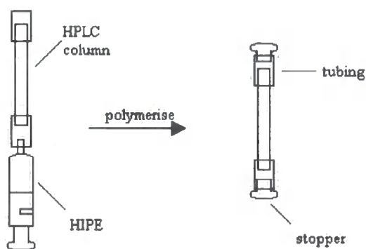
Figure 3.23 Preparation of VBC/DVB PolyHIPE inside a stainless steel HPLC column
