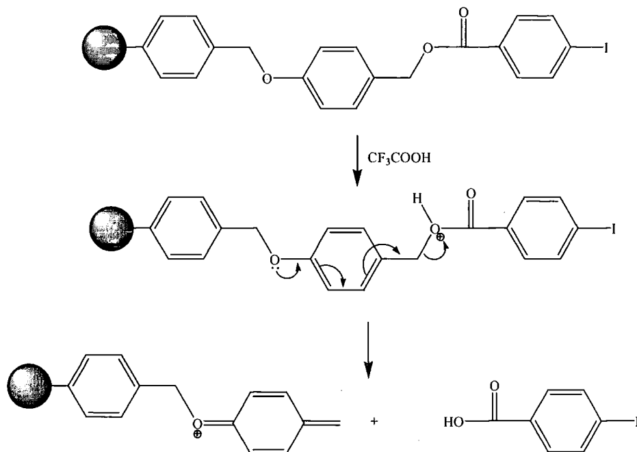
Figure 4.2 Acidolytic cleavage of TFA
