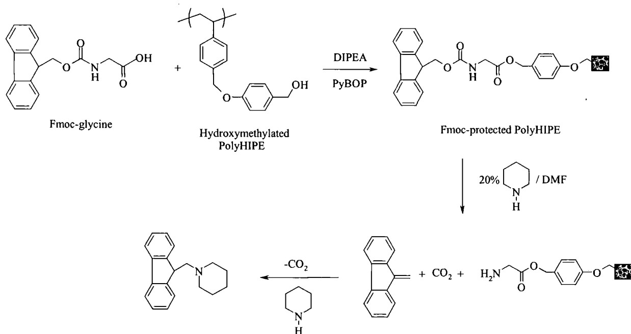
Figure 4.7 Synthesis involved in Fmoc analysis
