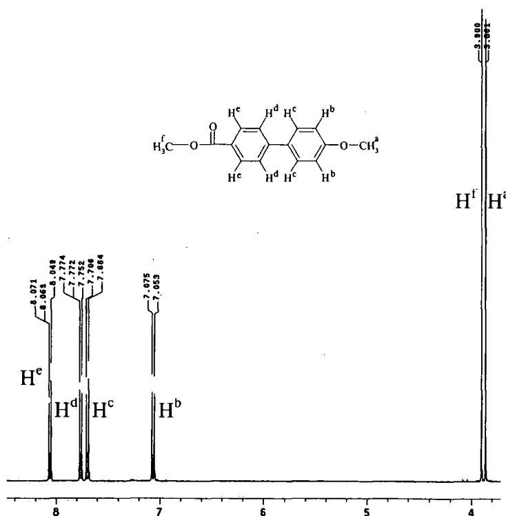
Figure 3.22 ^1\text{H} NMR spectrum of crude product (1) obtained from the bead-supported flow-through Suzuki synthesis
