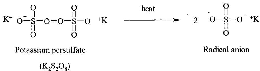
Figure 1.37 Potassium persulfate radical addition initiator
