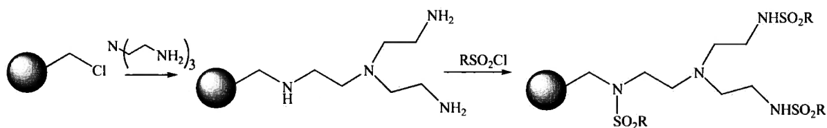
Figure 1.23 Scavenging of trans - \beta -styrene sulfonyl chloride with polymer-supported tris(2-aminoethyl)amine
