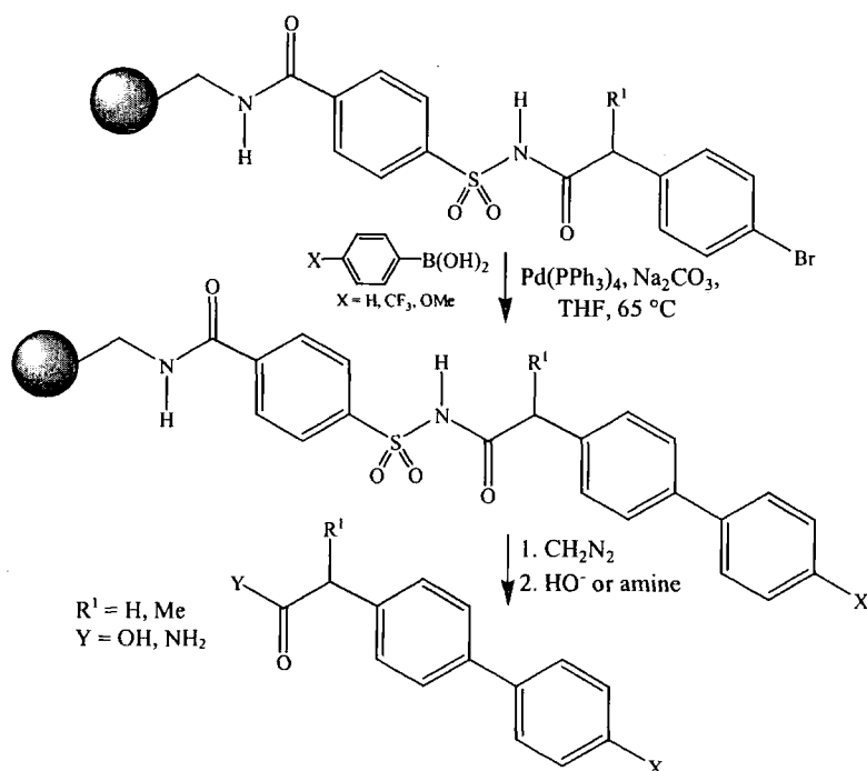
Figure 1.13 Use of aminomethylated resin in the Suzuki coupling of an acylsulfonamide
