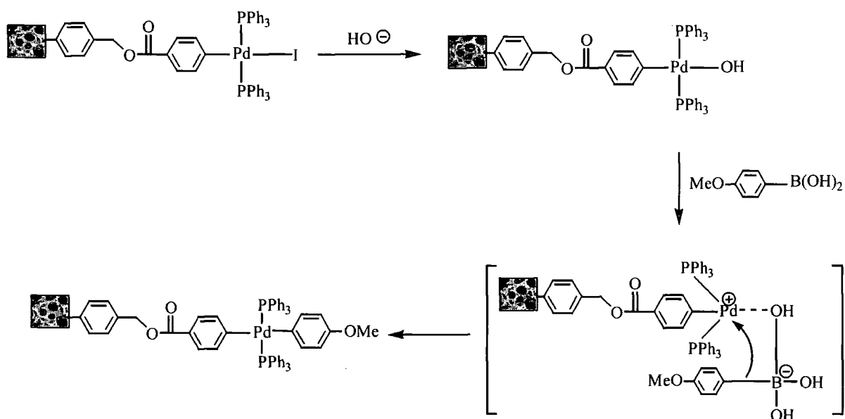
Figure 3.2 Transfer of the aryl group during transmetalation
