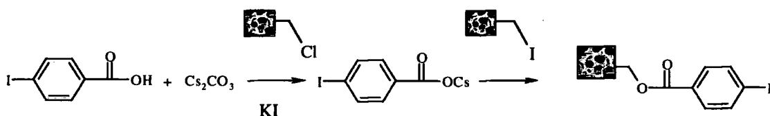
Figure 3.25 Reaction of cesium carboxylate salt with chloromethyl groups
