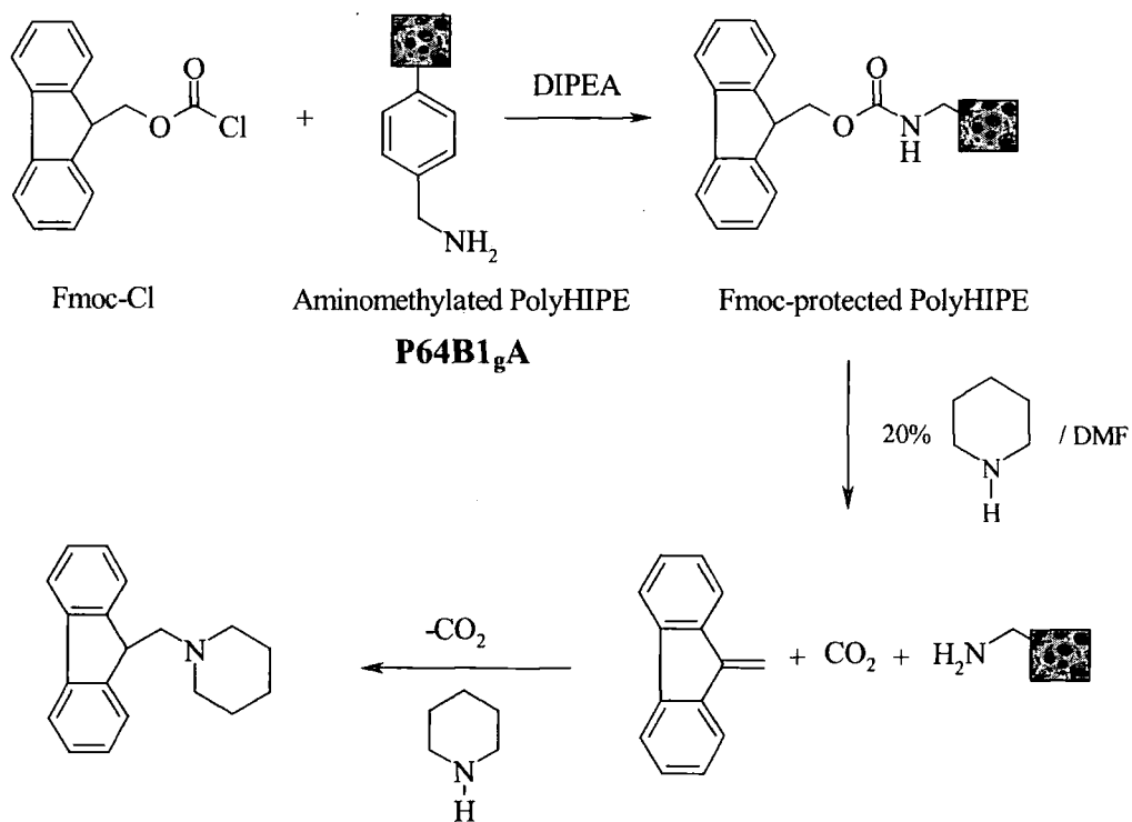
Figure 2.11 Synthesis involved in Fmoc analysis
