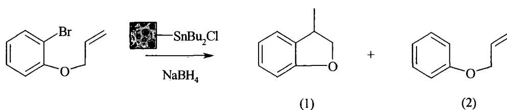
Figure 1.44 Radical cyclisation reaction of 1-bromo-2(prop-2-enyloxy)benzene
