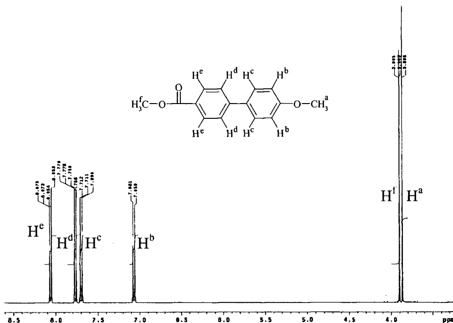
Figure 3.11 ^1\text{H} NMR spectrum of 4-methoxy-biphenyl-4'-carboxylic acid methyl ester ( 1 )
