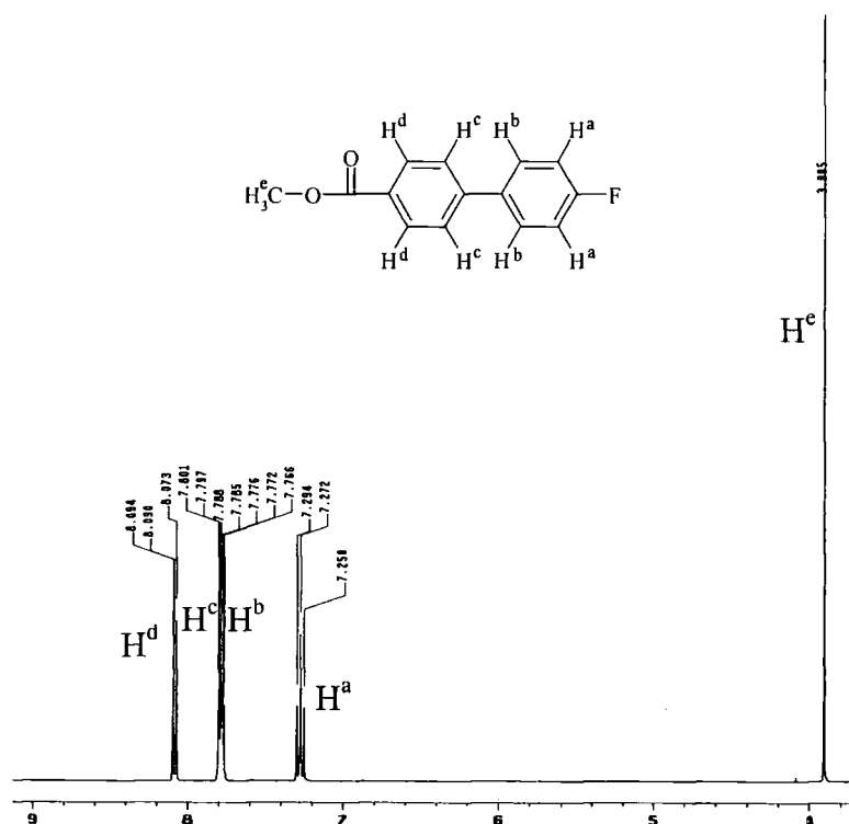
Figure 3.17 1 H NMR spectrum of 4-fluoro-biphenyl-4'-carboxylic acid methyl ester
