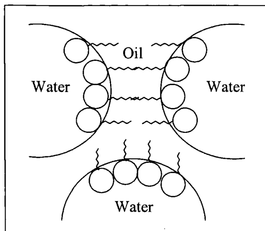
Figure 1.35 Schematic of non-ionic surfactant molecules at water/oil interface in a HIPE
