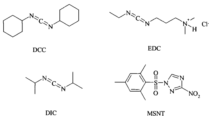
Figure 4.1 Carbodiimides and MSNT reagent used in solid phase synthesis
