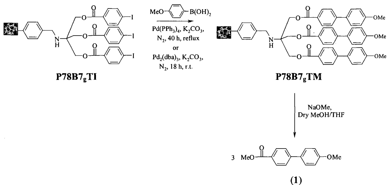
Figure 4.20 Solid-phase Suzuki coupling on tris-I functionalised PolyHIPE
