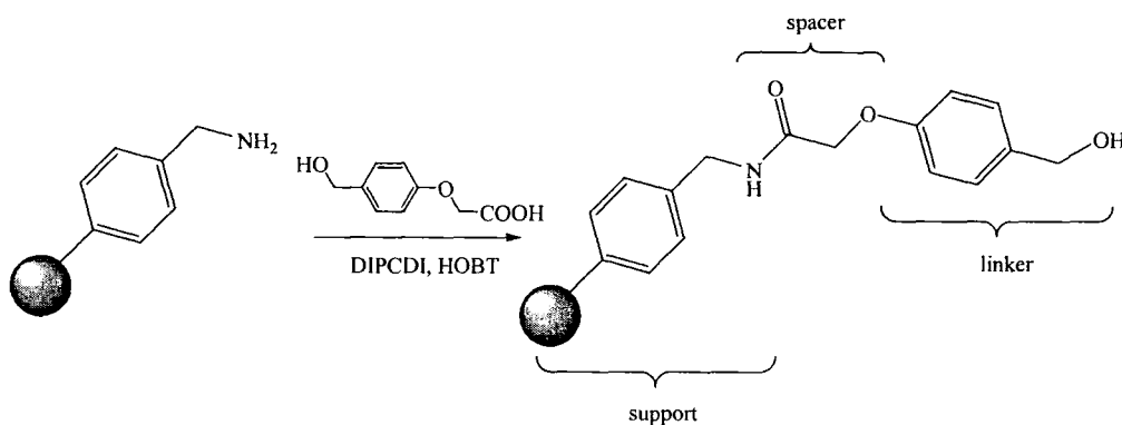
Figure 1.11 Coupling of HMPA linker onto aminomethyl resin
