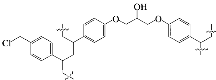
Figure 1.28 Structure of novel regio-reactive resins developed for use in SPOS
