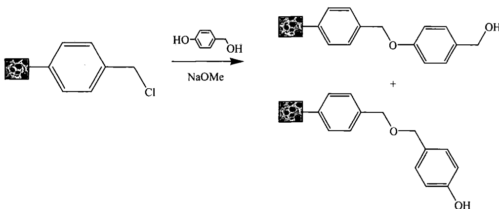
Figure 4.10 Mixture of products formed during HMP functionalisations
