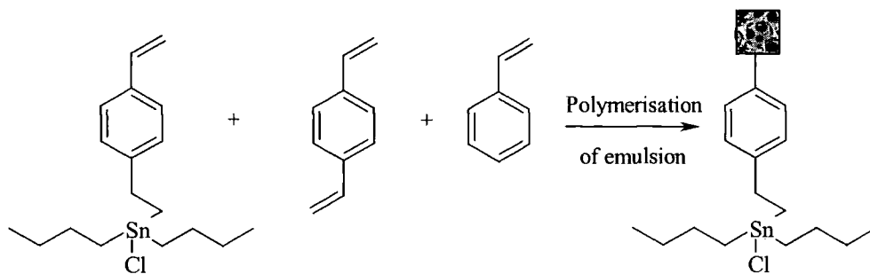
Figure 1.43 Preparation of the PolyHIPE-supported catalyst
