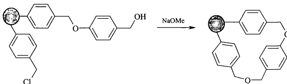
Figure 4.6 Displacement of chlorine by polymer-bound phenolate anions
