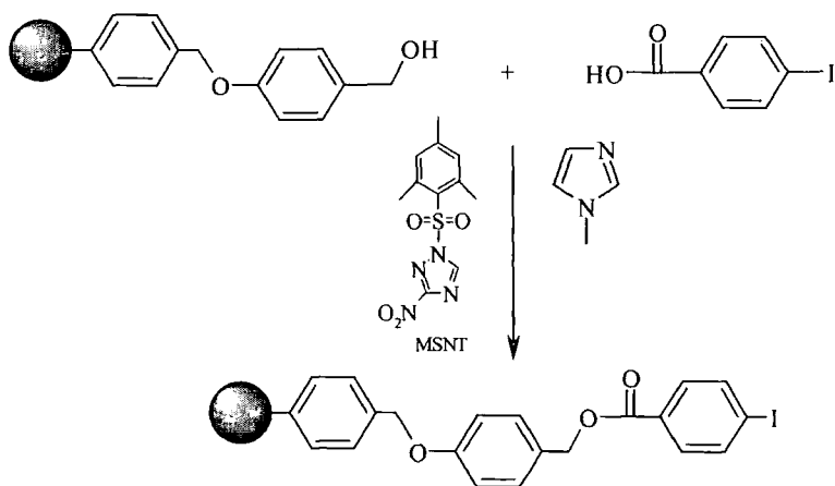
Figure 1.10 Synthesis of Wang-immobilised carboxylic acid
