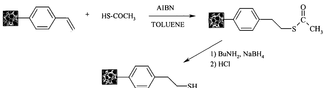
Figure 1.47 Preparation of PolyHIPE-supported thiol
