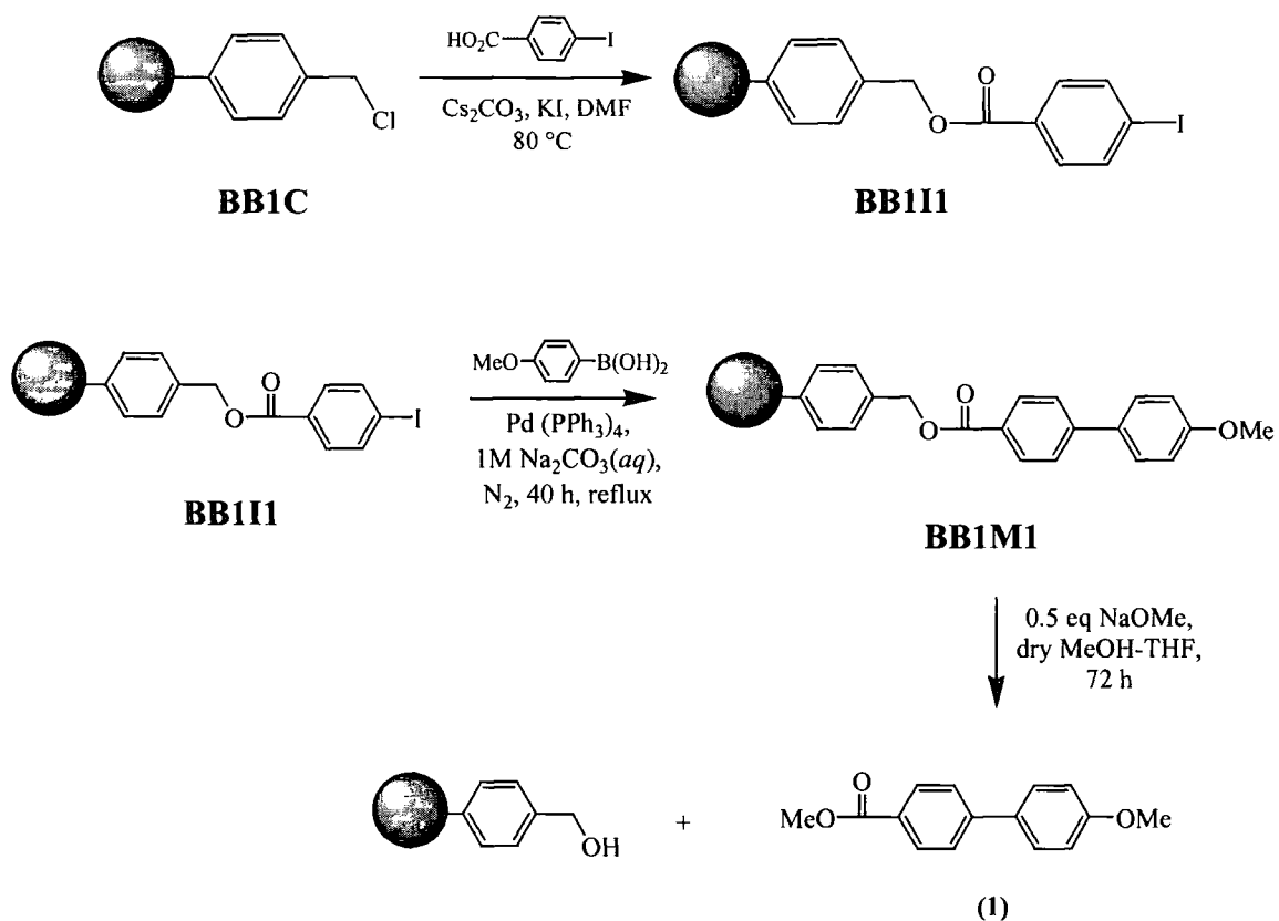
Figure 3.19 Bead-supported synthesis of 4-methoxy-biphenyl-4'-carboxylic acid methyl ester
