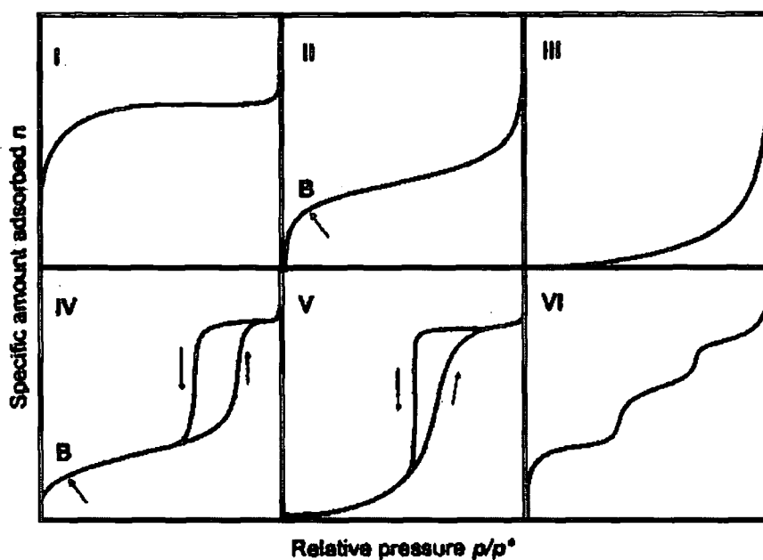
Figure 2.5 The six main types of gas physisorption isotherms, according to the IUPAC classification
