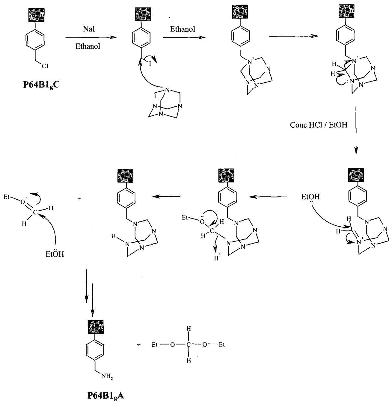
Figure 2.10 Synthesis of P64B1 g A and mechanism of formaldehyde diethylacetal formation
