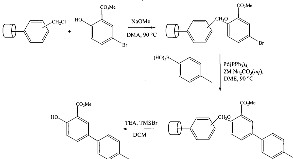
Figure 1.20 Use of VBC-based polymer discs in the solid phase Suzuki coupling reaction
