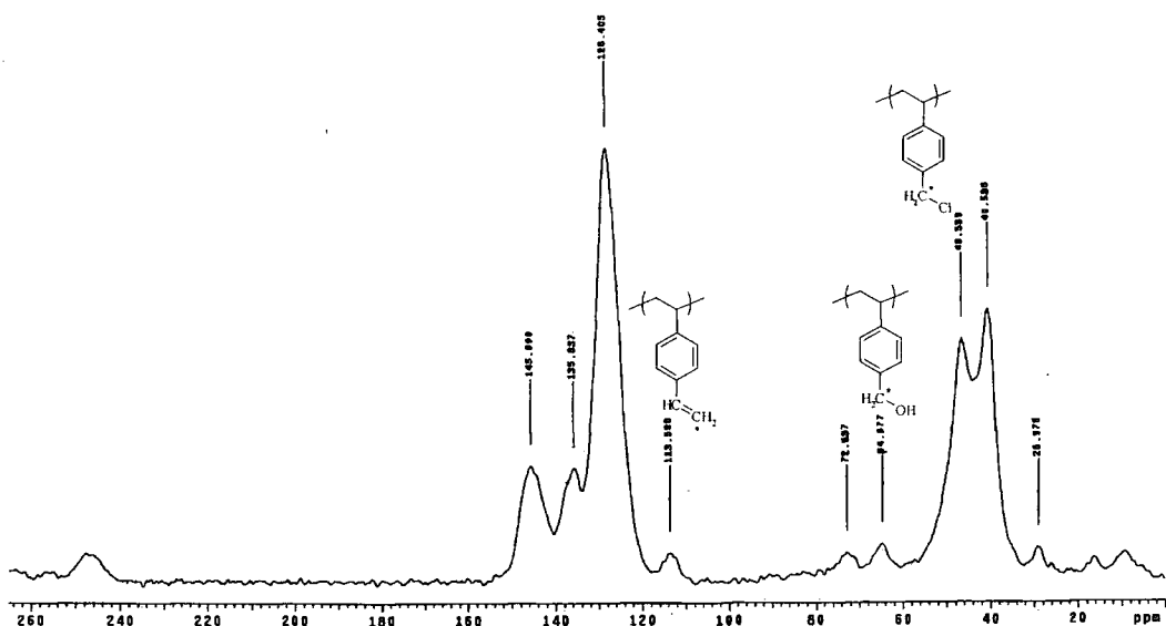
Figure 2.8 Solid state ^{13}\text{C} NMR spectrum of P64B1C
