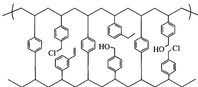
Figure 2.7 Structure of hydrolysed PolyHIPE
