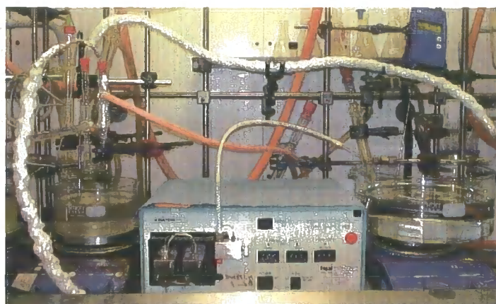
Figure 3.29 Apparatus used in the flow-through Suzuki Synthesis
