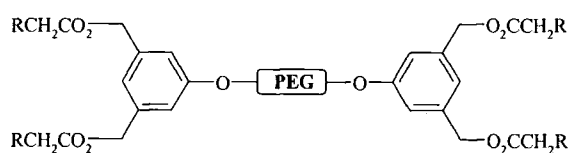
Figure 1.1 Bifunctional PEG-containing benzyl ether dendrons
