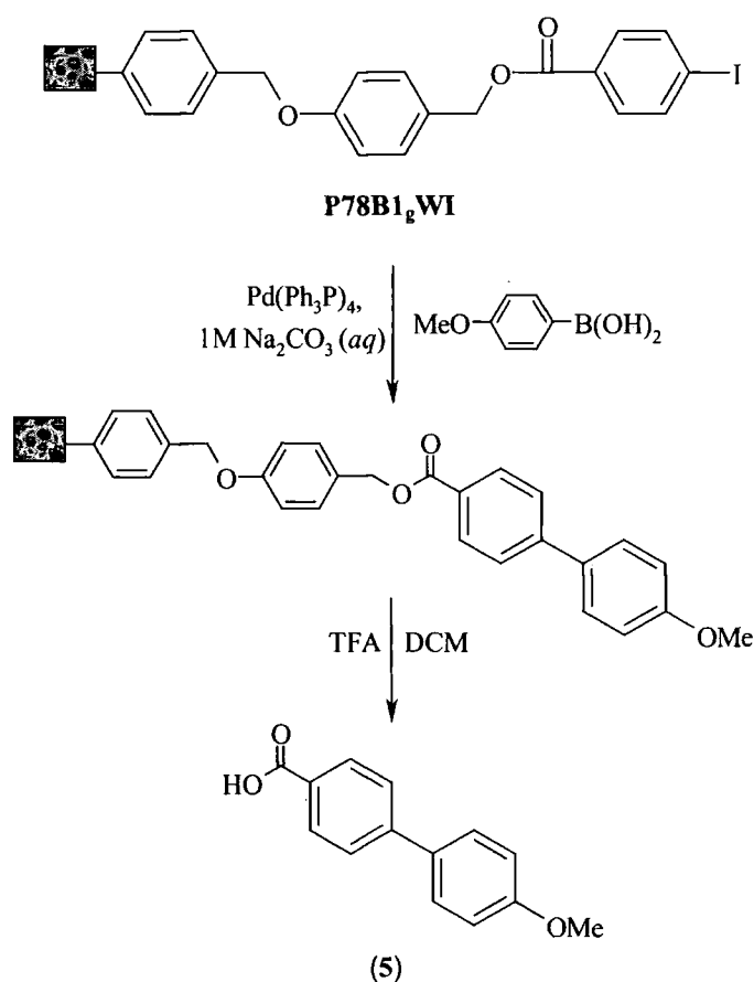
Figure 4.17 Solid-phase Suzuki coupling on Wang-functionalised PolyHIPE
