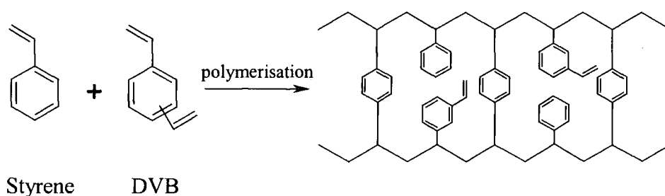
Figure 1.3 Synthesis of poly(styrene-divinylbenzene) copolymer
