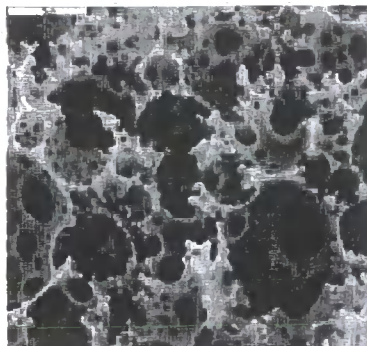
Figure 2.6 Scanning electron micrograph of VBC/DVB PolyHIPE (ratio of VBC/DVB = 63:37; pore volume 90%). Scale bar represents 5 \mu\text{m} 15
