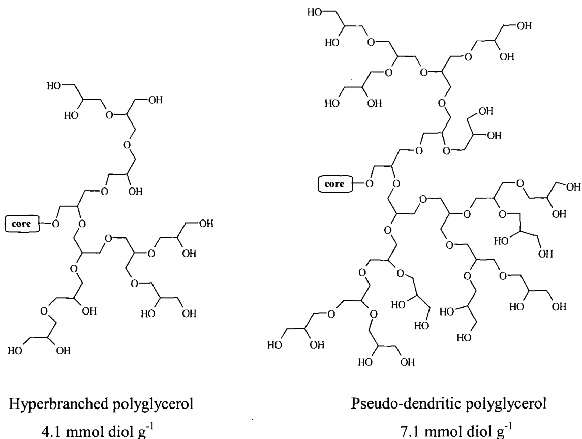
Figure 1.2 Hyperbranched polyglycerol and pseudo dendrimer supports
