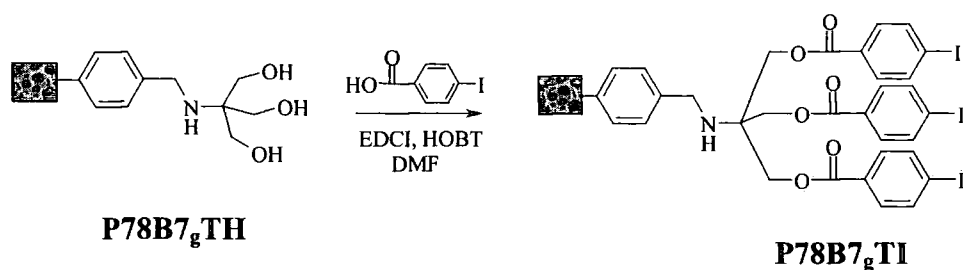
Figure 4.18 Attachment of 4-iodobenzoic acid to trishydroxymethyl PolyHIPE
