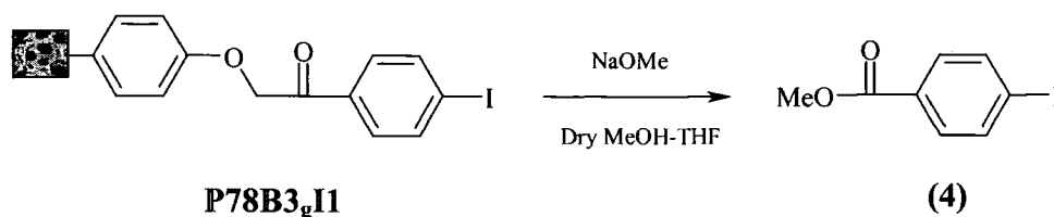
Figure 3.10 Cleavage of PolyHIPE-supported aryl iodide compound
