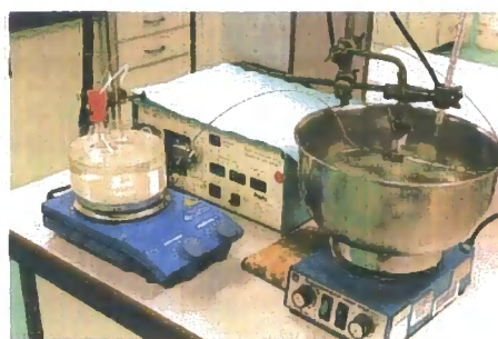
Figure 3.24 Photograph of the original automatic flow-through system developed
