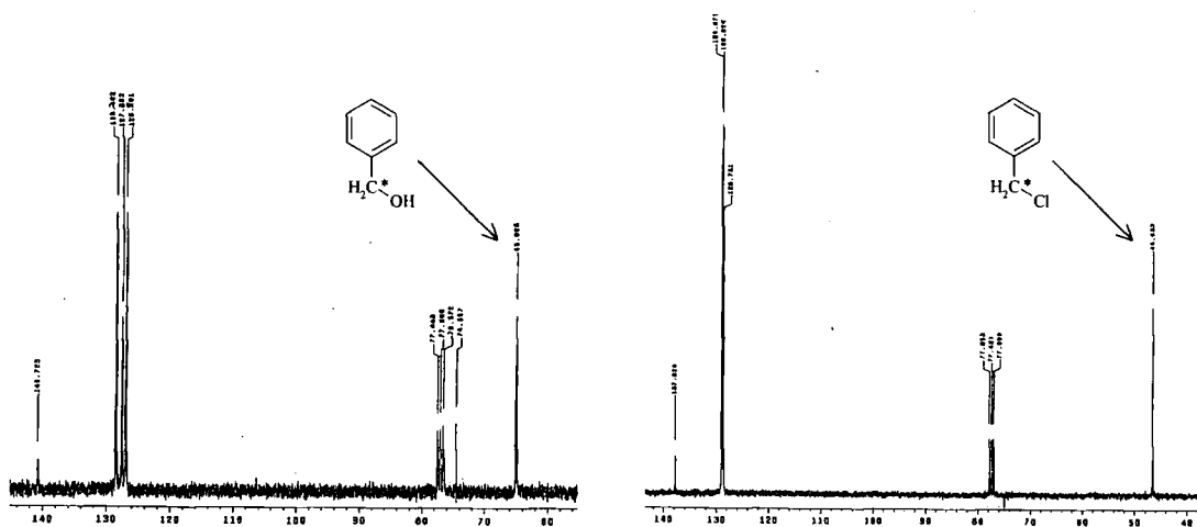
Figure 2.9 Solution state ^{13}\text{C} NMR spectra of benzyl alcohol and benzyl chloride
