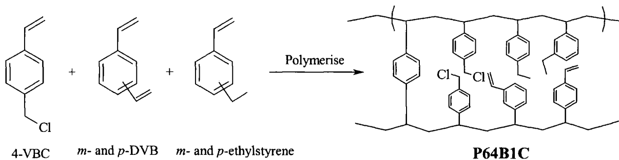
Figure 2.4 Synthesis of poly(VBC/DVB) PolyHIPE
