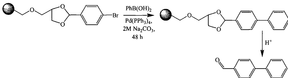
Figure 1.18 Suzuki synthesis of biaryl aldehydes using the Leznoff acetal linker
