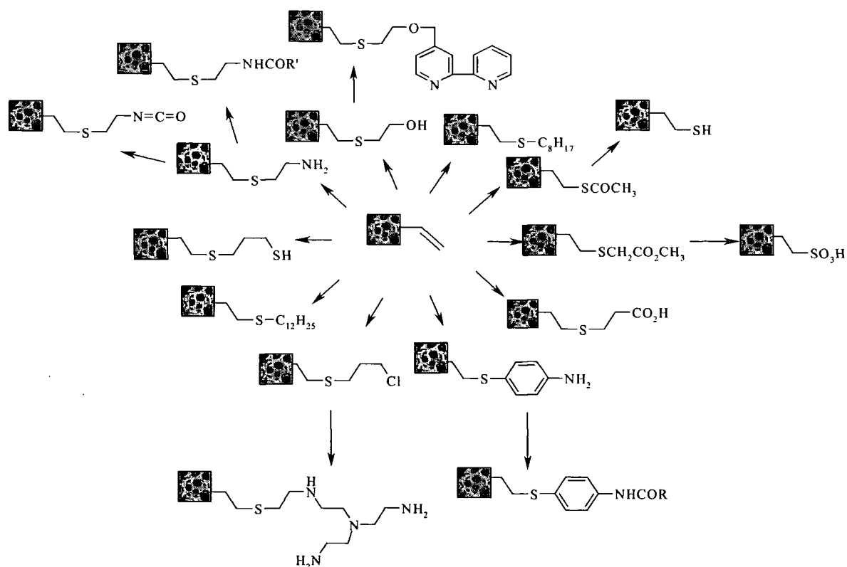
Figure 1.42 Functionalisation of (vinyl)polystyrene PolyHIPE by thiols
