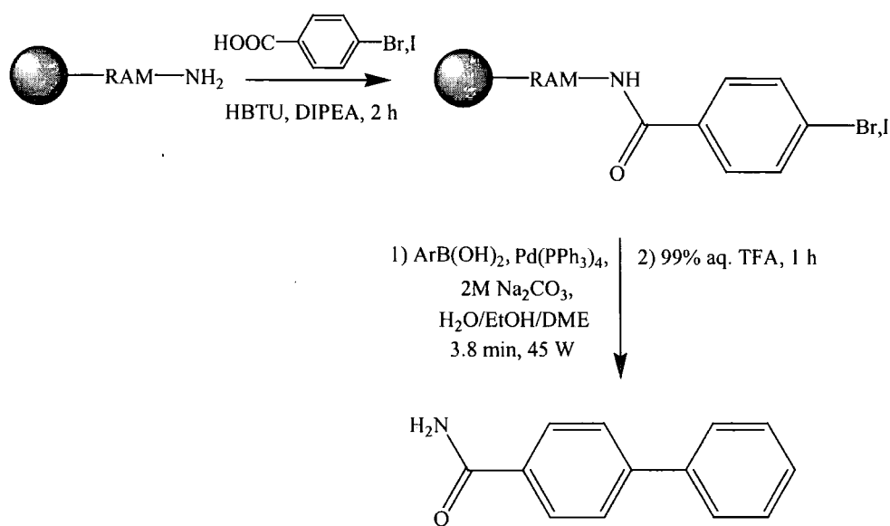
Figure 1.16 Synthesis of amido biaryls via microwave-assisted Suzuki coupling
