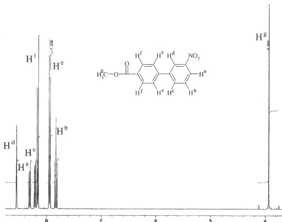
Figure 3.15 1 H NMR spectrum of 3-nitro-biphenyl-4'-carboxylic acid methyl ester
