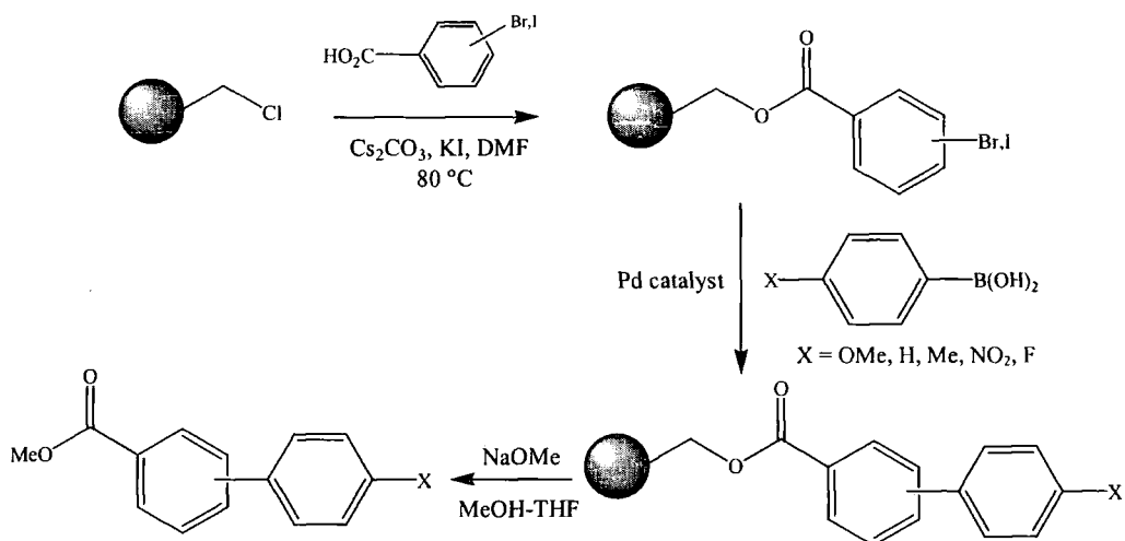
Figure 1.12 Synthesis of biaryls via Suzuki coupling of aryl boronic acids with Merrifield-bound aryl halides
