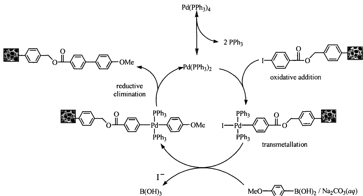
Figure 3.1 The Suzuki cross-coupling catalytic cycle
