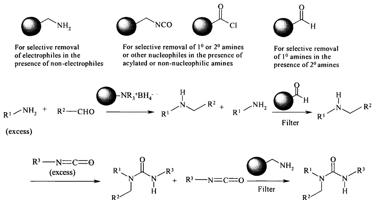
Figure 1.22 Polymer-supported scavenging reagents
