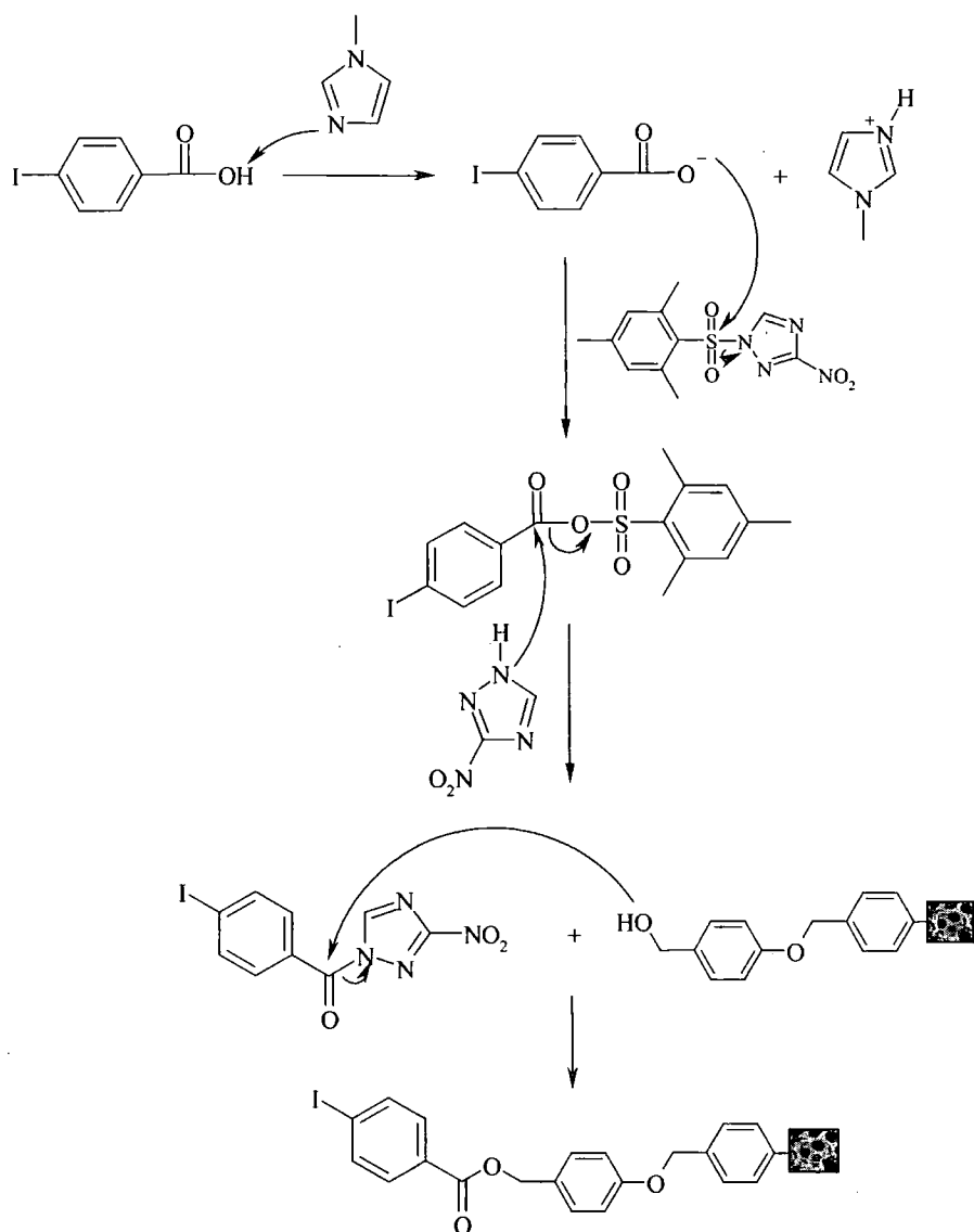
Figure 4.12 Mechanism of MSNT coupling
