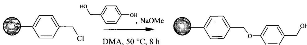
Figure 4.4 Synthesis of Wang Resin
