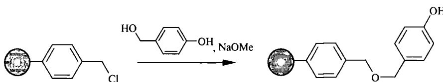
Figure 4.5 Displacement of chlorine by benzyl alcohol anion
