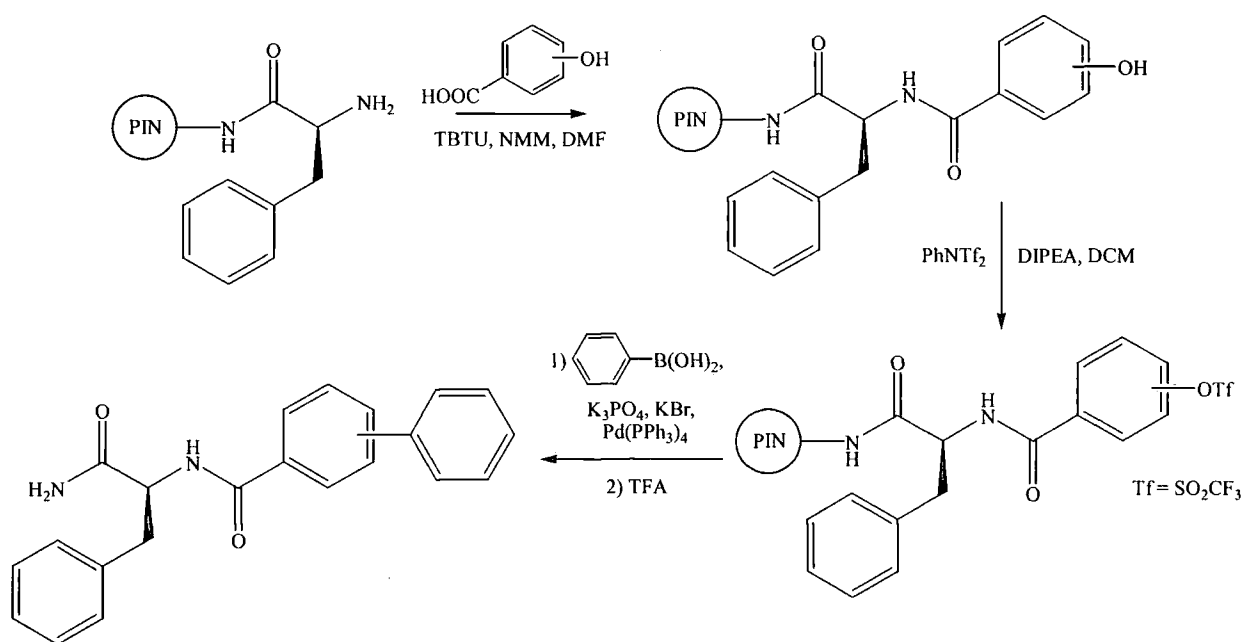
Figure 1.21 Triflation of phenols on Multipin supports and subsequent Suzuki coupling with phenylboronic acid
