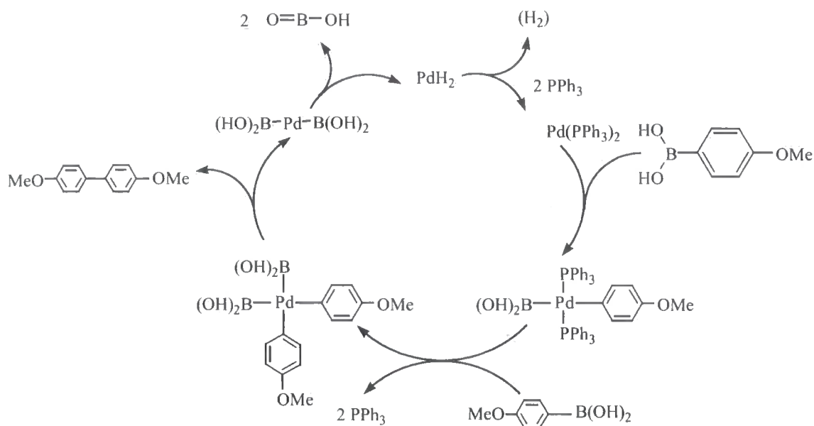
Figure 3.6 Self-coupling of 4-methoxybenzeneboronic acid
