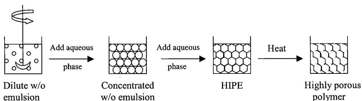
Figure 1.32 Schematic of PolyHIPE preparation
