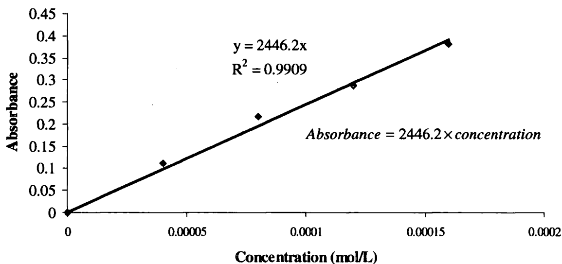
Figure 3.26 Calibration curve of cesium carboxylate salt in solution
