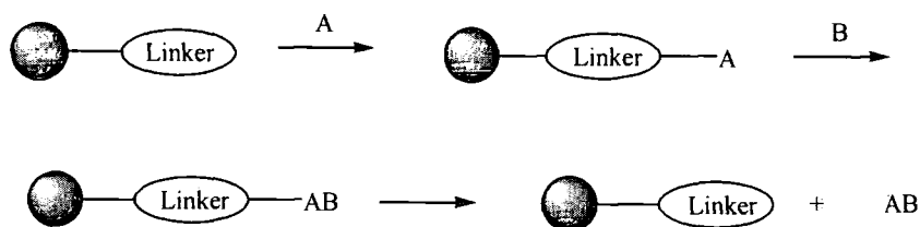
Figure 1.6 Principle of solid phase organic synthesis
