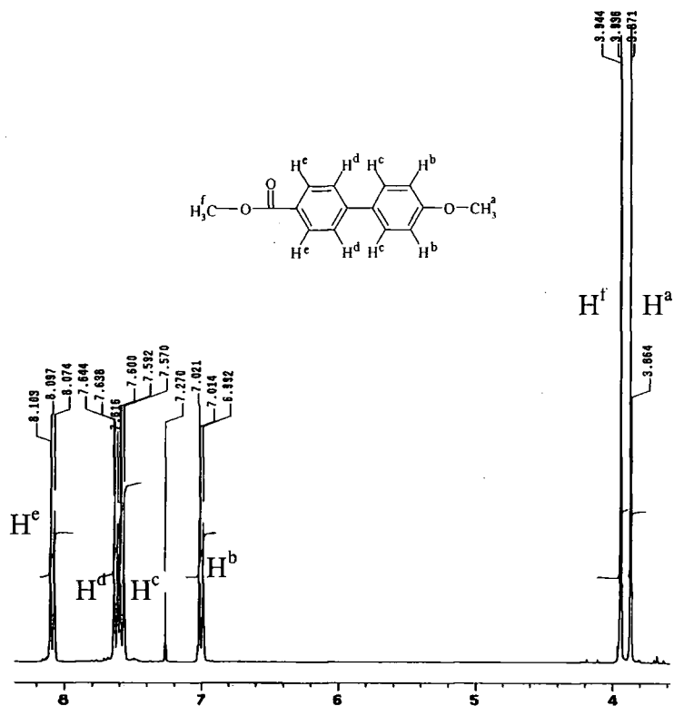
Figure 3.21 1 H NMR spectrum of crude product (1) obtained from the PolyHIPE-supported flow-through Suzuki synthesis
