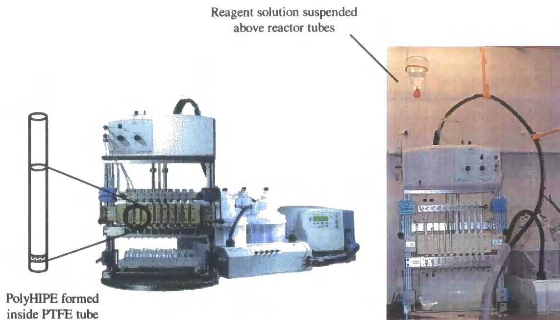
Figure 2.12 Quest apparatus for flow-through functionalisations
