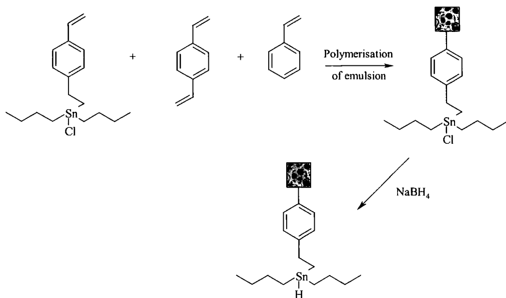
Figure 1.46 Preparation of PolyHIPE-supported organotin hydride
