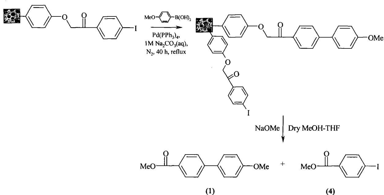
Figure 3.9 Synthesis of 4-iodo-benzoic acid methyl ester by-product
