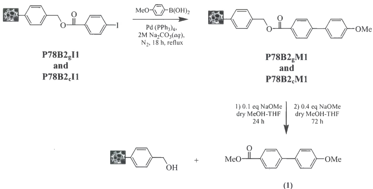
Figure 3.8 PolyHIPE-supported synthesis of 4-methoxy-biphenyl-4'-carboxylic acid methyl ester
