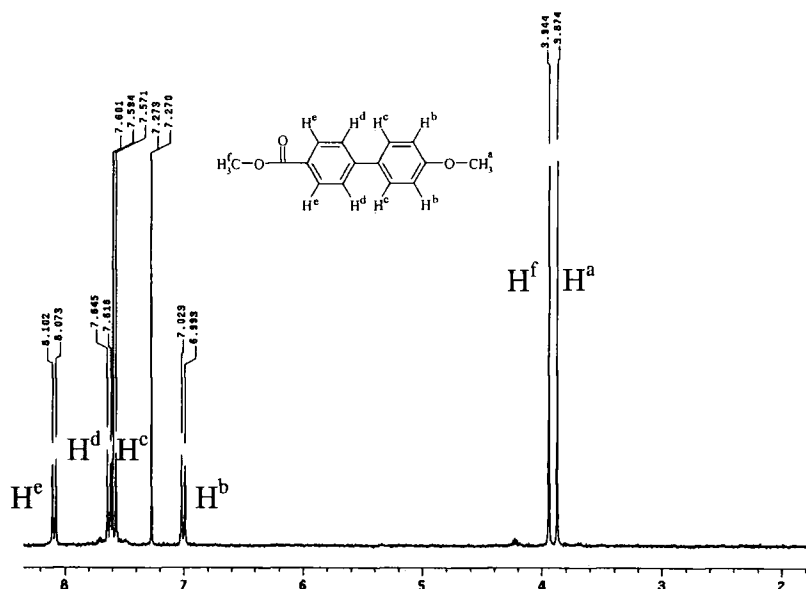
Figure 4.21 ^1\text{H} NMR spectrum of 4-methoxy-biphenyl-4'-carboxylic acid methyl ester (1)
