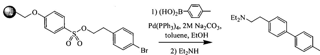
Figure 1.17 Synthesis of biaryl amines utilising arylsulfonate ester linkers in the Suzuki cross-coupling of 4-methylphenyl boronic acid
