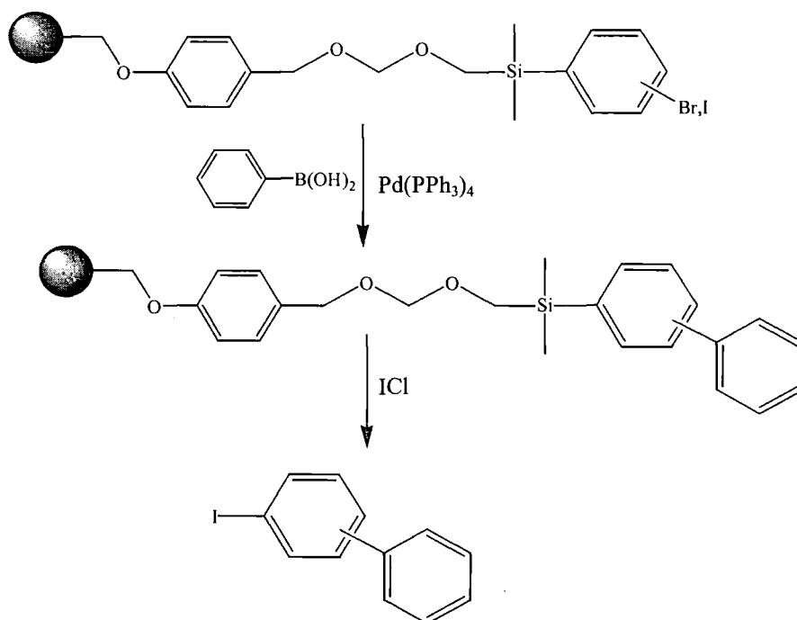
Figure 1.15 Use of Wang-bound haloarylsilane linkers in the coupling of phenylboronic acid
