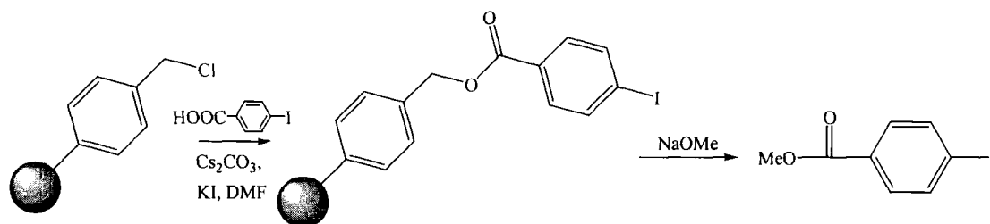
Figure 1.8 Synthesis of methyl ester on Merrifield resin
