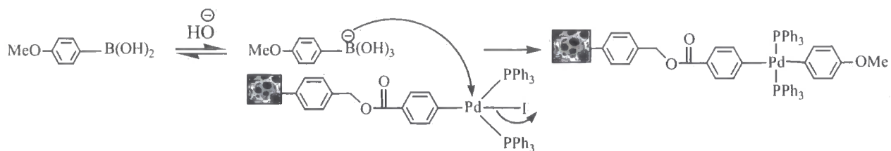
Figure 3.3 Alternative process for aryl group transfer
