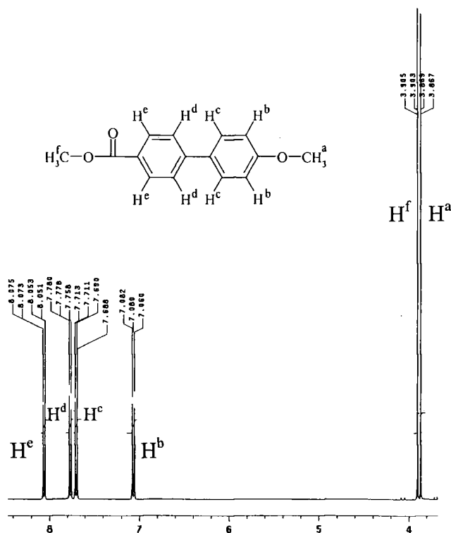
Figure 3.20 ^1\text{H} NMR spectrum of 4-methoxy-biphenyl-4'-carboxylic acid methyl ester ( 1 ) synthesised on beads
