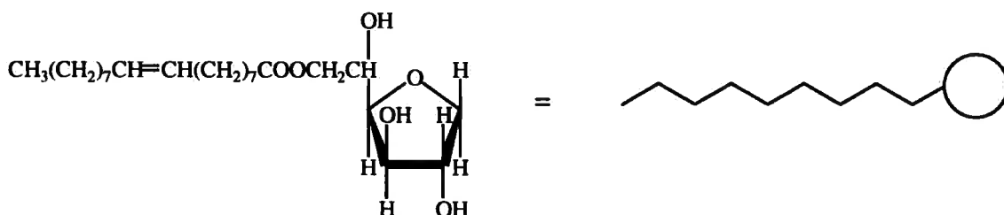
Figure 1.34 Sorbitan monooleate (Span 80)
