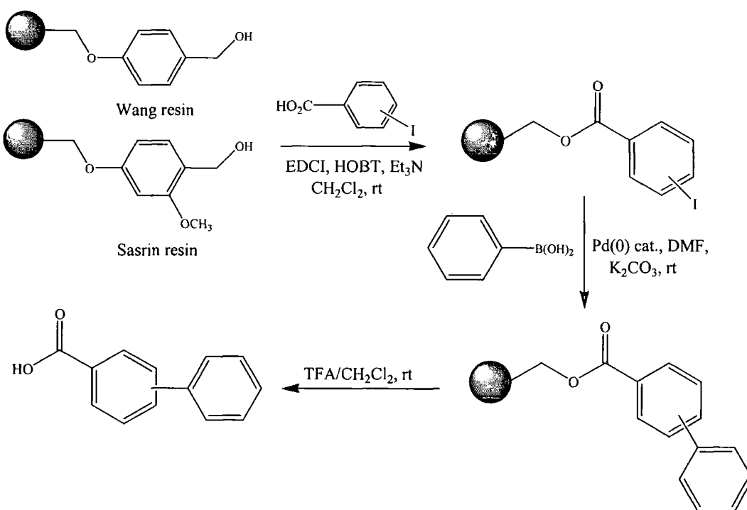
Figure 1.14 Synthesis of biaryl carboxylic acids via the Suzuki coupling of phenylboronic acid with Sasrin and Wang-bound aryl iodide
