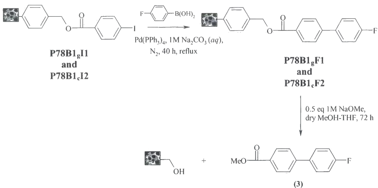
Figure 3.16 PolyHIPE-supported synthesis of 4-fluoro-biphenyl-4'-carboxylic acid methyl ester
