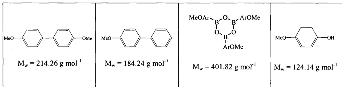
Figure 3.12 Possible by-products from the self-coupling of 4-methoxybenzeneboronic acid
