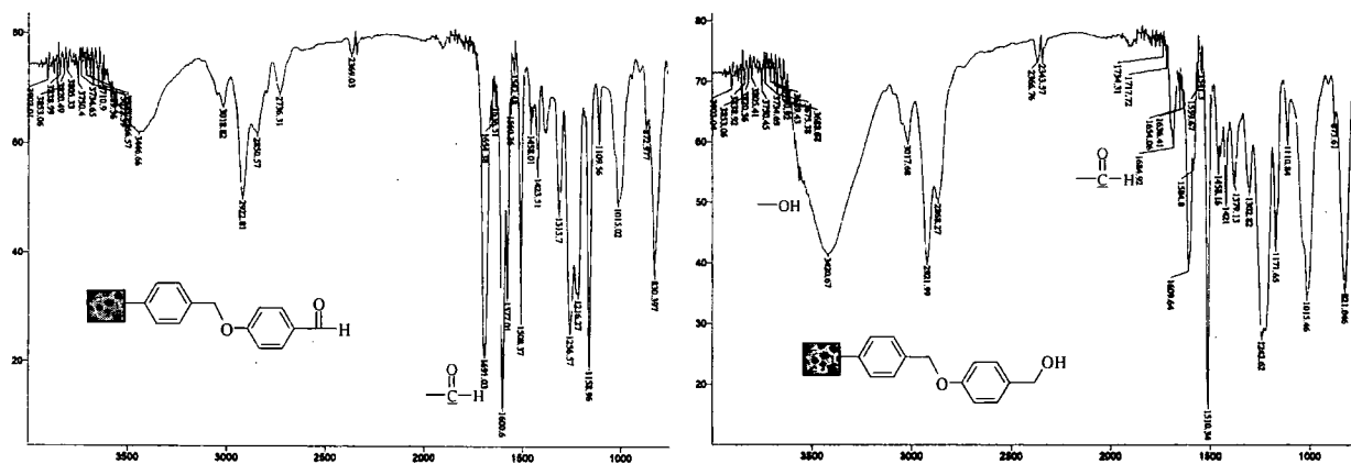
Figure 4.15 IR Spectra of PolyHIPE before and after reduction with \text{NaBH}_4
