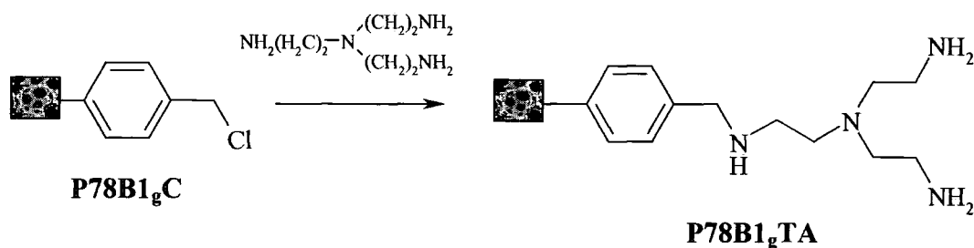
Figure 2.13 Synthesis of trisamine-immobilised PolyHIPE
