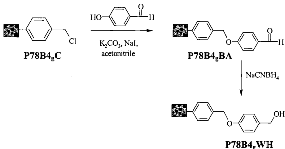
Figure 4.13 Alternative route to Wang-functionalised PolyHIPE
