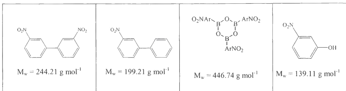
Figure 3.14 Possible by-products from the self-coupling of 3-nitrobenzeneboronic acid
