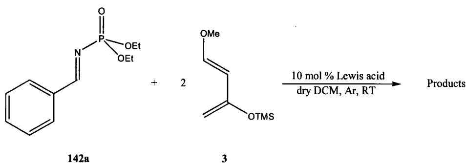
Equation 39
