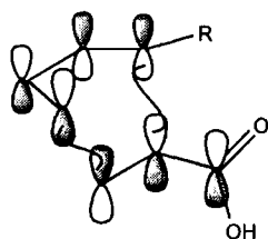
Exo-adduct T-S
