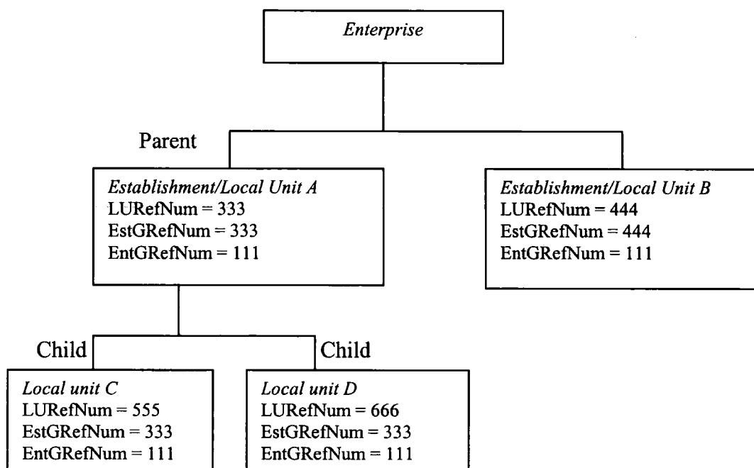
Figure 3.1 Structure of the ACOP Respondent Database (the ARD)
