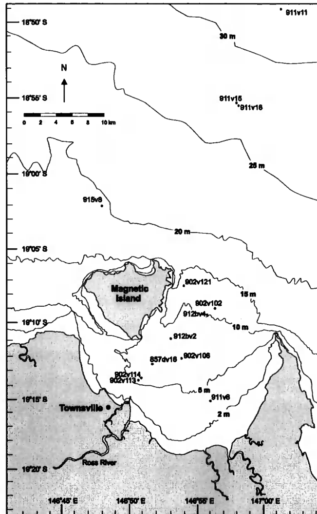
Fig. 4.1 Core locations for fossil samples in Cleveland Bay and the mid shelf
