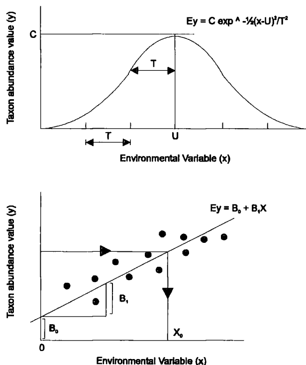
Fig. 4.3 Taxon response models (after ter Braak, 1988; Birks, 1995)
