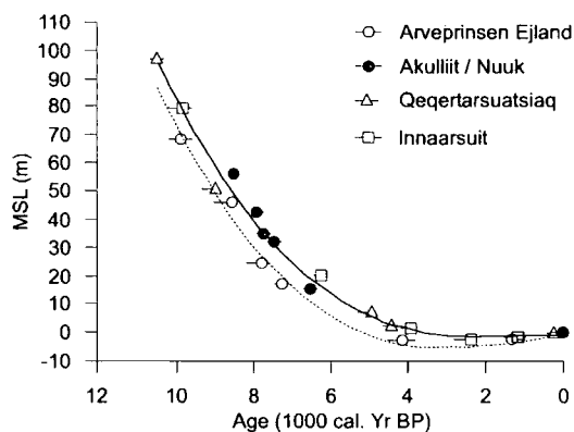
Fig. 2.2 RSL depicting MSL. The trend lines summarizing the data from Arveprinsen Ejland (Alluttoq), and the combined Innaarsuit and Qeqertarsuatsiaq data, are third-order polynomials. Other data are from Long and Roberts (2003) (Qeqertarsuatsiaq), Long and Roberts (2002) (Akullit/Nuuk), and Long et al. (1999) (Arveprinsen Ejland (Alluttoq)).
