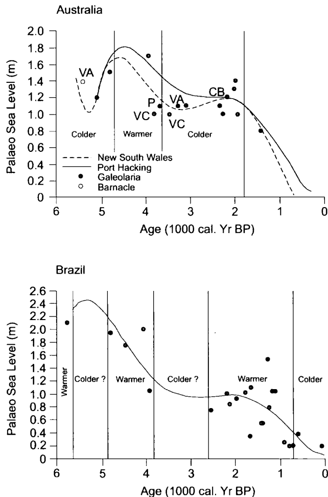
Fig. 2.13 The quintic polynomial regression models and histogram distribution of points. The vertical lines are event horizons of palaeoenvironmental change (Baker et al. , 2001b).
