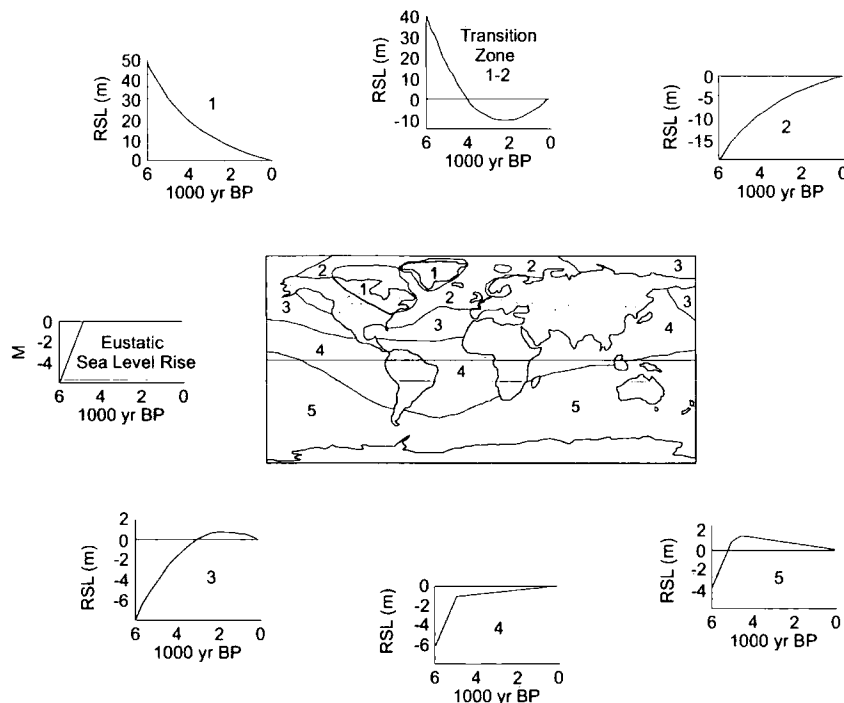
Fig. 2.1 Sea-level zones and typical RSL curves deduced for each zone by Clark et al. (1978) under the assumption that no eustatic change has occurred since 5,000 yr BP.
