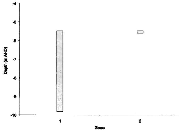
Fig. 3.16a Elevational range of the two foraminiferal zones highlighted for Transect 1
