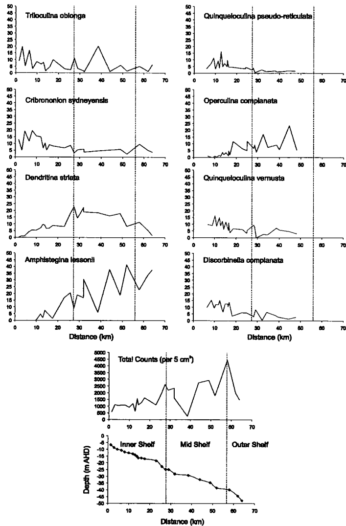
Fig. 3.6 Species plots with respect to distance offshore. Total counts are per 5cm 3 of sediment and extrapolated using the wet splitter. The inner, mid and outer shelf categories as defined by Belperio (1983).
