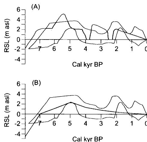
Fig. 2.8 Final sea-level curve for the study area (gray) against (A) the RSL curve for the Central Brazilian coast (solid line) of Bittencourt et al. (1979) and Suguio et al. (1985) and (B) the glacio-isostatic prediction of Peltier (1998a) (solid line) (Bezerra et al. , 2003).
