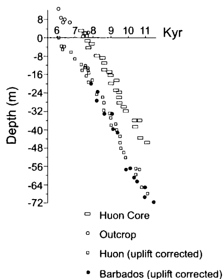
Fig. 2.5 Summary core log and age-depth plots of radiocarbon SLIPs (Chappell and Polach, 1991). The upper age-depth series is for samples uncorrected for uplift; lower series is corrected for uplift and is compared with Barbados (Fairbanks, 1989).
