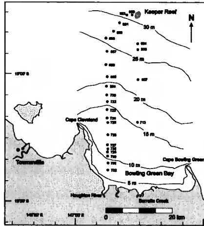
Fig. 3.3 Bowling Green Bay transect
