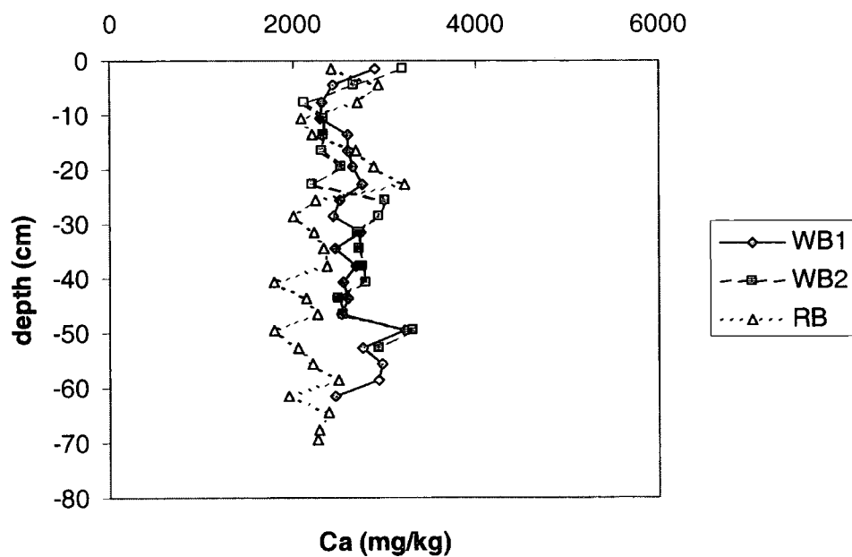
Figure 6.21. Stage 1 extractable Ca with depth in cores WB1, WB2 and RB from the Wansbeck impoundment.
