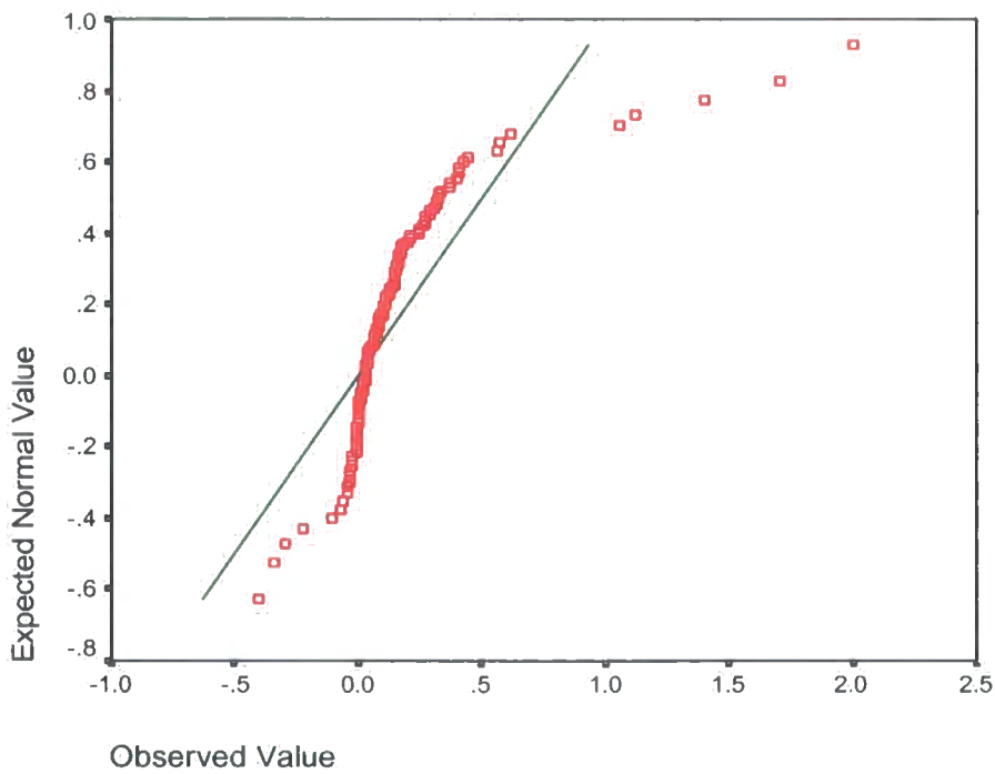
Figure 6-2 Normal Q-Q Plot of non-VC-backed IPOs
