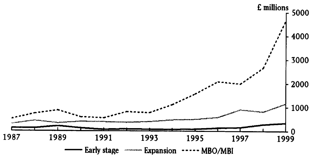
Figure 2-5 U.K. investment by stage
