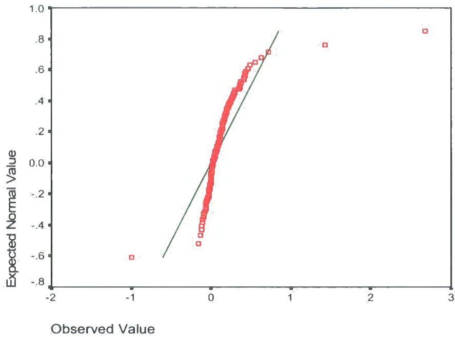
Figure 6-2 Normal Q-Q Plot of non-VC-backed IPOs
