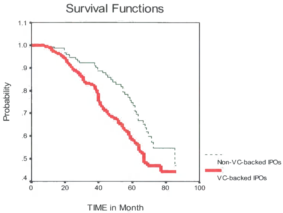
Figure 6-5 Survival functions
