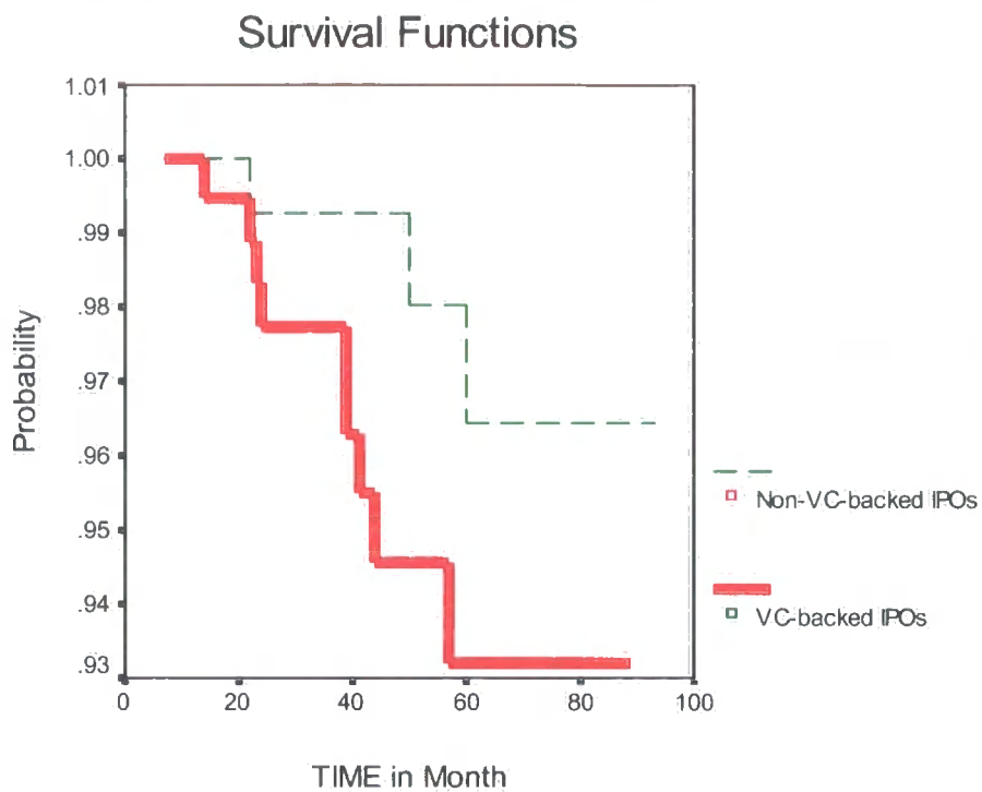
Figure 6-7 Survival functions excluding M&A
