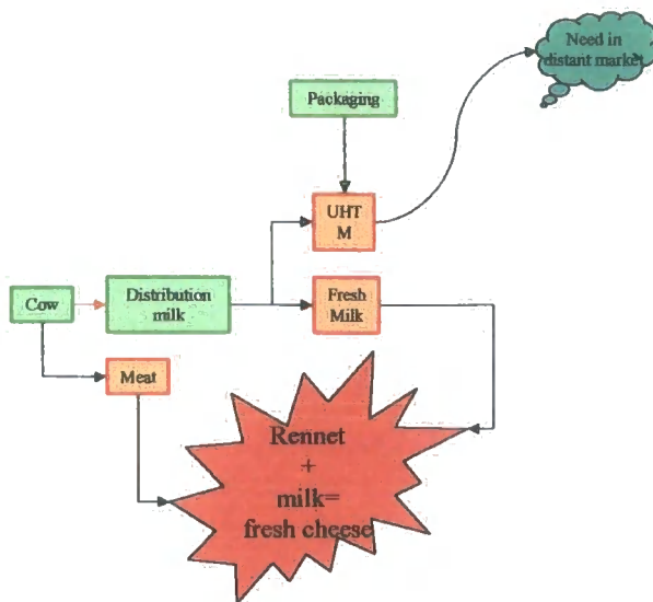
Figure 3 - Complementarity-based innovation
