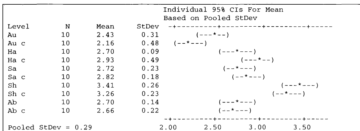
Figure 6-17: Control and cultivated means, standard deviation and 95% confidence intervals for available lead (Log10(100*mg kg -1 )) for farms Au, Ha, Sa, Sh and Ab
