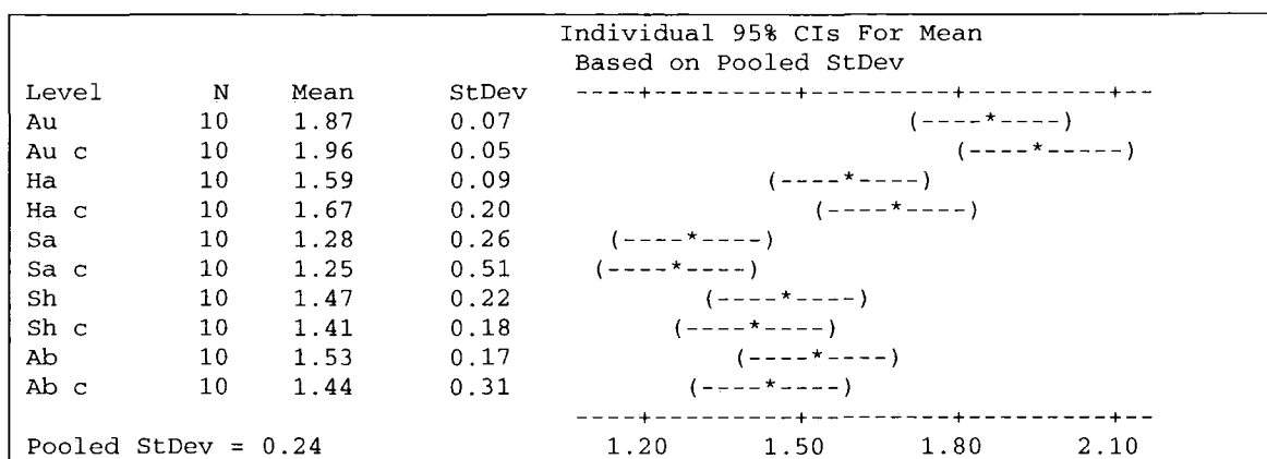
Figure 6-15: Control and cultivated means, standard deviation and 95% confidence intervals for available nickel (Log10(100*mg kg -1 )) for farms Au, Ha, Sa, Sh and Ab
