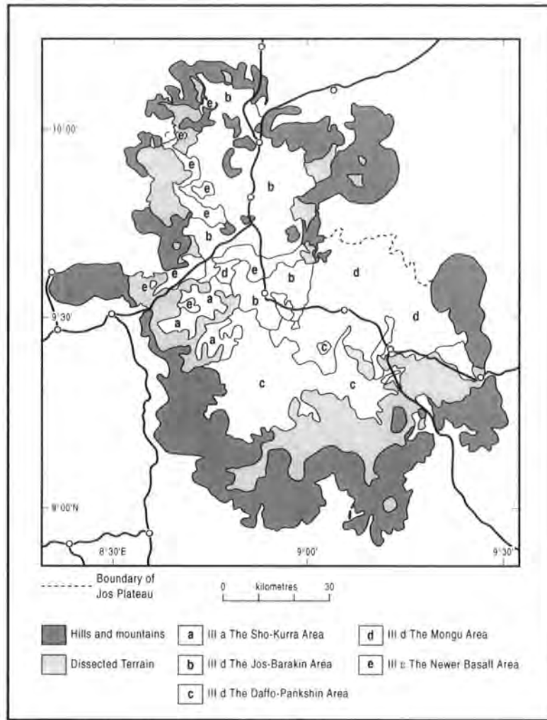
Figure 3-3: Physiography of the Jos Plateau (after Alford et al. , 1979)
