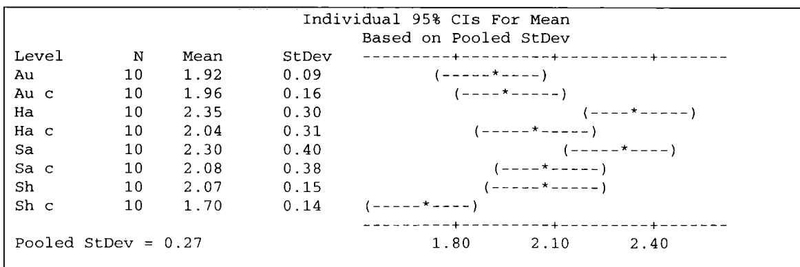
Figure 6-5: Control and cultivated means, standard deviation and 95% confidence intervals for exchangeable sodium ( \text{Log}_{10}(100 \times \text{cmol}_{(e)} \text{kg}^{-1}) ) for farms Au, Ha, Sa and Sh
