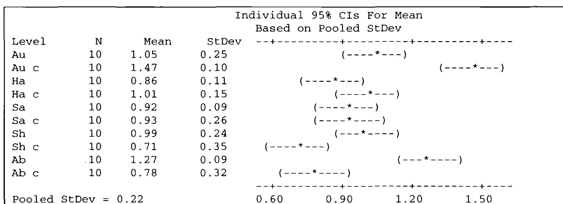
Figure 6-16: Control and cultivated means, standard deviation and 95% confidence intervals for available cadmium (Log10(100*mg kg -1 )) for farms Au, Ha, Sa, Sh and Ab
