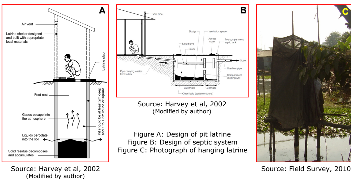
Figure 6.1: Different types and design of latrines in the study areas
