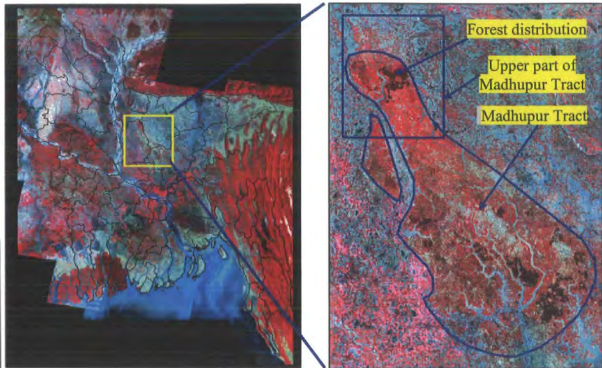
Figure 8: Location of Madhupur Tract in satellite image mosaic map of Bangladesh (left). Distribution of deciduous sal forest in the upper parts of that physiographic unit (right).
