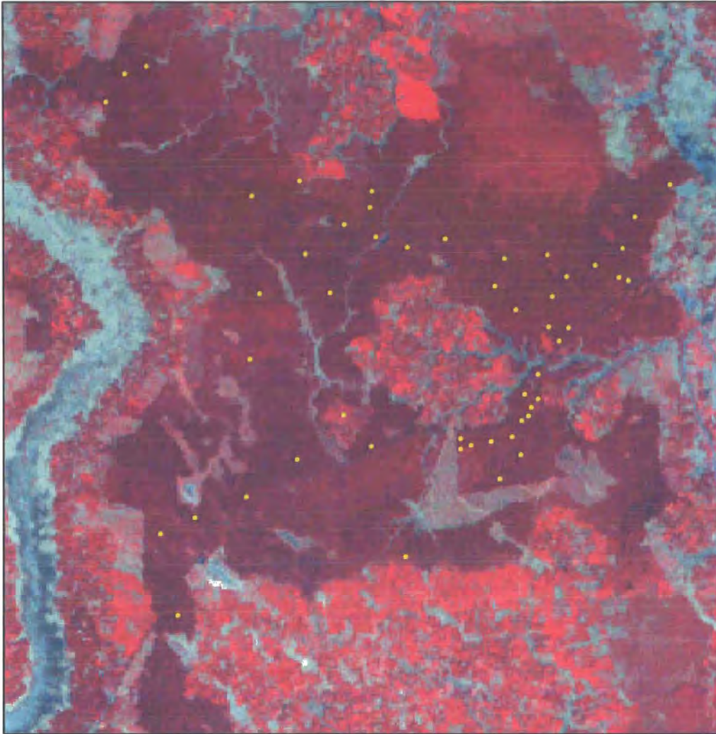
Figure 3: Distribution of sample plots in Landsat ETM+ 2003 image.
