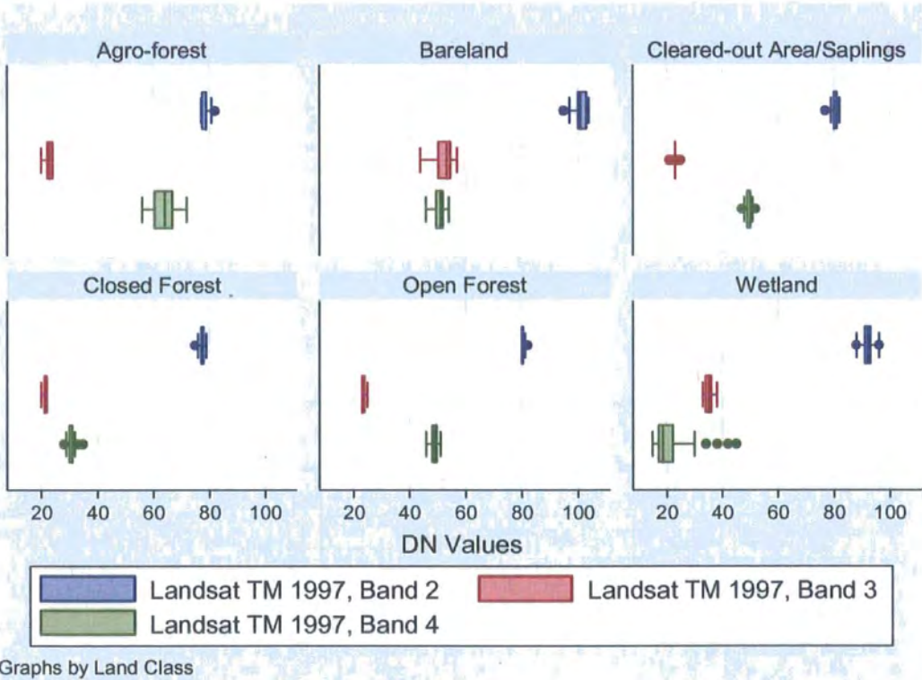
Figure 3a: Spectral response patterns of different bands of IRS-LISS III 2005 and Landsat TM 1997 for different land classes (data extracted from sample plots).
