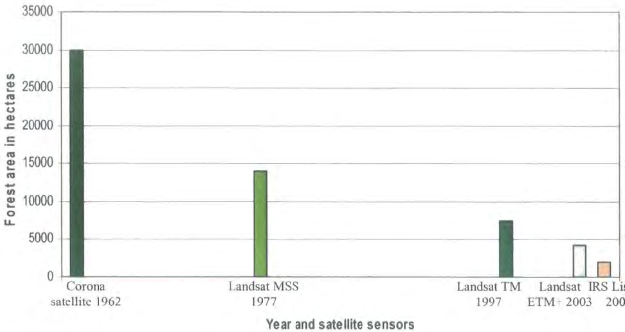
Figure 9: Forest cover in madhupur thana in different satellite sensors.
