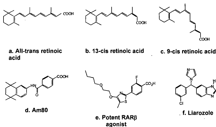
Figure 1.5: Chemical structures of retinoids (a-e) and a retinoic acid metabolism blocking agents (RAMBAs) compound (f) which are either already being used in therapy regimes for neurological disorders (a, b, c, d & f) or show promising potential as therapeutic agents (e). a, b, & c are naturally occurring retinoids and d, e, & f are synthetic compounds. Diagram taken from Christie et al 2008 123 .
