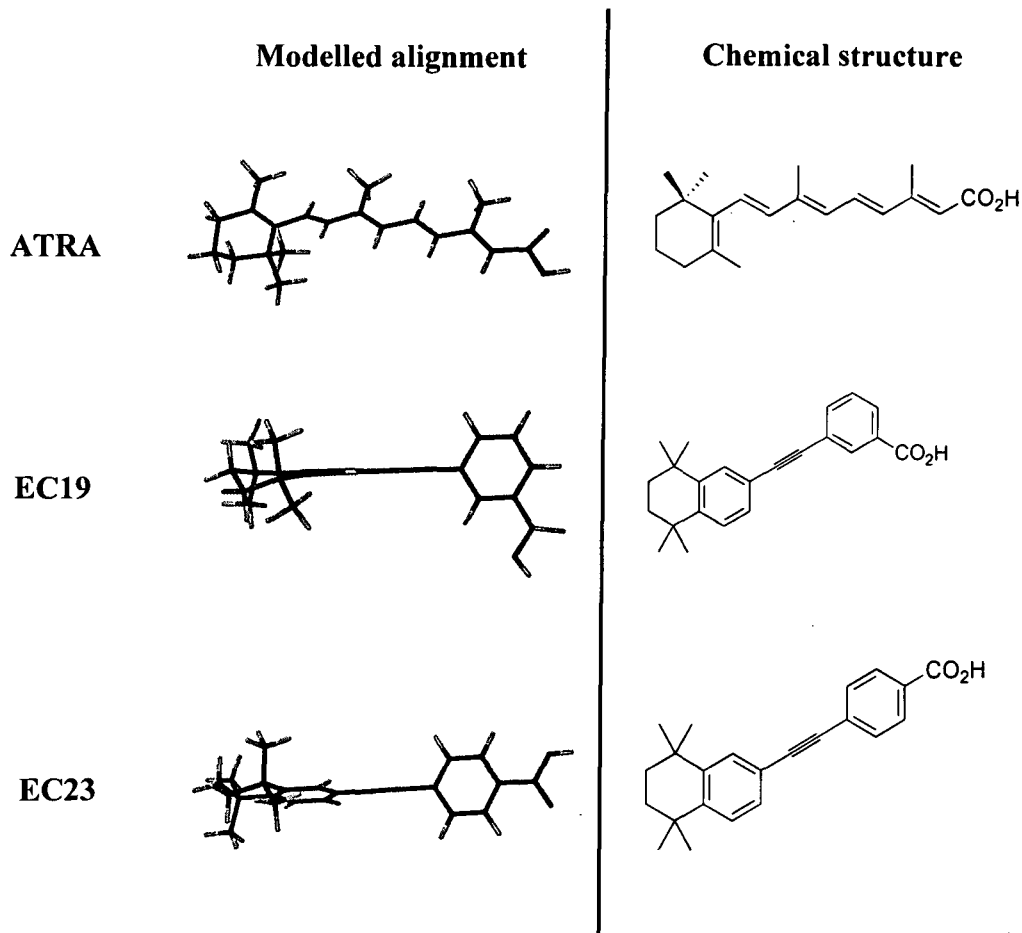
Figure 1.6: Structure and chemical alignment of ATRA and the synthetic retinoids EC19 and EC23. It is noted that the chemical alignment of EC23 is most similar to the natural retinoid ATRA. Both EC19 and EC23 have a triple carbon bond inserted into the polyene chain. This is hypothesised to instil stability to these synthetic analogues.
