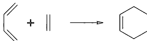
Figure 3.5 Scheme for the Diels-Alder reaction between butadiene and ethene
