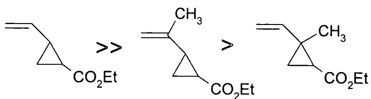
Figure 2.55 Schematic illustrating the relation between three monomers and resultant molecular weights, decreasing from left to right, of the polymers investigated by Endo 80
