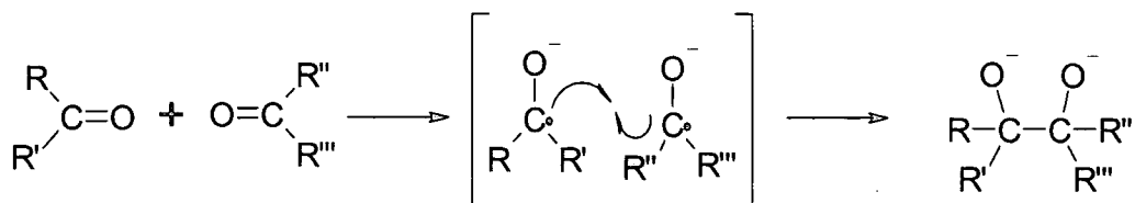
Figure 2.23 Dimerisation step
