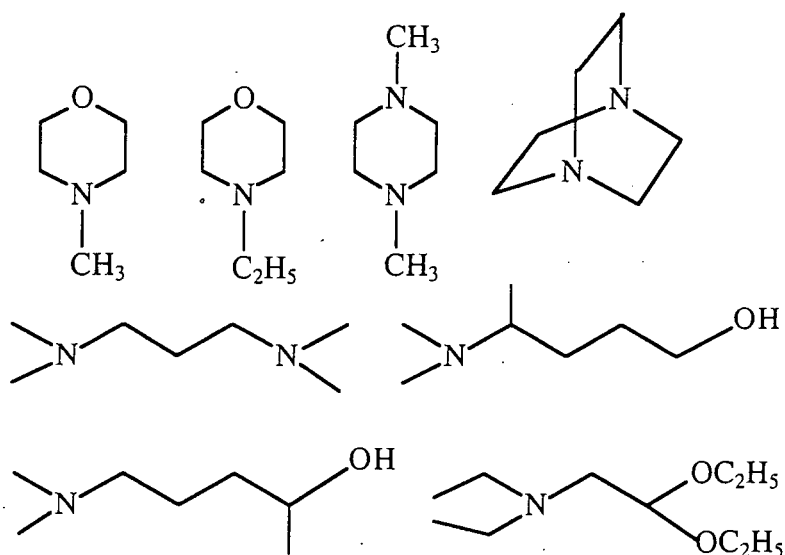
Scheme 161
