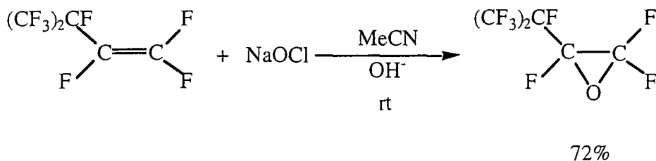
Scheme 121
