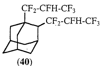
Scheme 56
