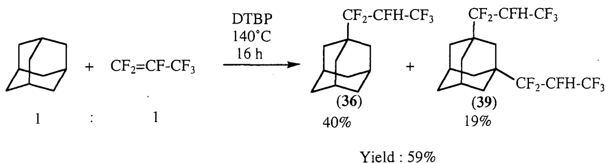
Scheme 50
