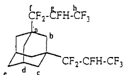
No. 2 1,1,2,3,3,3-hexafluoro-1-[3-(1,1,2,3,3,3-hexafluoropropyl)adamantanyl]propane (39)
