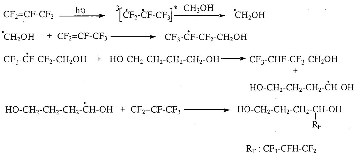
Scheme 28
