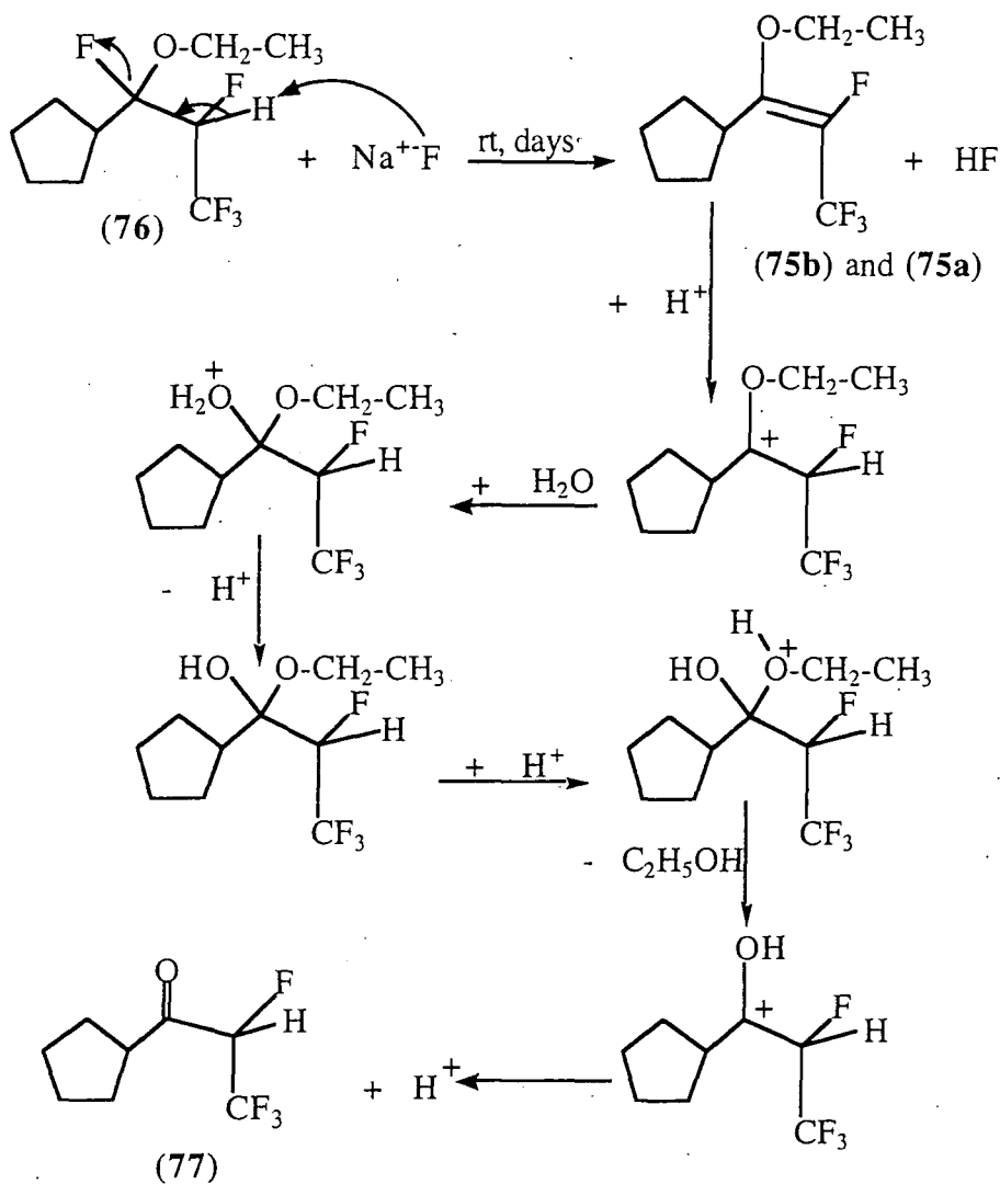
Scheme 130
