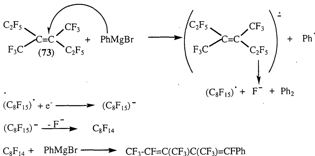
Scheme 115
