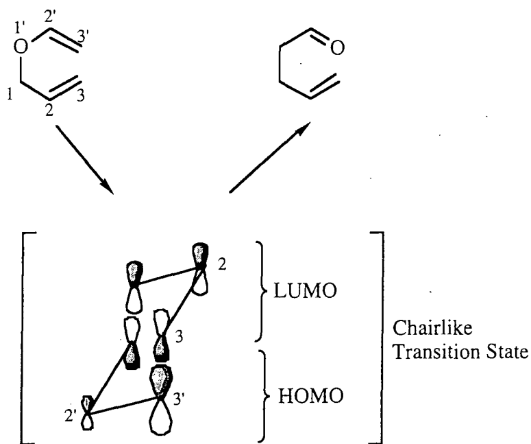
Scheme 103
