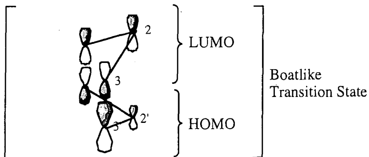
Scheme 104
