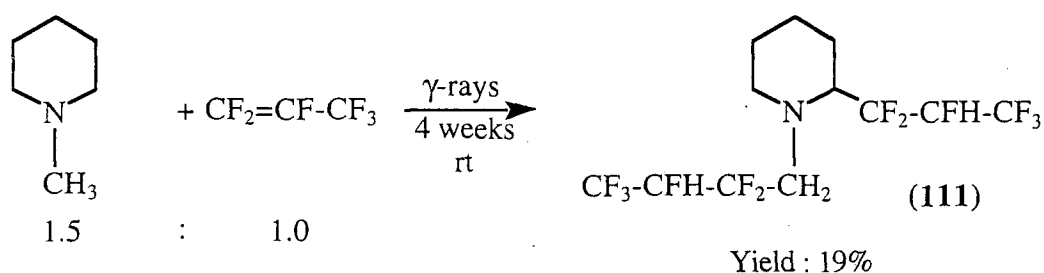
Scheme 171
