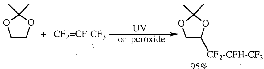
Scheme 35
