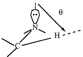
Scheme 40
