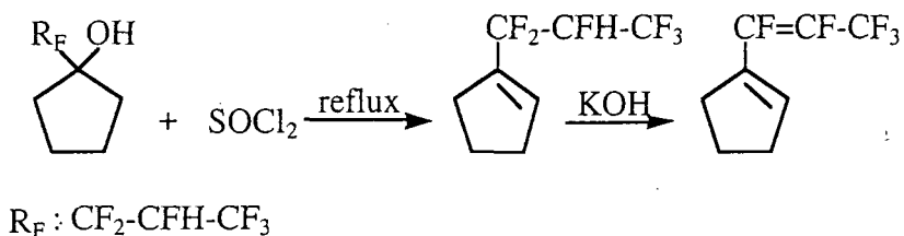
Scheme 69
