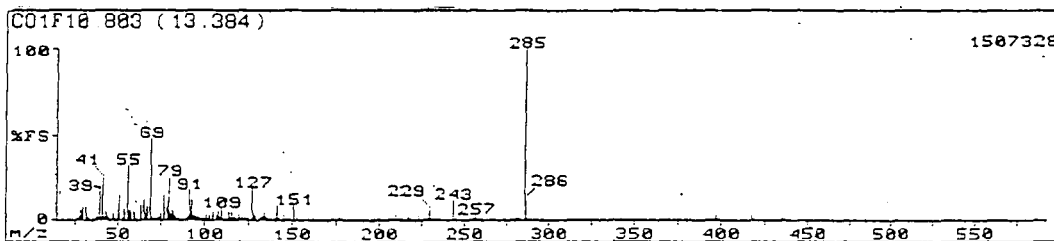
No. 2 1,1,2,3,3,3-hexafluoro-1-(3-(1,1,2,3,3,3-hexafluoropropyl)adamantanyl)propane (39)
