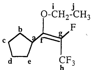
Scheme 127
