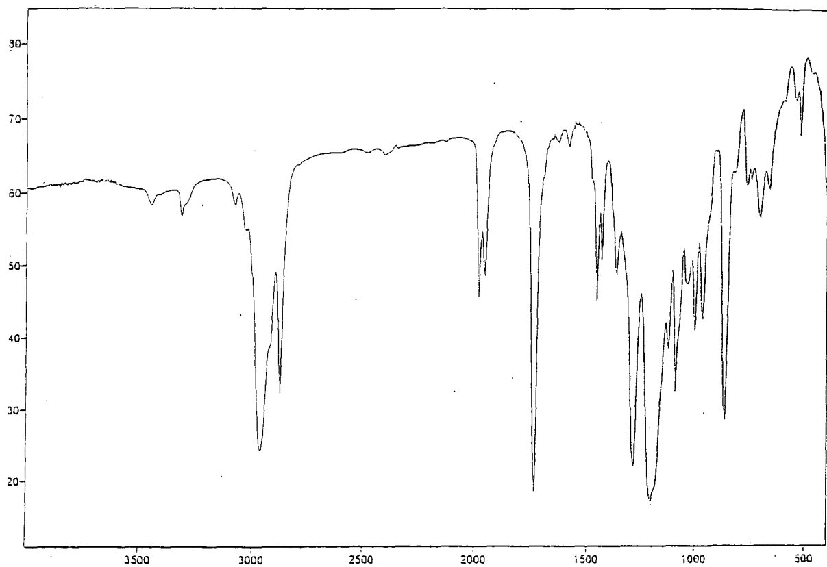
No. 19 1-cyclopentyl-2-fluoro-3-methyl-2-trifluoromethyl-4-penten-1-one (86)
