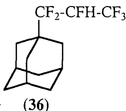
Scheme 53
