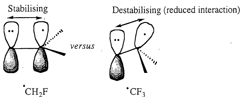
Scheme 12
