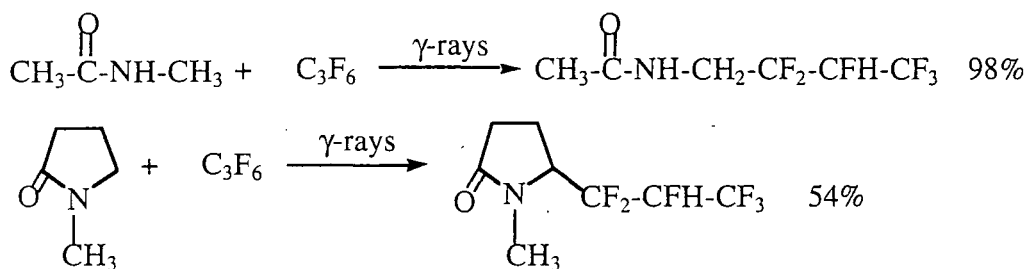
Scheme 41
