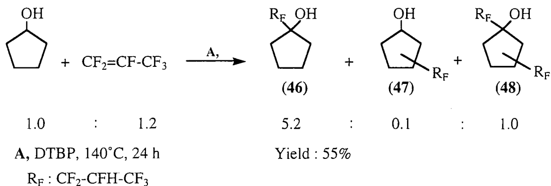
Scheme 66
