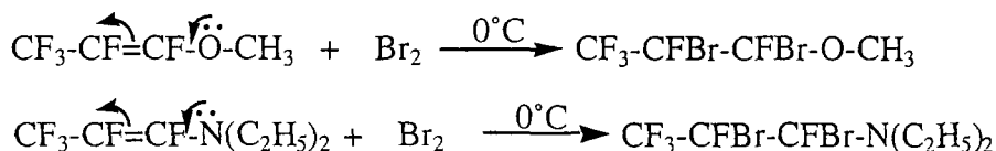
Scheme 118
