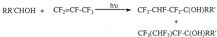
Scheme 26
