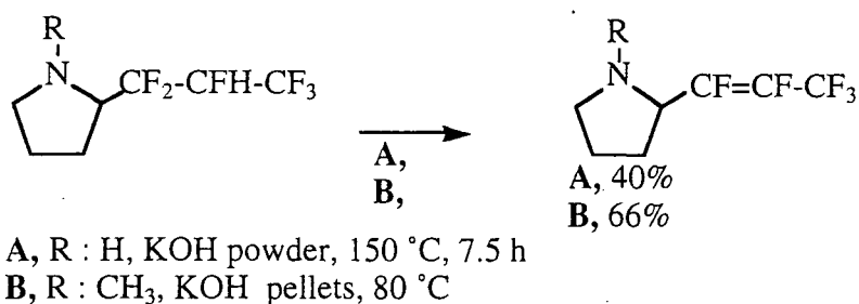
Scheme 80
