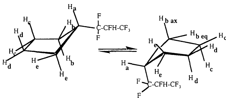
Scheme 59
