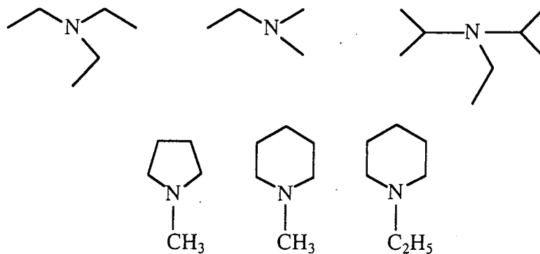
Scheme 160
