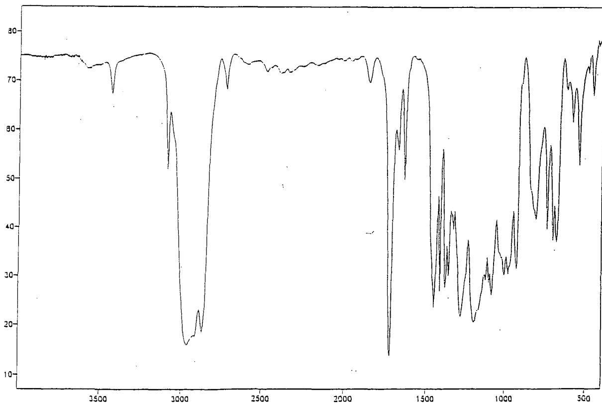
No. 21 1-cyclopentyl-3-ethenyl-2-fluoro-3,7-dimethyl-2-trifluoromethyl-6-octen-1-one (92)
