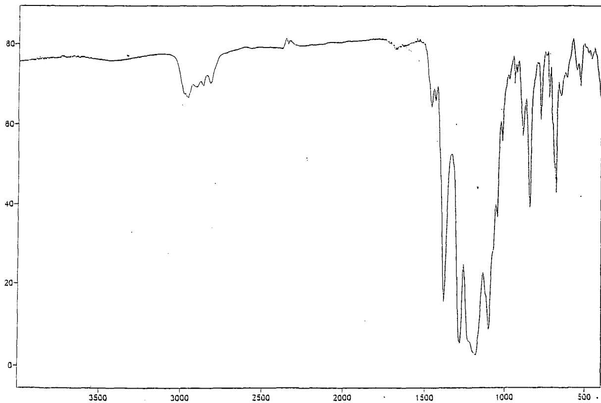
No. 41 1,4-dimethyl-2,3,5-tris(1,1,2,3,3,3-hexafluoropropyl)piperazine (118)
