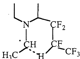
Scheme 166
