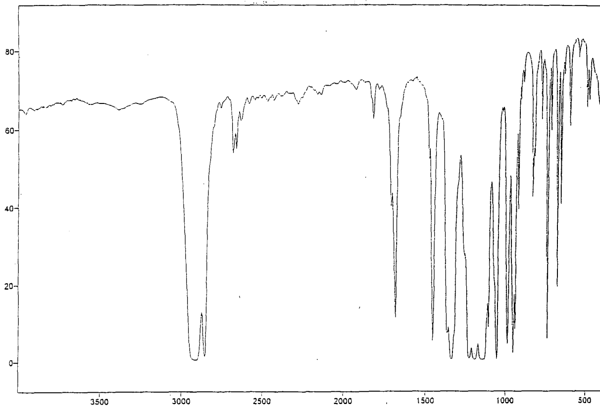
No. 9 ( E )-1-adamantanyl-1,2,3,3,3-pentafluoroprop-1-ene (53a) and ( Z )-1-adamantanyl-1,2,3,3,3-pentafluoroprop-1-ene (53b)
