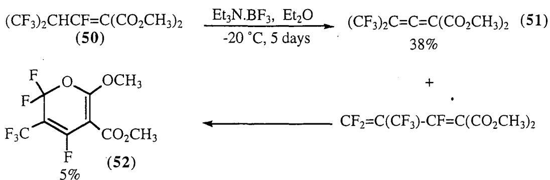
Scheme 82
