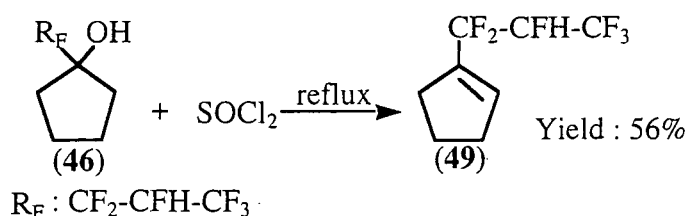
Scheme 72
