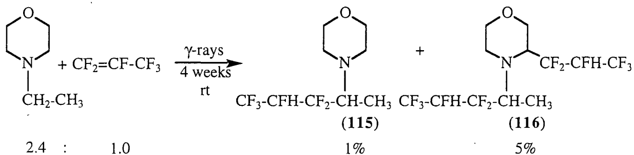
Scheme 179
