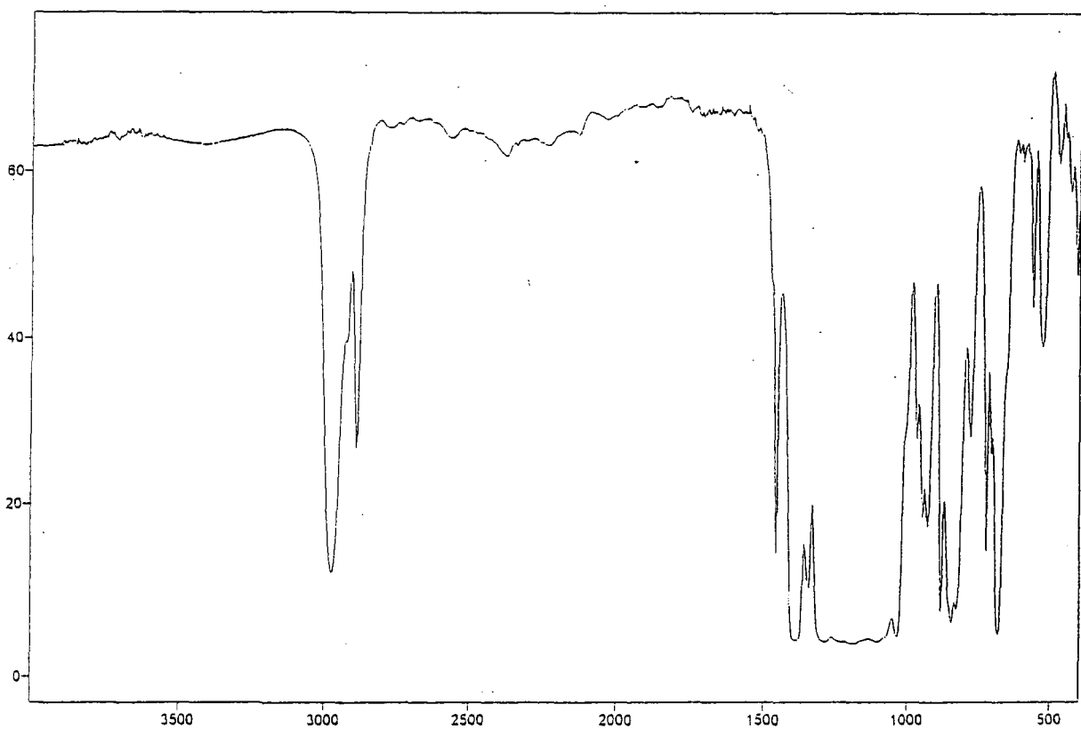
No. 6 1,1,2,3,3-hexafluoro-1-[3-(1,1,2,3,3,3-hexafluoropropyl)cyclopentyl]propane (44b)
