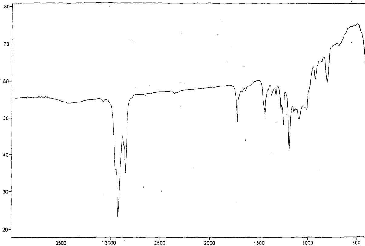
No. 17 1-cyclopentyl-2-fluoro-2-trifluoromethyl-4-penten-1-one (79)
