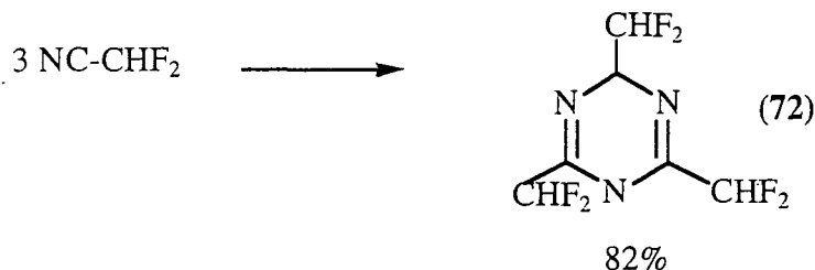
Scheme 111
