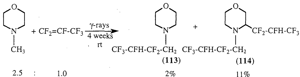
Scheme 177
