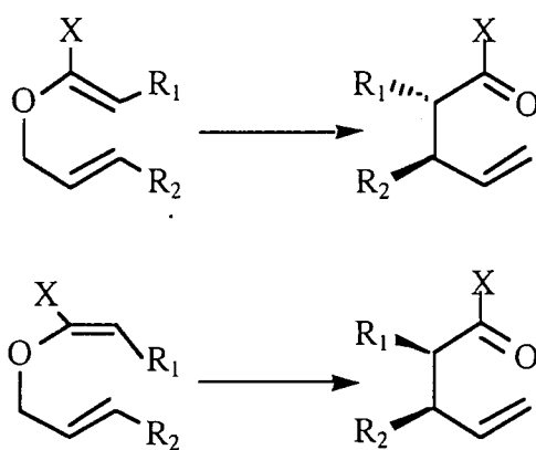
Scheme 105
