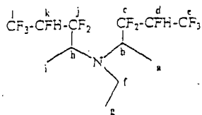
No. 28 bis(2,2,3,4,4,4-hexafluoro-1-methylbutyl)ethylamine (105) Minor Diastereoisomers
