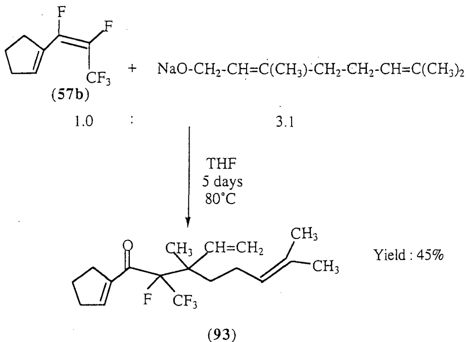
Scheme 146
