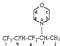
No. 38 4-(2,2,3,4,4,4-hexafluoro-1-methylbutyl)morpholine (115) Minor Diastereoisomers
