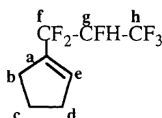
Scheme 73
