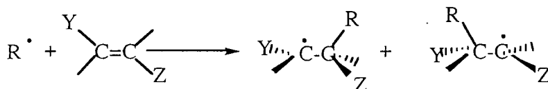
Scheme 17
