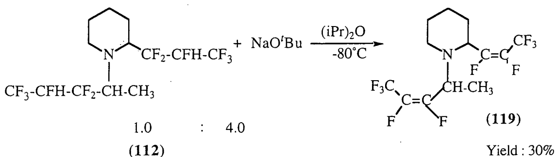
Scheme 182
