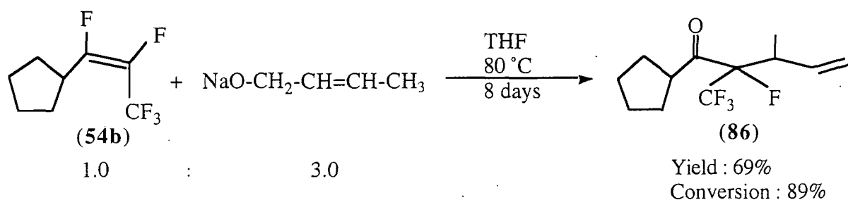
Scheme 139
