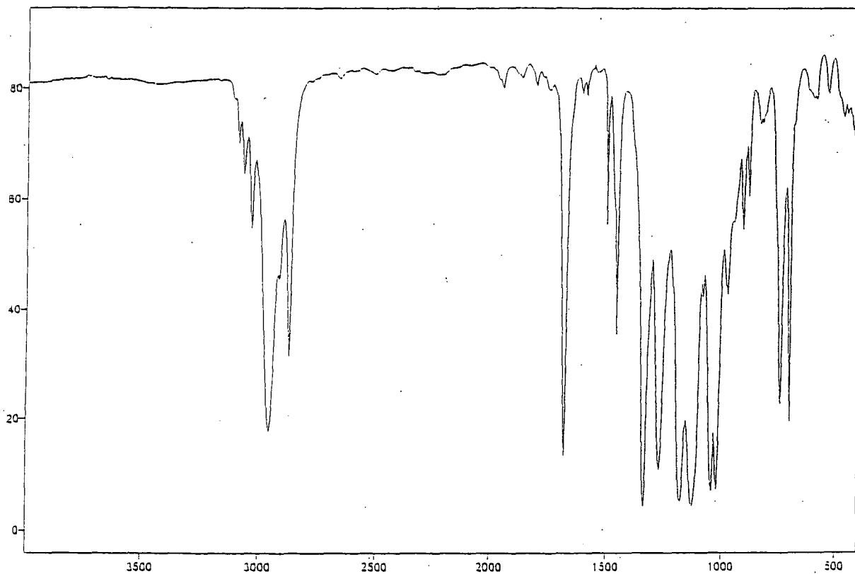
No. 23 Z-(1-cyclopentyl-2,3,3,3-tetrafluoro-1-propenoxy)methylbenzene (94)
