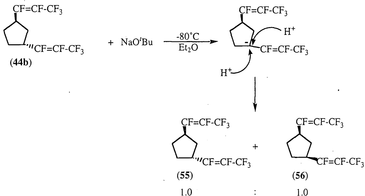
Scheme 89
