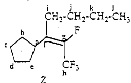
No. 24 Z-(1-butyl-2,3,3,3-tetrafluoro-1-propenyl)cyclopentane (99)
