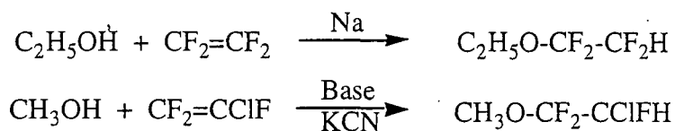
Scheme 97
