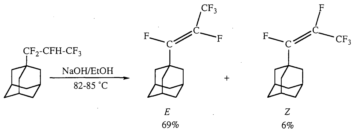
Scheme 76
