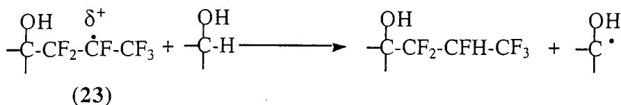
Scheme 24
