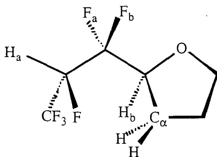
Scheme 34
