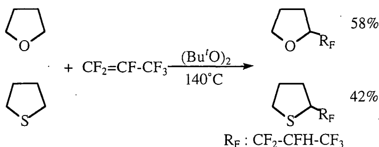
Scheme 43
