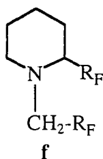
Scheme 174
