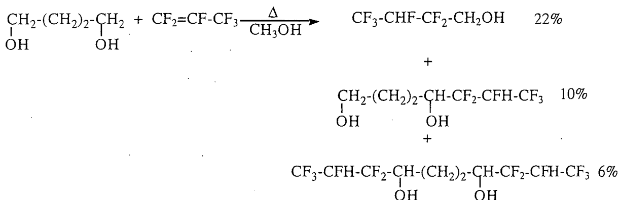
Scheme 27
