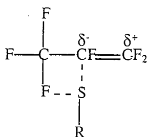
Scheme 22
