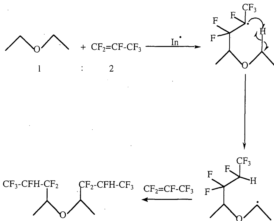
Scheme 29
