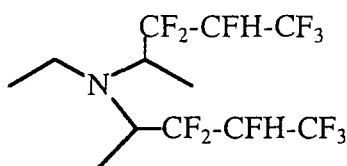
Scheme 165
