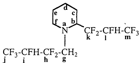
Scheme 175
