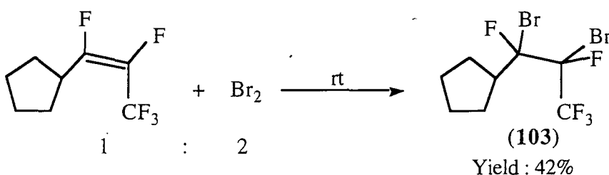
Scheme 159
