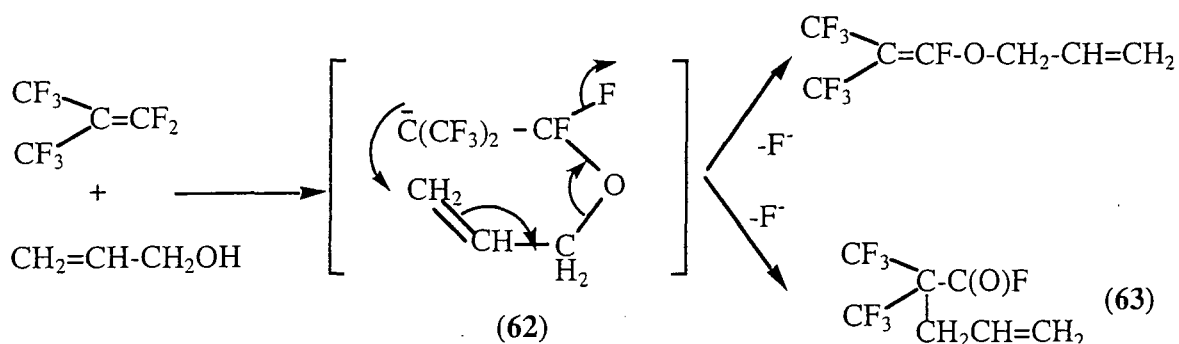
Scheme 107
