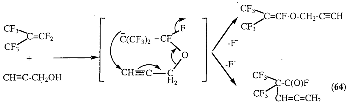
Scheme 108
