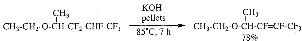
Scheme 79
