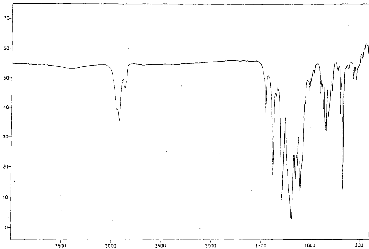
No. 2 1,1,2,3,3,3-hexafluoro-1-[3-(1,1,2,3,3,3-hexafluoropropyl)adamantanyl] propane (39)
