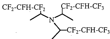
Scheme 167
