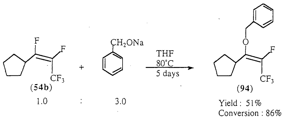
Scheme 147
