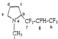
110 2-(1,1,2,3,3,3-hexafluoropropyl)-1-methylpyrrolidine (110) Major Diastereoisomers
