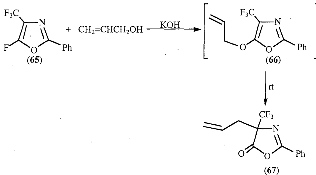
Scheme 109
