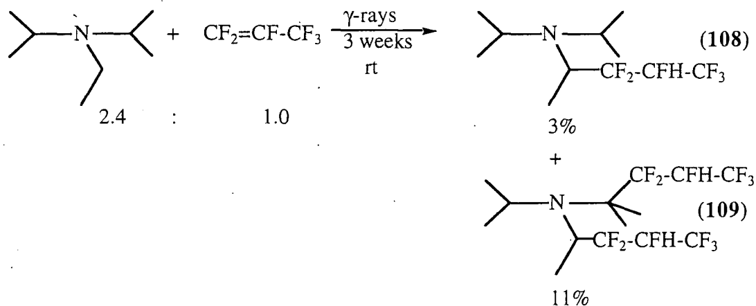
Scheme 169
