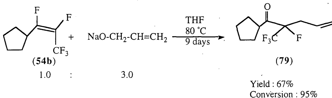
Scheme 132
