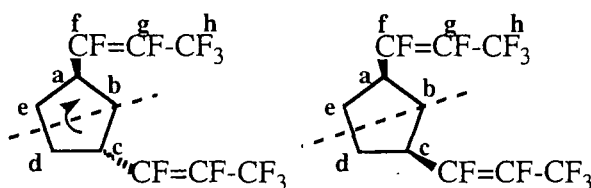
Scheme 88
