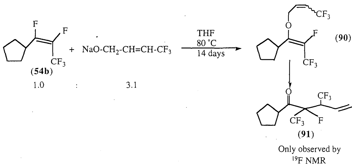
Scheme 144
