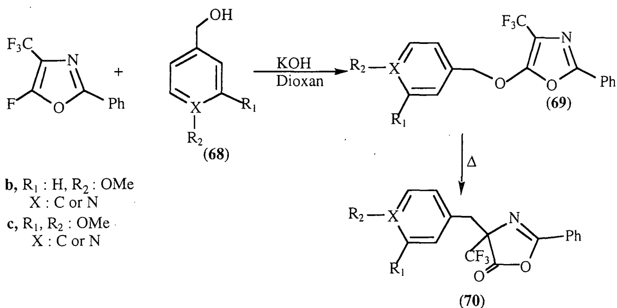
Scheme 110
