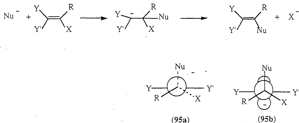
Scheme 148
