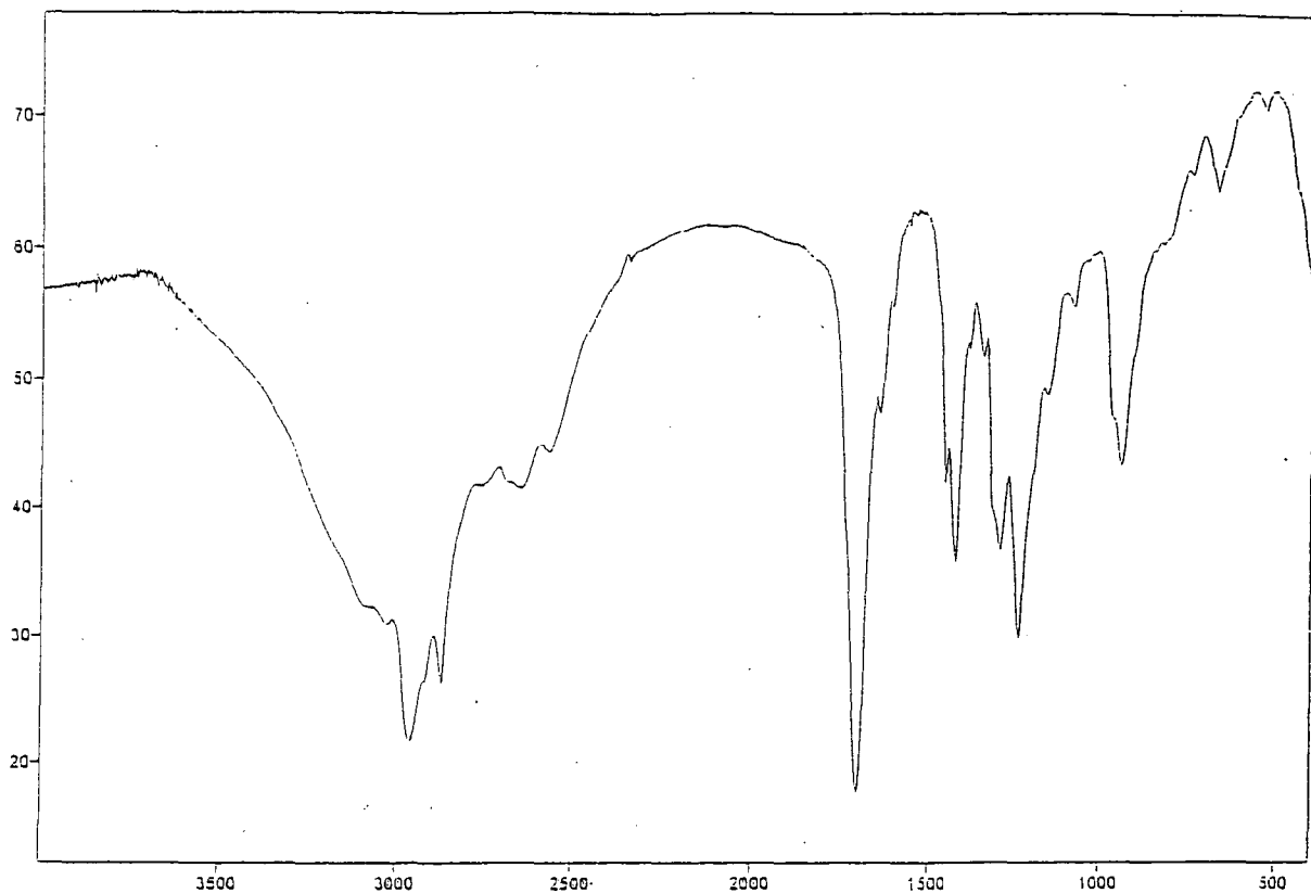
No. 20 cyclopentane carboxylic acid (88)
