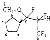
No. 16 1-cyclopentyl-1,2,3,3,3-pentafluoro-1-methoxypropane (78)
