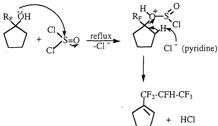
Scheme 71
