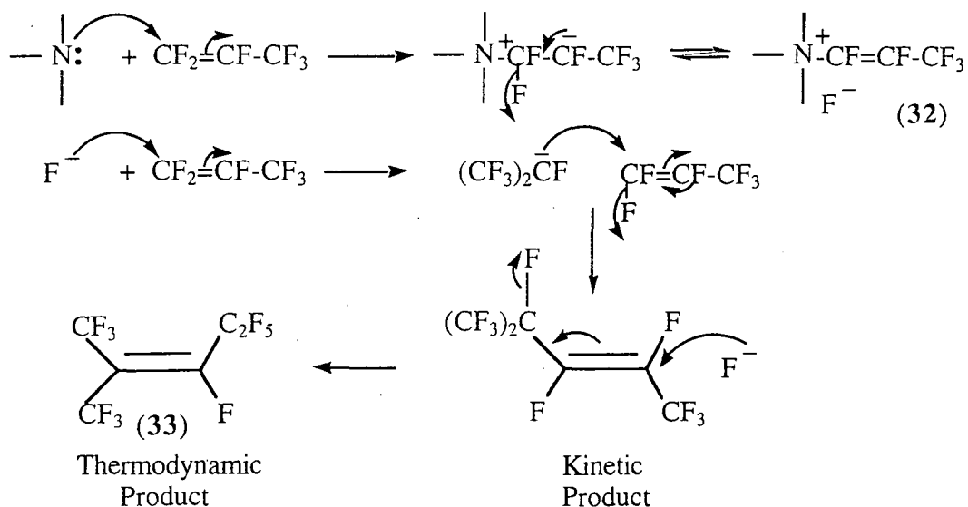
Scheme 37
