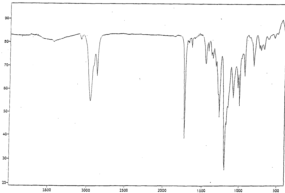
No. 19 1-cyclopentyl-2-fluoro-3-methyl-2-trifluoromethyl-4-penten-1-one (86)
