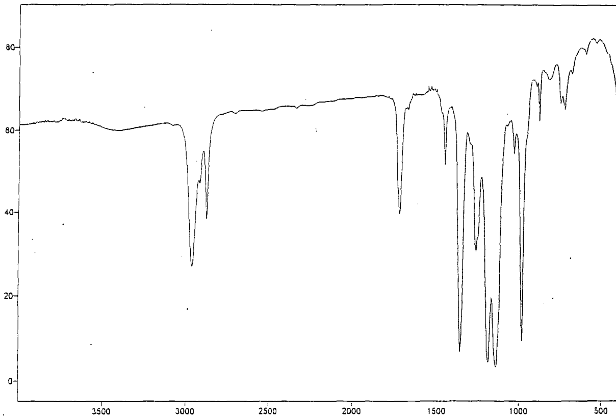
No. 10 1-( E -pentafluoroprop-2-enyl)cyclopentane (54a) and 1-( Z -pentafluoroprop-2-enyl)cyclopentane (54b)
