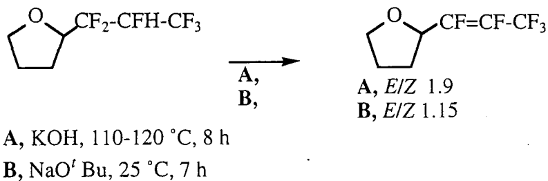
Scheme 77
