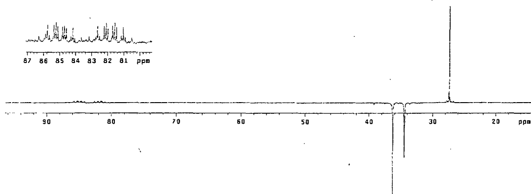
Scheme 52
