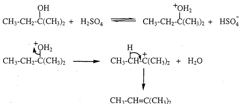
Scheme 70
