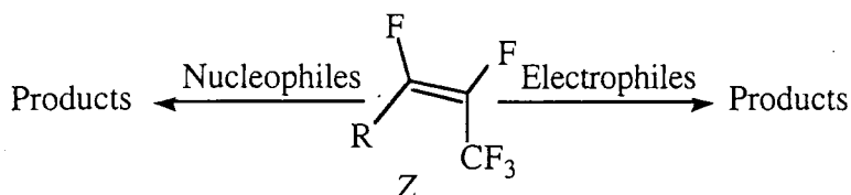
Scheme 91
