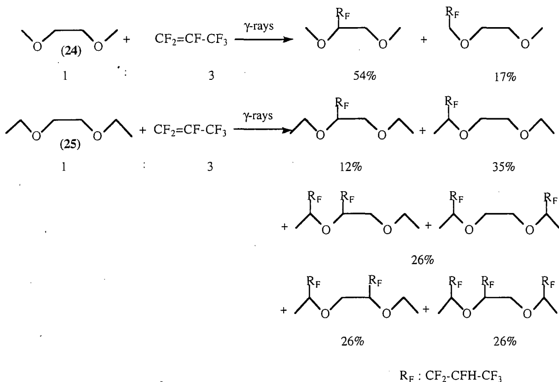
Scheme 31
