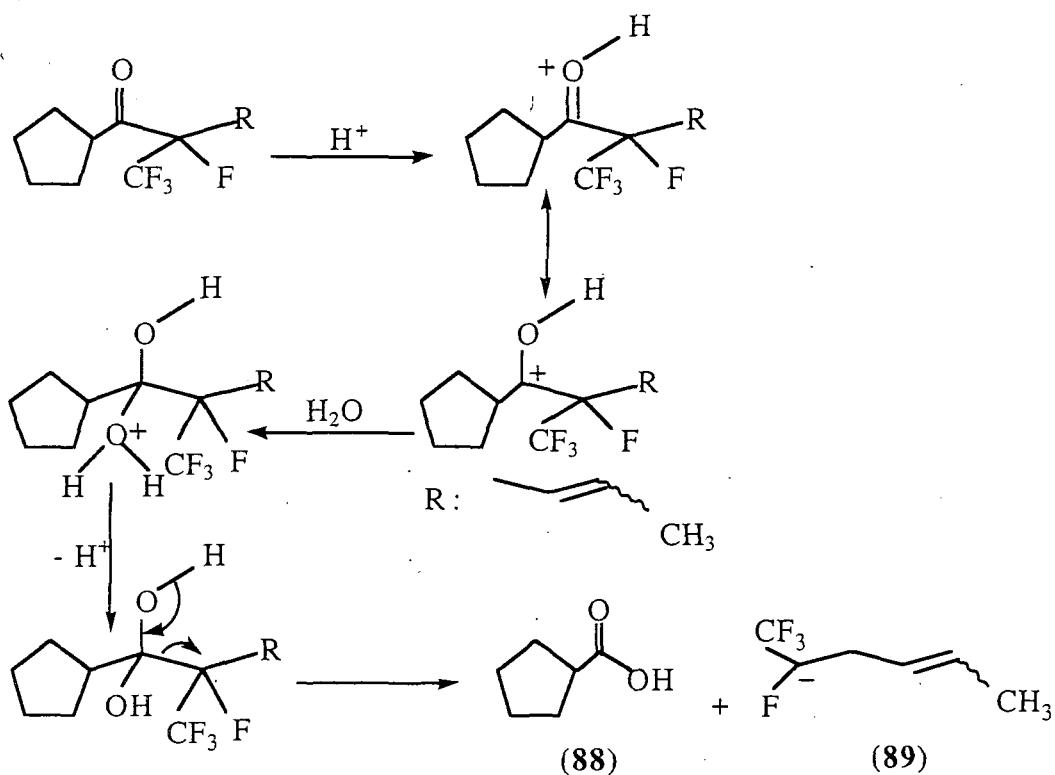
Scheme 143
