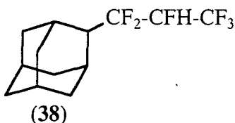
Scheme 54
