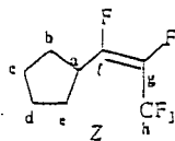
No. 10 1-(Z-pentafluoroprop-2-enyl)cyclopentane (54b)
