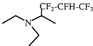
Scheme 164
