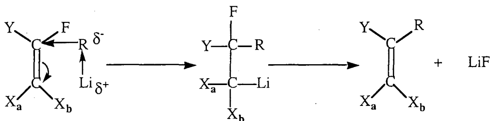
Scheme 114
