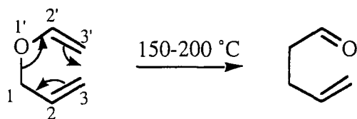
Scheme 102
