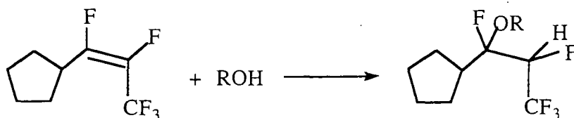
Scheme 125
