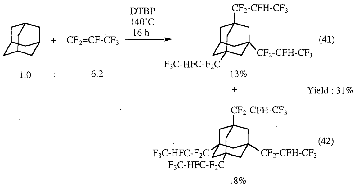
Scheme 57
