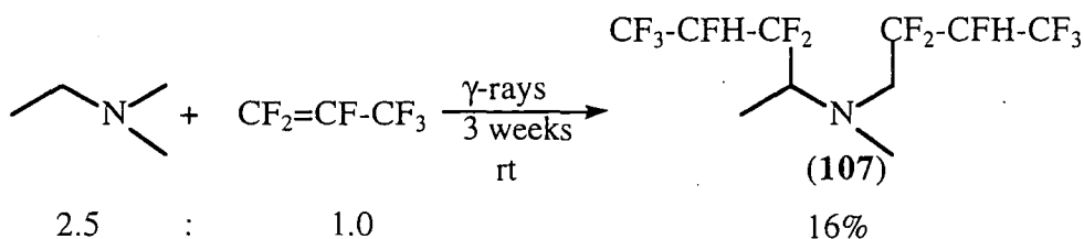
Scheme 168
