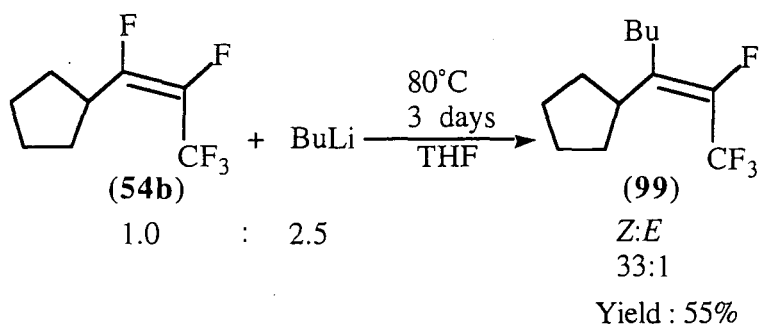
Scheme 154
