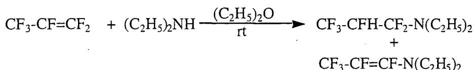
Scheme 112
