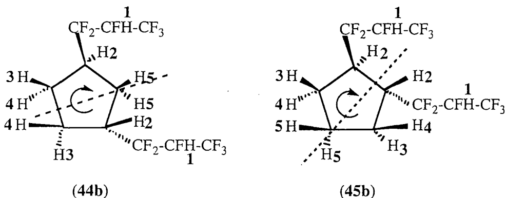
Scheme 62
