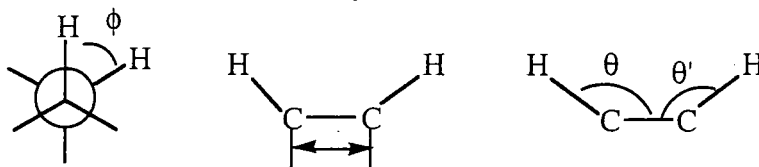
Scheme 49
