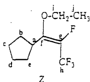
No. 13 (1Z)-1-cyclopentyl-1-ethoxy-2,3,3,3-tetrafluoroprop-1-ene (75b)
