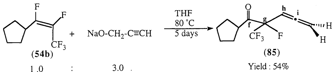
Scheme 138
