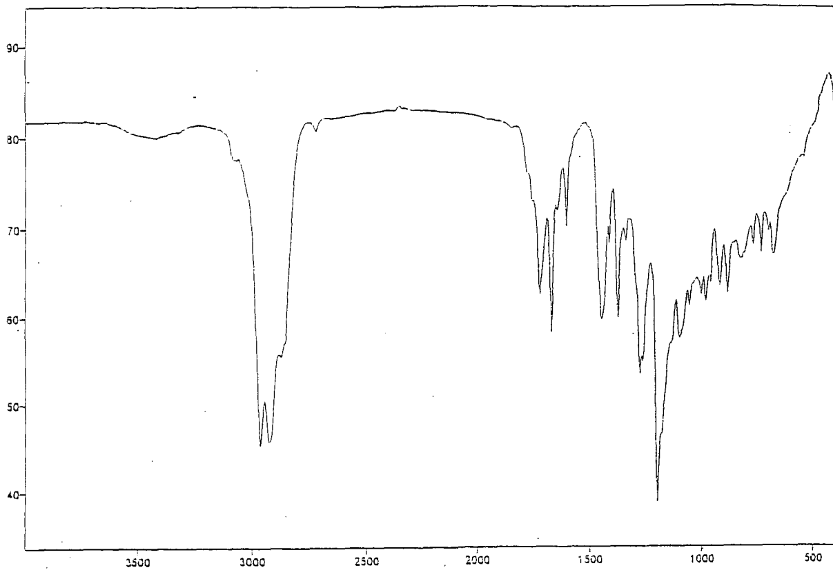
No. 23 Z-(1-cyclopentyl-2,3,3,3-tetrafluoro-1-propenoxy)methylbenzene (94)
