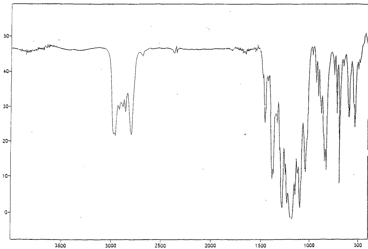
No. 33 2-(1,1,2,3,3,3-hexafluoropropyl)-1-methylpyrrolidine (110)
