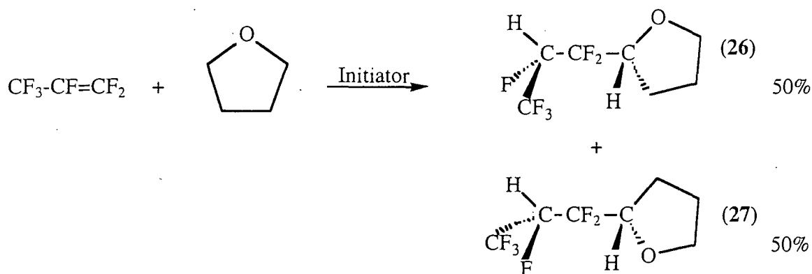
Scheme 33
