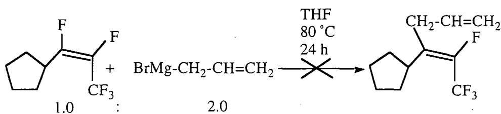
Scheme 157
