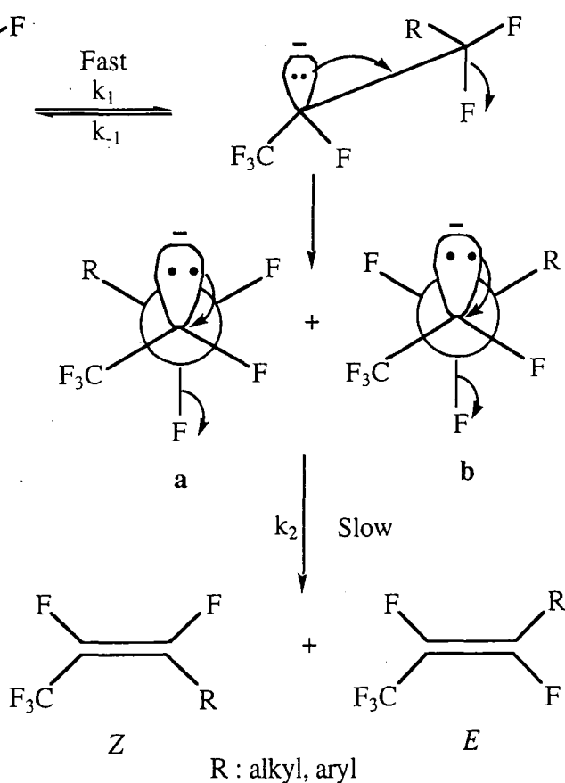
Scheme 83
