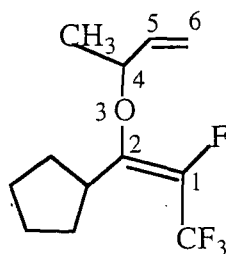
Scheme 142
