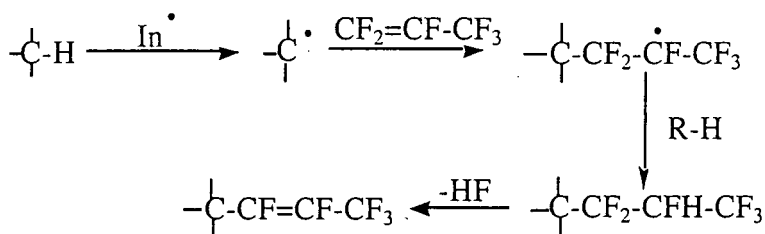
Scheme 48
