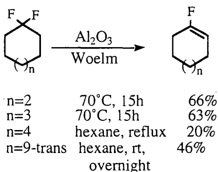
Scheme 75
