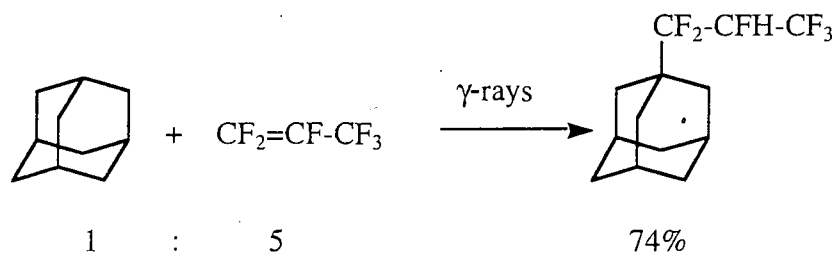
Scheme 44
