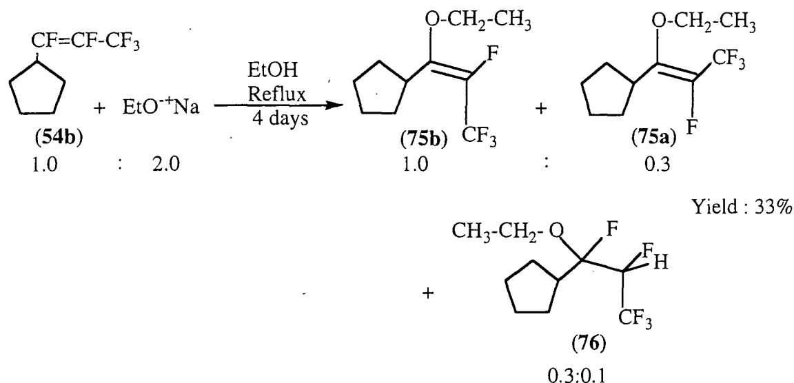
Scheme 126
