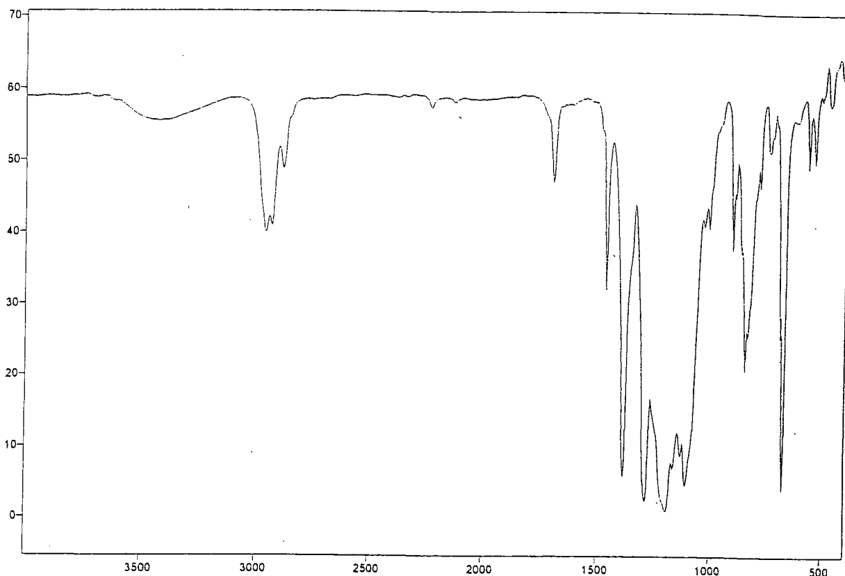
No. 3 1-[3,5-bis(1,1,2,3,3,3-hexafluoropropyl)adamantanyl]-1,1,2,3,3,3-hexafluoro propane (41)
