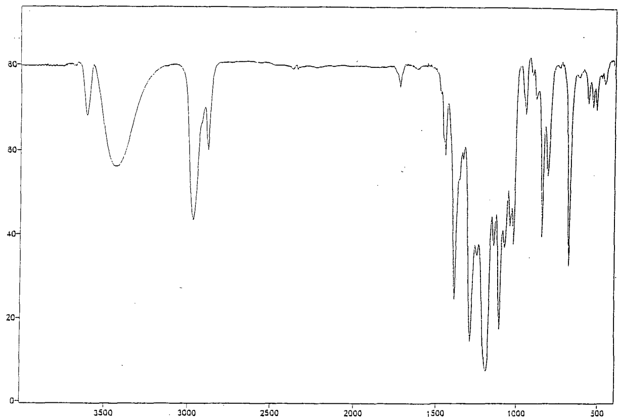
No. 7 1-(1,1,2,3,3,3-hexafluoropropyl)cyclopentanol (46)
