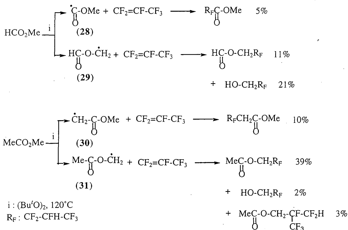
Scheme 36
