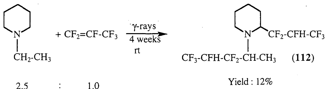
Scheme 176
