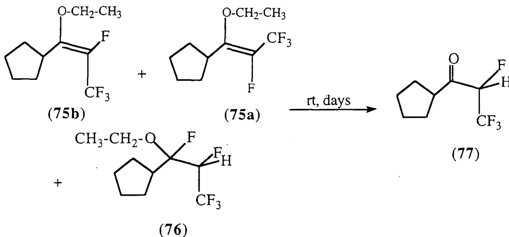
Scheme 129
