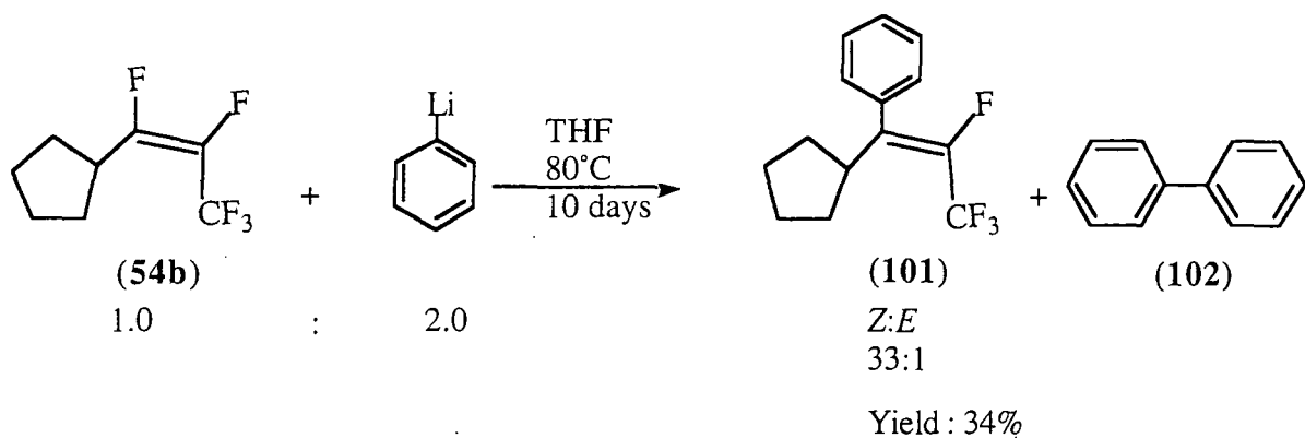
Scheme 156
