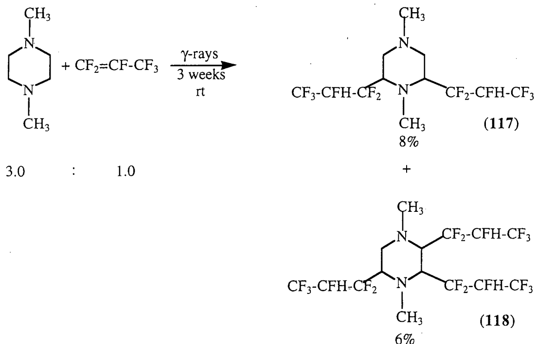
Scheme 181
