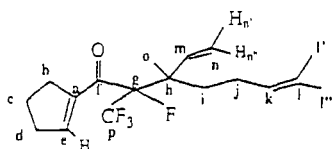
22 1-cyclopent-1-enyl-2-fluoro-3,7-dimethyl-2-(trifluoromethyl)-3-vinyloct-6-ene (93)
