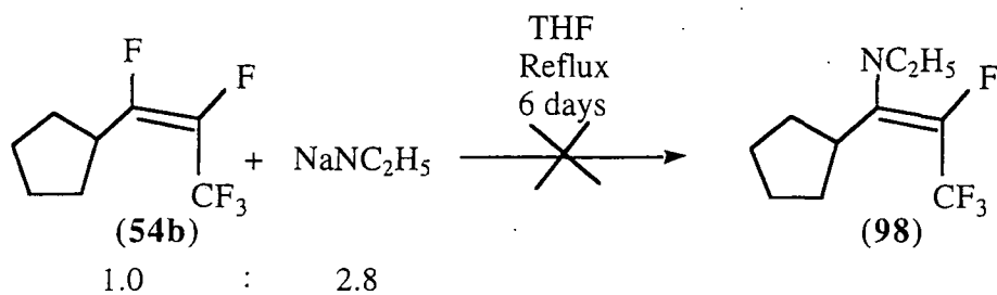
Scheme 153
