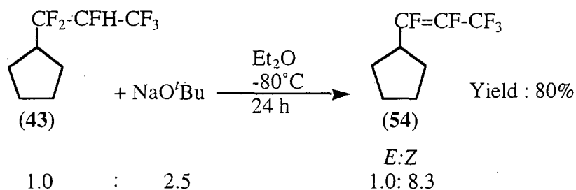
Scheme 85
