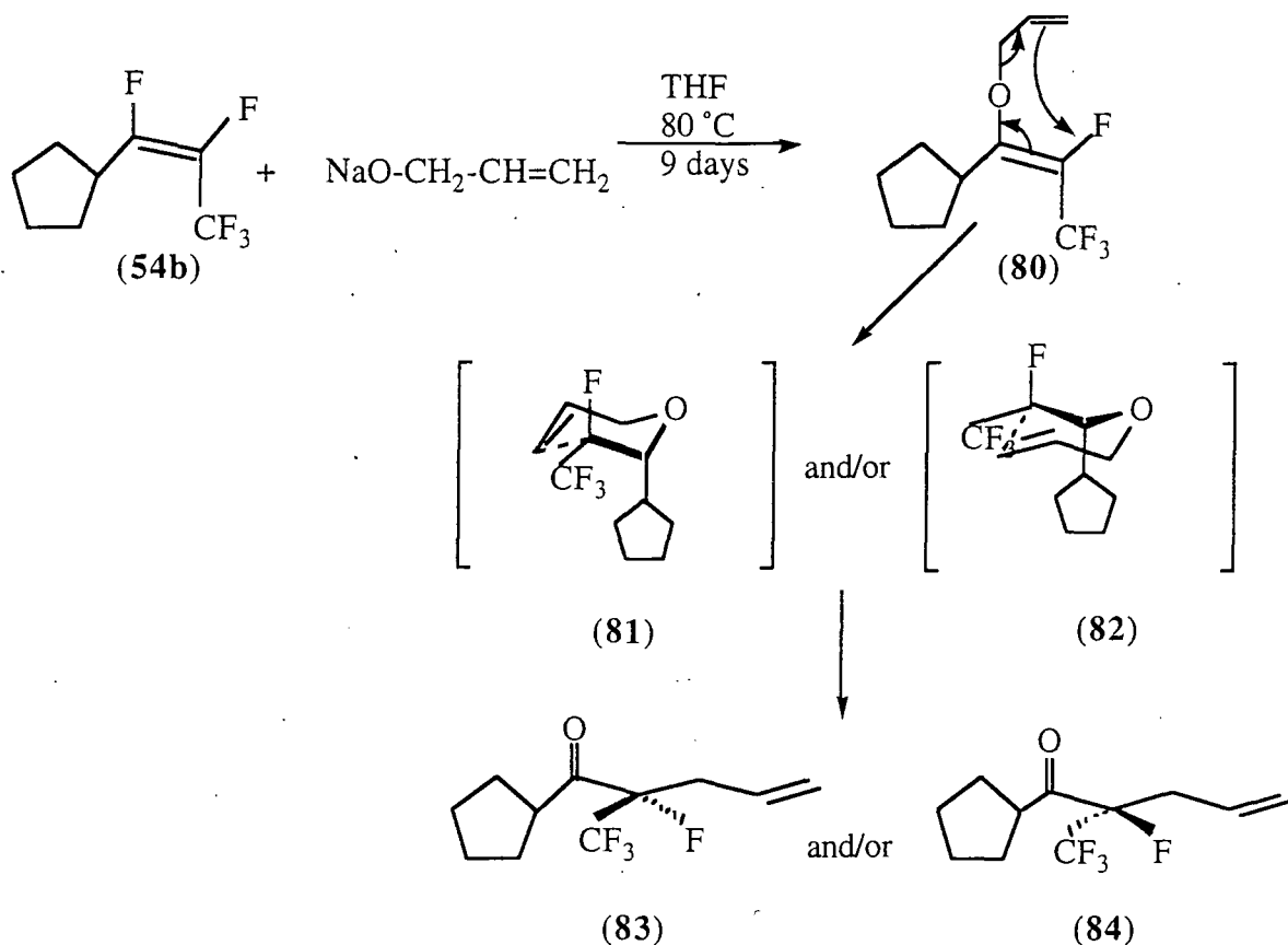
Scheme 133
