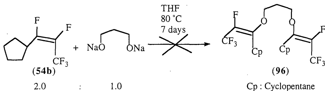
Scheme 151
