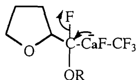
Scheme 100
