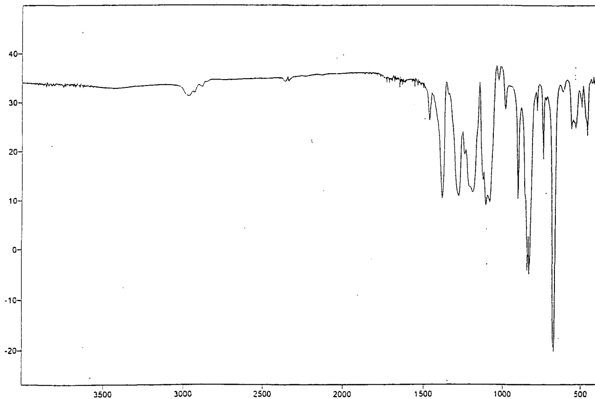
No. 4 1,1,2,3,3,3-hexafluoro-1-[3,5,8-tris(1,1,2,3,3,3-hexafluoropropyl)adamantanyl] propane (42)
