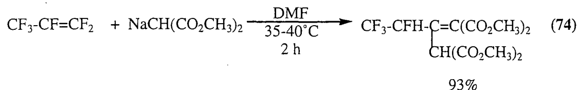
Scheme 116
