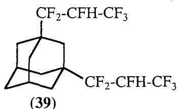
Scheme 55
