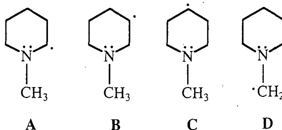
Scheme 173
