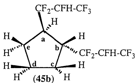
Scheme 64
