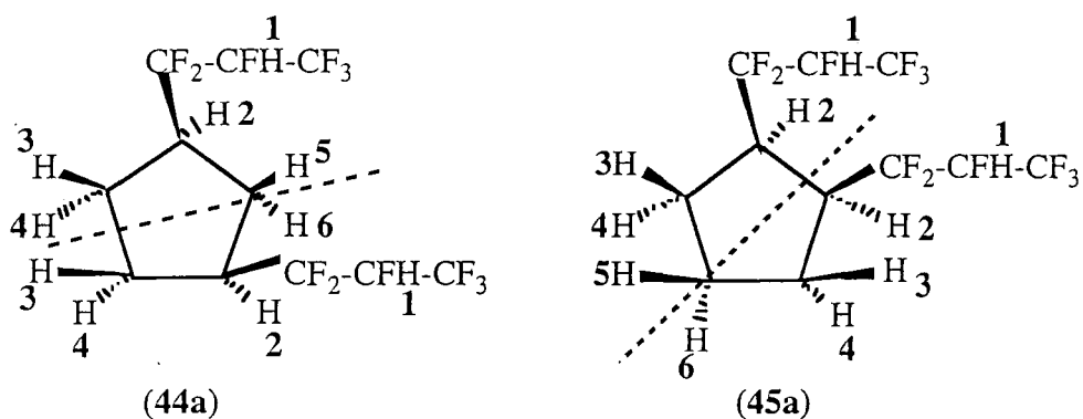
Scheme 61
