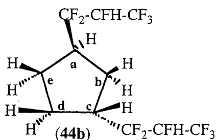
Scheme 65
