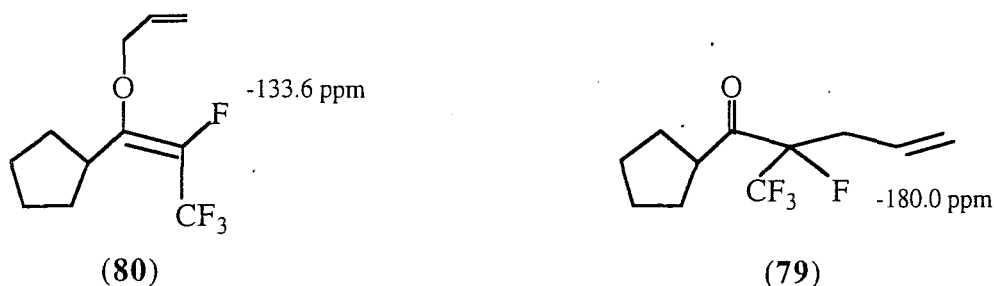
Scheme 134
