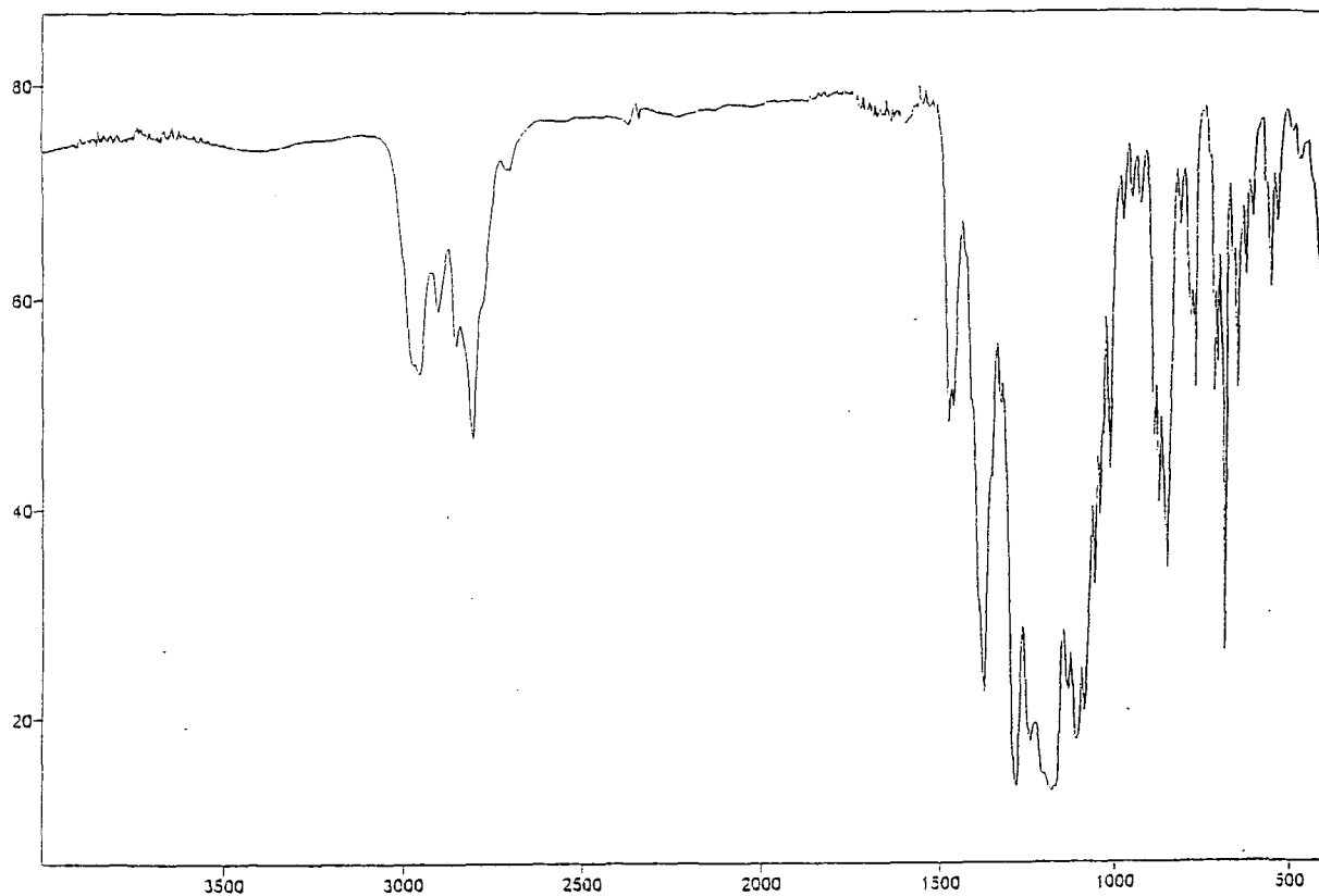
No. 41 1,4-dimethyl-2,3,5-tris(1,1,2,3,3,3-hexafluoropropyl)piperazine (118)
