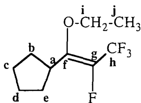
Scheme 128
