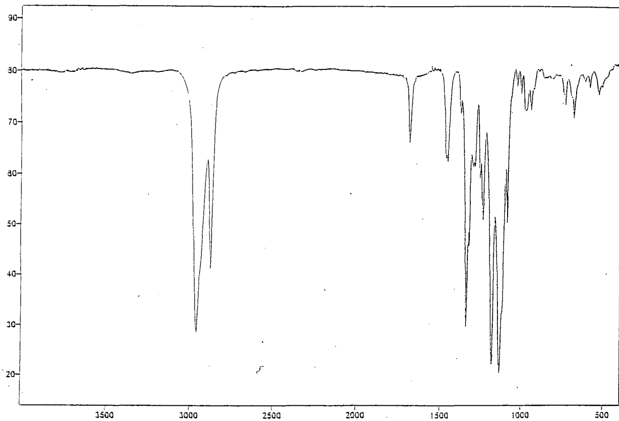
No. 25 Z-(1-phenyl-2,3,3,3-tetrafluoro-1-propenyl)cyclopentane (101)
