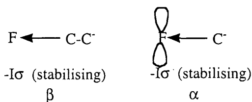
Scheme 93
