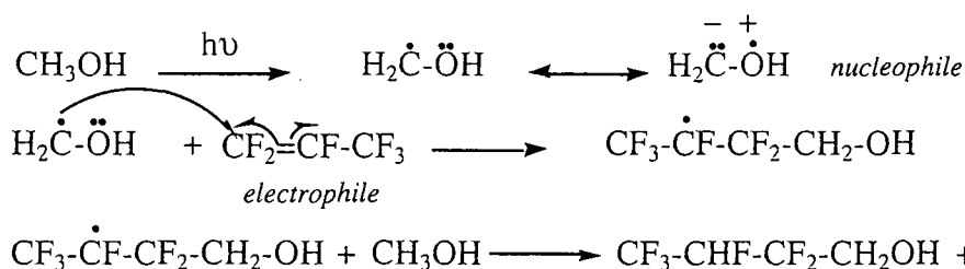
Scheme 23
