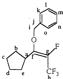
Scheme 149
