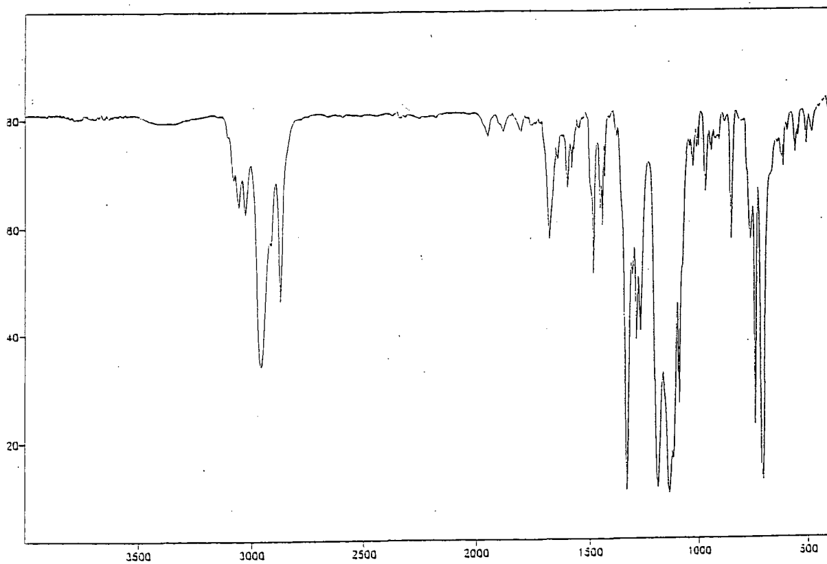
No. 25 Z-(1-phenyl-2,3,3,3-tetrafluoro-1-propenyl)cyclopentane (101)
