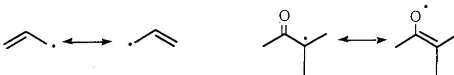
Scheme 9
