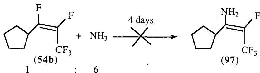
Scheme 152
