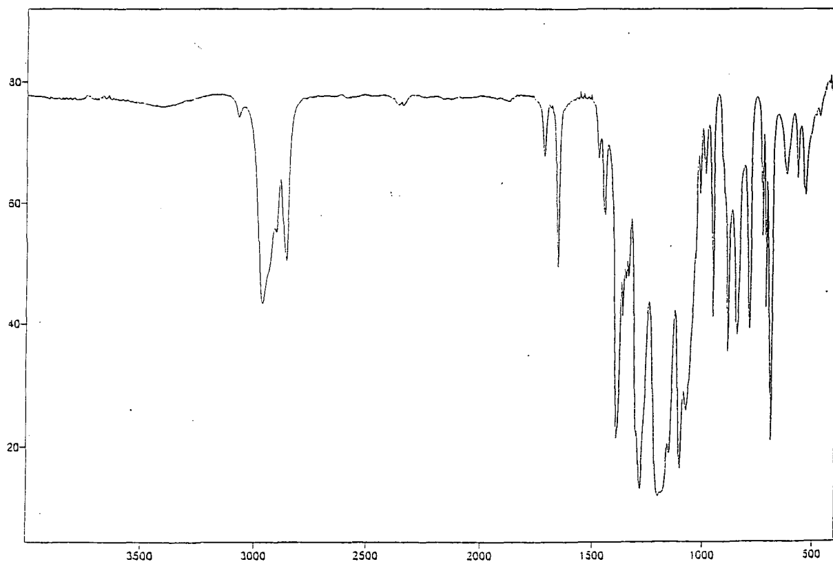
No. 8 1-(1,1,2,3,3,3-hexafluoropropyl)cyclopentene (49)
