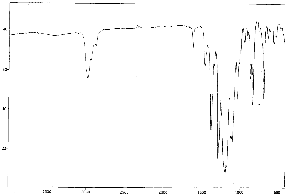
No. 33 2-(1,1,2,3,3,3-hexafluoropropyl)-1-methylpyrrolidine (110)
