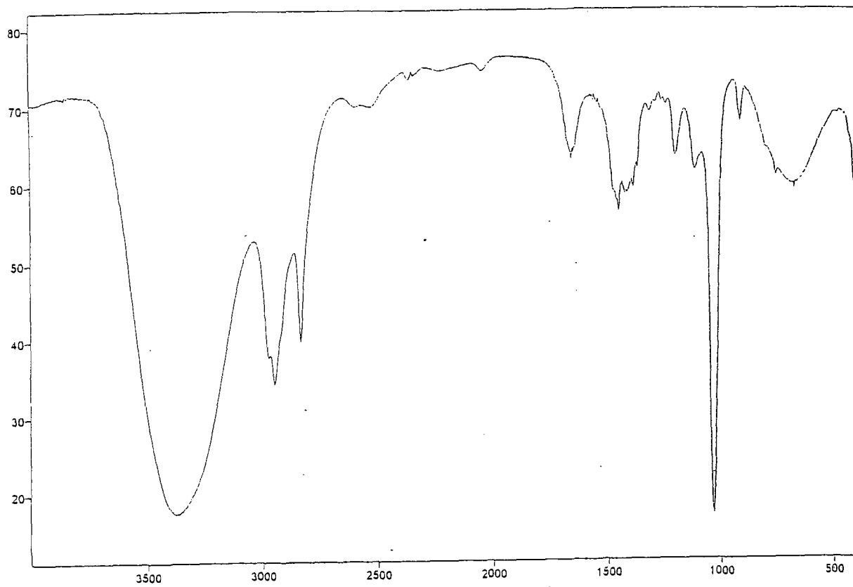
No. 17 1-cyclopentyl-2-fluoro-2-trifluoromethyl-4-penten-1-one (79)
