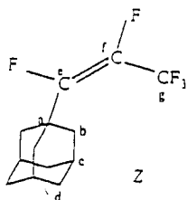
No. 9 (1Z)-1-(adamantanylidene)-1,2,3,3,3-pentafluoroprop-1-ene (53b)
