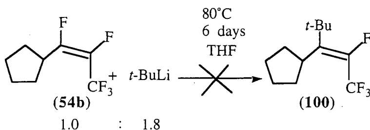
Scheme 155
