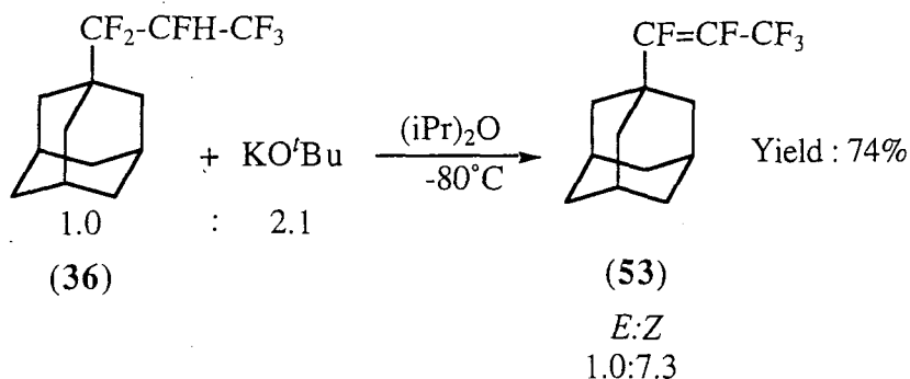
Scheme 84
