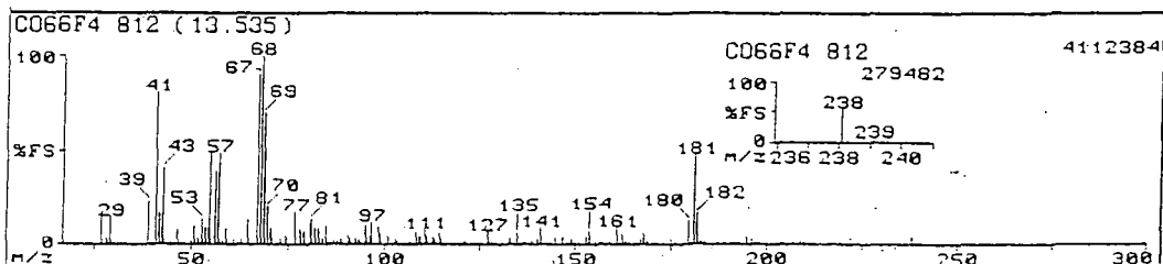
No. 24 Z-(1-butyl-2,3,3,3-tetrafluoro-1-propenyl)cyclopentane (99)
