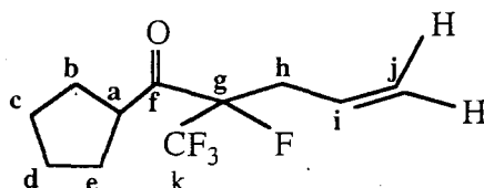
Scheme 137
