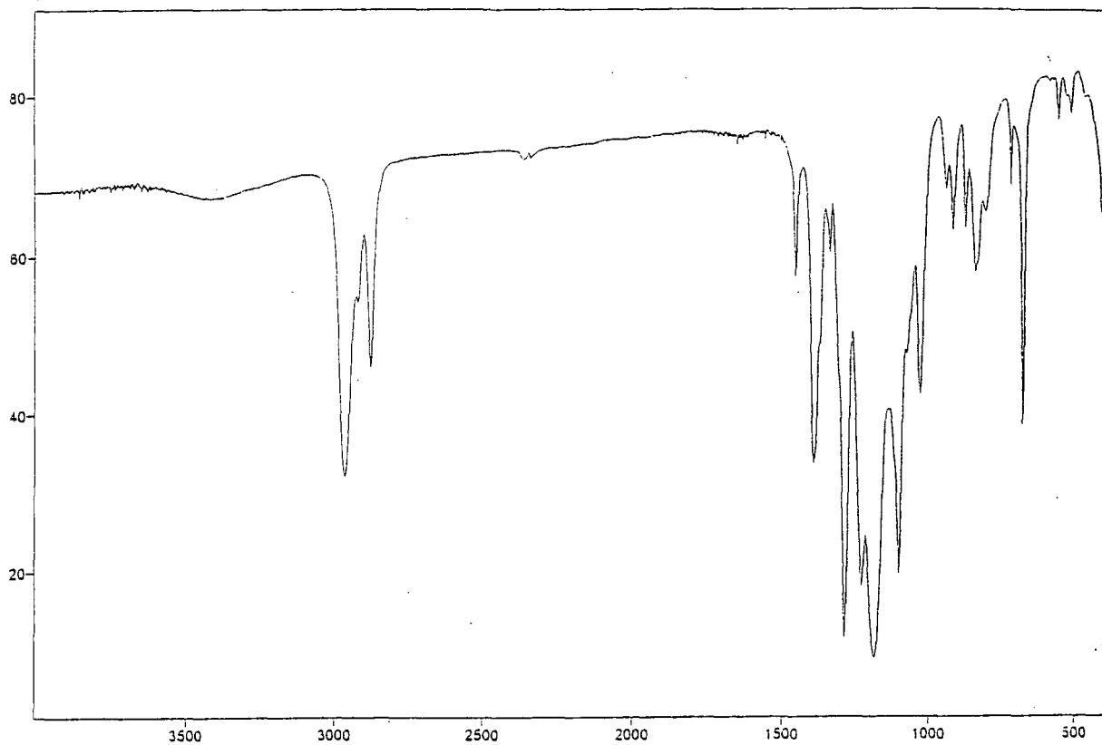
No. 5 1-(1,1,2,3,3,3-hexafluoropropyl)cyclopentane (43)
