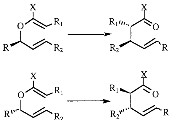
Scheme 106
