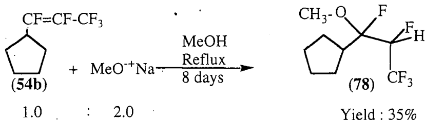
Scheme 131
