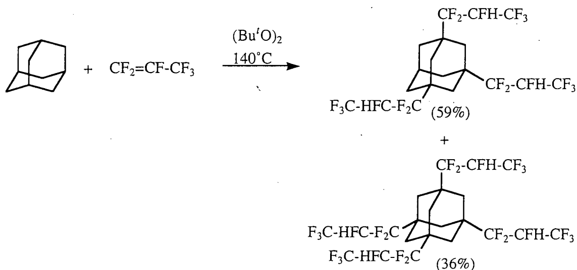
Scheme 45
