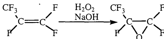
Scheme 122
