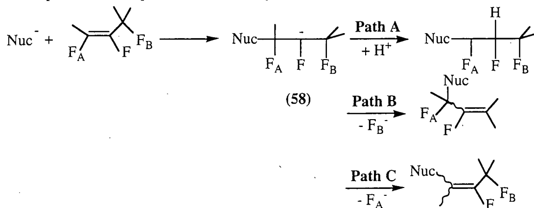
Scheme 92
